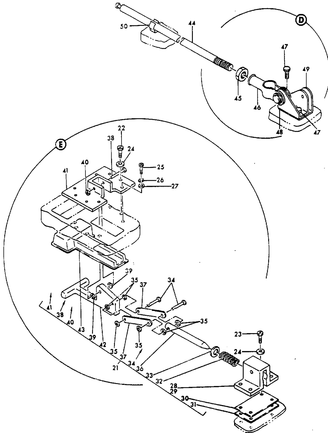
FIGURE 34. POD ASSY, MARK IV (SHEET 3)
