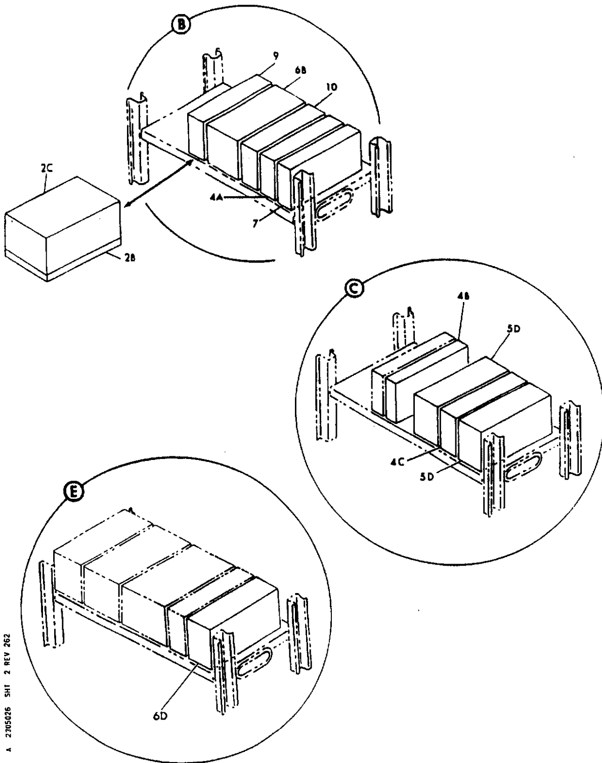
FIGURE 26. EQUIPMENT INSTL, LH RADIO RACK (COMMUNICATIONS ONLY) (SHEET 2)
