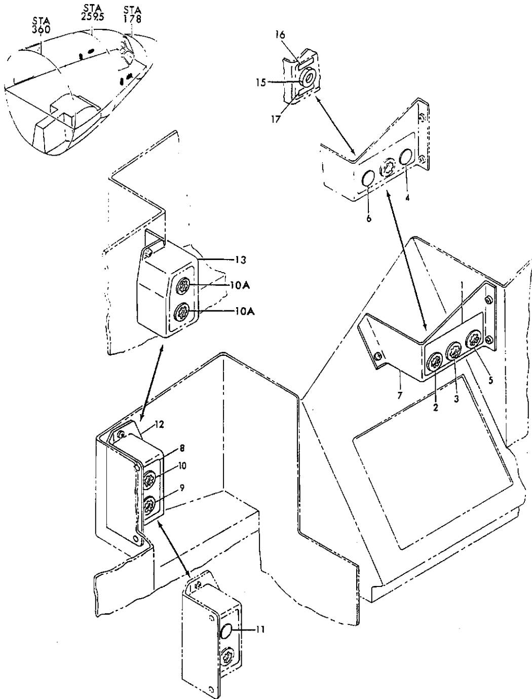
FIGURE 9D. BOX INSTL, CREW INTERPHONE JACK BOX INSTL, CREW OXYGEN MASK JACK
