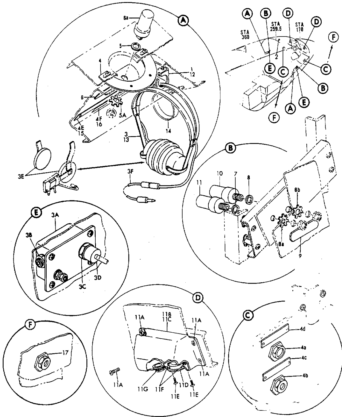
HANGER AND JACK INSTL, PILOT AND COPILOT INTERPHONE HEADSET SUPPORT INSTL, PILOT AND COPILOT HEADSET INTERPHONE JACK FIGURE L HANGER INSTL, PILOT AND COPILOT MASK AND HEADSET
