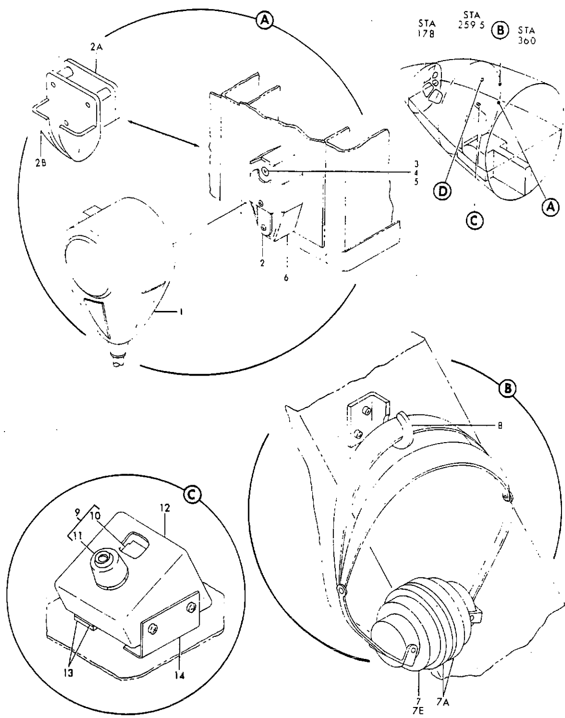
FIGURE 33P. INTERPHONE INSTL., FLIGHT ENGINEER (COMMUNICATIONS ONLY) (SHEET 1)
