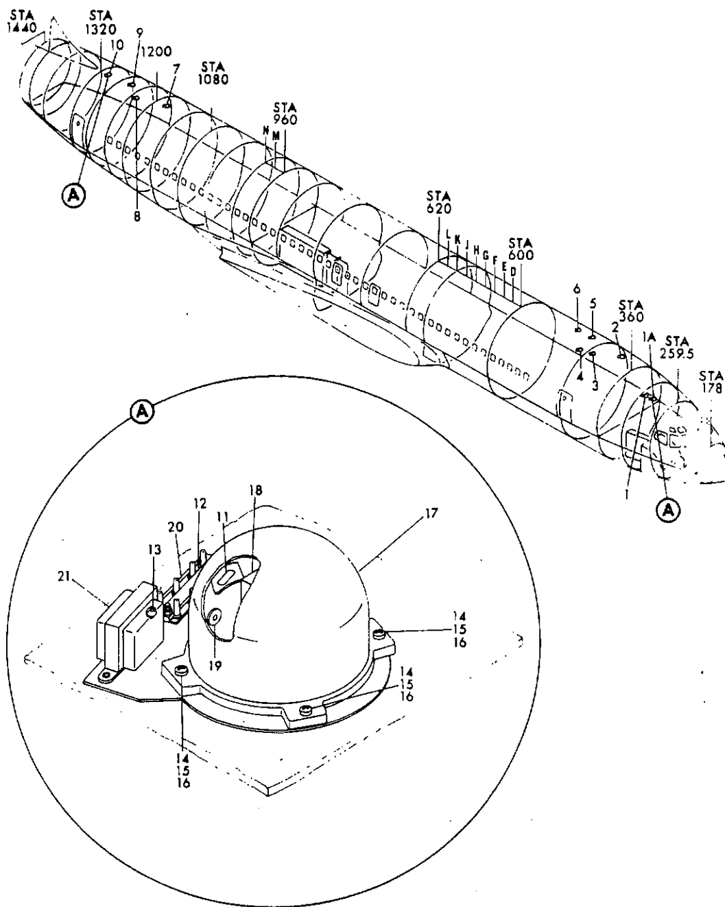
FIGURE 49A. SPEAKER INSTL, LOWERED CEILING
