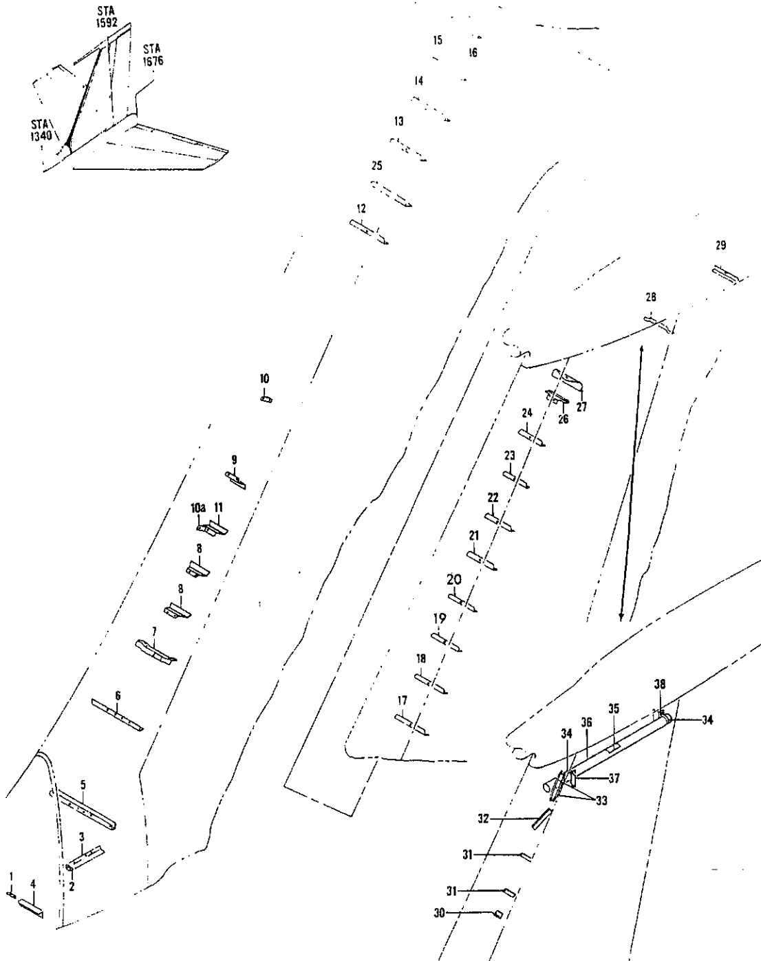
FIGURE 8. SUPPORT INSTL, FIN ELECTRONICS WIRE
