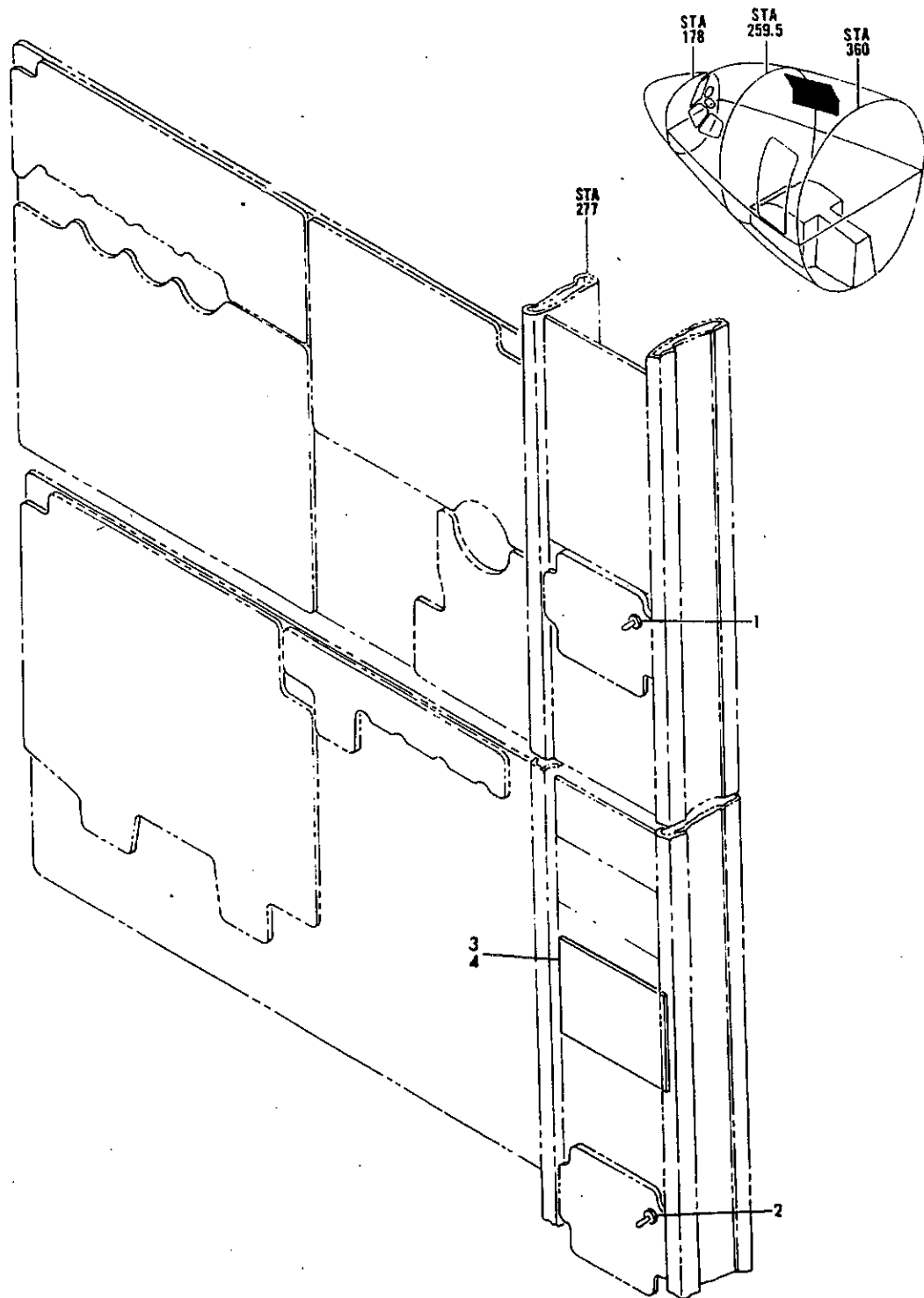
FIGURE 76G. PANEL INSTL, FLIGHT ENGINEERS AUXILIARY (COMMUNICATIONS ONLY)
