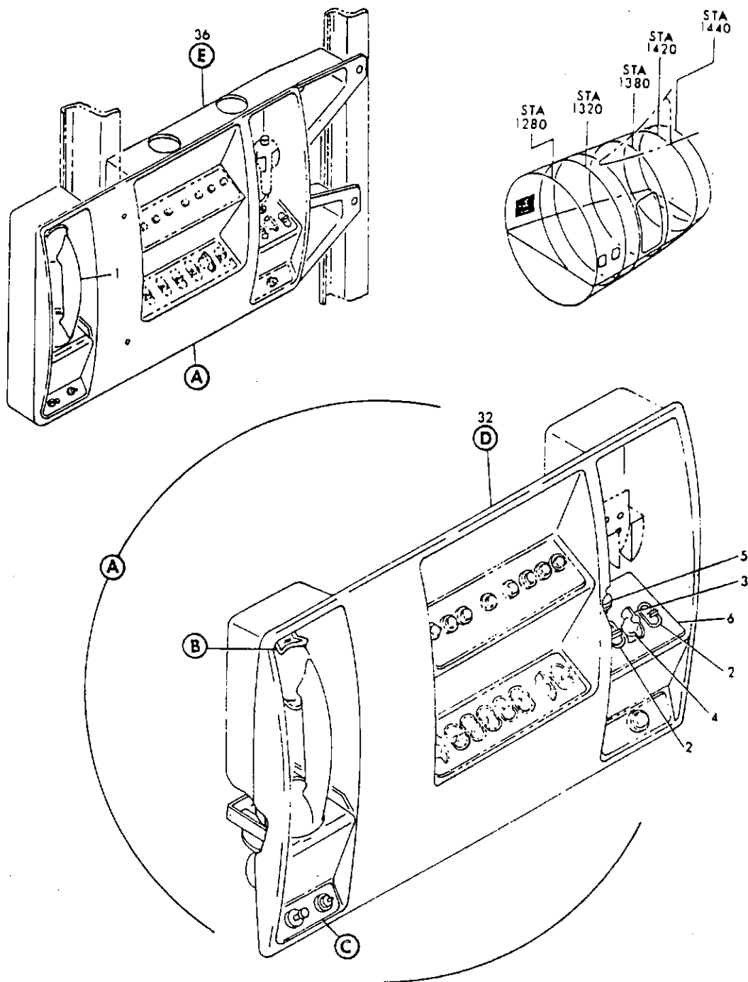
FIGURE 123M. PANEL INSTL, AFT GALLEY ATTENDANTS (COMMUNICATIONS ONLY) (SHEET 1)
