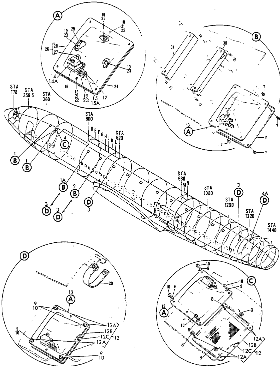
FIGURE 50. SPEAKER INSTL, CARGO COMPARTMENT CEILING
