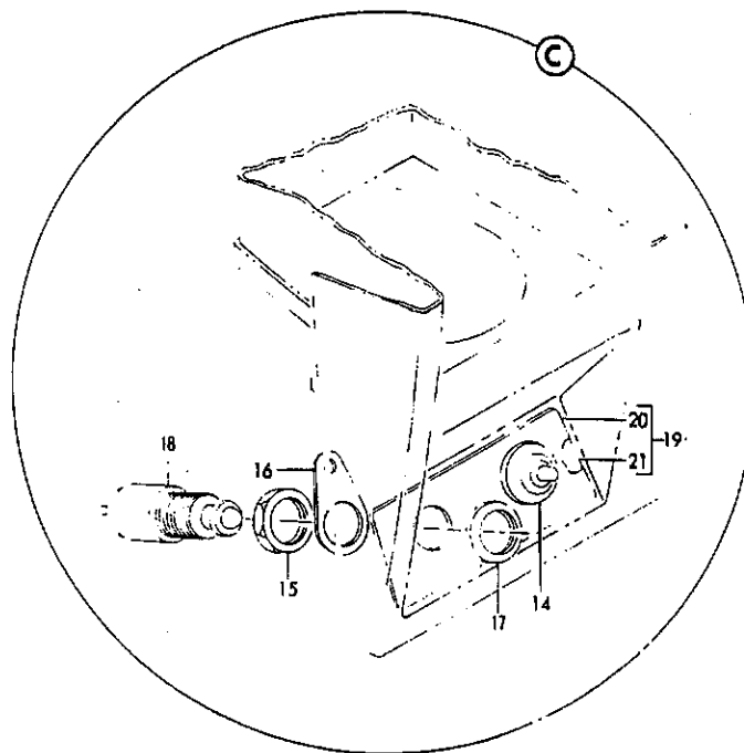
FIGURE 123C. PANEL INSTL, AFT GALLEY ATTENDANTS (COMMUNICATIONS ONLY) (SHEET 2)
