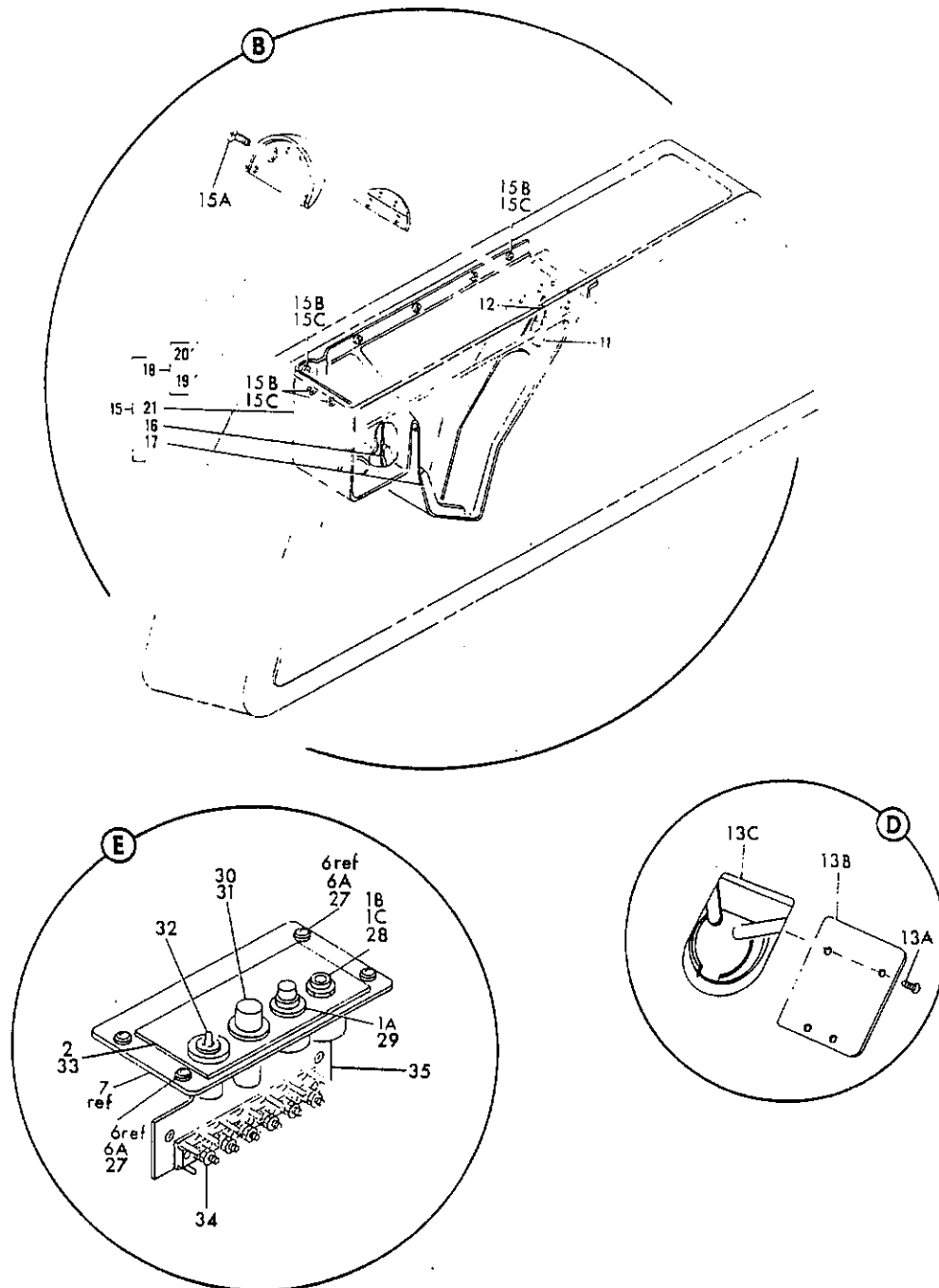
FIGURE 155. PANEL INSTL, ATTENDANTS BOLSTER AUXILIARY (SHEET 2)
