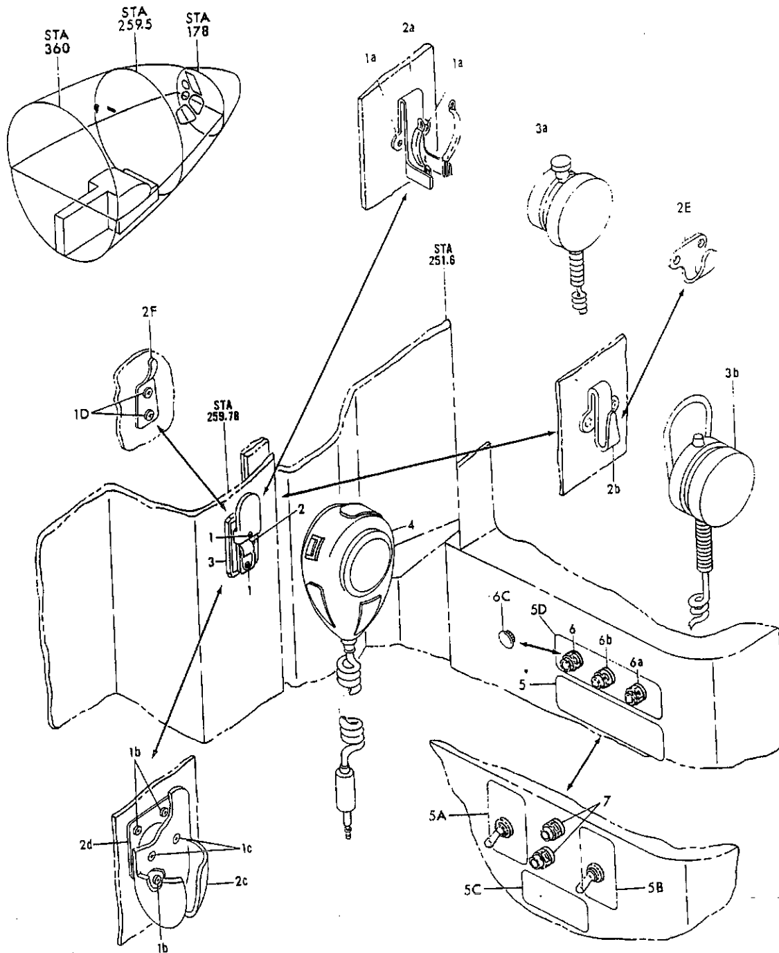
MICROPHONE INSTL, OBSERVER INTERPHONE HOLDER INSTL, OBSERVER INTERPHONE MICROPHONE FIGURE 17F, JACK INSTL, OBSERVER INTERPHONE
