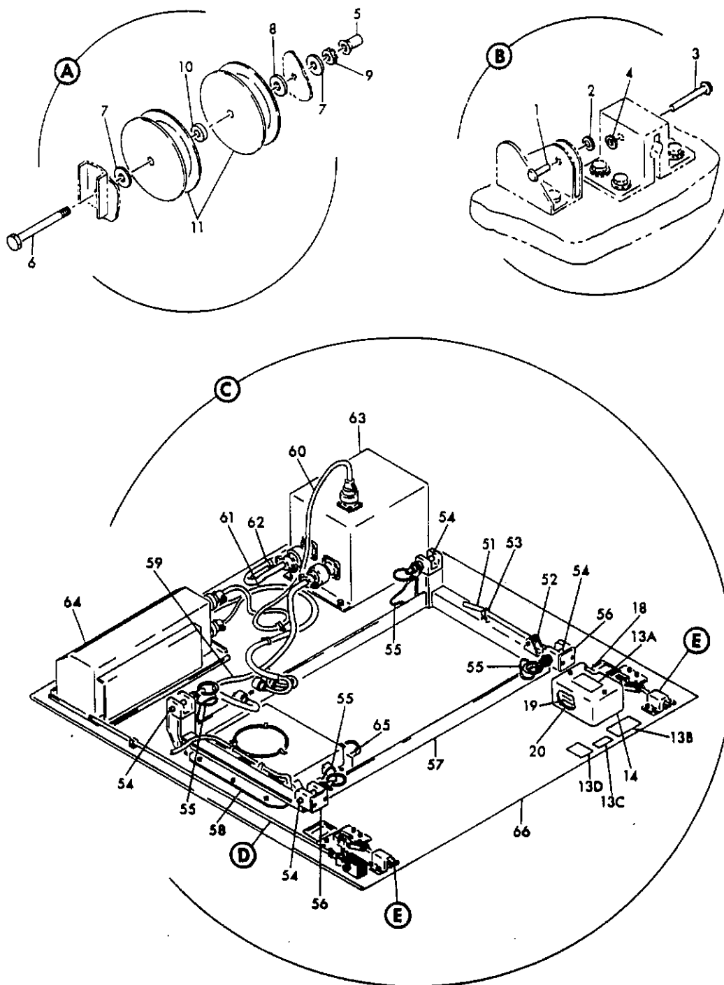
FIGURE 34. POD ASSY, MARK IV (SHEET 2)
