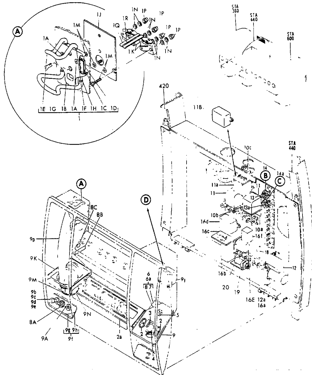
FIGURE 113B. PANEL INSTL, FORWARD ATTENDANTS (COMMUNICATIONS ONLY) (SHEET 1)
