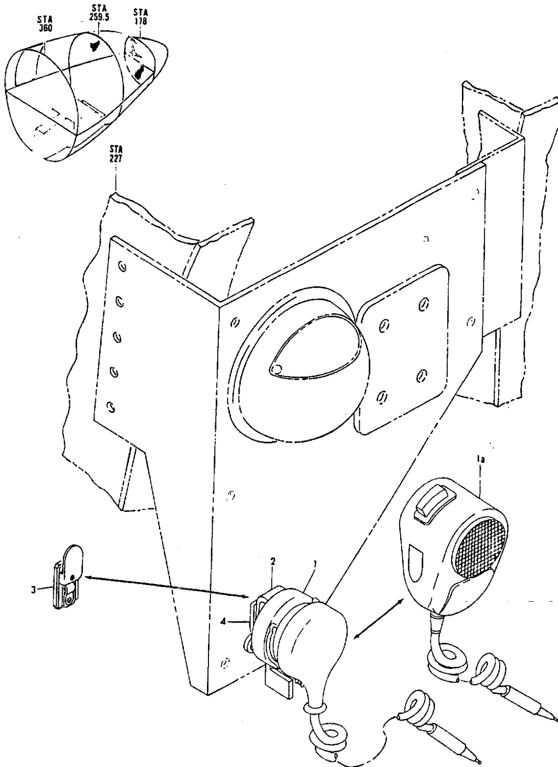
FIGURE 62P. PANEL INSTL, PILOTS AND COPILOTS AUXILIARY EQUIPMENT (COMMUNICATIONS ONLY)
