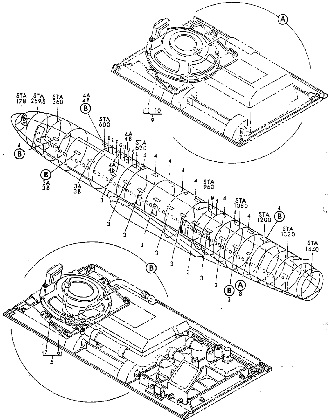
FIGURE 143A, SERVICE UNIT INSTL, PASSENGER (COMMUNICATIONS ONLY)
