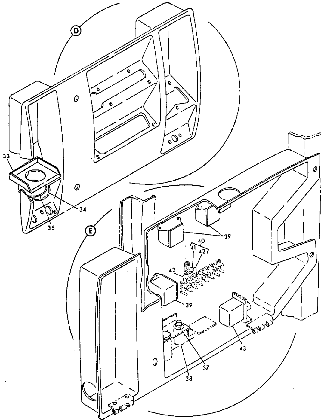
FIGURE 123M. PANEL INSTL, AFT GALLEY ATTENDANTS (COMMUNICATIONS ONLY) (SHEET 3)
