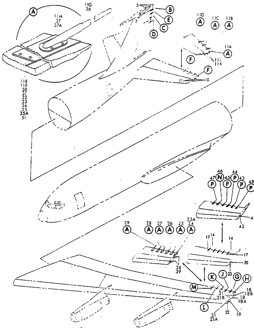
FIGURE 21. DISCHARGER INSTL, DECOUPLED STATIC (SHEET 1)
