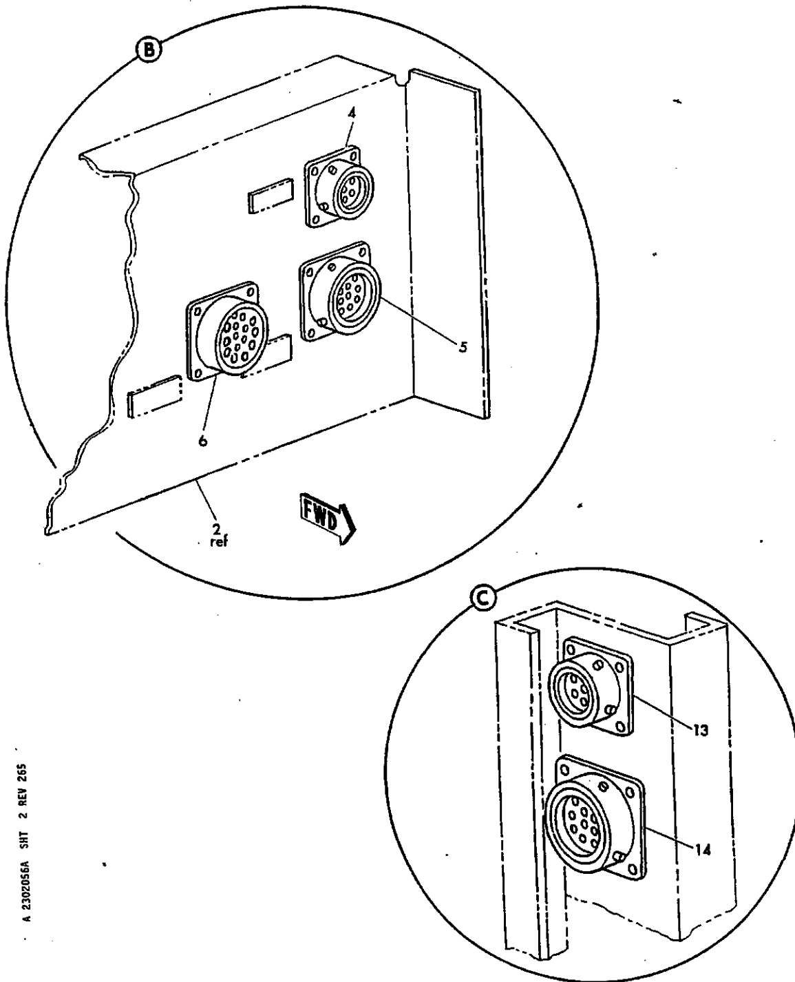
FIGURE 56A. INTERCOM BOX INSTL. (SHEET 2)
