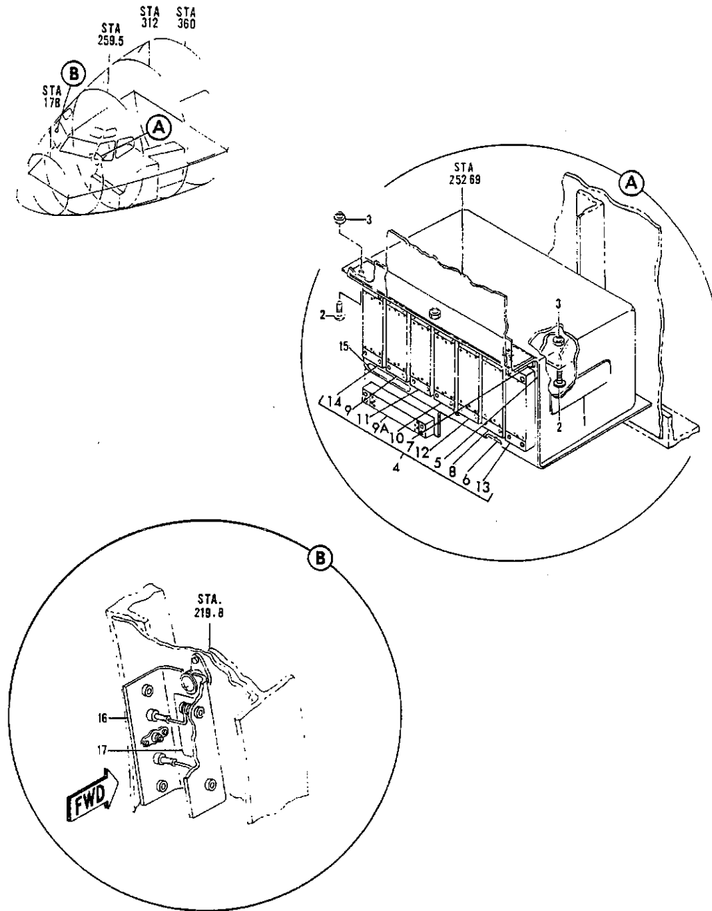
FIGURE 54. BOX INSTL, RJ4 INTERPHONE SYSTEM INTERCONNECTION
