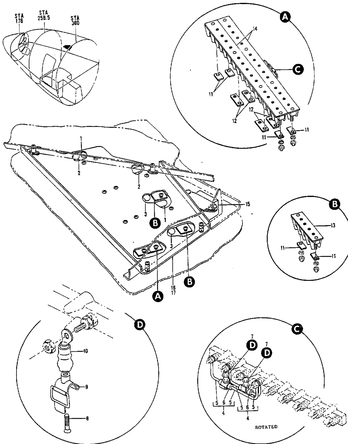
FIGURE 83. PANEL INSTL, ENGINEERS INTERPHONE TERMINAL
