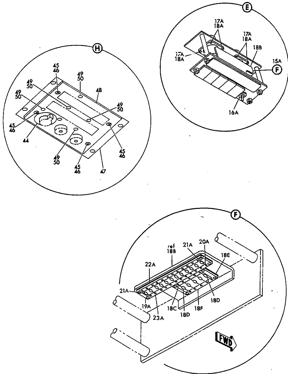
FIGURE 31G. MODULE INSTL, P13 PILOTS OVERHEAD (COMMUNICATION ONLY) (SHEET 3)
