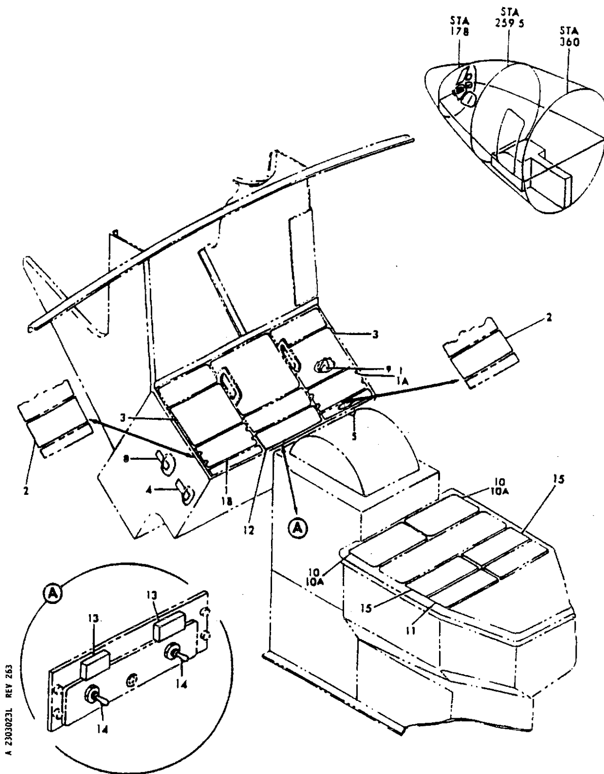
FIGURE 23L. PANEL INSTL. RADIO, RADAR AND AUTOPILOT CONTROL (COMMUNICATIONS ONLY)
