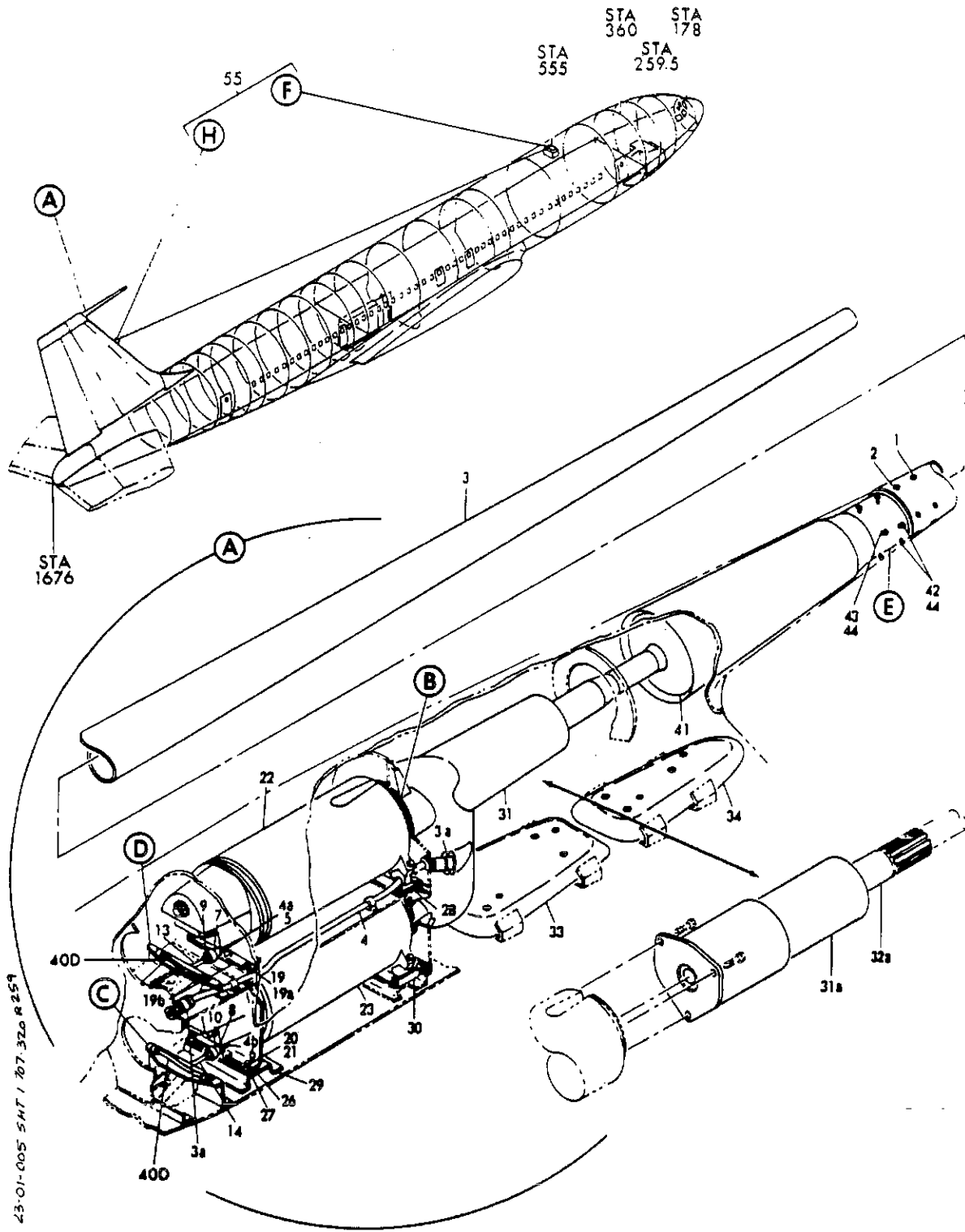
FIGURE 5. ANTENNA AND COMPONENTS INSTL, FIN HF COMMUNICATION (COMMUNICATIONS ONLY) (SHEET 1)
