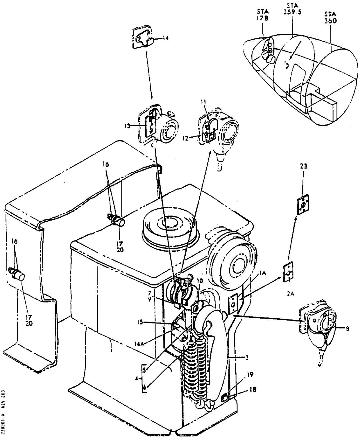
FIGURE 10A. STAND ASSY. PILOT AND COPILOT CONTROL (COMMUNICATIONS ONLY)
