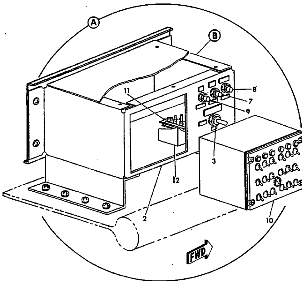
FIGURE 56A. INTERCOM BOX INSTL. (SHEET 1)
