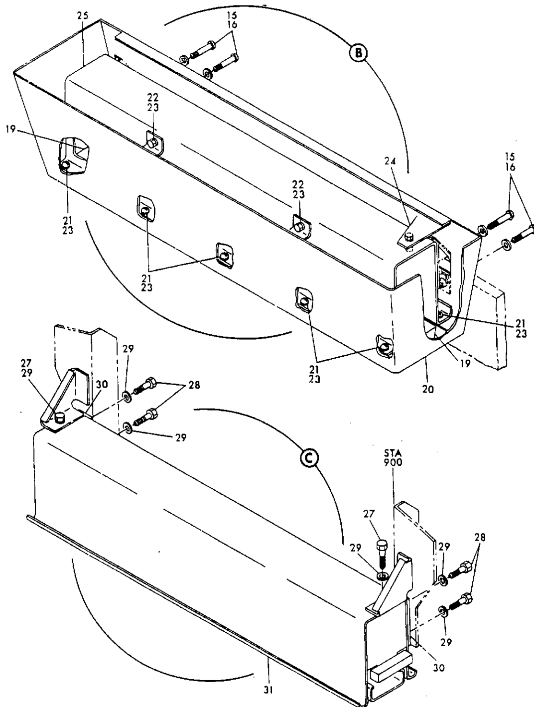
FIGURE 18. SCREEN INSTL. ROLL (SHEET 2)
