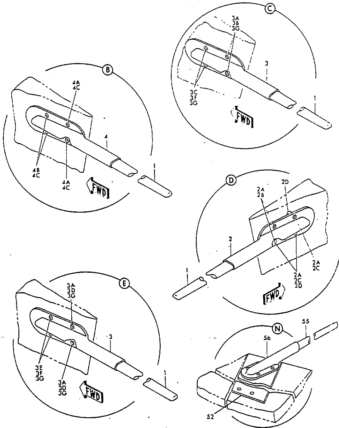
FIGURE 21. DISCHARGER INSTL, DECOUPLED STATIC (SHEET 2)
