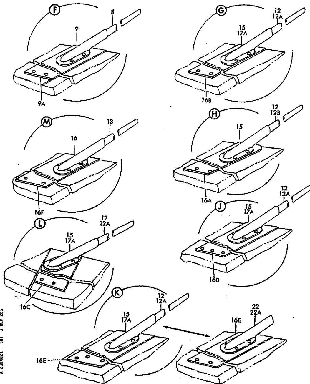
FIGURE 21. DISCHARGE INSTL, DECOUPLED STATIC (SHEET 3)
