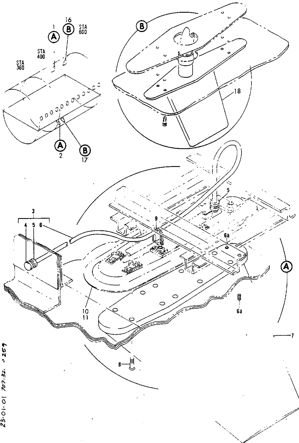
FIGURE 1. ANTENNA INSTL, STATION 470 UPPER AND 490 LOWER VHF COMMUNICATION SUPPORT INSTL, STATION 470 UPPER AND 490 LOWER UHF ANTENNA
