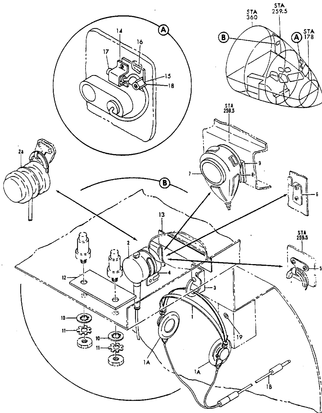
FIGURE 16. EQUIPMENT INSTL, OBSERVER INTERPHONE
