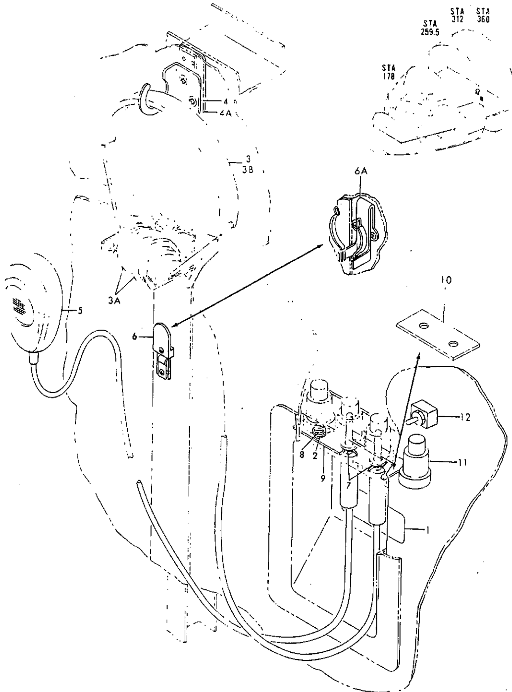
FIGURE 14B. COMMUNICATION-INTERPHONE SYSTEM
