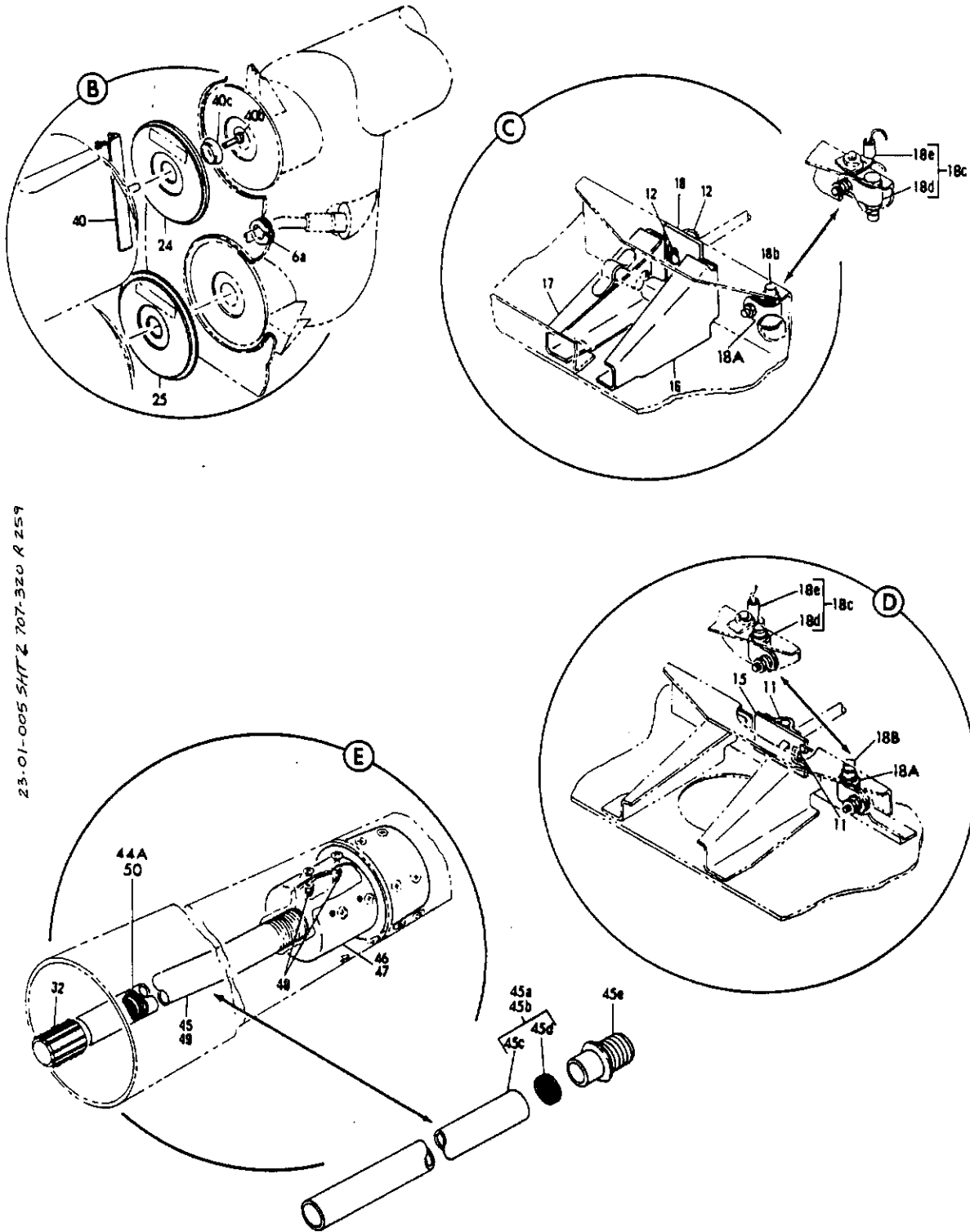
FIGURE 5. ANTENNA AND COMPONENTS INSTL, FIN HF COMMUNICATION (COMMUNICATIONS ONLY) (SHEET 2)
