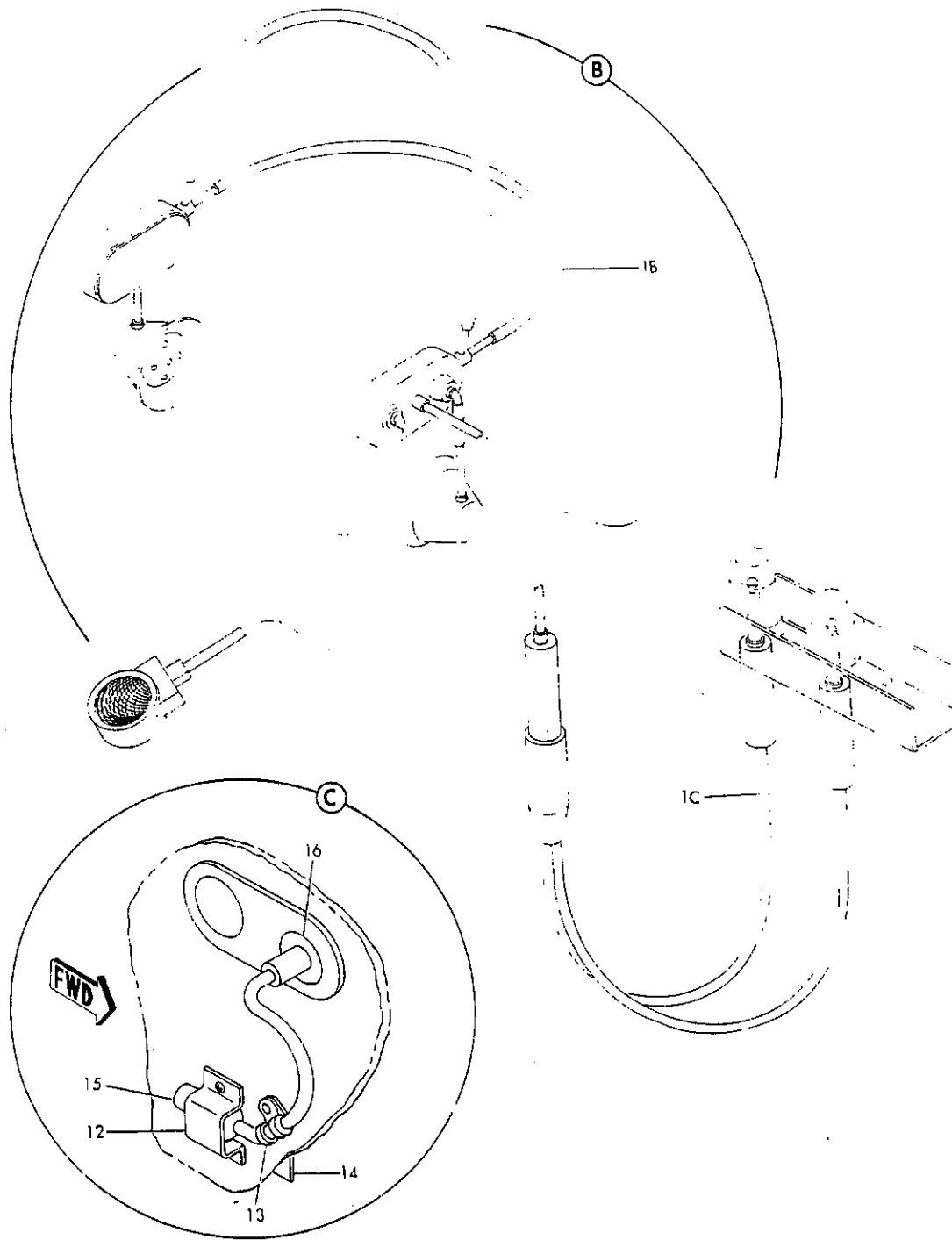
INTERPHONE INSTALLATION FIGURE 14. JACK INSTL, NAVIGATOR OXYGEN MICROPHONE (SHEET 2)
