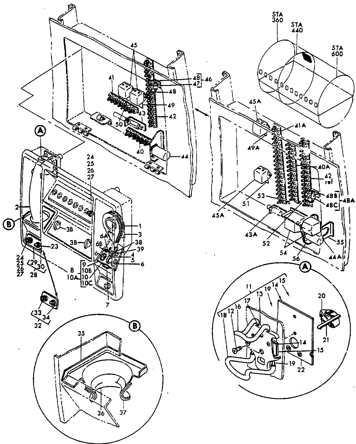
FIGURE 112E. PANEL INSTL, FORWARD GALLEY ATTENDANTS (COMMUNICATIONS ONLY)
