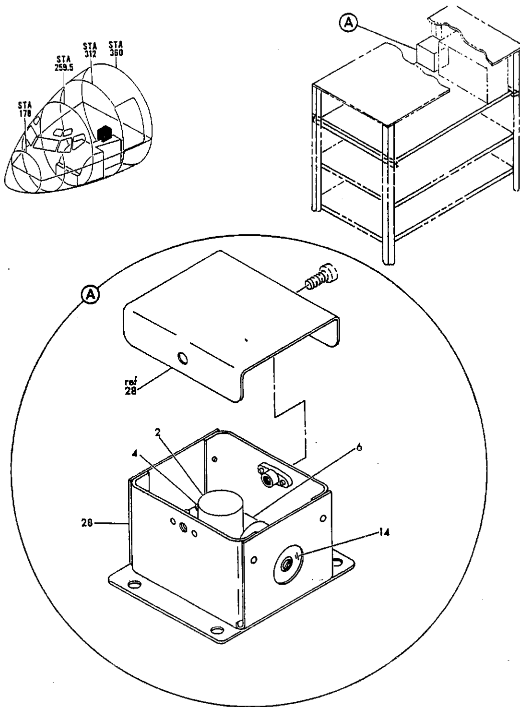
FIGURE 212 EQUIPMENT INSTL, COMMUNICATION SYS (SHEET 1)
