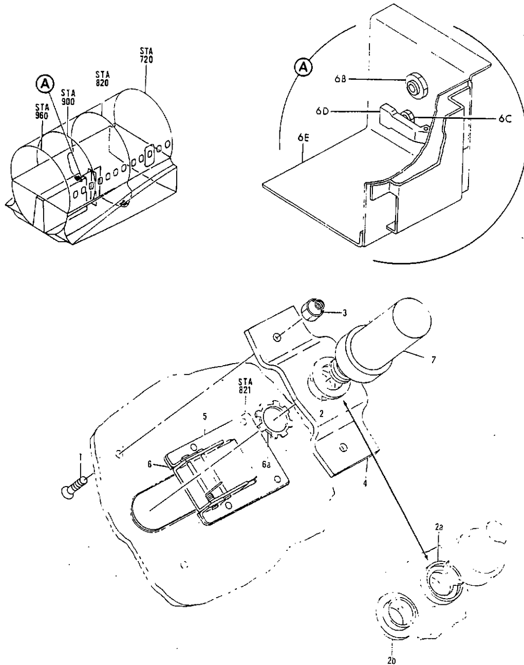
FIGURE 45. JACK INSTL. WHEEL WELL INTERPHONE BUNDLE ASSY, WHEEL WELL INTERPHONE JACKS ELECTRICAL
