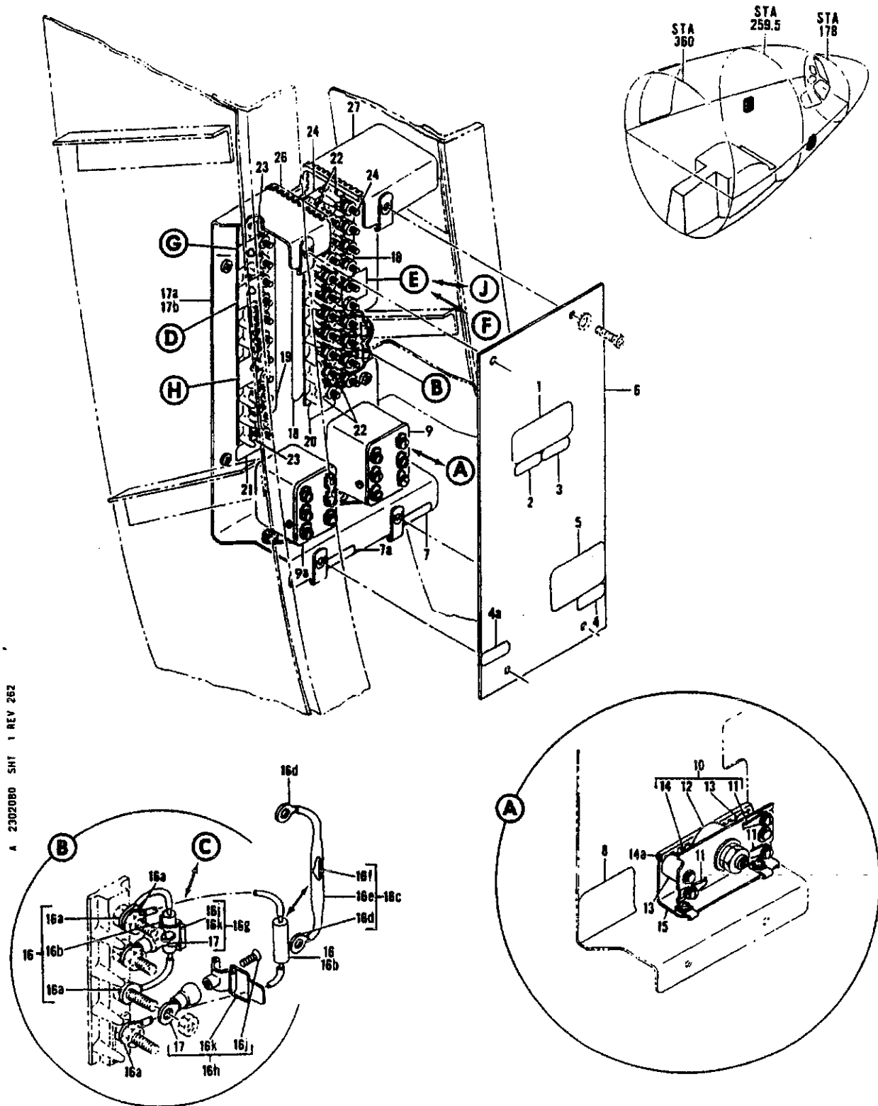
FIGURE 80. PANEL INSTL. RJ17 AND RJ18 INTERPHONE (SHEET 1)
