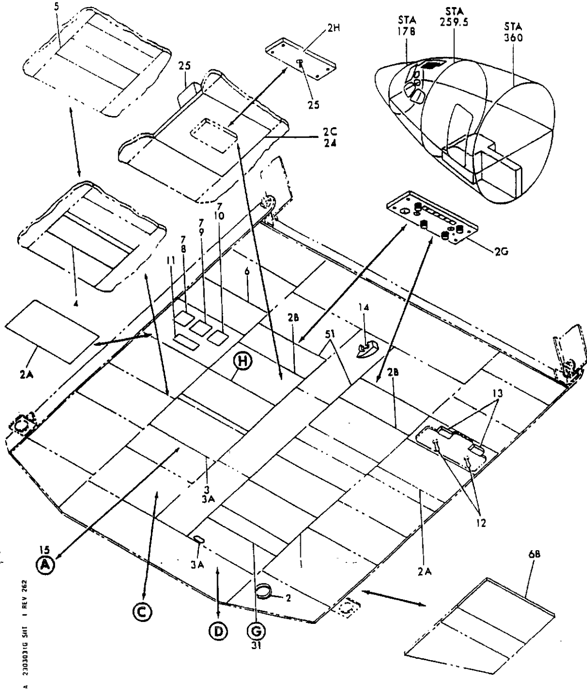
FIGURE 31G. MODULE INSTL. P13 PILOTS OVERHEAD (COMMUNICATIONS ONLY) (SHEET 1)
