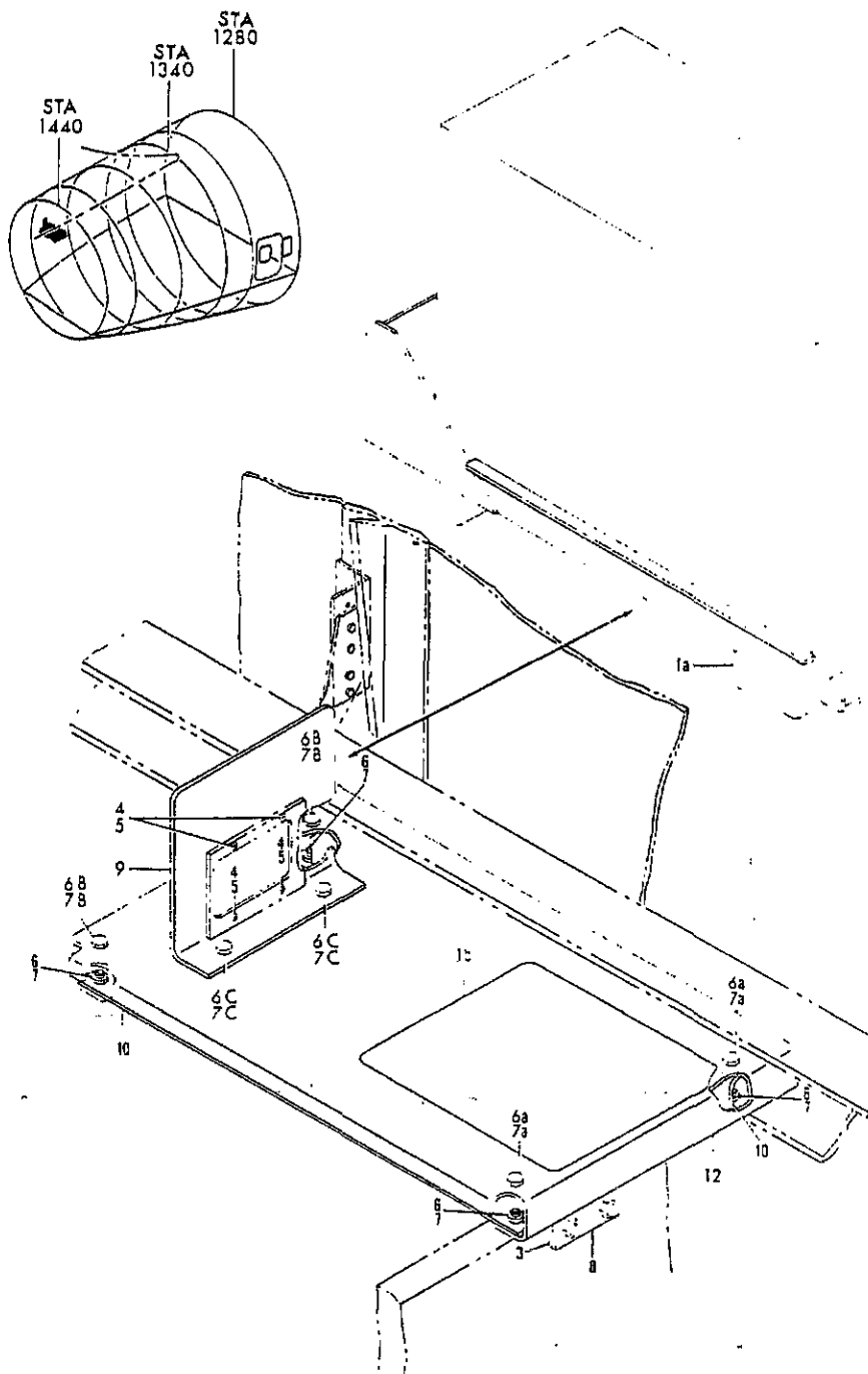
FIGURE 45. SHELF INSTL, STATION 1440 VOICE RECORDER (COMMUNICATIONS ONLY) VOICE RECORDER INSTL, STATION 1440 (COMMUNICATIONS ONLY)
