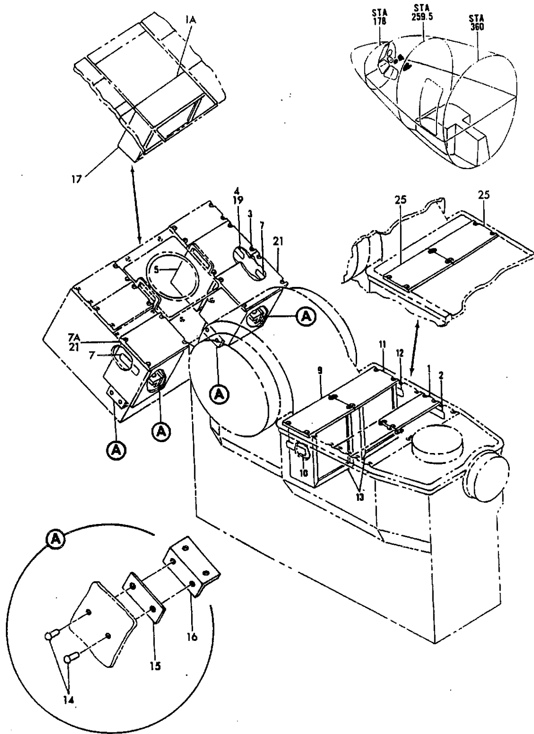
FIGURE 23B. PANEL INSTL, RADIO, RADAR AND AUTOPILOT CONTROL (COMMUNICATIONS ONLY)
