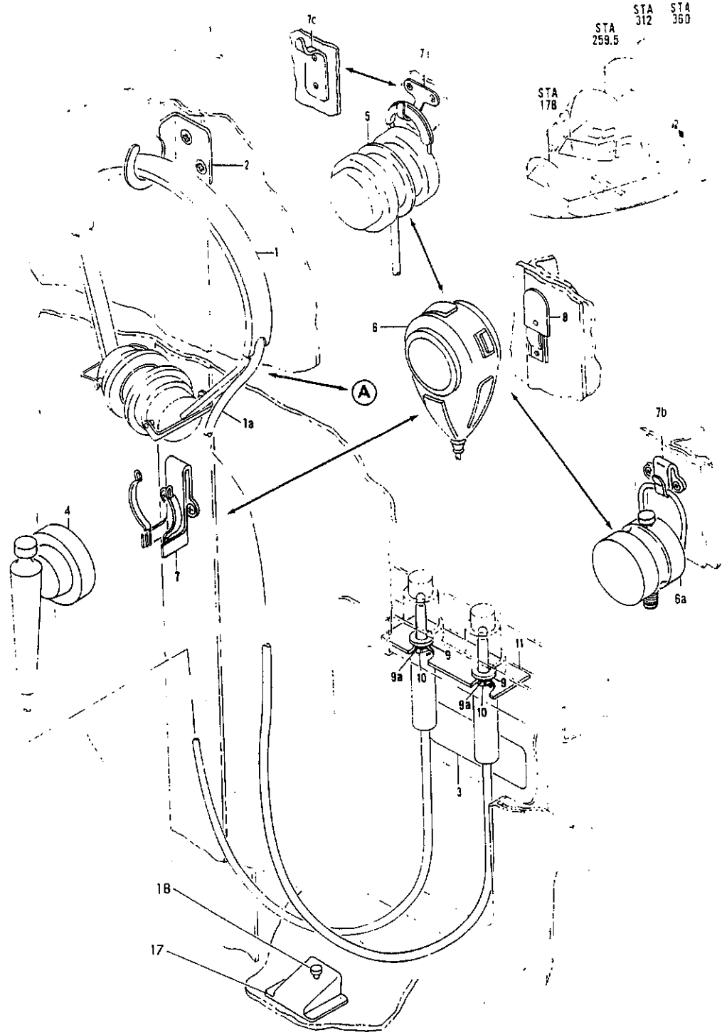
FIGURE 14. INTERPHONE INSTL. NAVIGATORS (SHEET 11)
