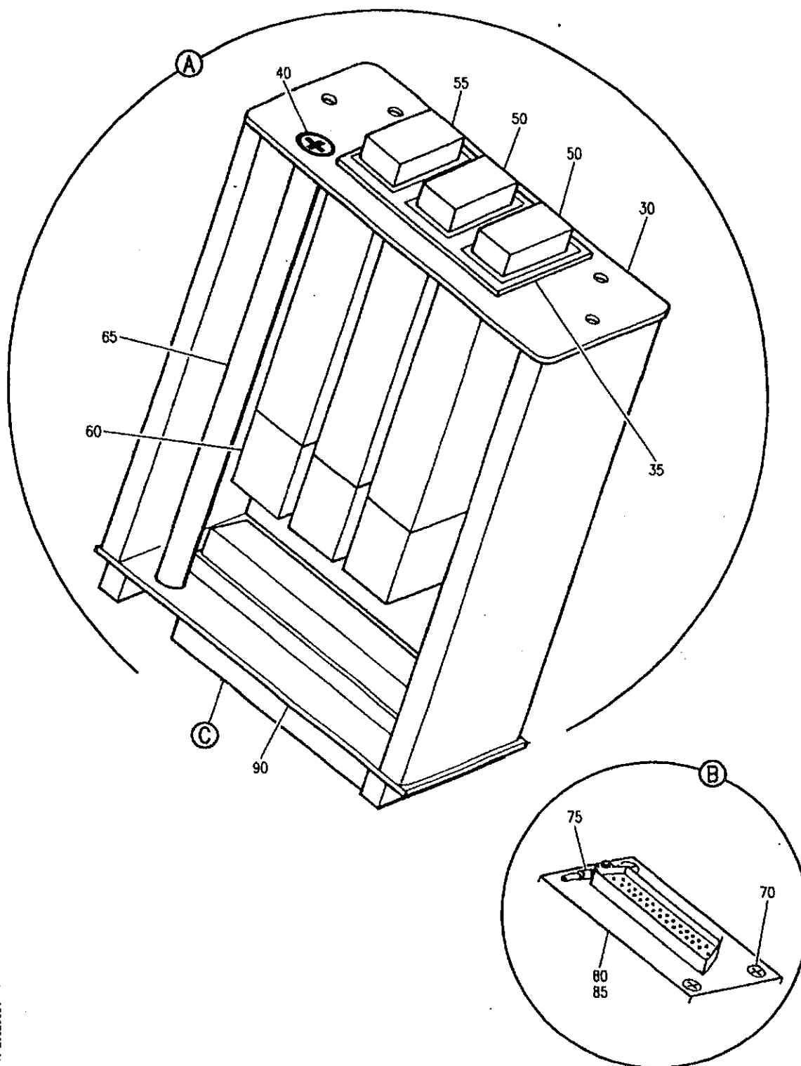
COMMUNICATIONS - INTERPHONE SYSTEM FIGURE 62C. PANEL INSTL, PILOT AUXILIARY EQUIPMENT (SHEET-2)
