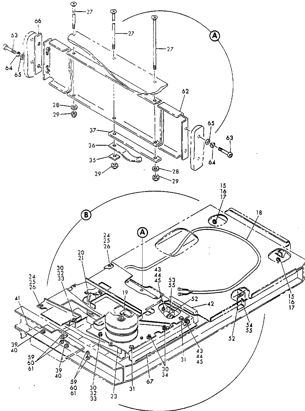
FIGURE 36. FRAME ASSY, MARK IV PROJECTOR (SHEET 2)
