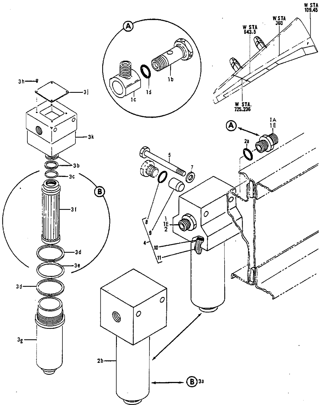
FIGURE 28. FILTER INSTL, AUXILIARY PRESSURE HYDRAULIC (HYDRAULIC POWER ONLY)
