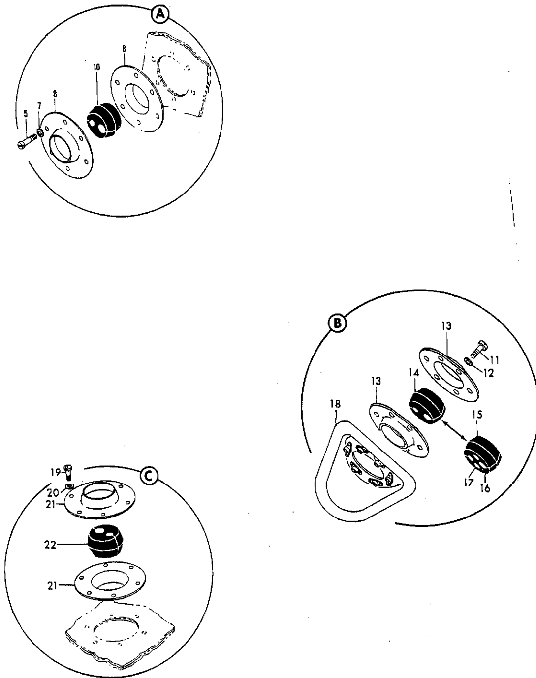
FIGURE 20. HYDRAULIC INSTL, SECTION 46 AND 48 (SHEET 2)
