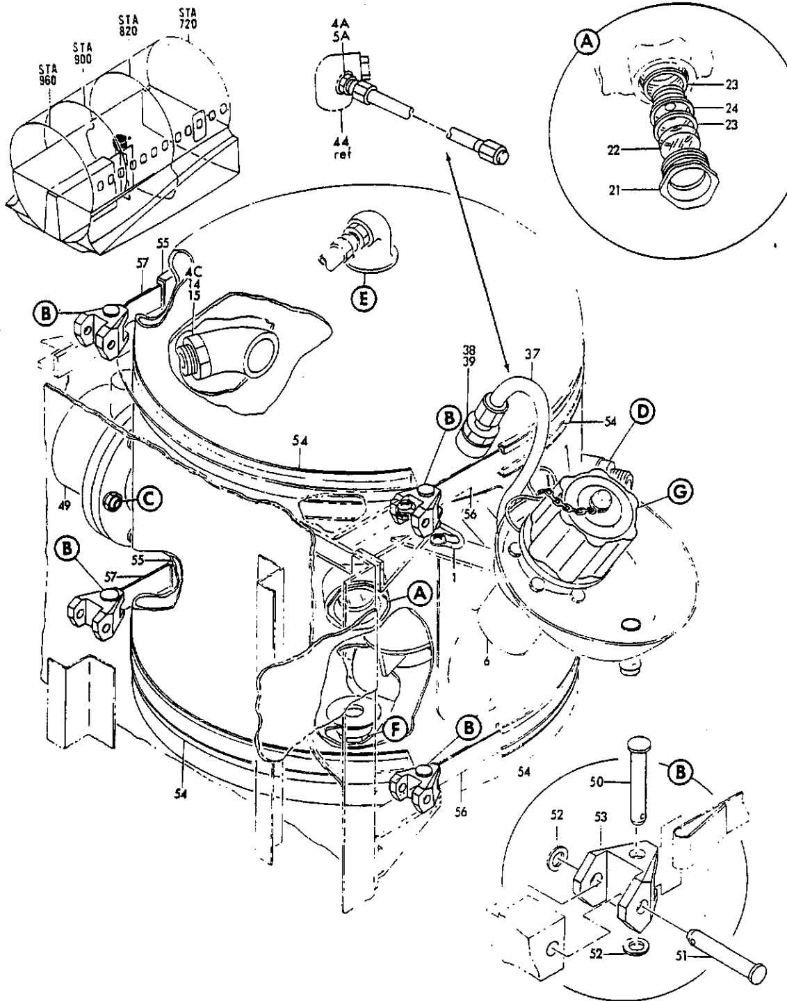
FIGURE 31A. RESERVOIR INSTL, HYDRAULIC (HYDRAULIC POWER ONLY) (SHEET 1)
