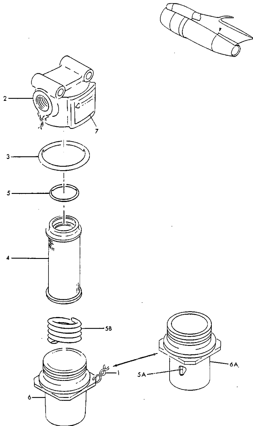
FIGURE 15A. FILTER ASSY, HYDRAULIC
