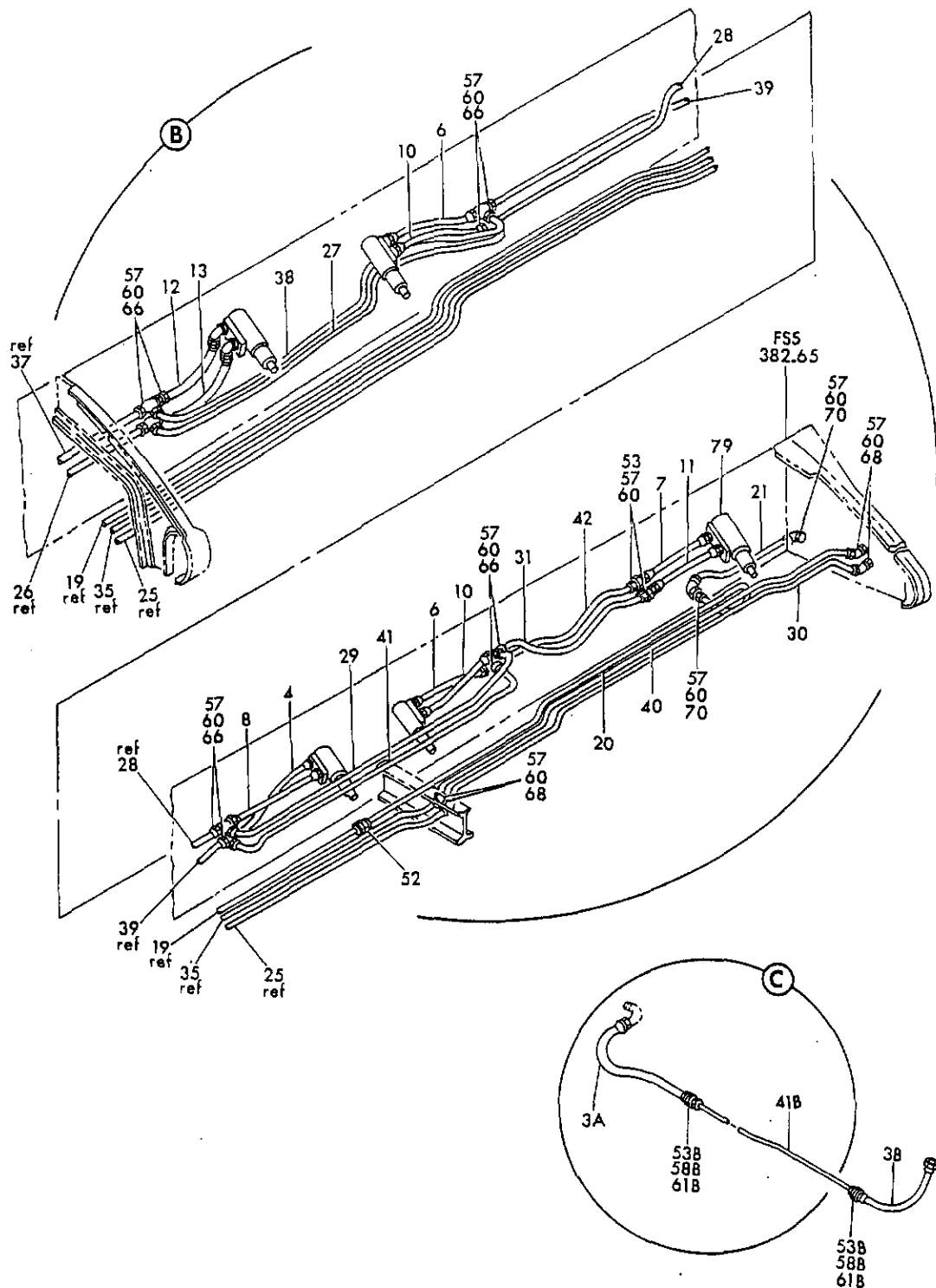
FIGURE 10. HYDRAULIC INSTL. WING (BODY SEAT TO FRONT SPAR STATION 382.65) (HYDRAULIC POWER ONLY) (SHEET 2)
