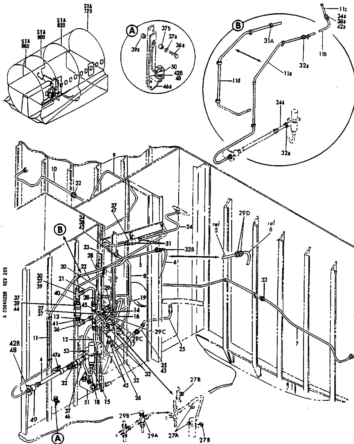
FIGURE 28B. HYDRAULIC INSTL, SECTION 43 CARGO DOOR SYSTEM (STATION 820 TO 960) (HYDRAULIC POWER ONLY)
