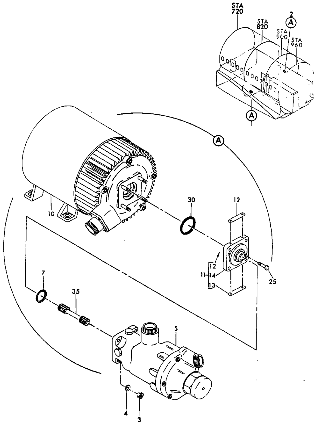
FIGURE 37F. PUMP ASSY, HYDRAULIC WATER
