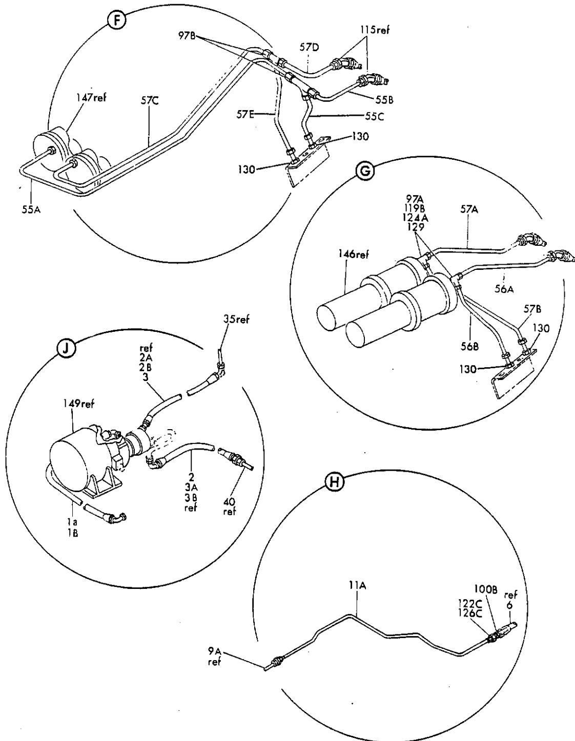
FIGURE 27. HYDRAULIC INSTL, WING FILLET (RH) (HYDRAULIC POWER ONLY) (SHEET 4)
