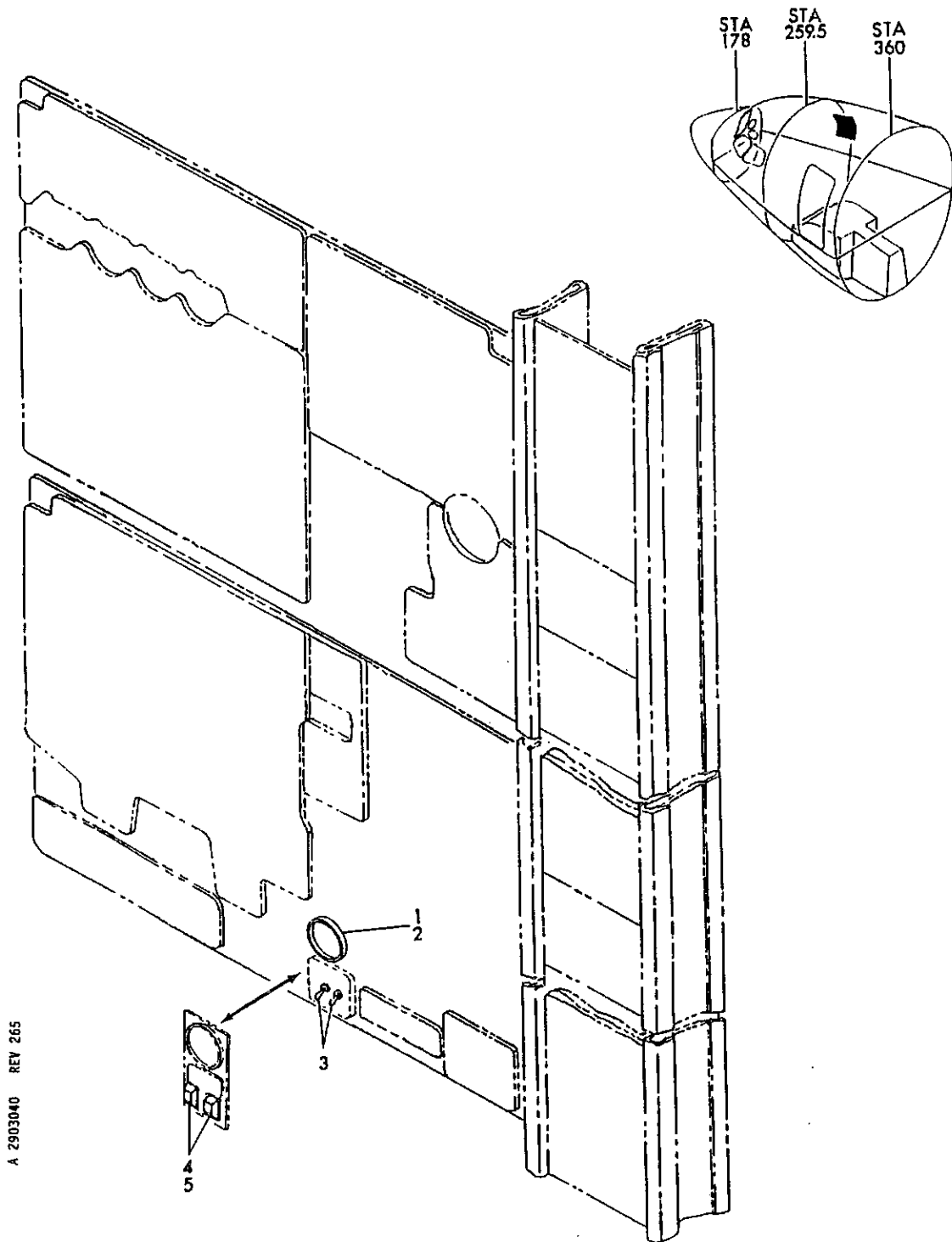
FIGURE 40. PANEL INSTL, FLIGHT ENGINEERS LOWER (HYDRAULIC POWER ONLY)
