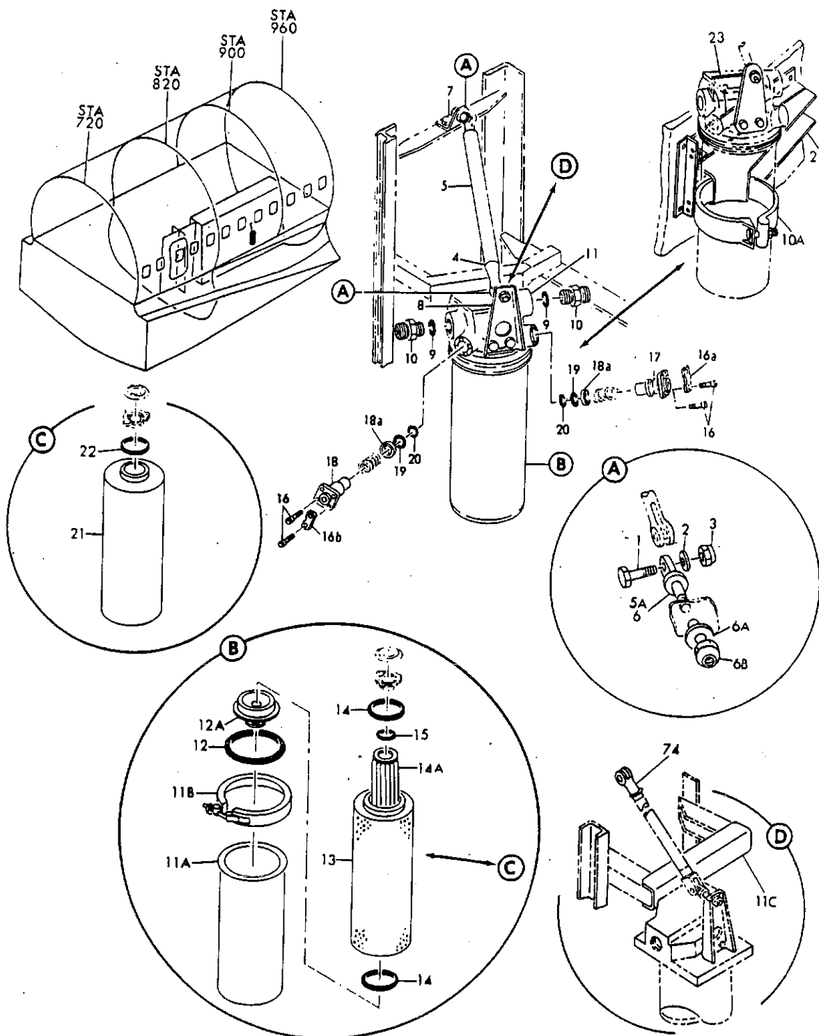
FIGURE 18A. FILTER INSTL, HYDRAULIC UTILITY RETURN
