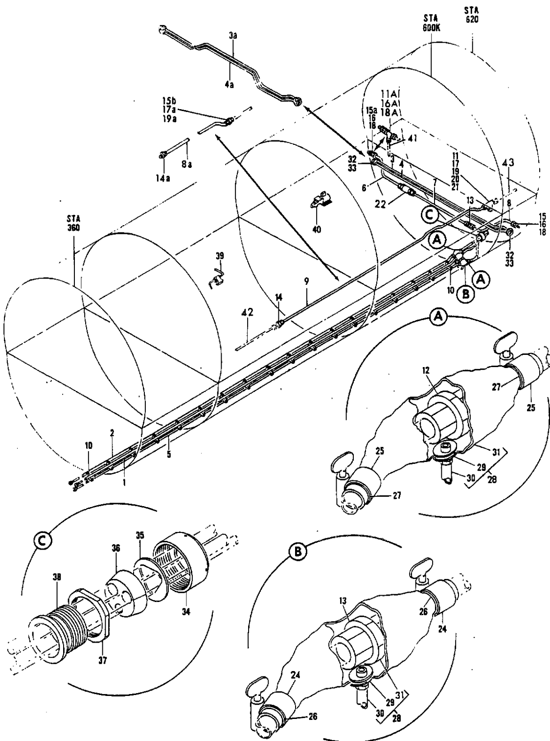
FIGURE 2. HYDRAULIC INSTL, SECTION 43 (STATION 360 TO 620) (HYDRAULIC POWER ONLY)
