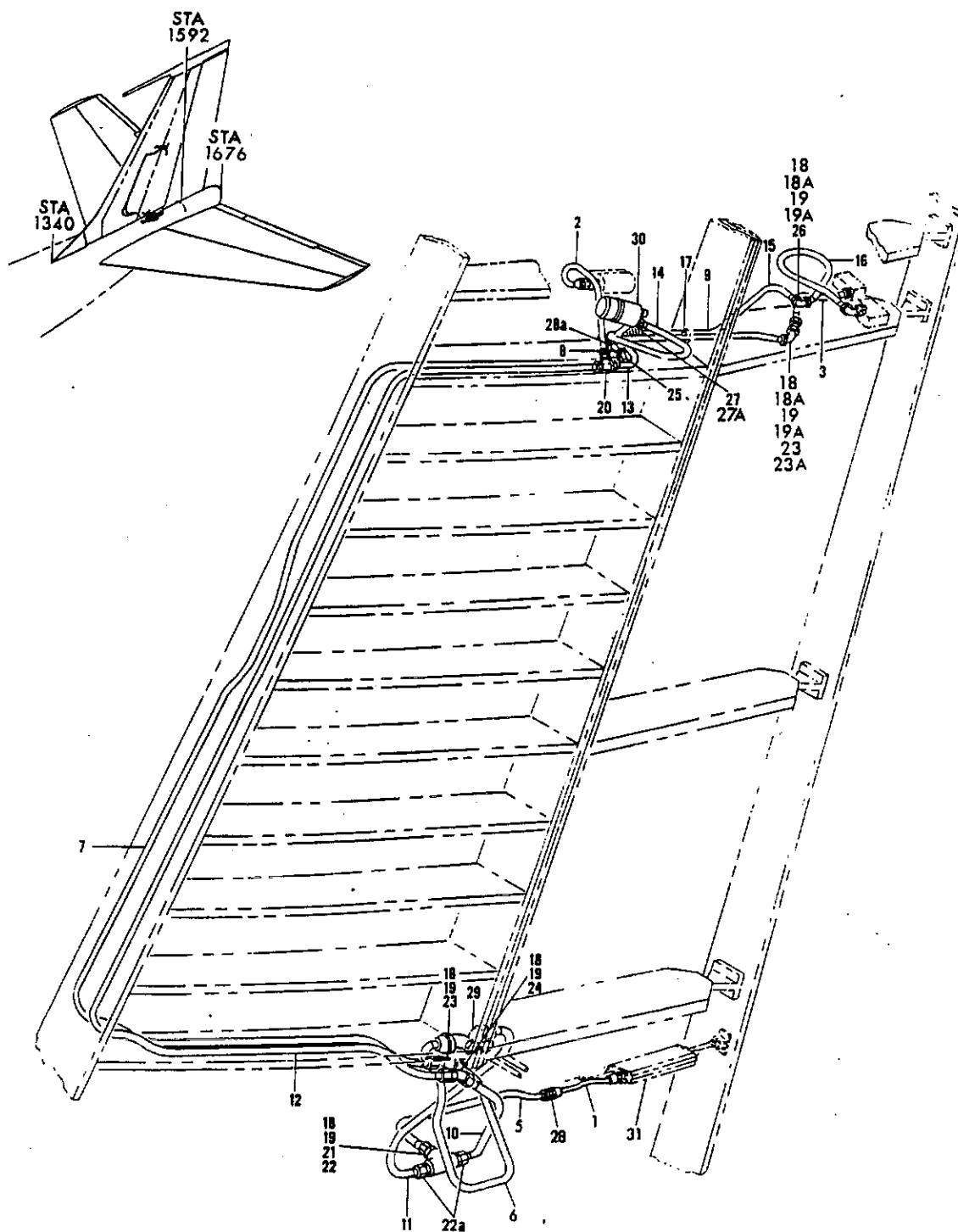
FIGURE 23A. TUBING INSTL. SECTION 92 EMPENNAGE HYDRAULIC
