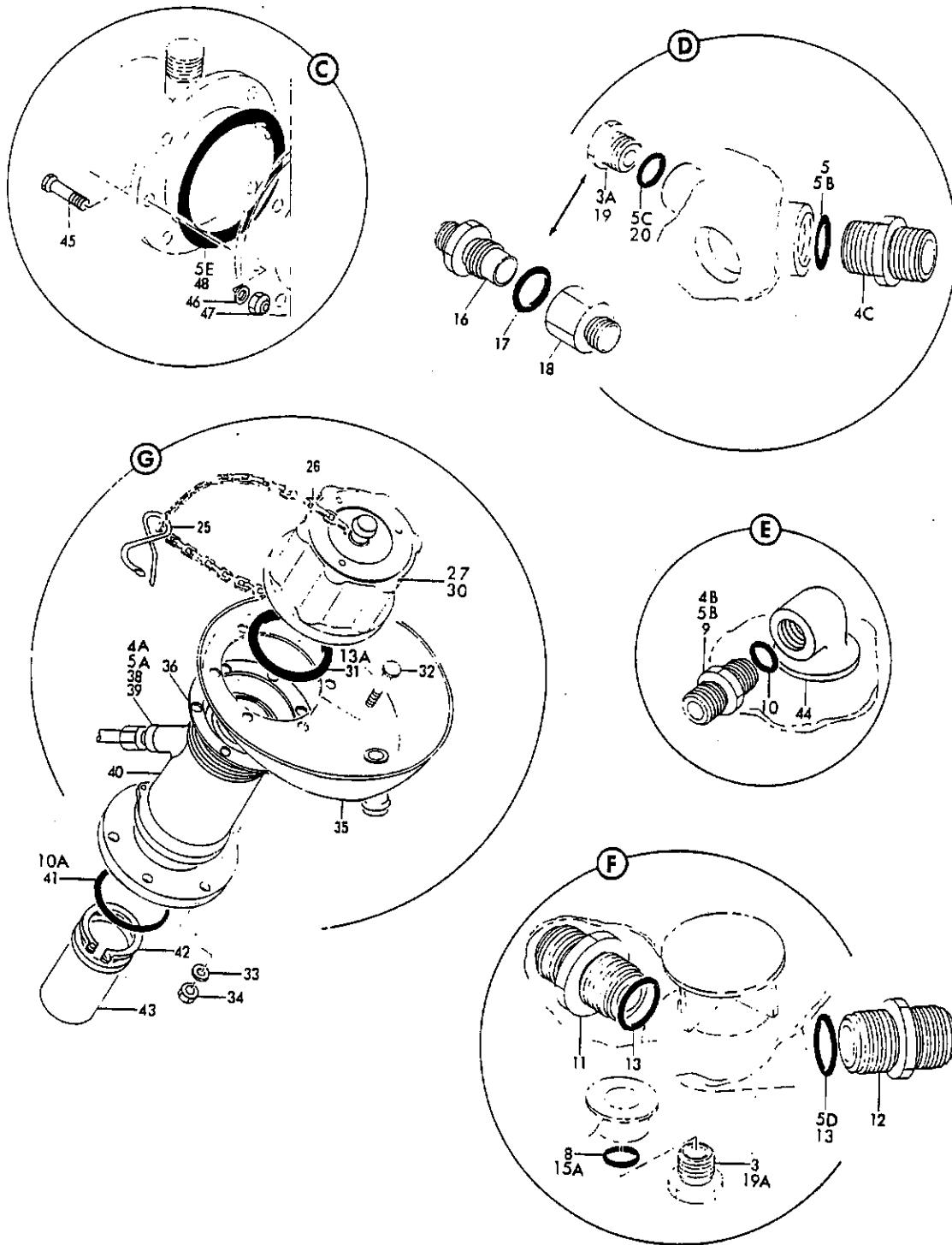
FIGURE 31A. RESERVOIR INSTL, HYDRAULIC (HYDRAULIC POWER ONLY) (SHEET 2)
