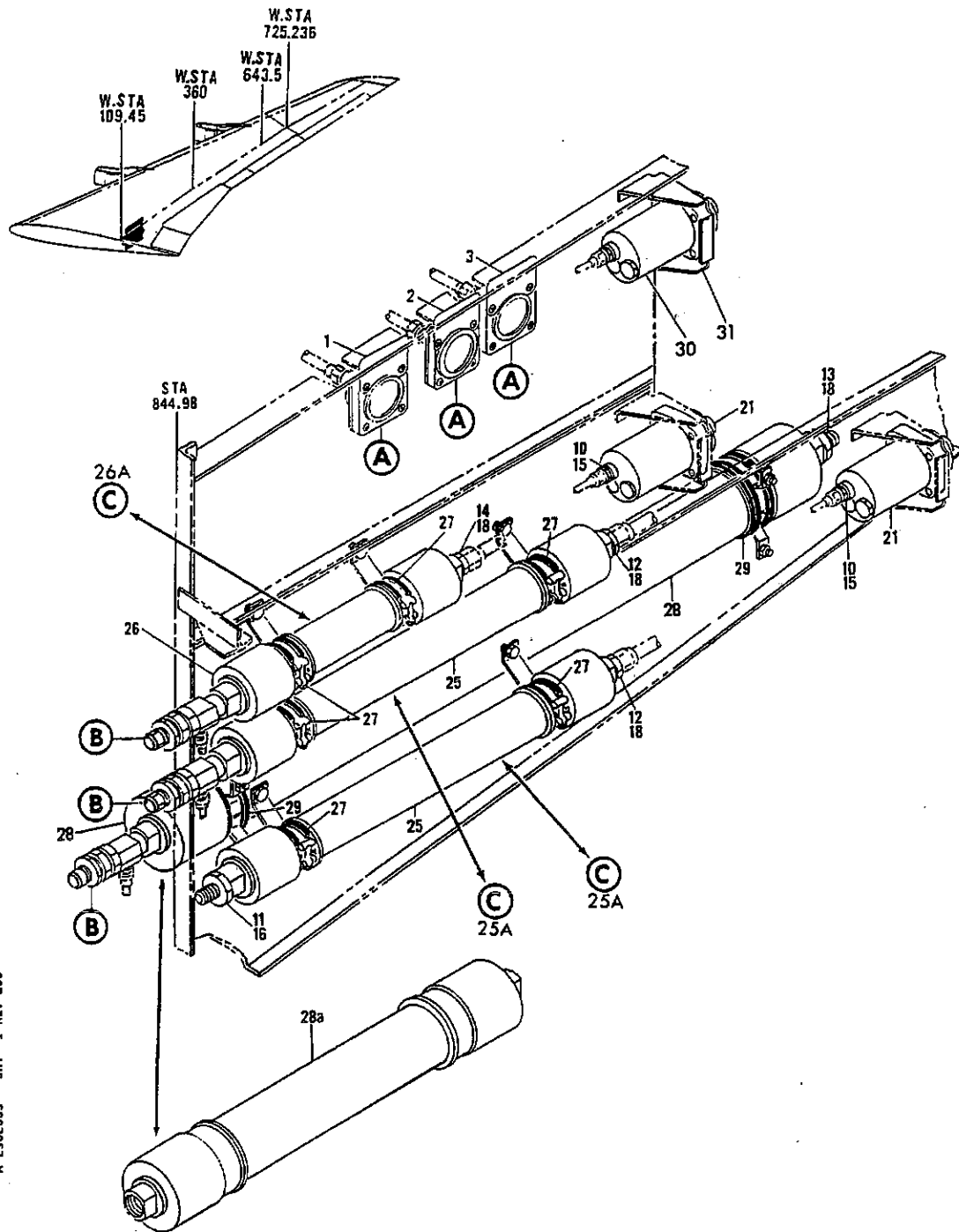
FIGURE 33. ACCUMULATOR INSTL, TRAILING EDGE BEAM(HYDRAULIC POWER ONLY)(SHEET 1)
