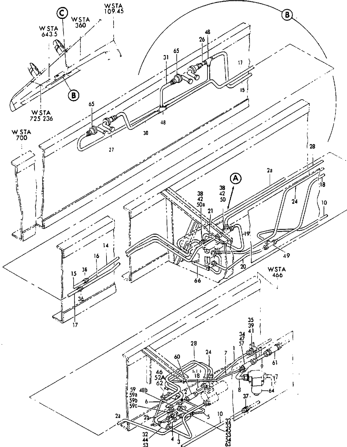
FIGURE 6A. HYDRAULIC INSTL, WING (WING STA 500 TO 725) (HYDRAULIC POWER ONLY) (SHEET 1)
