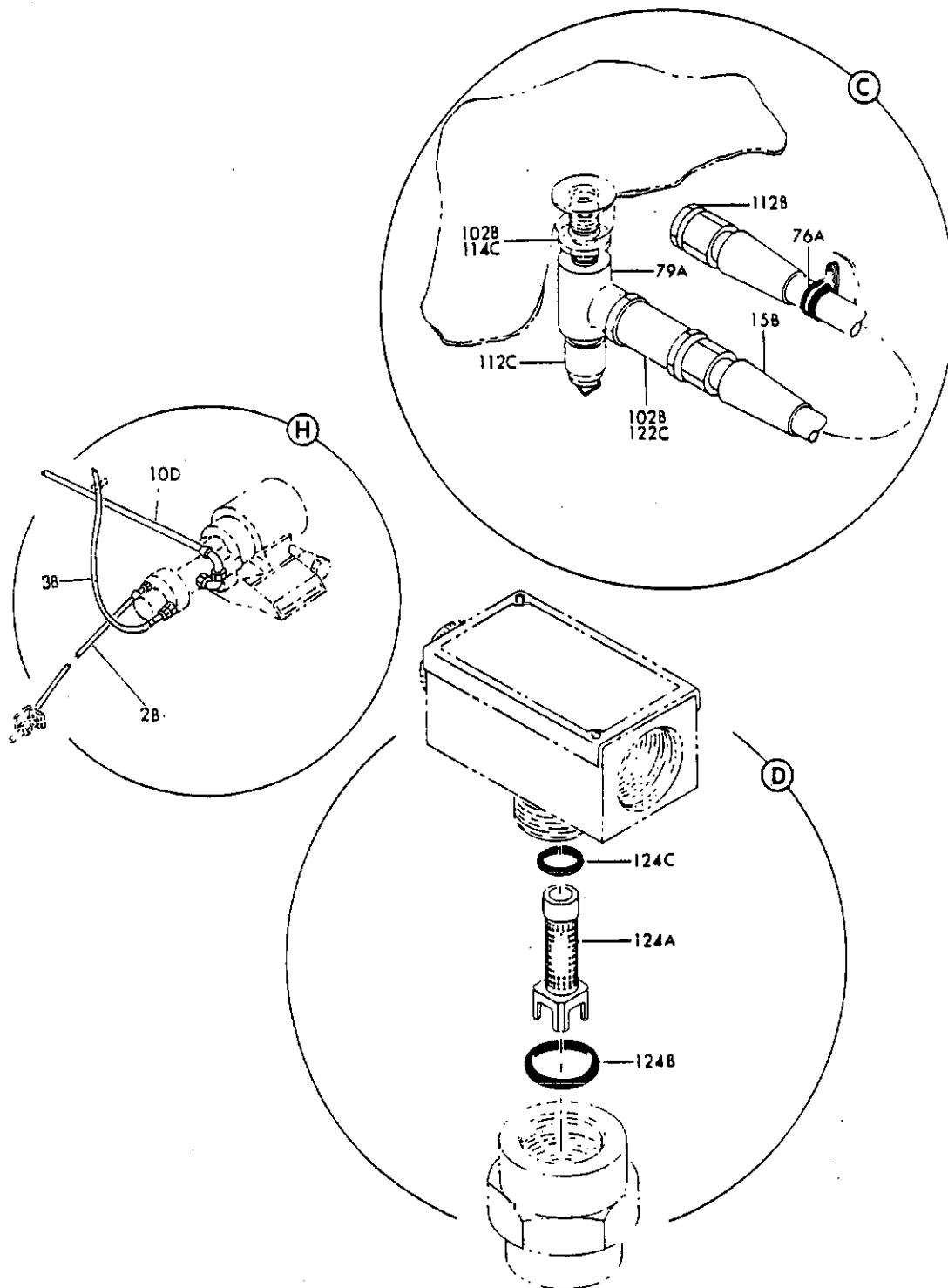
FIGURE 21. HYDRAULIC INSTL, WING FILLET (LH) (HYDRAULIC POWER ONLY) (SHEET 3)
