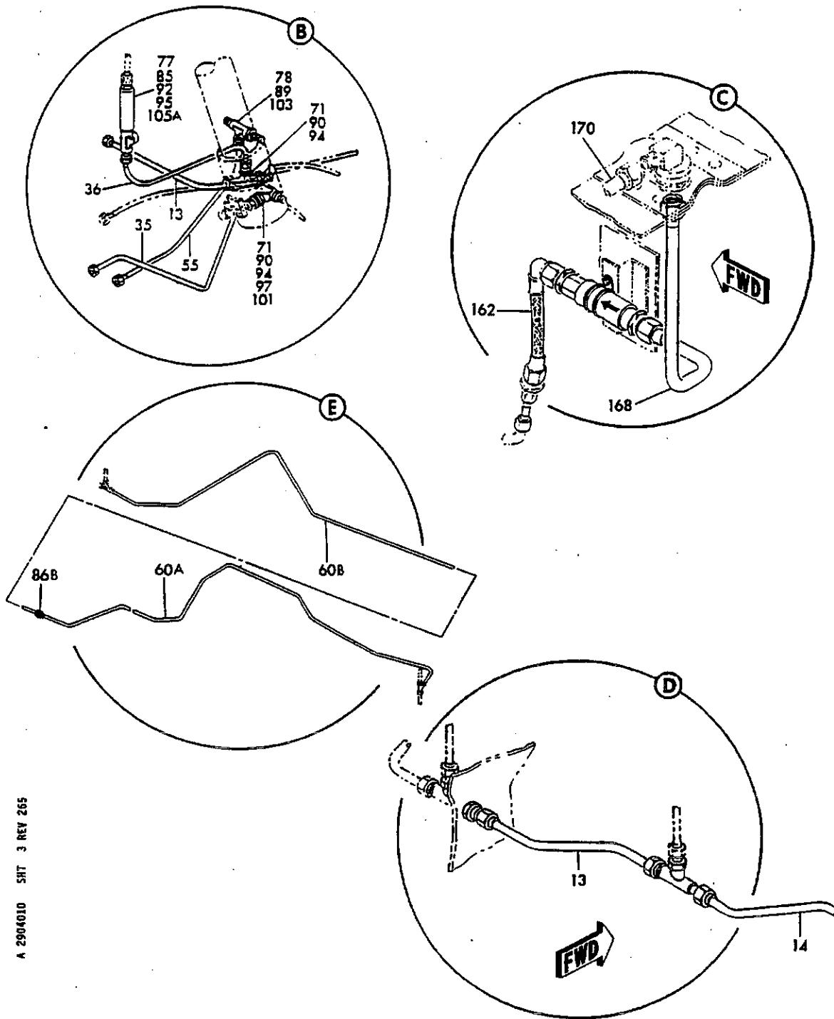
FIGURE 10. HYDRAULIC INSTL, SECT. 43 (STA 820 TO 840 RH) (HYDRAULIC POWER ONLY) (SHEET 3)
