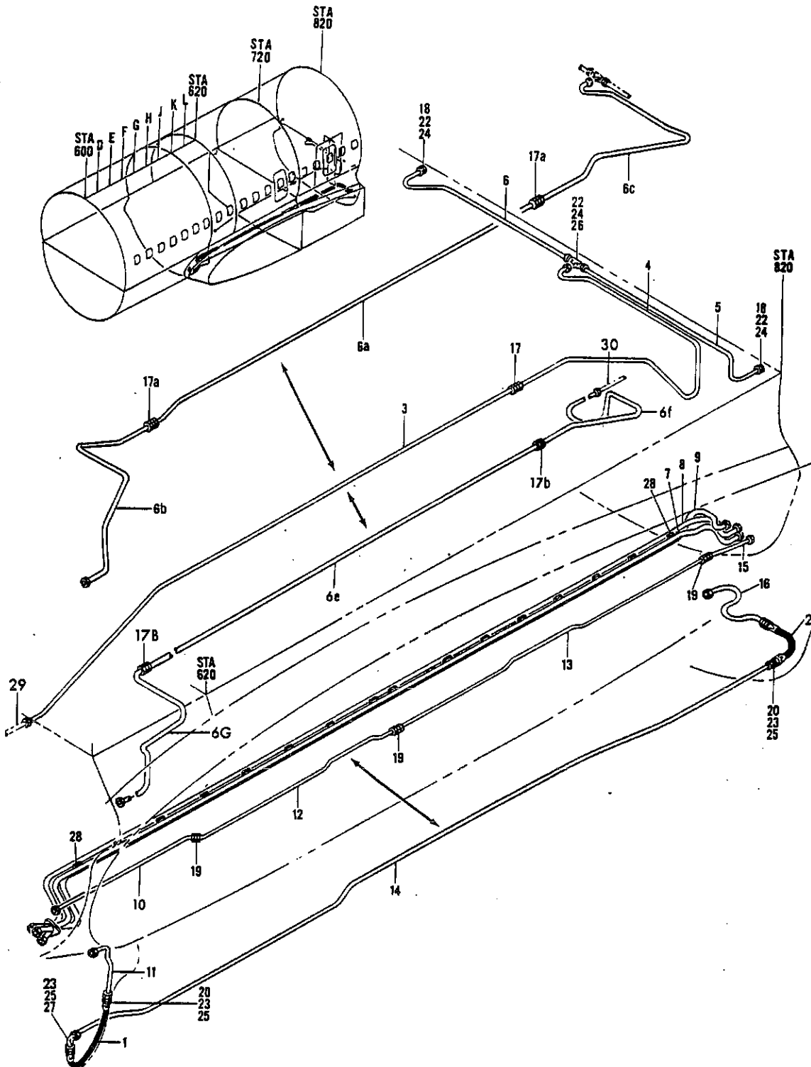
FIGURE 3. HYDRAULIC INSTL. SECTION 43 (STATION 620 TO 820) (HYDRAULIC POWER ONLY)
