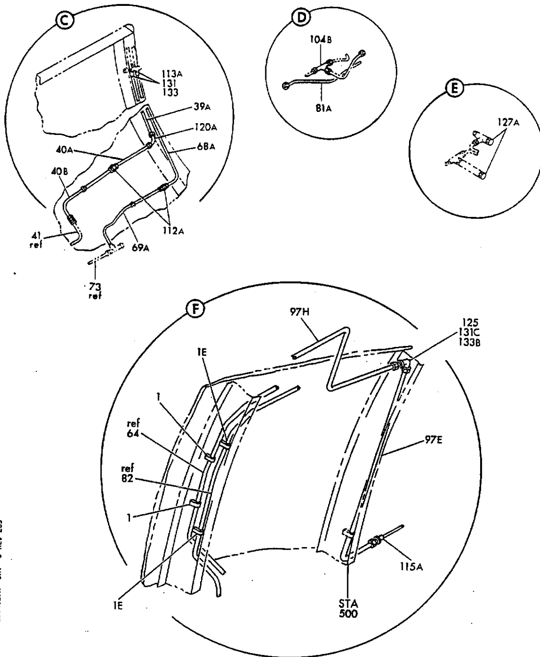
FIGURE 27A. HYDRAULIC INSTL, CARGO DOOR (HYDRAULIC POWER ONLY) (SHEET 3)
