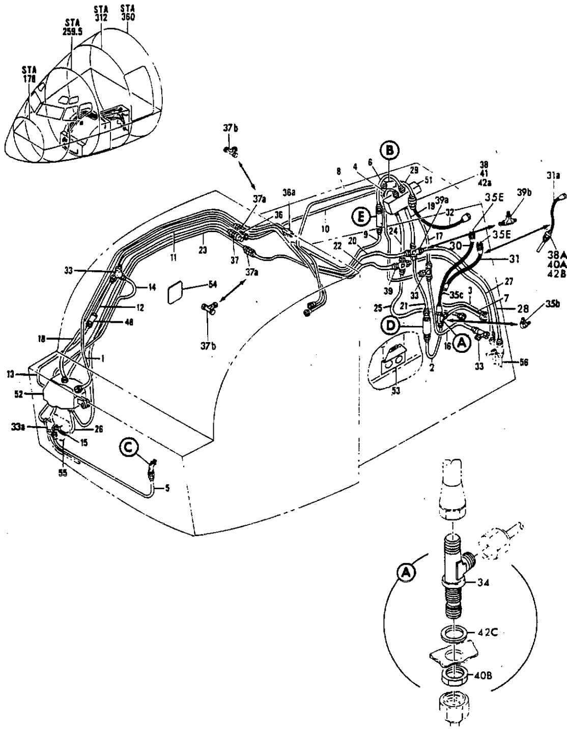
FIGURE 3. HYDRAULIC INSTL, SECTION 41 (HYDRAULIC POWER ONLY) (RH WHEEL WELL AREA) (SHEET 1)
