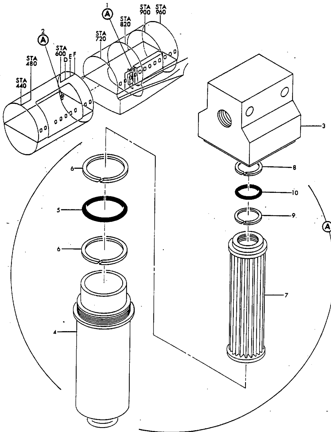
FIGURE 38. FILTER ASSY, AUXILIARY HYDRAULIC PRESSURE
