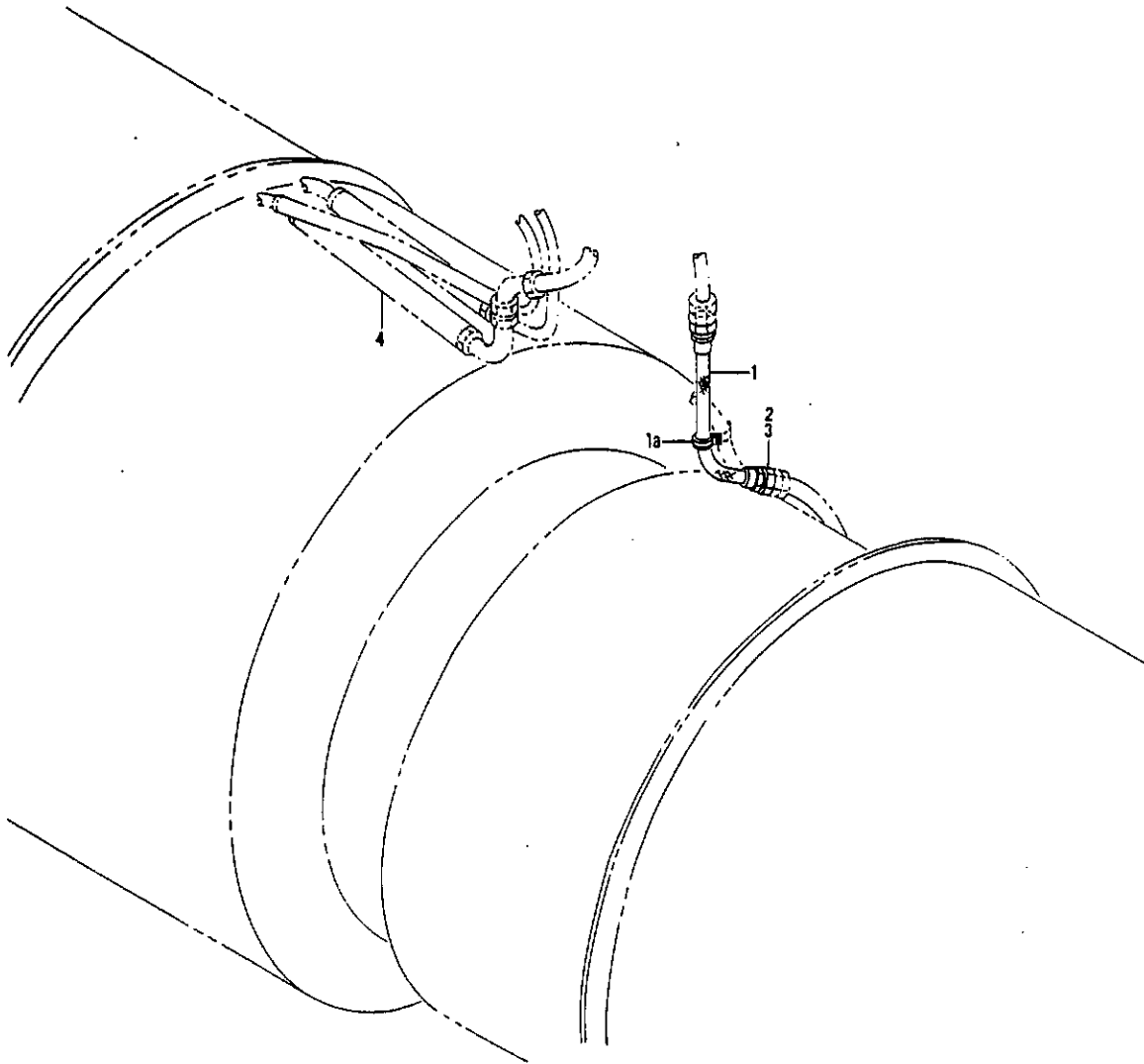
FIGURE 10. PLUMBING INSTL, FAN ENGINES NO. 2 AND 3 (HYDRAULIC POWER ONLY)
