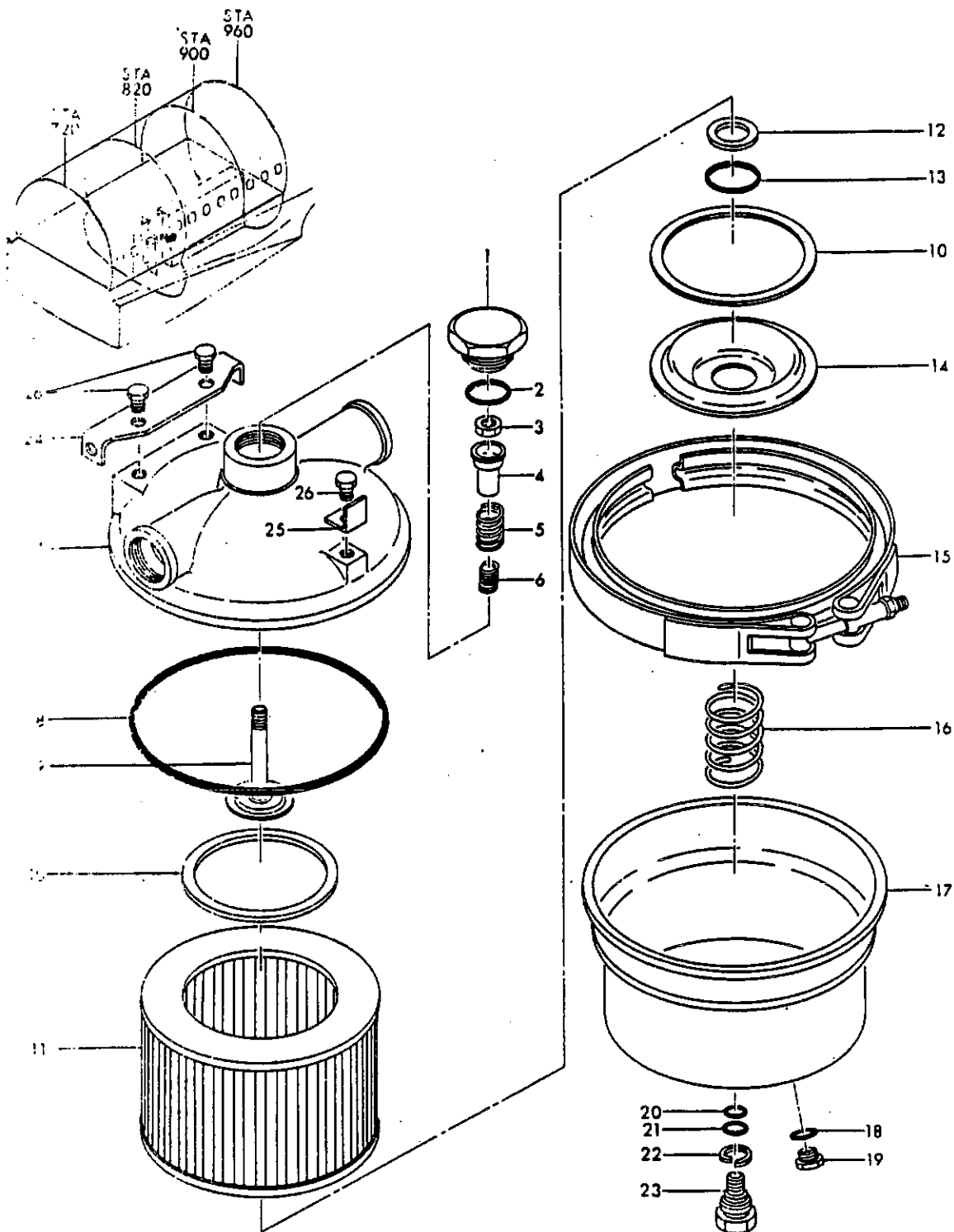
FIGURE 37. FILTER ASSY, HYDRAULIC UTILITY RETURN
