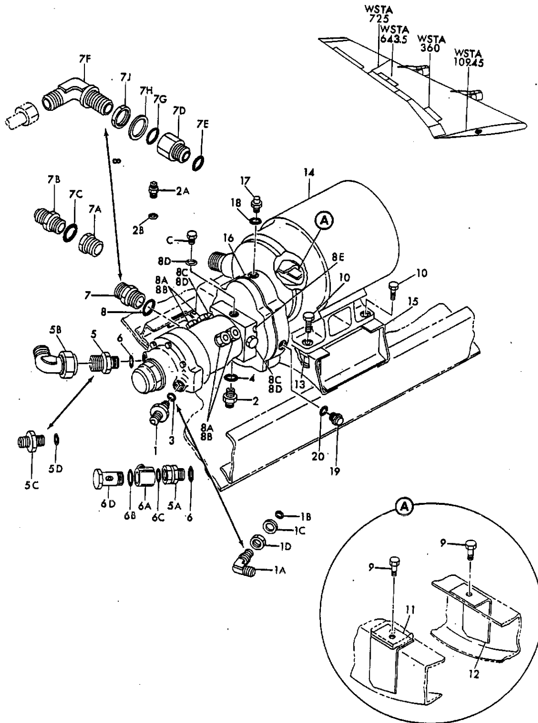
FIGURE 37. PUMP INSTL, AUXILIARY HYDRAULIC
