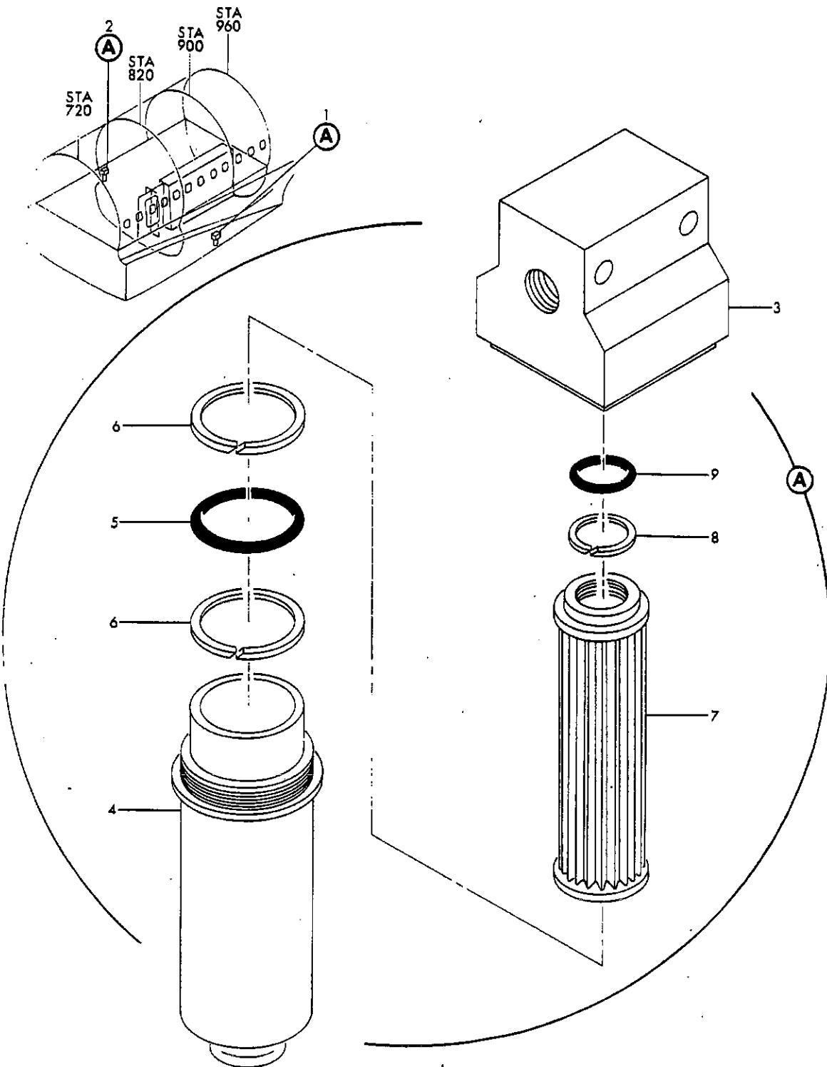
FIGURE 47. FILTER ASSY, AUXILIARY HYDRAULIC PRESSURE
