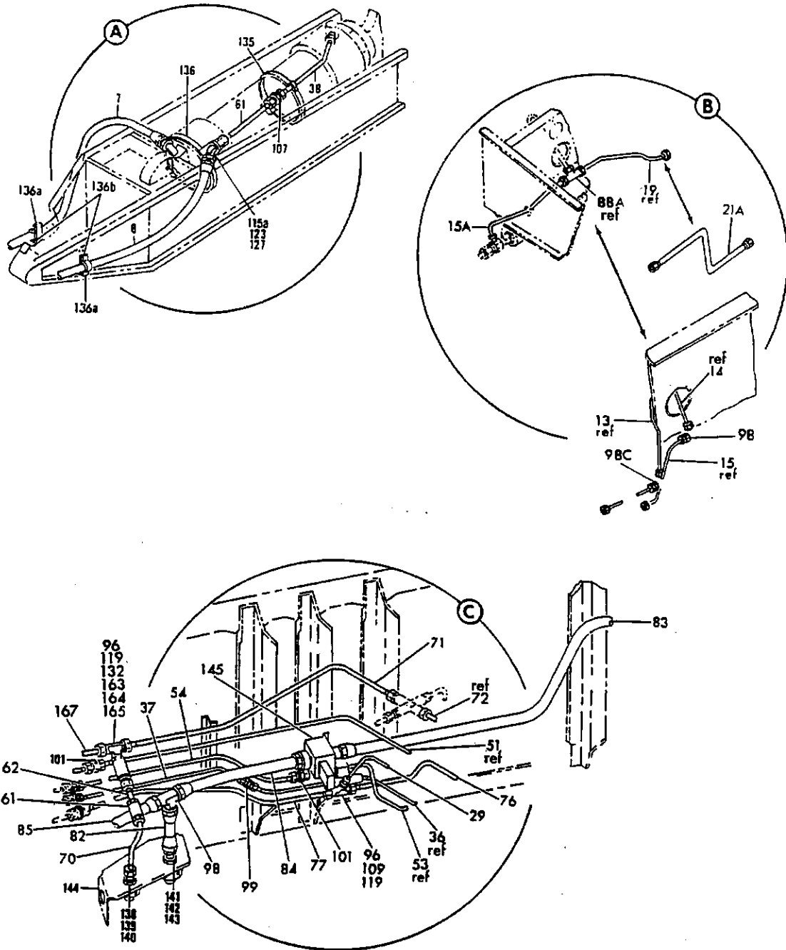
FIGURE 27. HYDRAULIC INSTL. WING FILLET (RH) (HYDRAULIC POWER ONLY)(SHEET 2)
