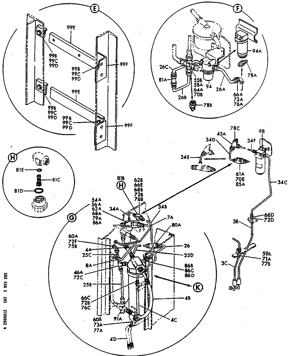
FIGURE 12. HYDRAULIC INSTL, SECT. 43 (STA 840 TO 860 LH) (HYDRAULIC POWER ONLY)(SHEET 3)
