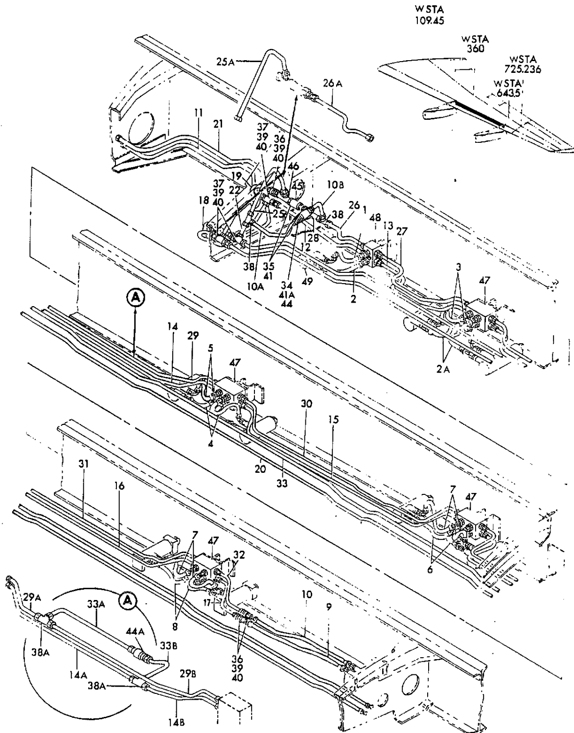
FIGURE 13. HYDRAULIC INSTL, WING (FRONT SPAR STATION 382.65 TO 666.14) (HYDRAULIC POWER ONLY)
