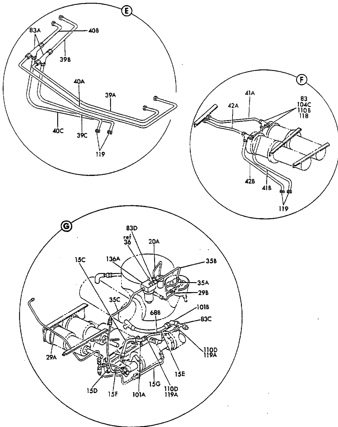
FIGURE 21. HYDRAULIC INSTL, WING FILLET (LH) (HYDRAULIC POWER ONLY) (SHEET 4)
