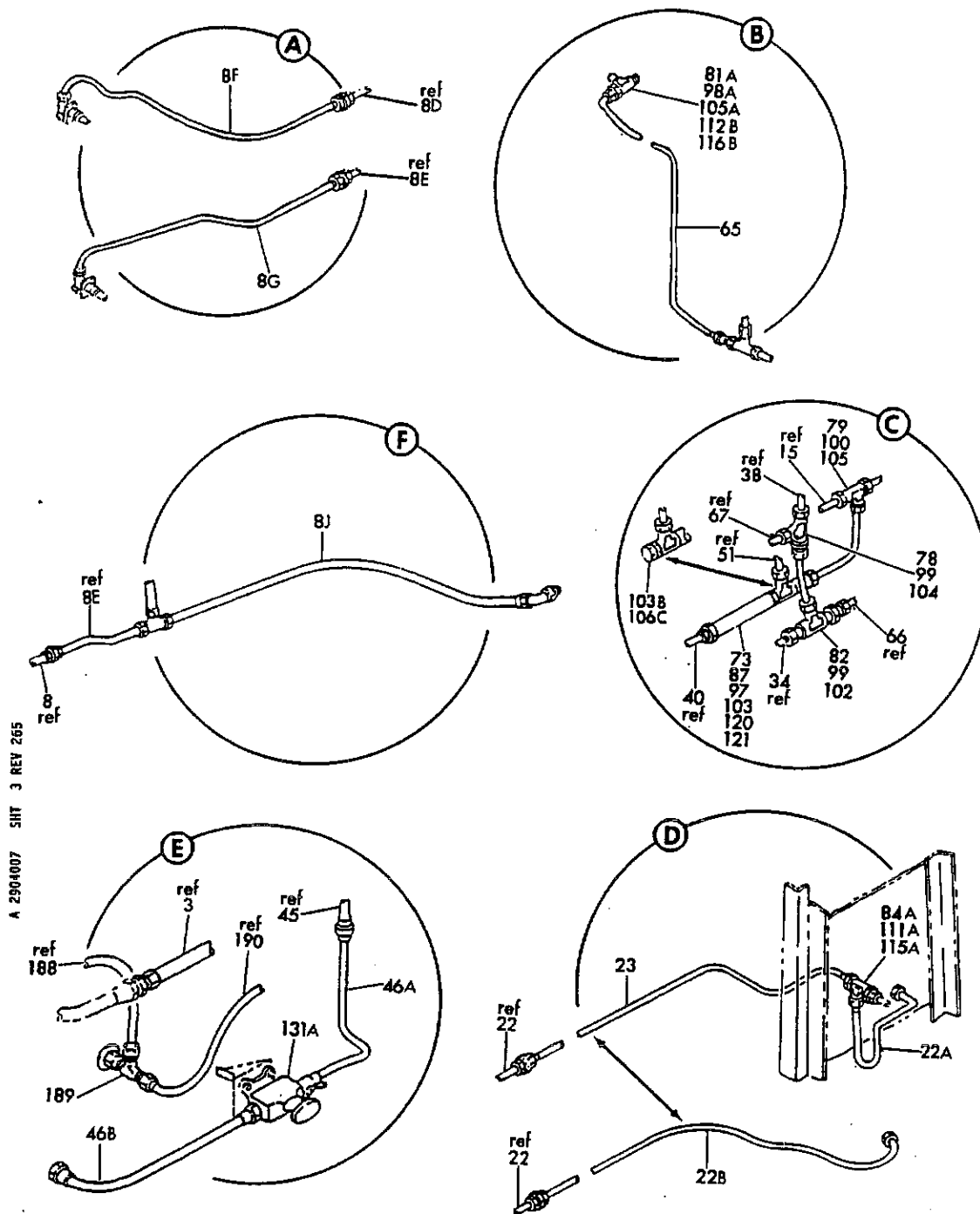
FIGURE 7. HYDRAULIC INSTL, SECT. 43 (STA 820 TO 840 LH) (HYDRAULIC POWER ONLY) (SHEET 3)
