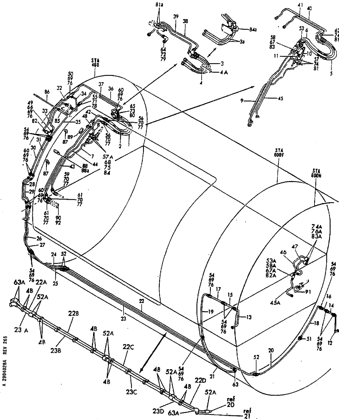
FIGURE 28A. HYDRAULIC INSTL. SECTION 43 CARGO DOOR SYSTEM (STATION 400 TO 600K) (HYDRAULIC POWER ONLY)
