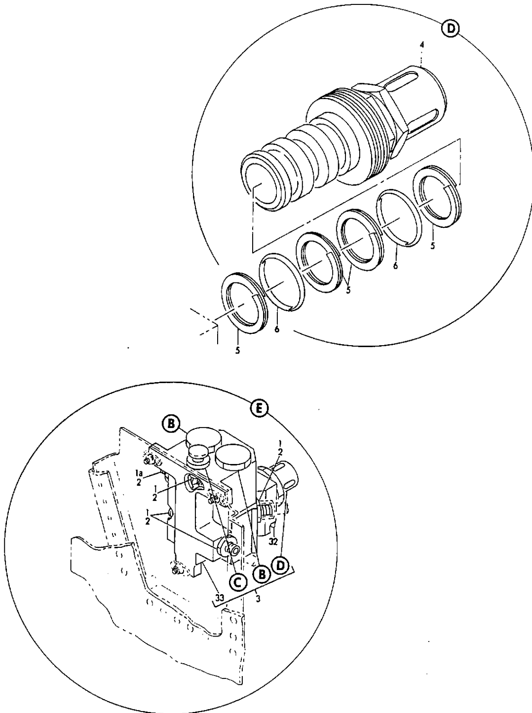
FIGURE 42. MODULAR PACKAGE INSTL, SPOILER SYSTEM (HYDRAULIC POWER ONLY) (SHEET 2)
