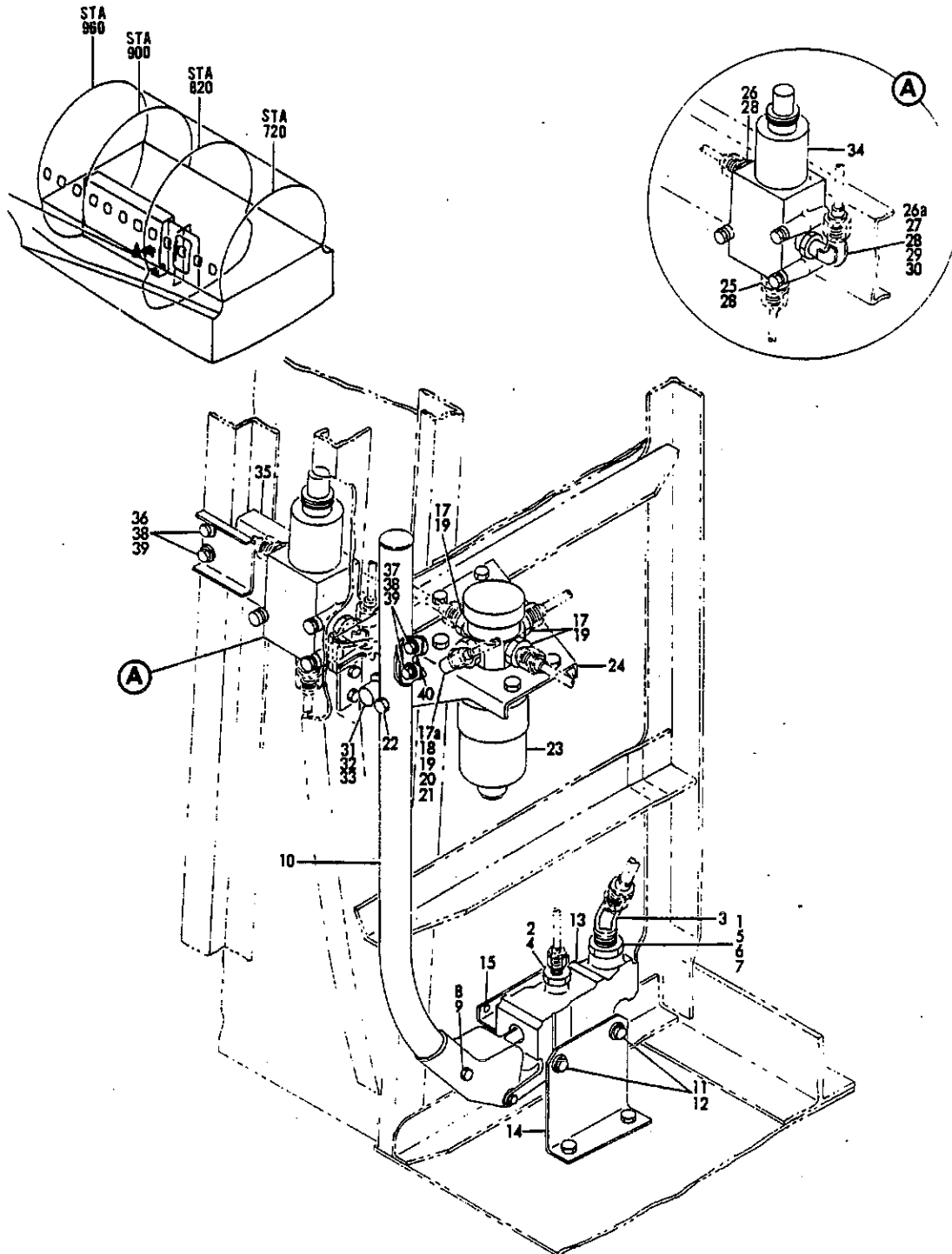
FIGURE 30. PUMP INSTL, MAIN CARGO DOOR HYDRAULIC HAND (HYDRAULIC POWER ONLY) VALVE INSTL, MAIN CARGO DOOR HYDRAULIC 4-WAY VALVE INSTL, MAIN CARGO DOOR HYDRAULIC SOLENOID
