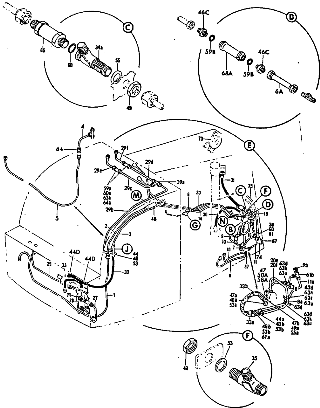
FIGURE 2. HYDRAULIC INSTALLATION, SECTION 41 (HYDRAULIC POWER ONLY) (FORWARD AND LH WHEEL WELL AREA) (SHEET 2)
