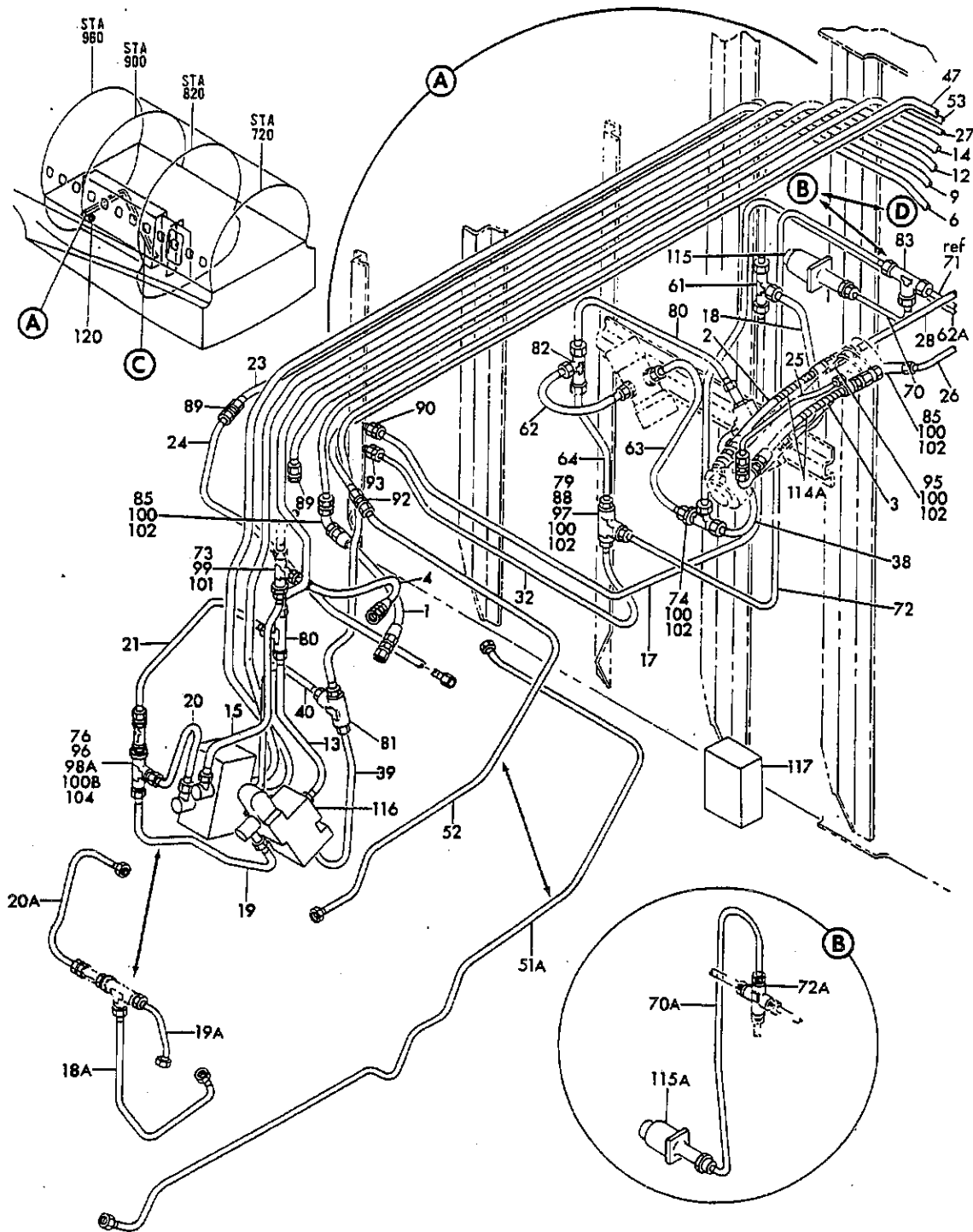
FIGURE 16. HYDRAULIC INSTL. SECTION 43 (STATION 840 TO 960 RH) (HYDRAULIC POWER ONLY) (SHEET 1)
