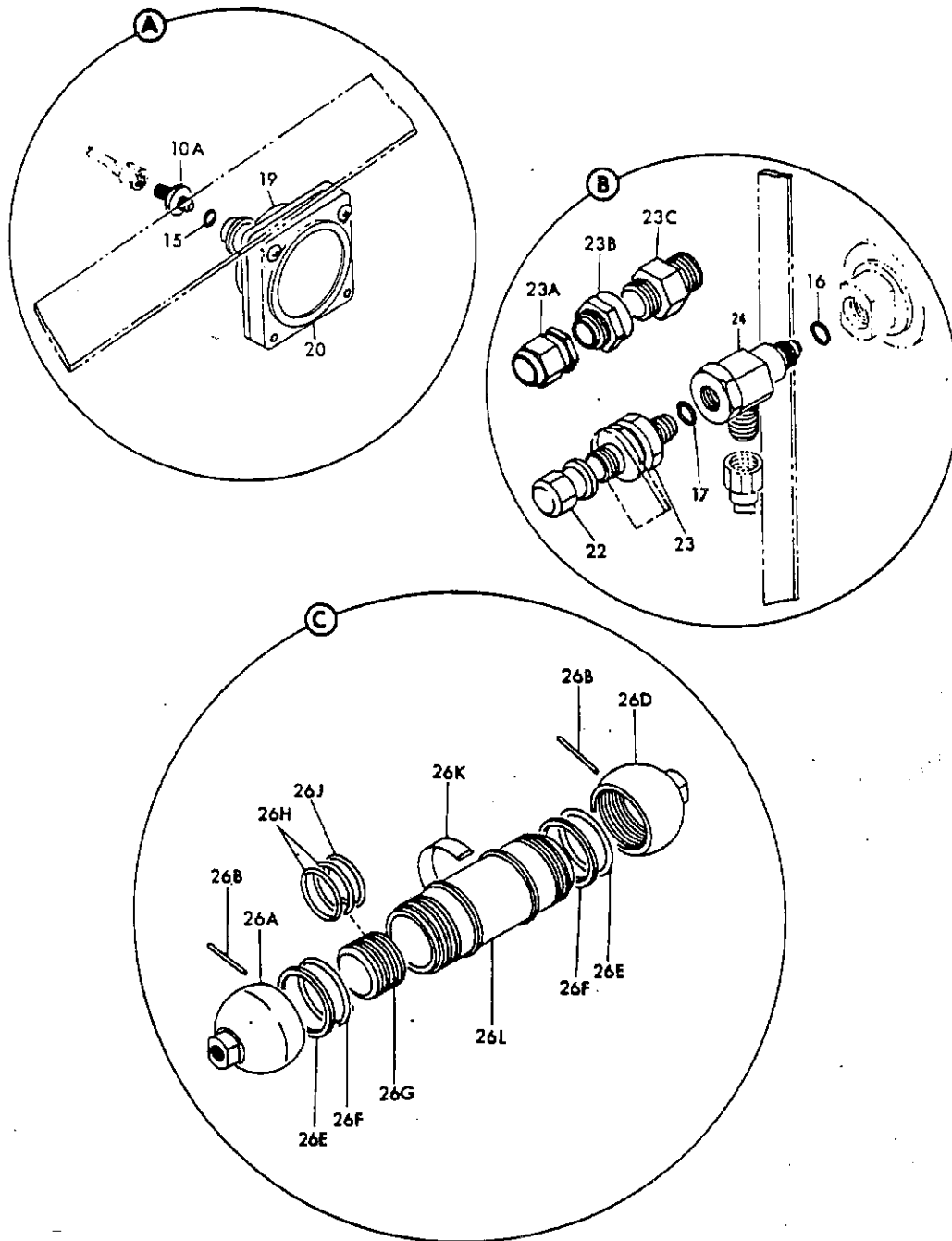
FIGURE 33. ACCUMULATOR INSTL, TRAILING EDGE BEAM (HYDRAULIC POWER ONLY) (SHEET 2)
