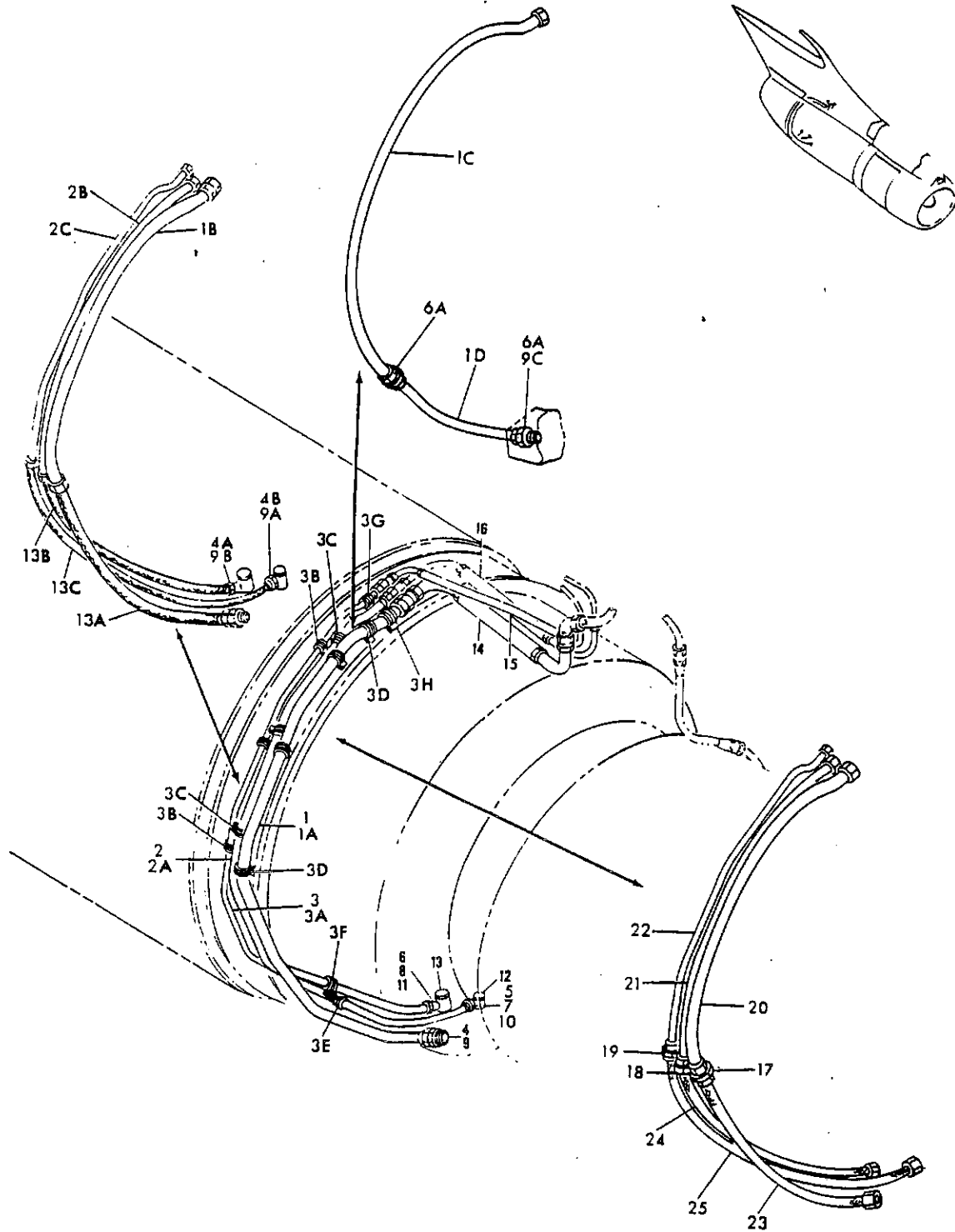
PLUMBING INSTL, FAN ENGINES NO. 2 AND 3 (HYDRAULIC POWER ONLY) PLUMBING INSTL, FAN ENGINE KELLOGG HYDRAULIC PUMP (ENGINES NO. 2 AND 3) FIGURE 9A. PLUMBING INSTL, ABEX HYDRAULIC PUMP (ENGINES NO. 2 AND 3)
