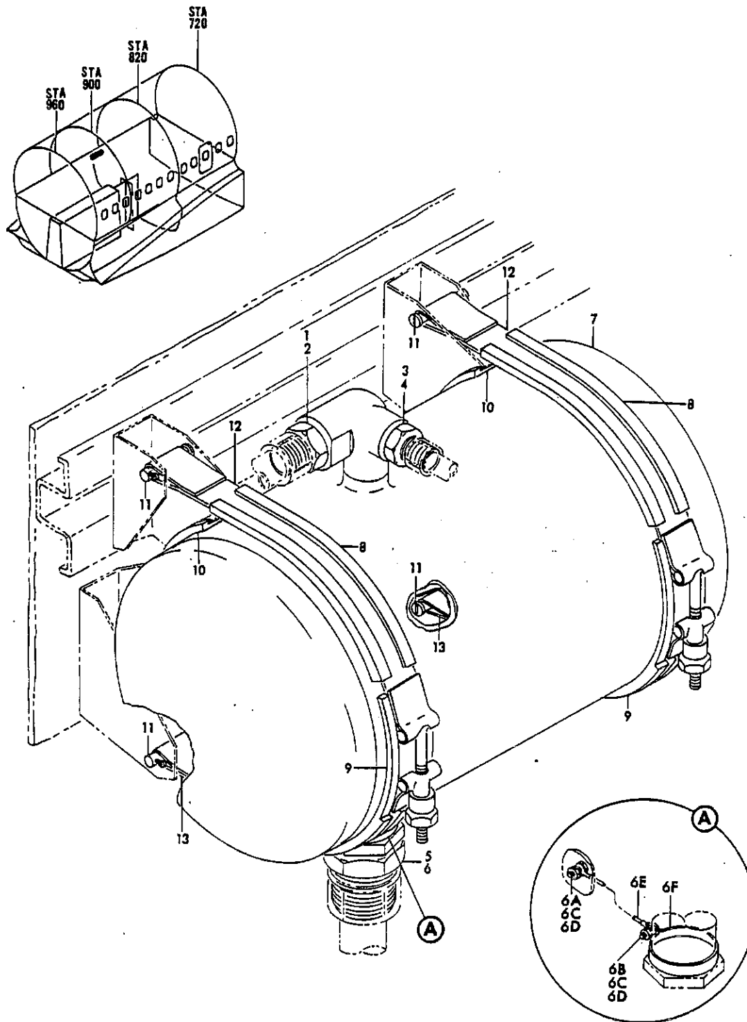
FIGURE 25A. TANK INSTL, HYDRAULIC SURGE
