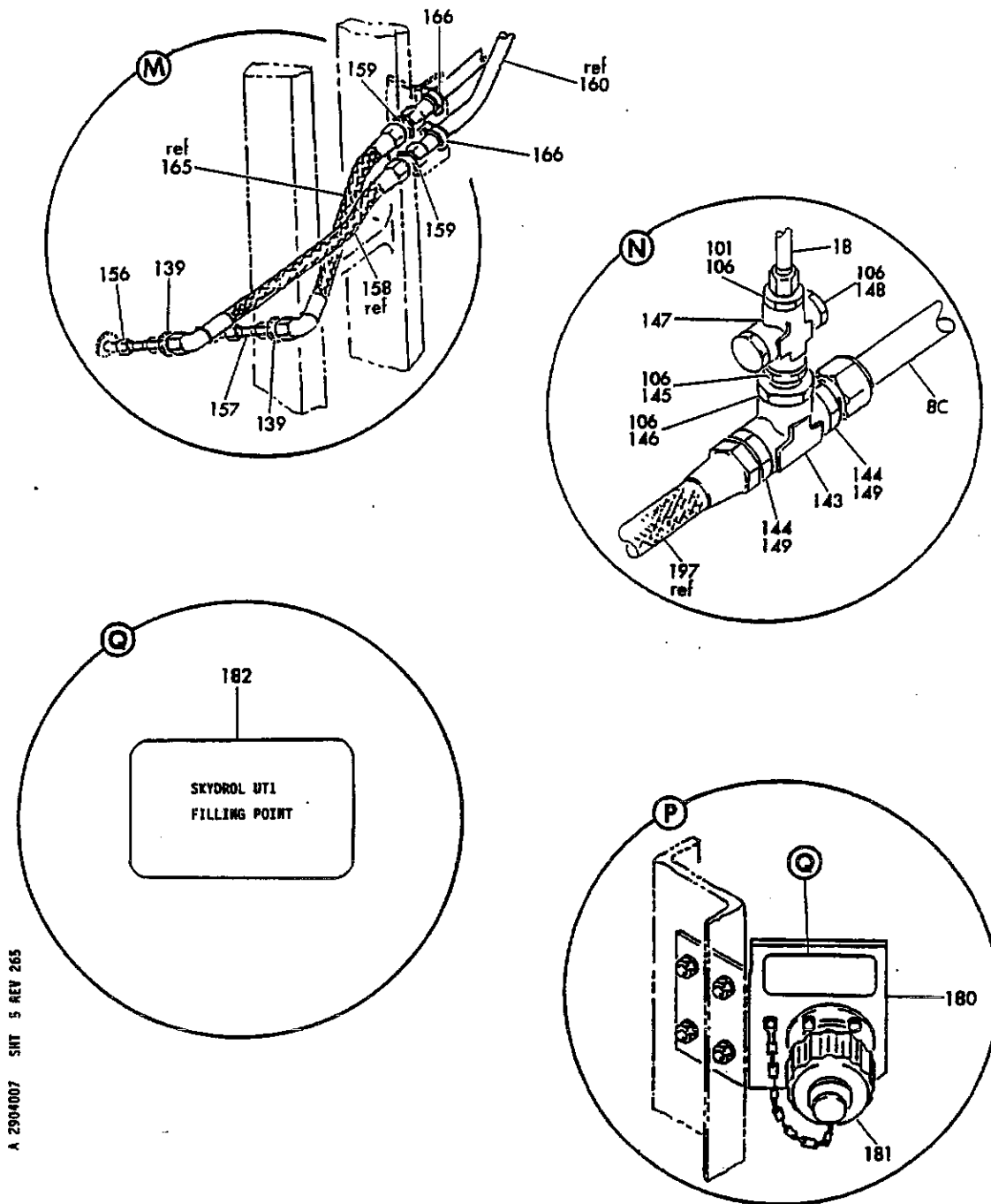
FIGURE 7. HYDRAULIC INSTL, SECT. 43 (STA 820 TO 840 LH) (HYDRAULIC POWER ONLY) (SHEET 5)
