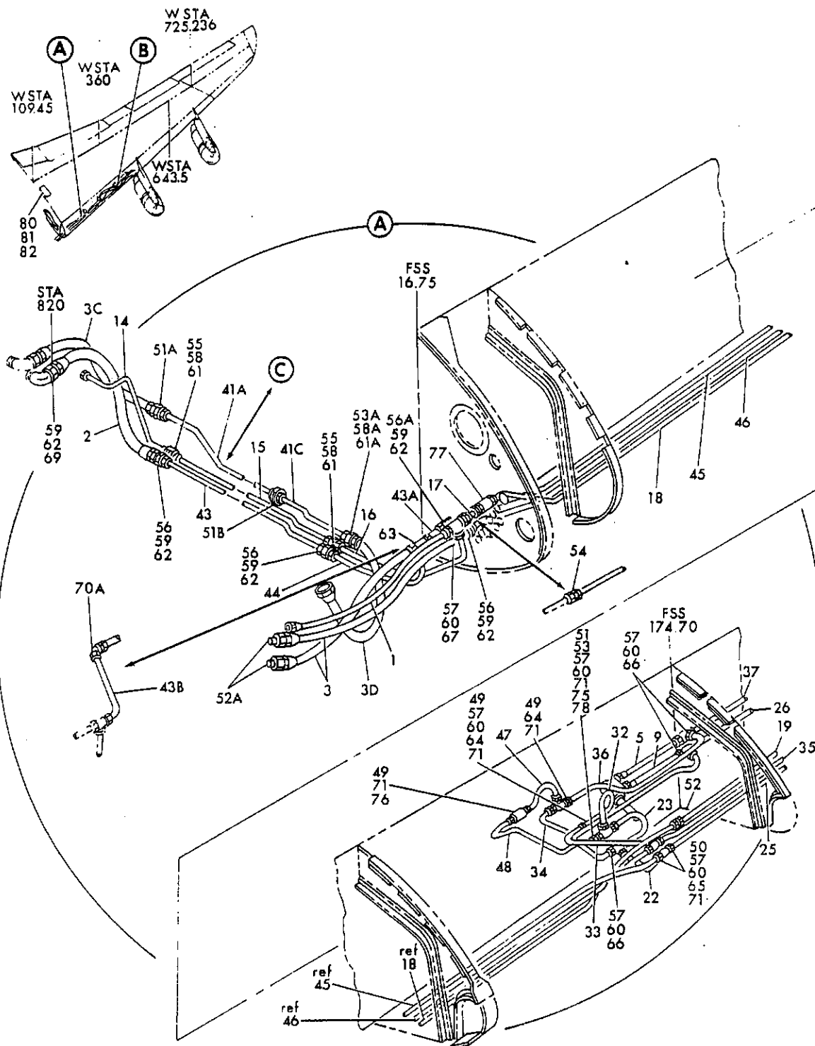
FIGURE 10. WING HYDRAULIC INSTL. (BODY SEAL TO FRONT SPAR STATION 382.65) (HYDRAULIC POWER ONLY)
