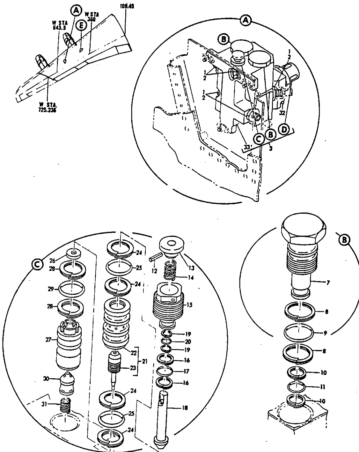
FIGURE 42. MODULAR PACKAGE (INSTL. SPOILER SYSTEM (HYDRAULIC POWER ONLY) (SHEET 1)
