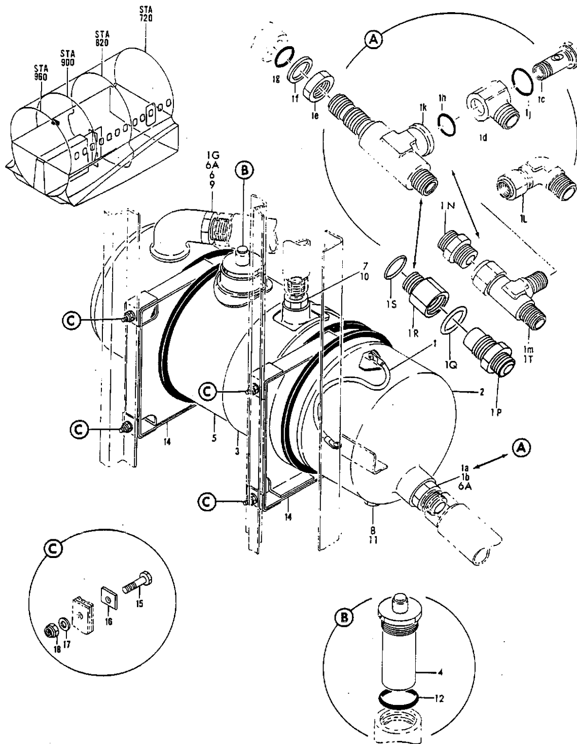
FIGURE 34. RESERVOIR INSTL, AUXILIARY HYDRAULIC
