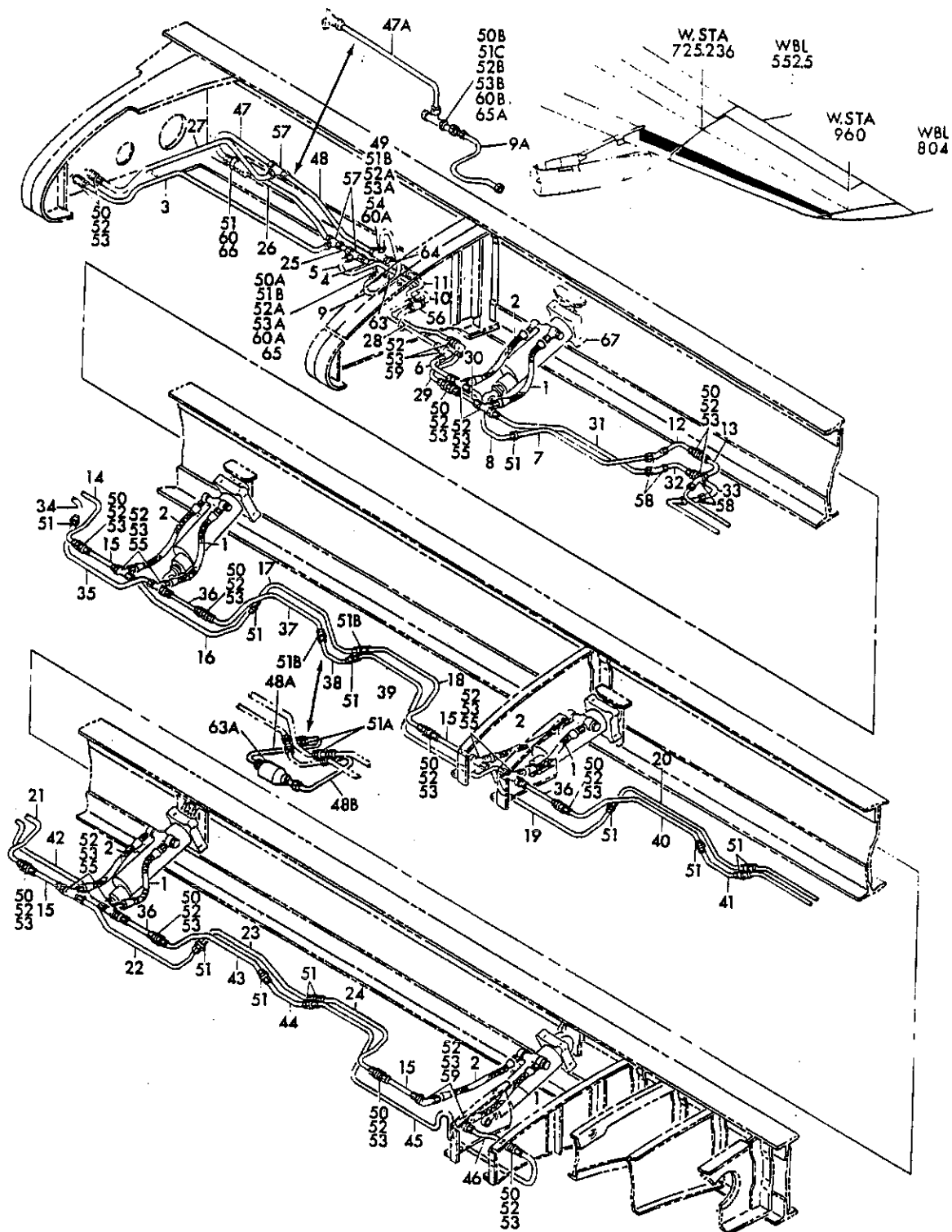
FIGURE 16. HYDRAULIC INSTL, WING (FRONT SPAR STATION 66, 14 TO 960) (HYDRAULIC POWER ONLY)
