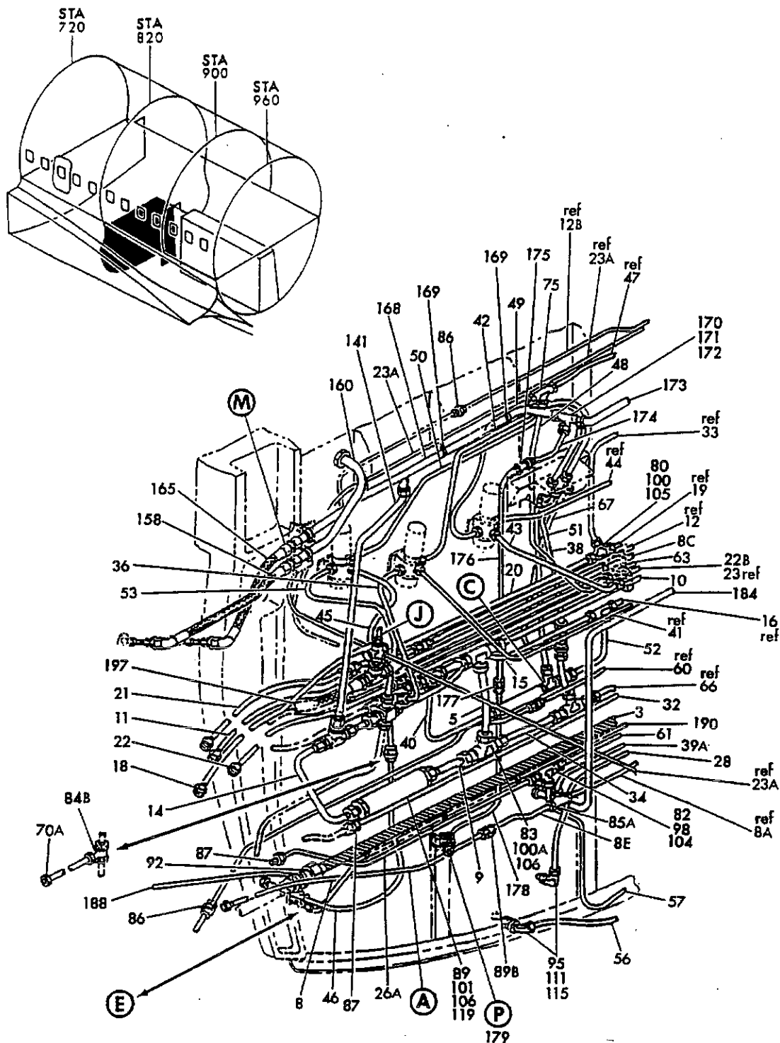
FIGURE 7. HYDRAULIC INSTL, SECT. 43 (STA 820 TO 840 LH) (HYDRAULIC POWER ONLY) (SHEET 1)
