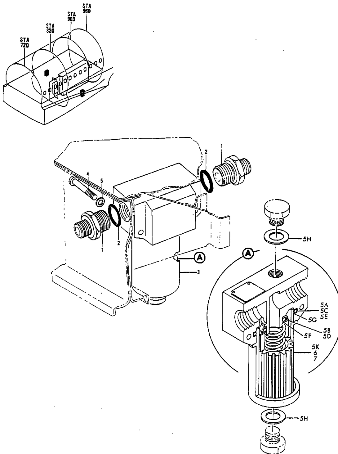
FIGURE 38. FILTER INSTL, AUXILIARY HYDRAULIC RETURN (HYDRAULIC POWER ONLY)
