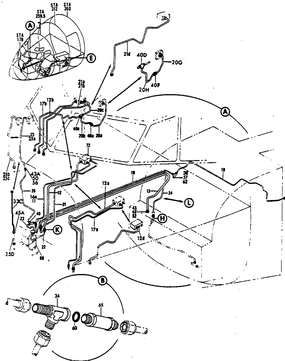
FIGURE 2. HYDRAULIC INSTL, SECTION 41 (HYDRAULIC POWER ONLY) (FORWARD AND LH WHEEL WELL AREA) (SHEET 1)
