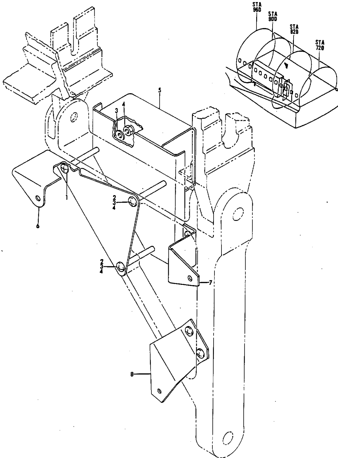
FIGURE 32. SUPPORT INSTL, STATION 900 TO 910 HYDRAULIC TUBING AND AIR START RELIEF VALVE
