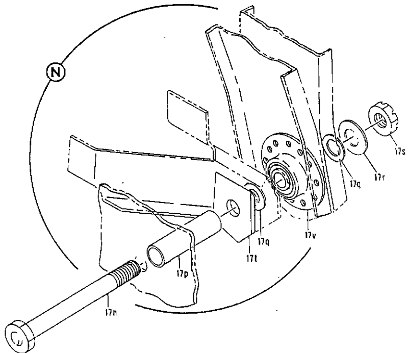
FIGURE 11. RELEASE INSTL, MAIN GEAR EMERGENCY (SHL11 4)
