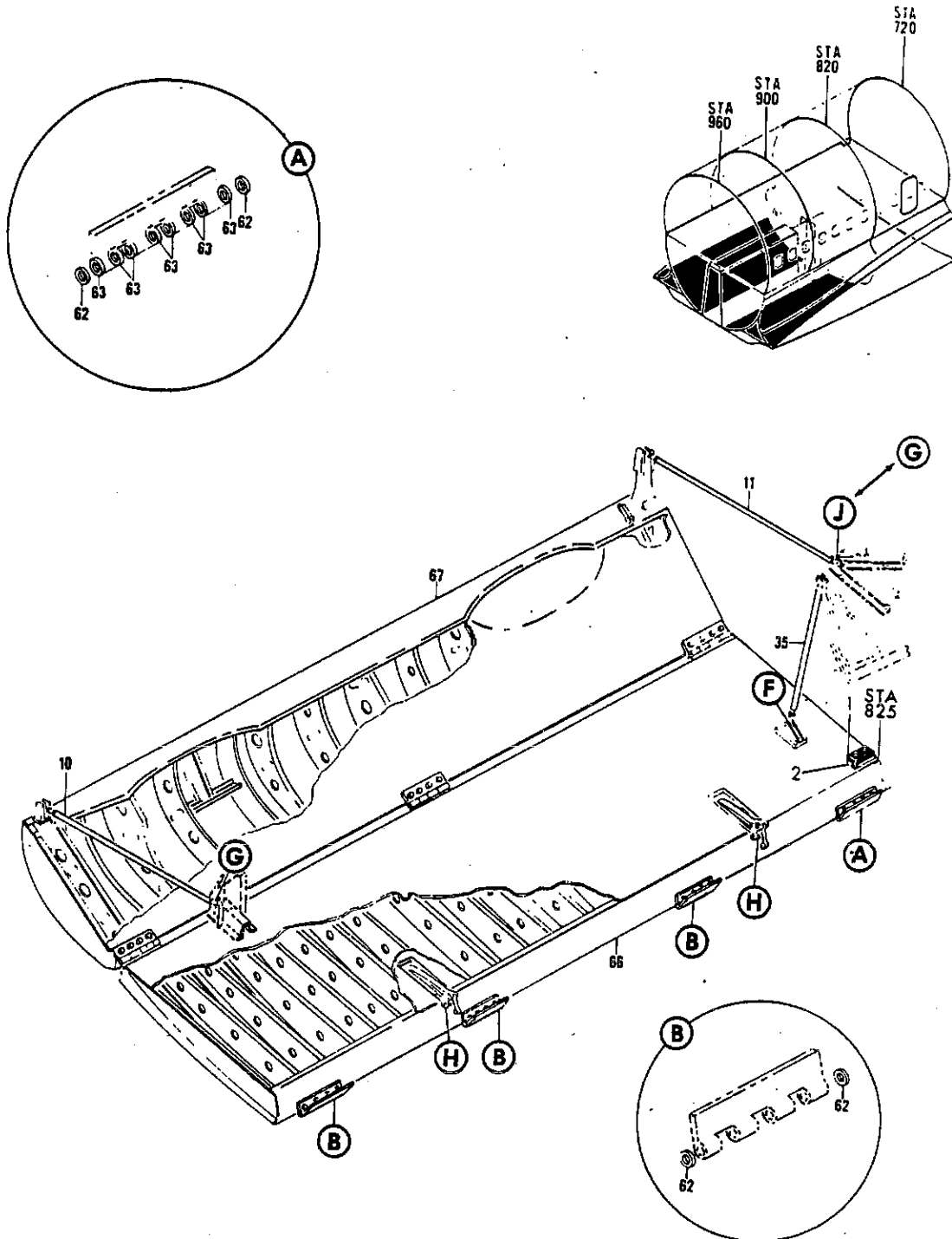
FIGURE 10. DOOR INSTL, MAIN GEAR (SHEET 1)
