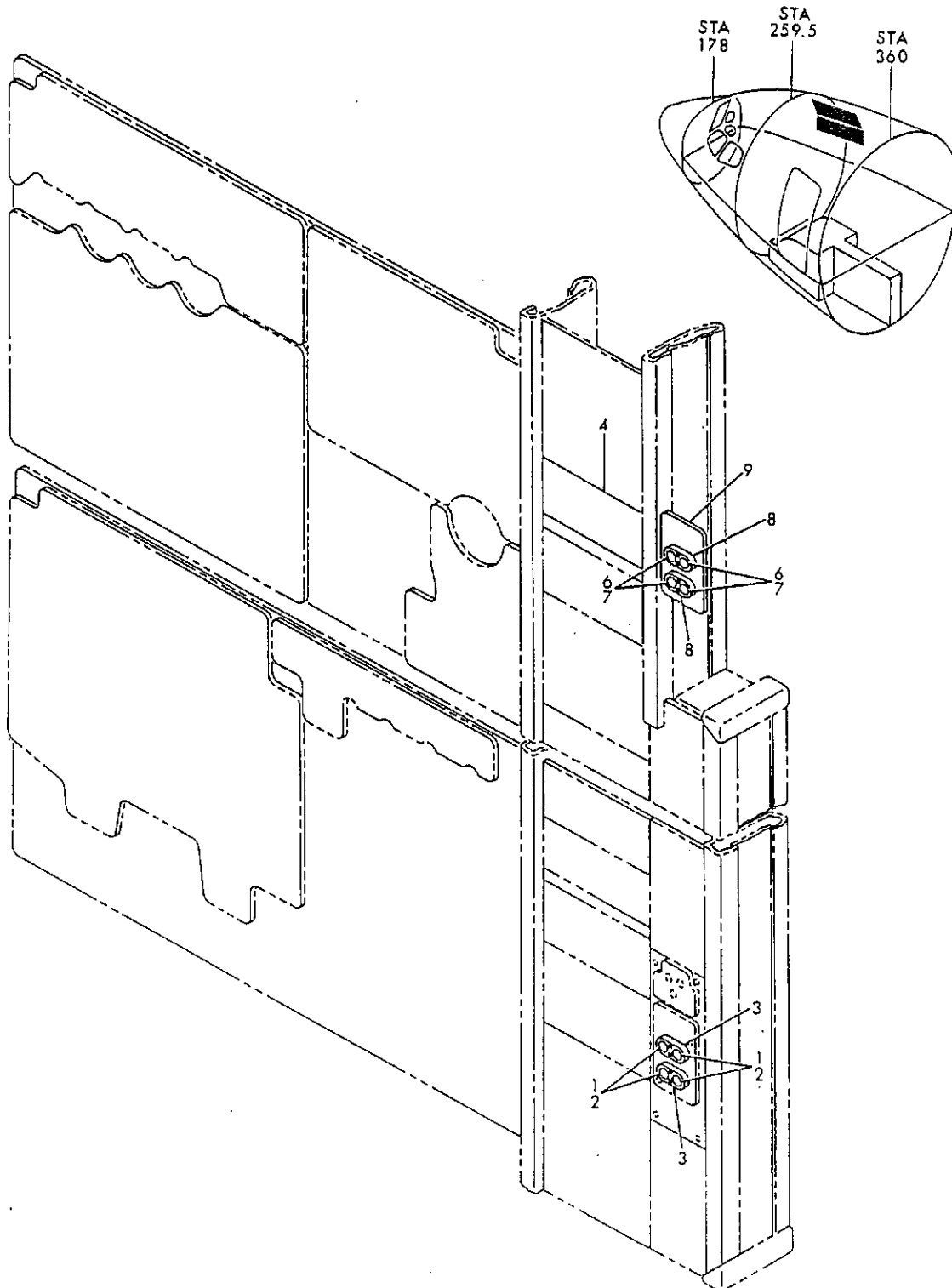
FIGURE 30. PANEL INSTL, FLIGHT ENGINEERS AUXILIARY (LANDING GEAR ONLY)
