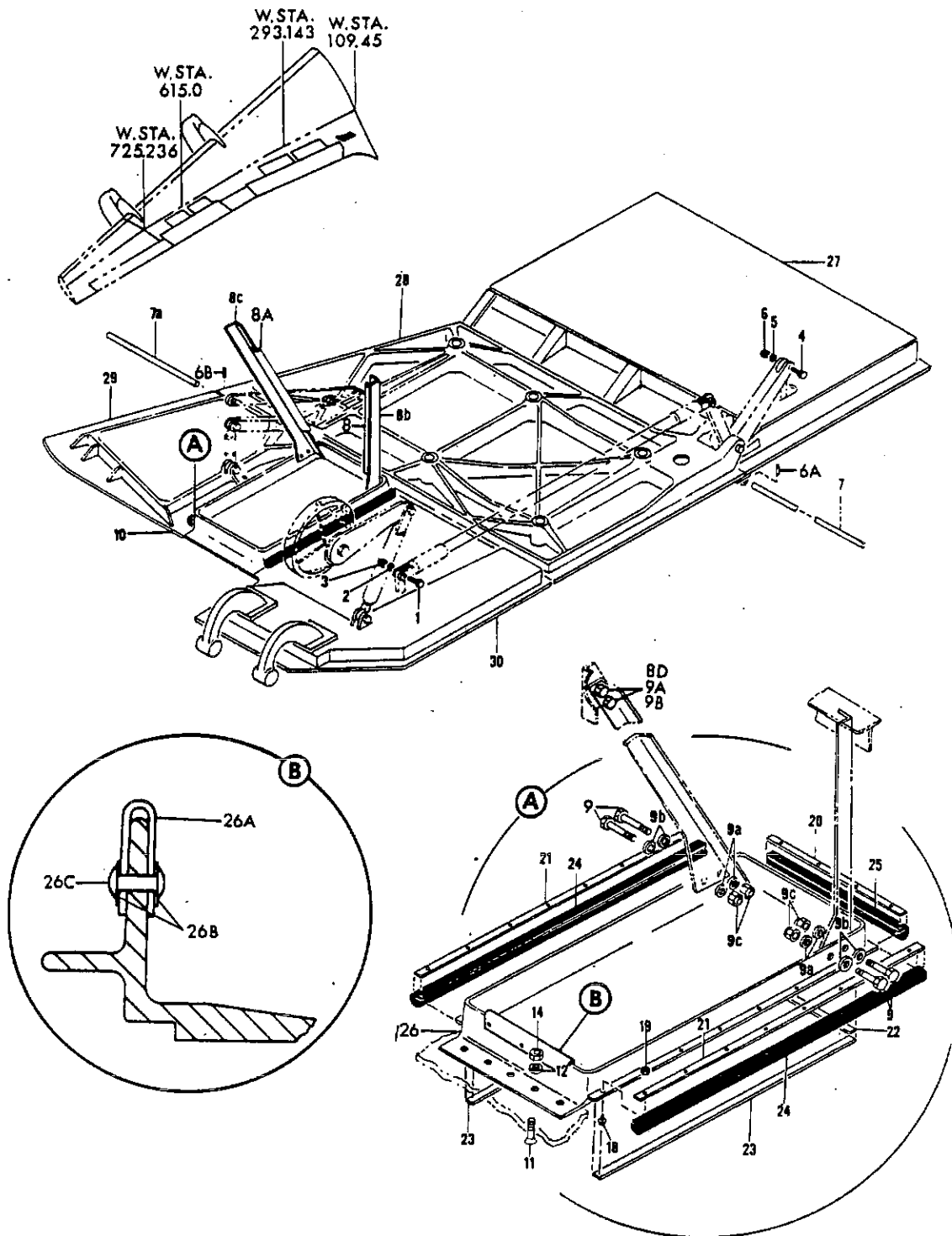
FIGURE 1. DOOR INSTL, SECTION 16 LANDING GEAR
