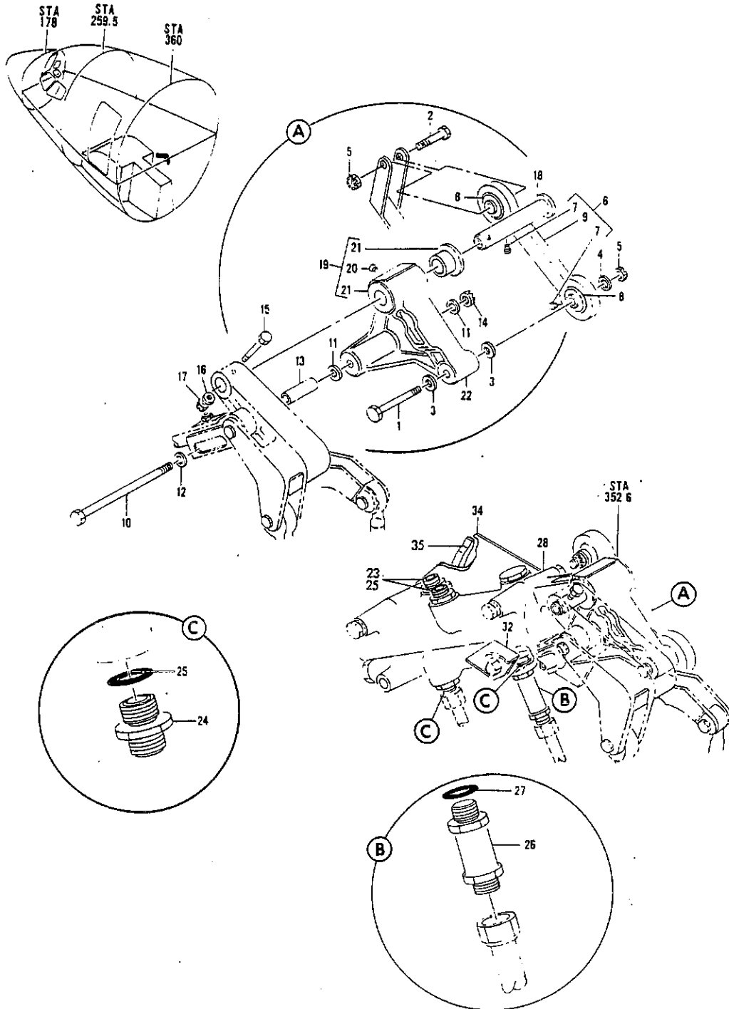
FIGURE 11. VALVE INSTL, DOOR CONTROL NOSE GEAR
