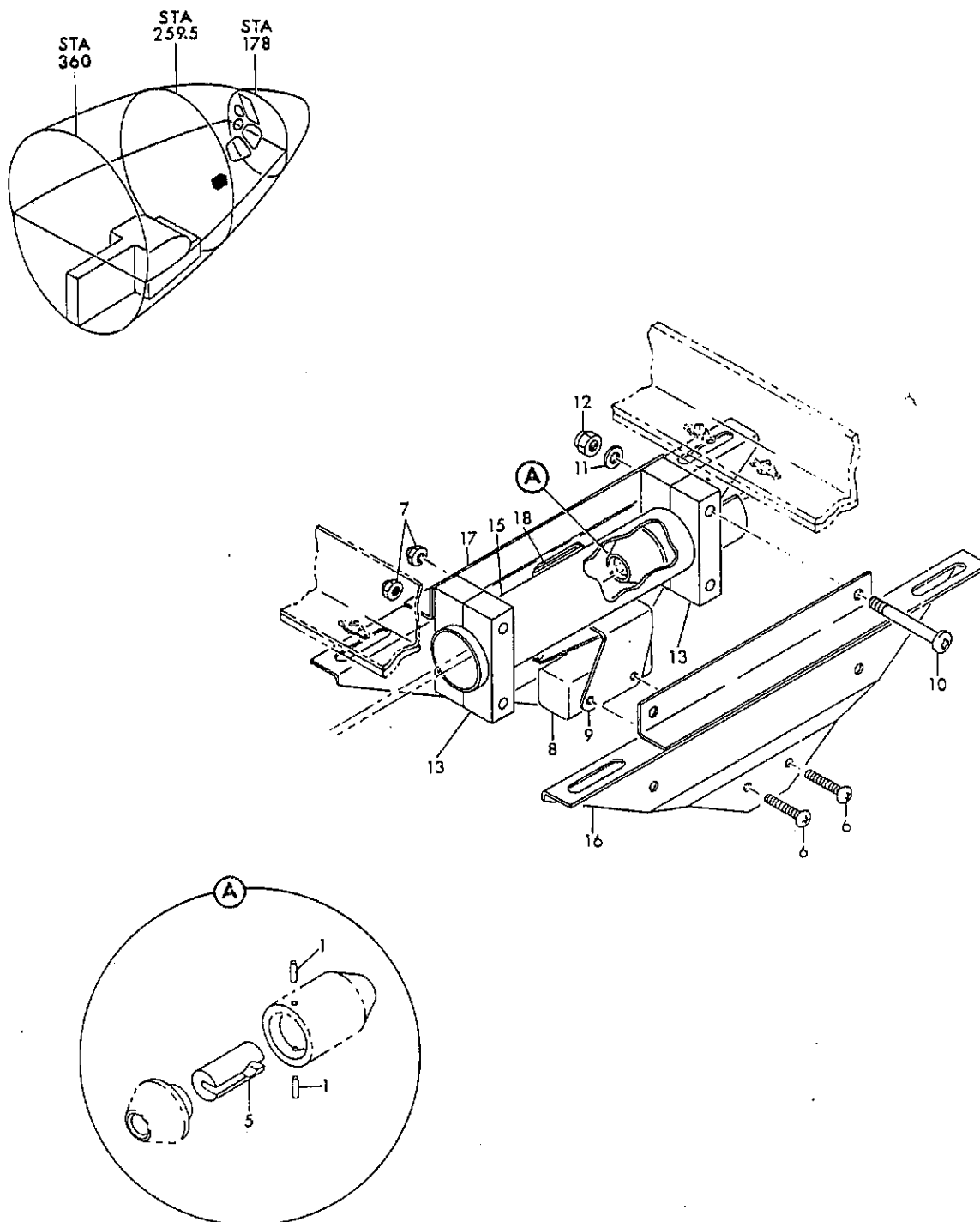
FIGURE 15. SWITCH INSTL, GEAR UP WARNING FLAP POSITION
