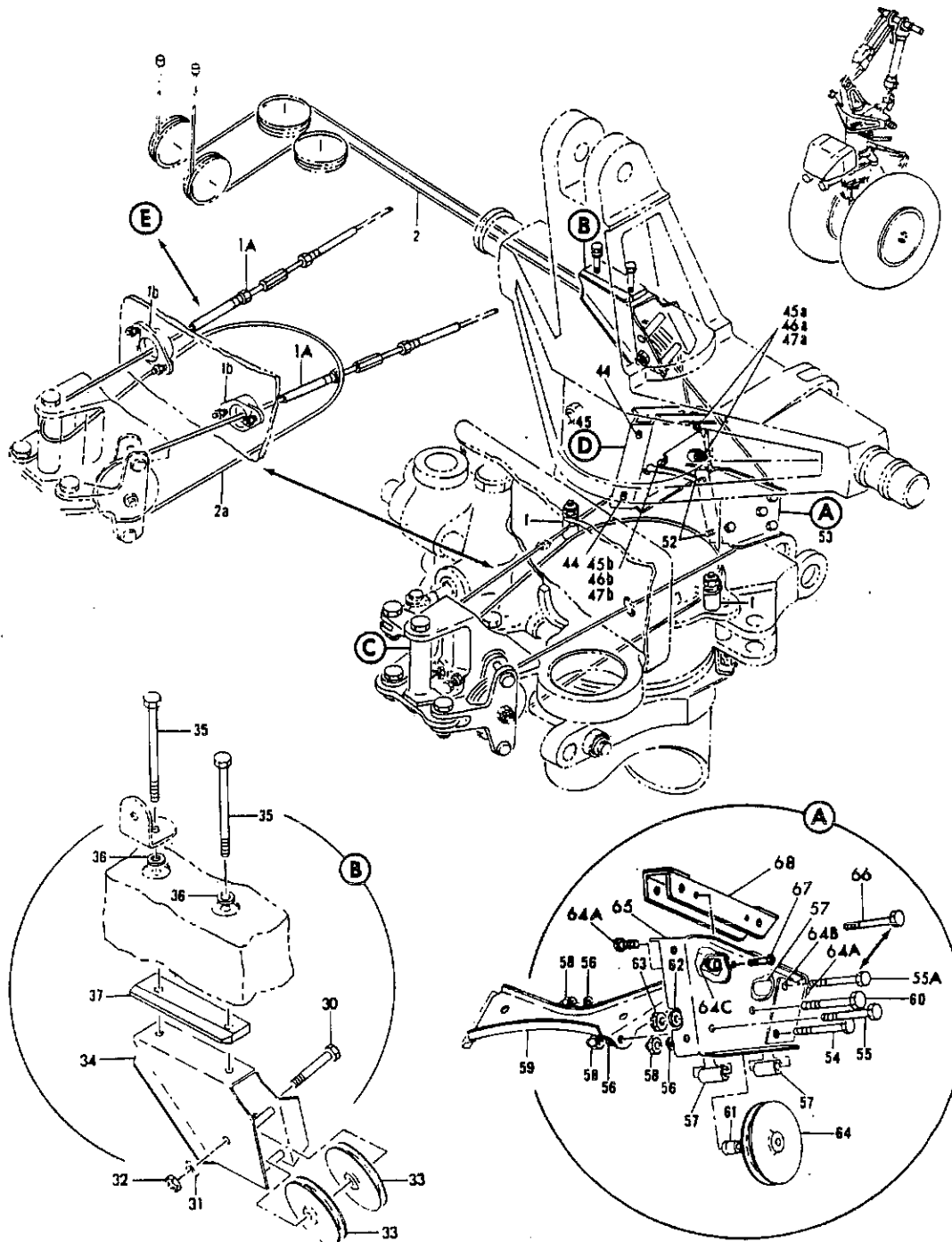
FIGURE 2. CONTROL INSTL. SECTION 67 NOSE WHEEL STEERING (SHEET 1)
