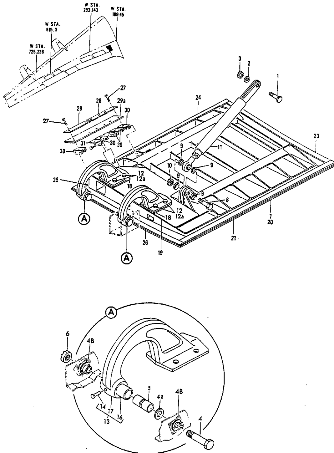
FIGURE 6. DOOR INSTL. LANDING GEAR AFT OUTBOARD
