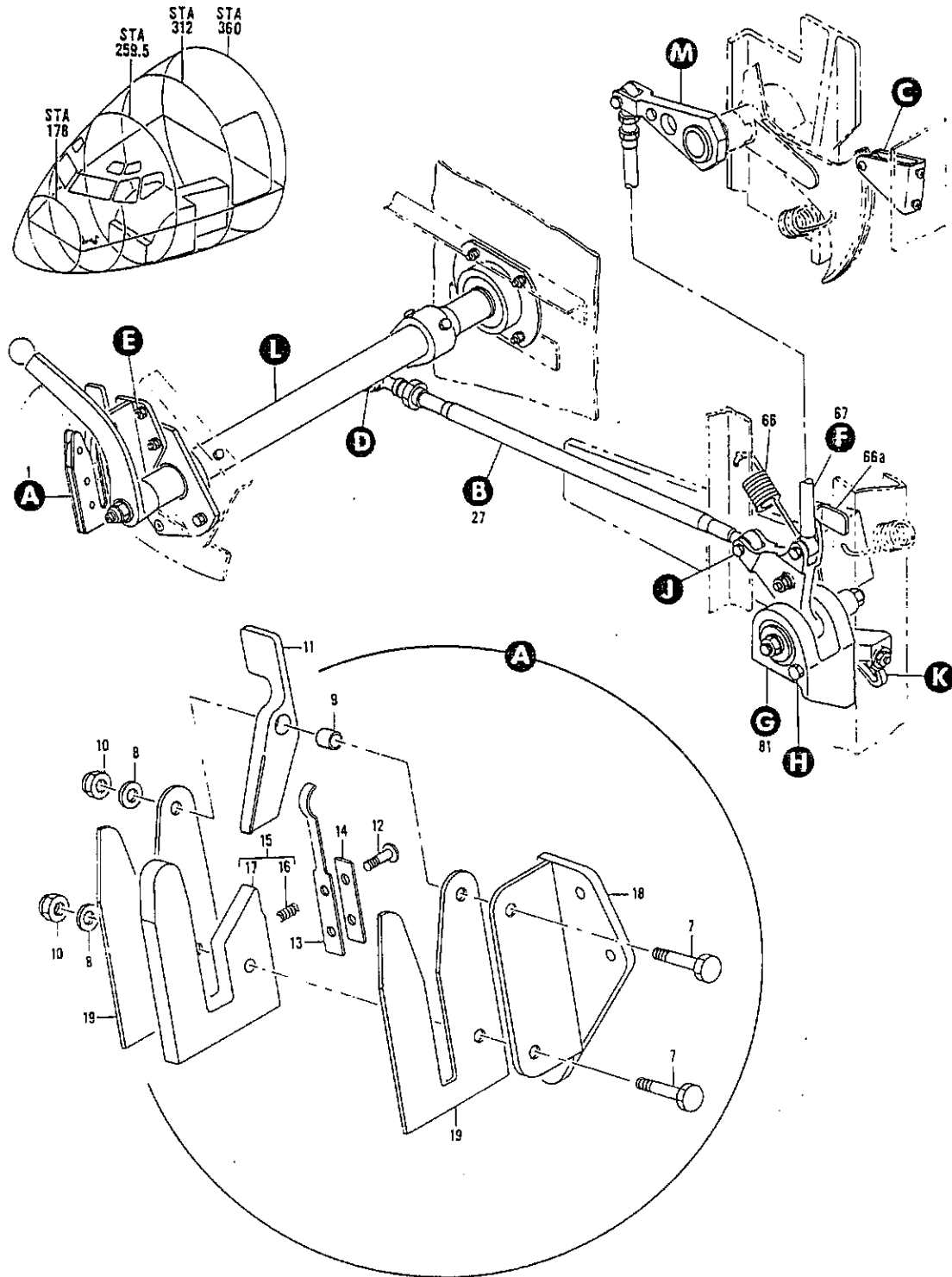
FIGURE 4. CONTROL INSTL, GROUND DOOR RELEASE (SHEET 1)
