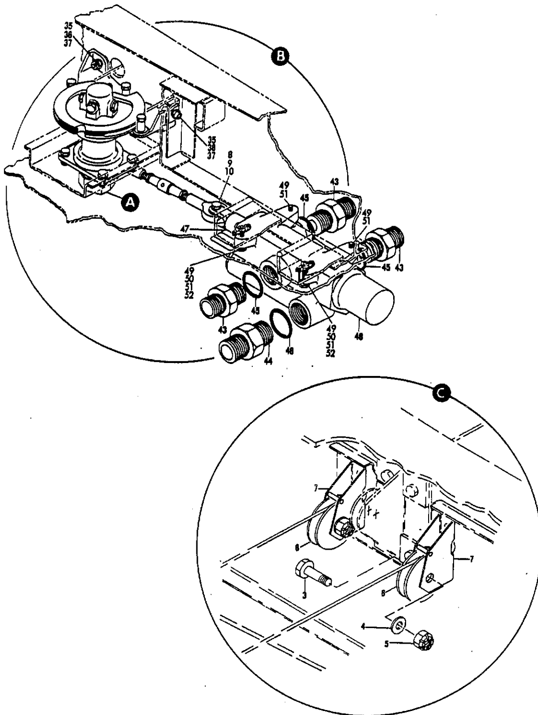
FIGURE 4. CONTROL INSTL, SECTION 53 LANDING GEAR VALVE (SHEET 3)
