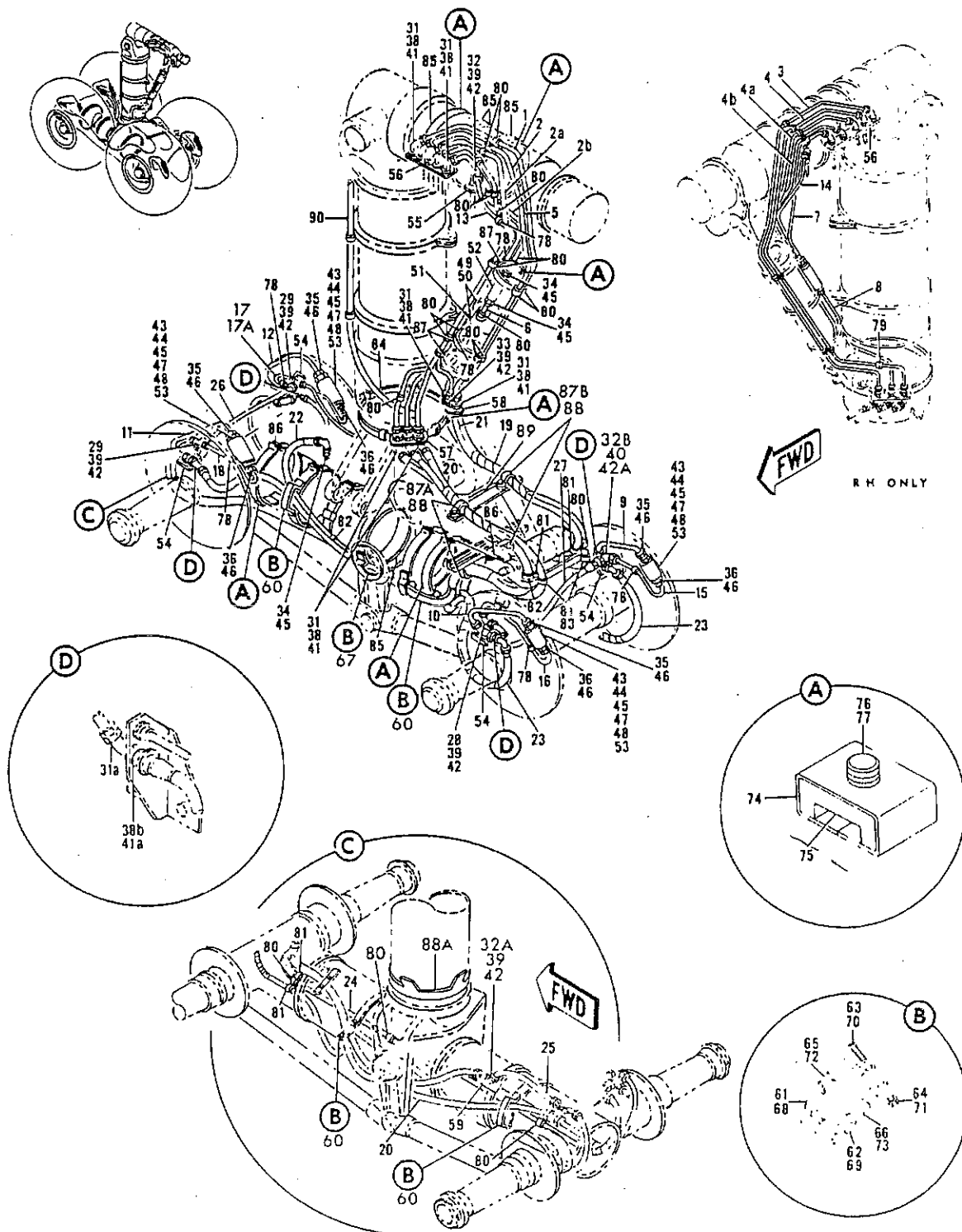
FIGURE 20. HYDRAULIC INSTL, MAIN LANDING GEAR BRAKE SYSTEM
