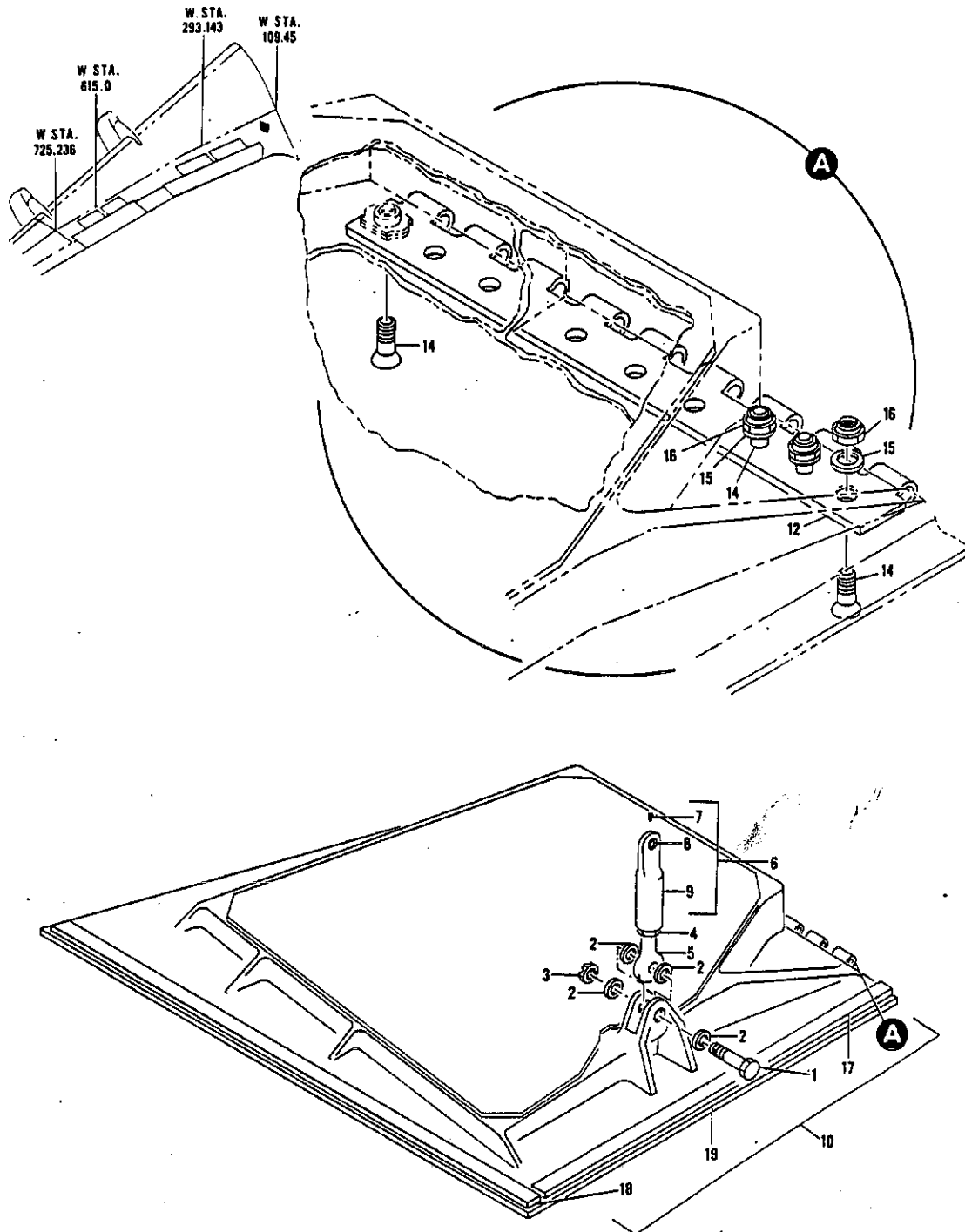
FIGURE 5. DOOR INSTL, LANDING GEAR FORWARD OUTBOARD
