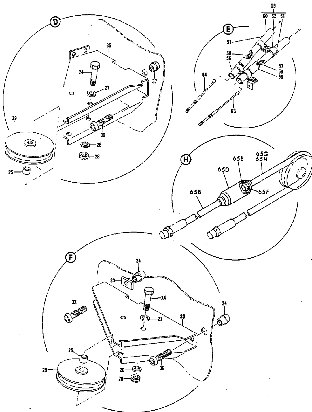
FIGURE 3. CONTROL INSTL, SECTION 51 NOSE WHEEL STEERING (SHEET 3)
