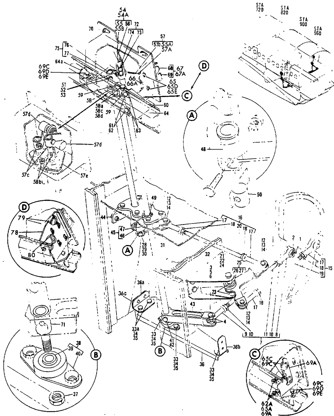
INDICATOR INSTL, MAIN LANDING GEAR EMERGENCY FIGURE 12. SWITCH INSTL, MAIN LANDING GEAR EMERGENCY INDICATOR
