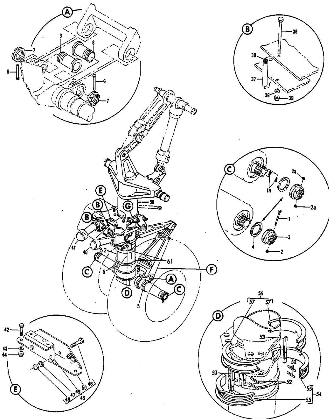
FIGURE 4. GEAR ASSY, SECTION 62 NOSE (SHEET 1)
