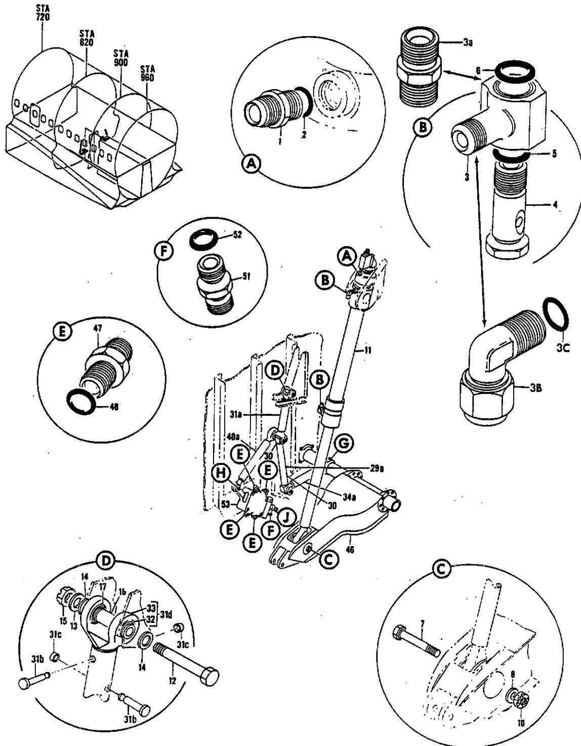
FIGURE 22. MECHANISM INSTL. MAIN GEAR DOOR (SHEET 1)
