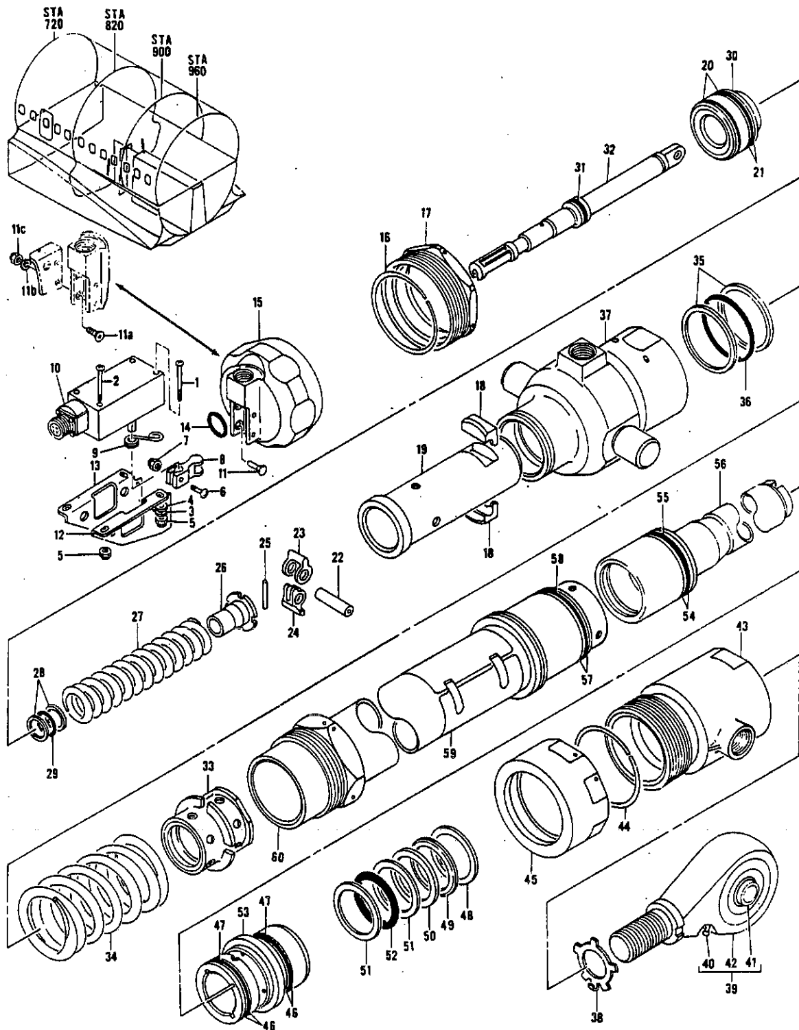
FIGURE 22A. ACTUATOR ASSY, MAIN LANDING GEAR DOOR
