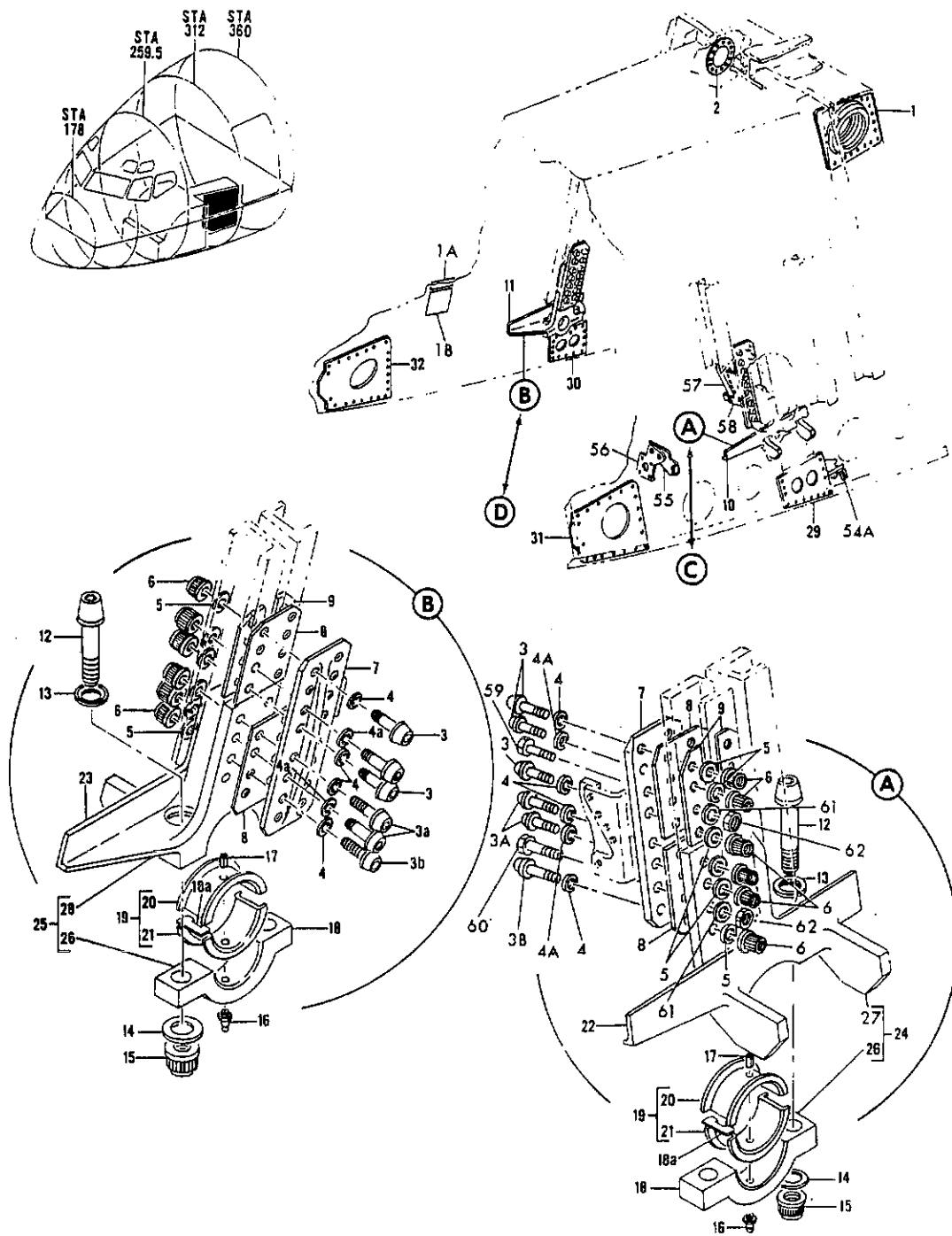
FIGURE 23. PANEL INSTL, STATION 312 TO 360 NOSE GEAR WHEEL WELL SIDE (SHEET 1)
