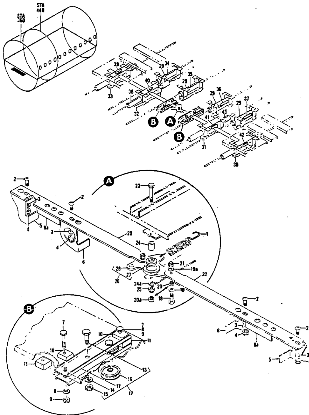
FIGURE 4. SWITCH INSTL, STATION 360 TO 380 THROTTLE OPERATED
