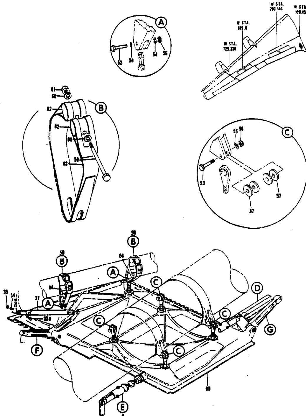
FIGURE 3. DOOR INSTL. WING TRAILING EDGE LANDING GEAR OLED (SHEET 1)
