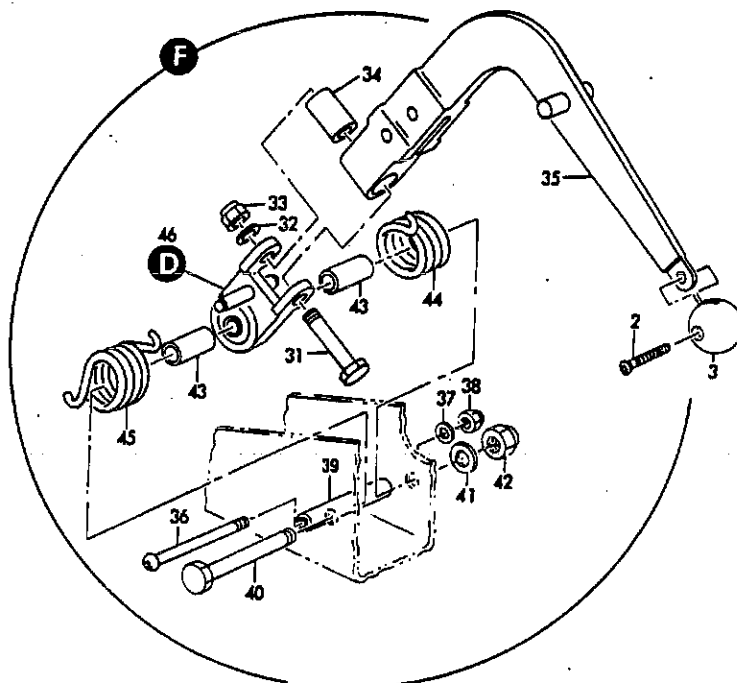
FIGURE 20. CONTROL INSTL. LANDING GEAR GROUND DOOR RELEASE (LANDING GEAR ONLY) (SHEET 3)
