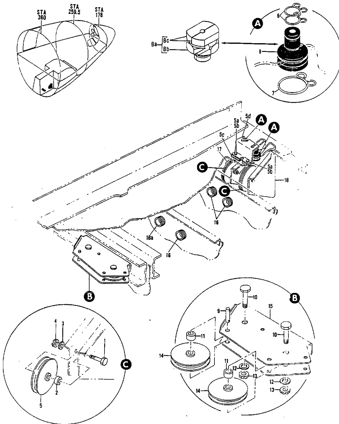
FIGURE 8. BRACKET INSTL, NOSE GEAR STEERING CONTROL
