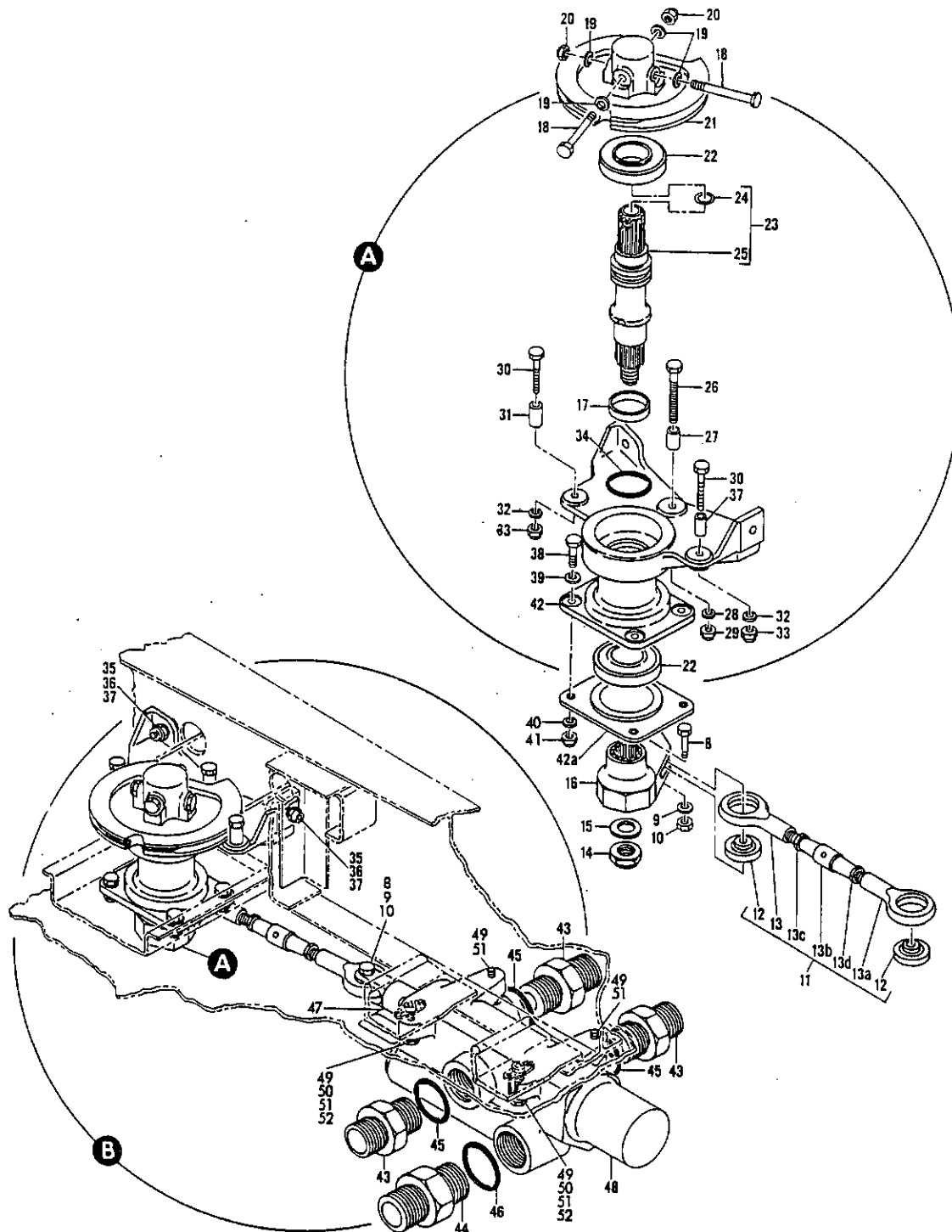
FIGURE 4. CONTROL INSTL, SECTION 53 LANDING GEAR VALVE (SHEET 2)
