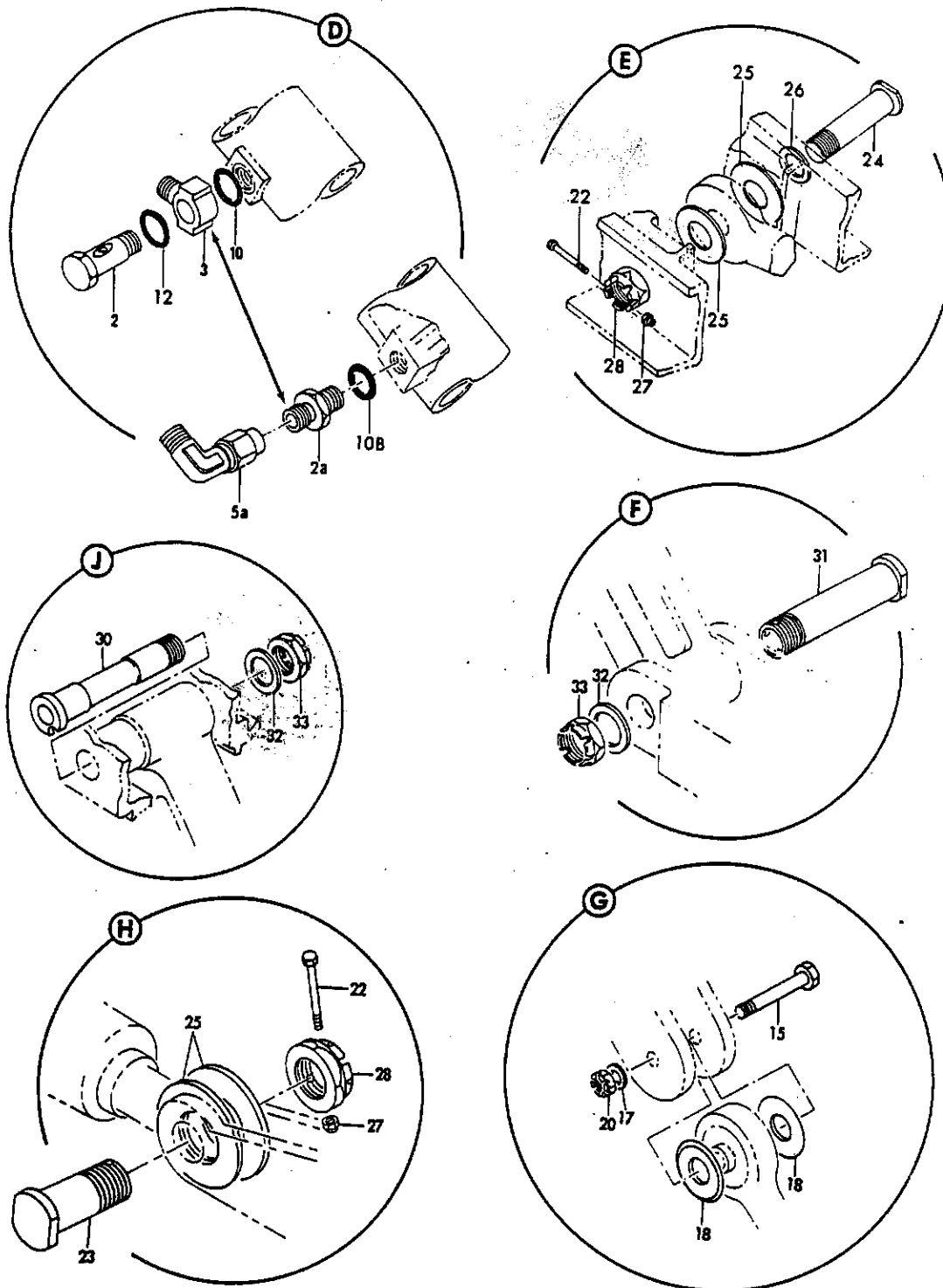
FIGURE 2. GEAR INSTL, SECTION 61 MAIN LANDING (LH) MAIN GEAR, BUILD-UP (LH) (SHEET 2)
