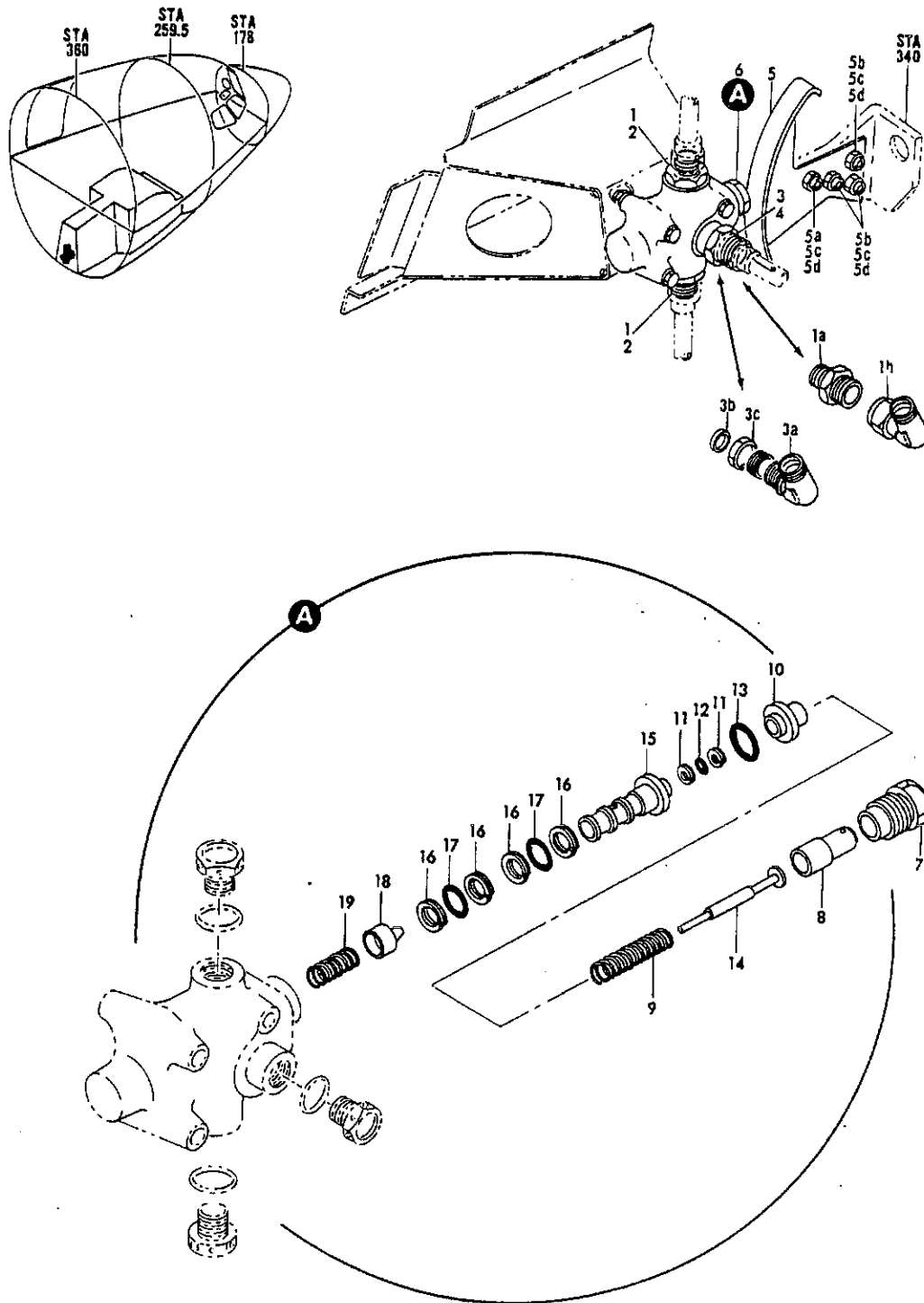
FIGURE 20. VALVE INSTL, NOSE GEAR STEERING DISCONNECT
