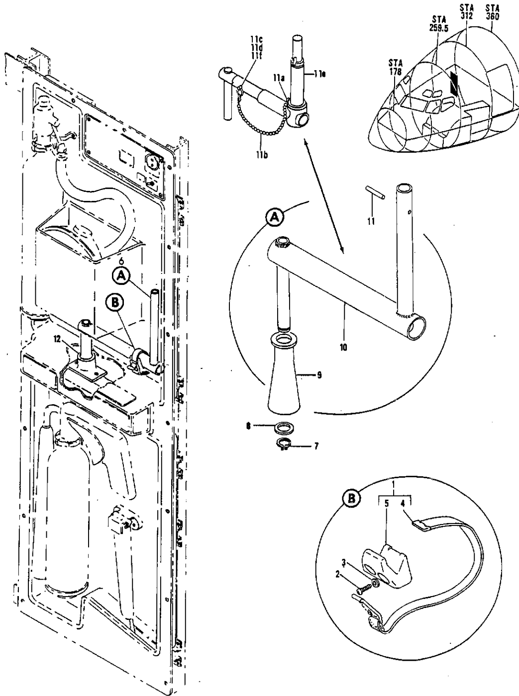
FIGURE 15. EQUIPMENT INSTL, CONTROL CAB EMERGENCY (LANDING GEAR ONLY)
