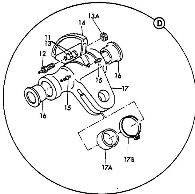
FIGURE 5. STRUT ASSY, SECTION 61 MAIN GEAR SIDE (SHEET 2)
