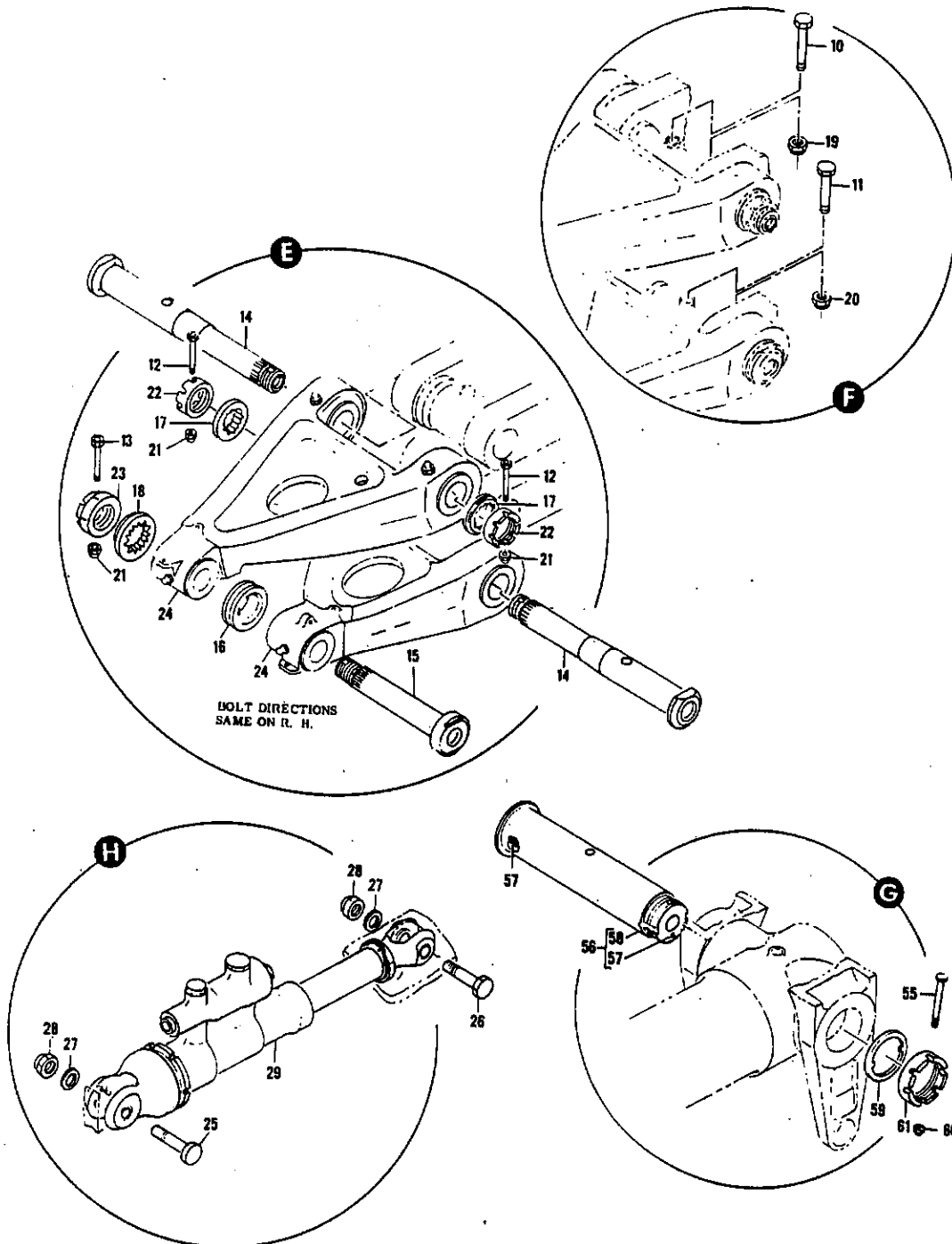
FIGURE 9. COMPONENT ASSY, MAIN GEAR (SHEET 2)
