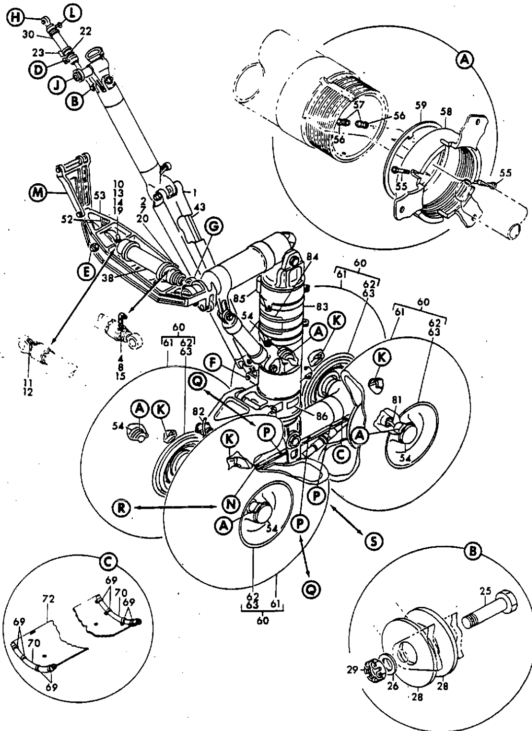
FIGURE 2B. GEAR INSTL, SECTION 61 MAIN LANDING (RH) MAIN GEAR, BUILD-UP (RH) (SHEET 1)
