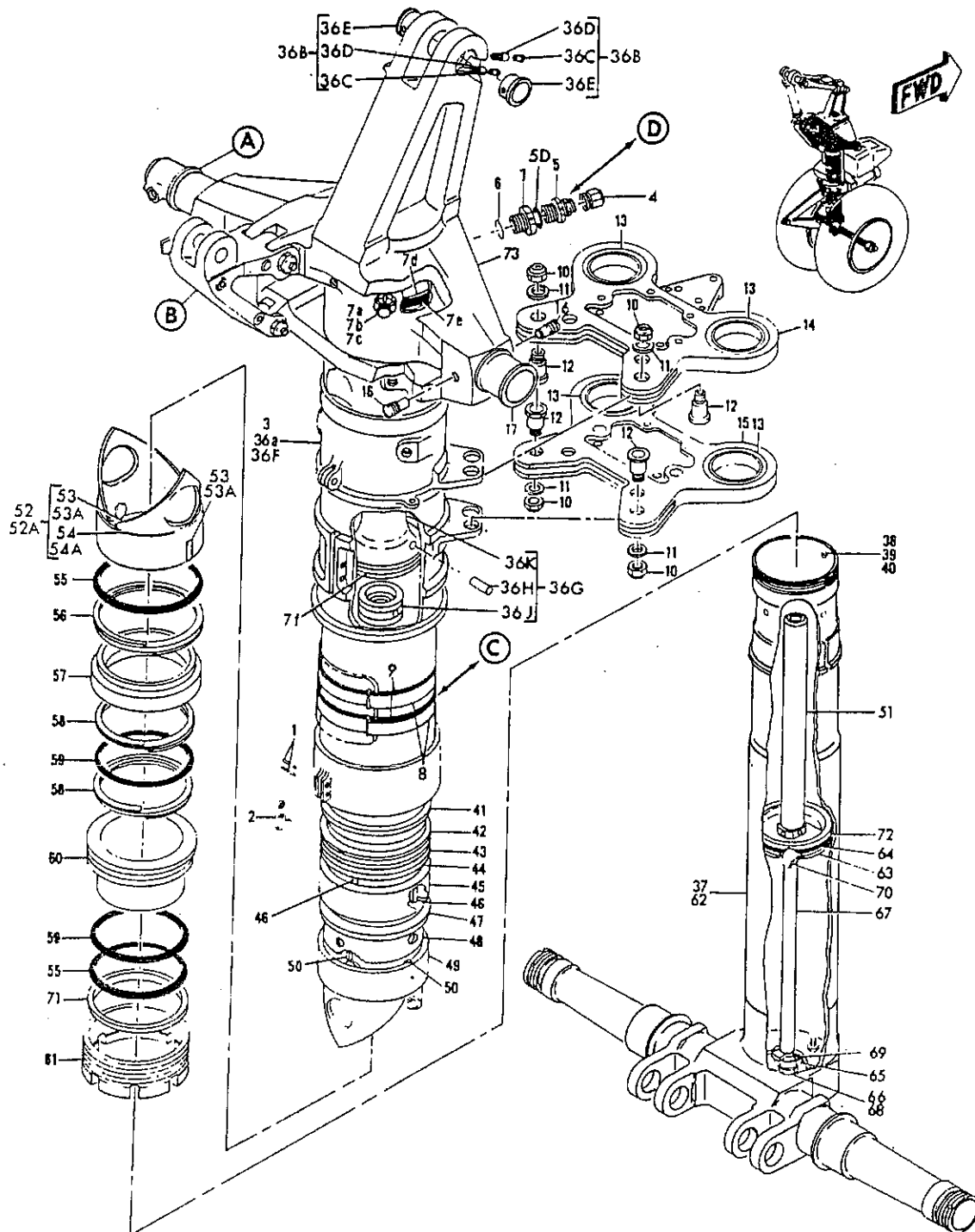
FIGURE 7. OLEO ASSY, NOSE GEAR (SHEET 1)
