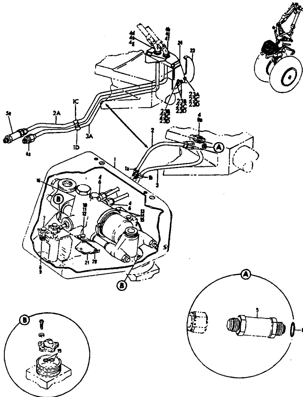
FIGURE 13 HYDRAULIC INSTL, NOSE GEAR STEERING (HYDRAULIC POWER ONLY)
