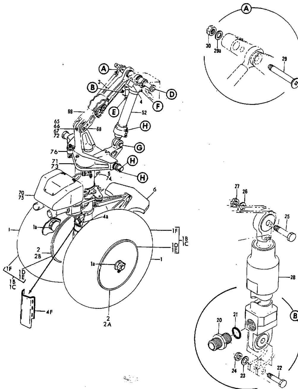
FIGURE 2 GEAR INSTL. SECTION 62 NOSE (SHEET 1)
