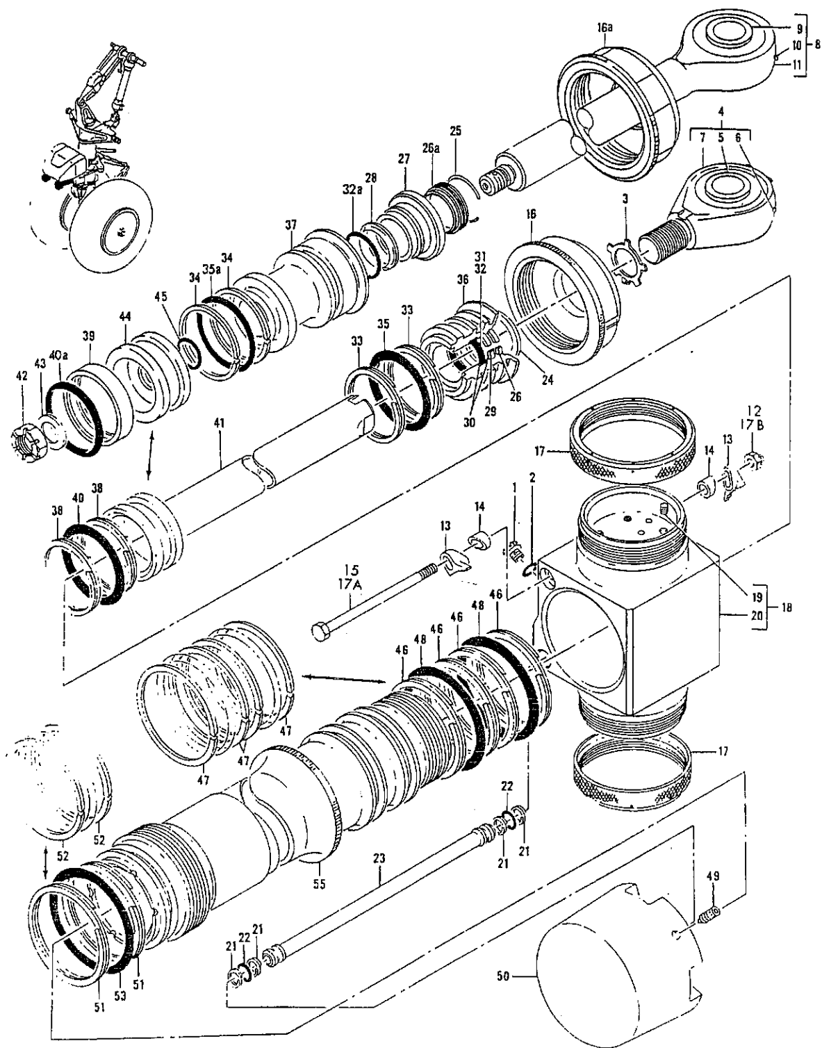
FIGURE 8A CYLINDER ASSY, NOSE WHEEL STEERING (LANDING GEAR ONLY)
