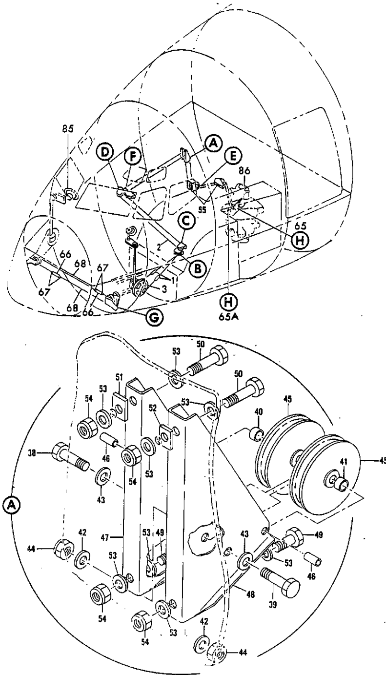
FIGURE 3. CONTROL INSTL, SECTION 51 NOSE WHEEL STEERING (SHEET 1)
