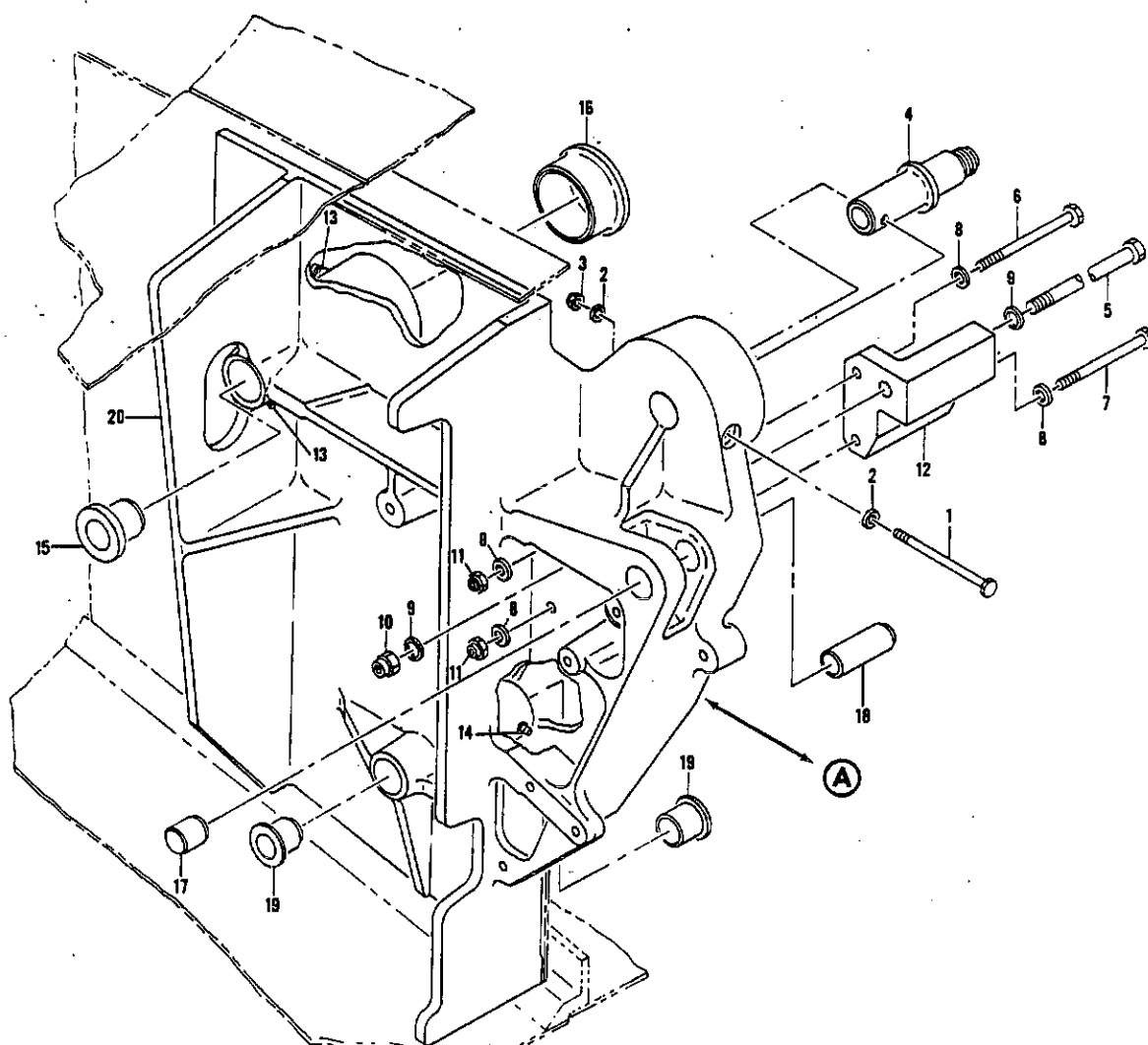
FIGURE 38. SUPPORT ASSY. MAIN LANDING GEAR LOCK
