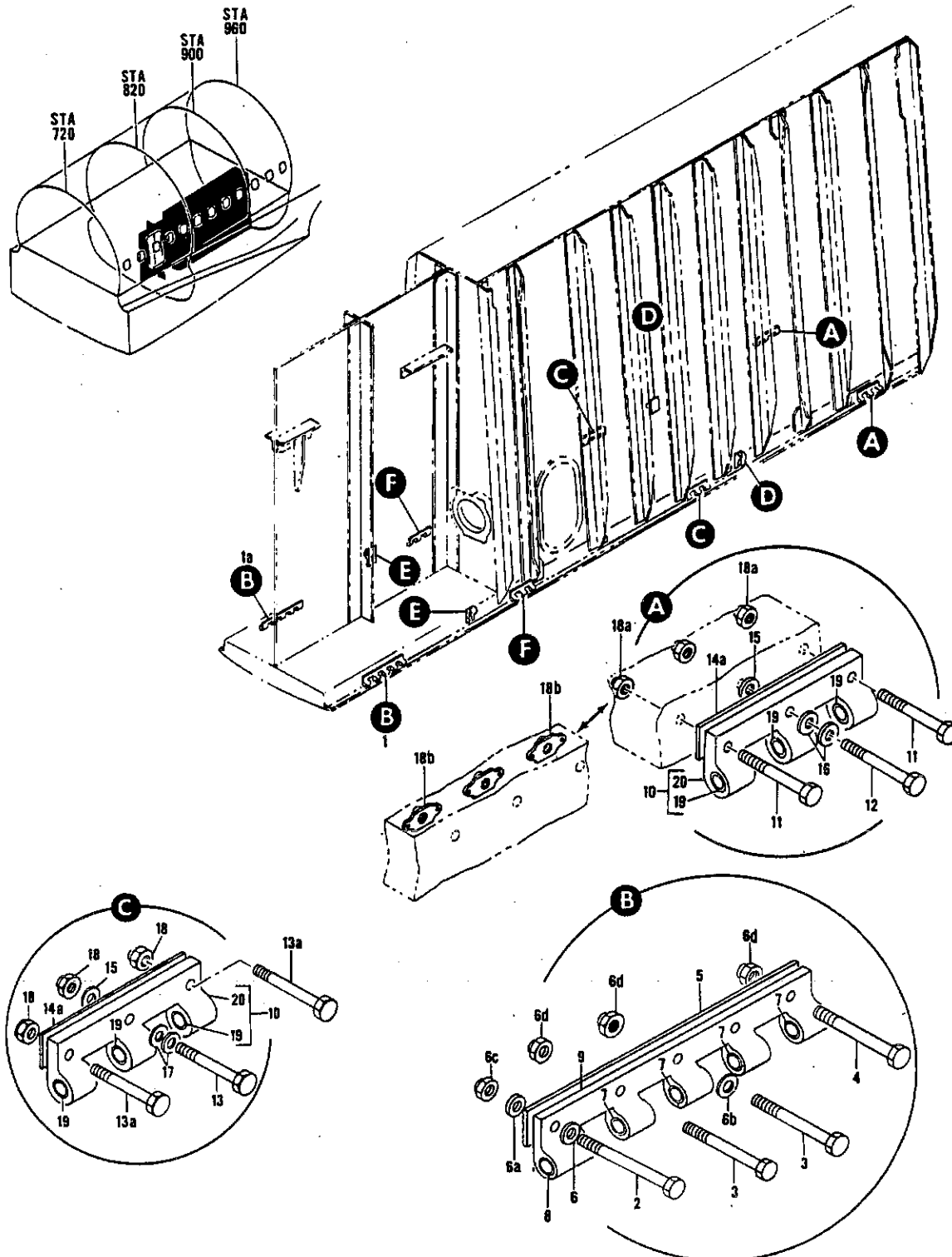
FIGURE 15. BEAM INSTL, STATION 820 TO 960 KEEL (LANDING GEAR ONLY) (SHEET 1)
