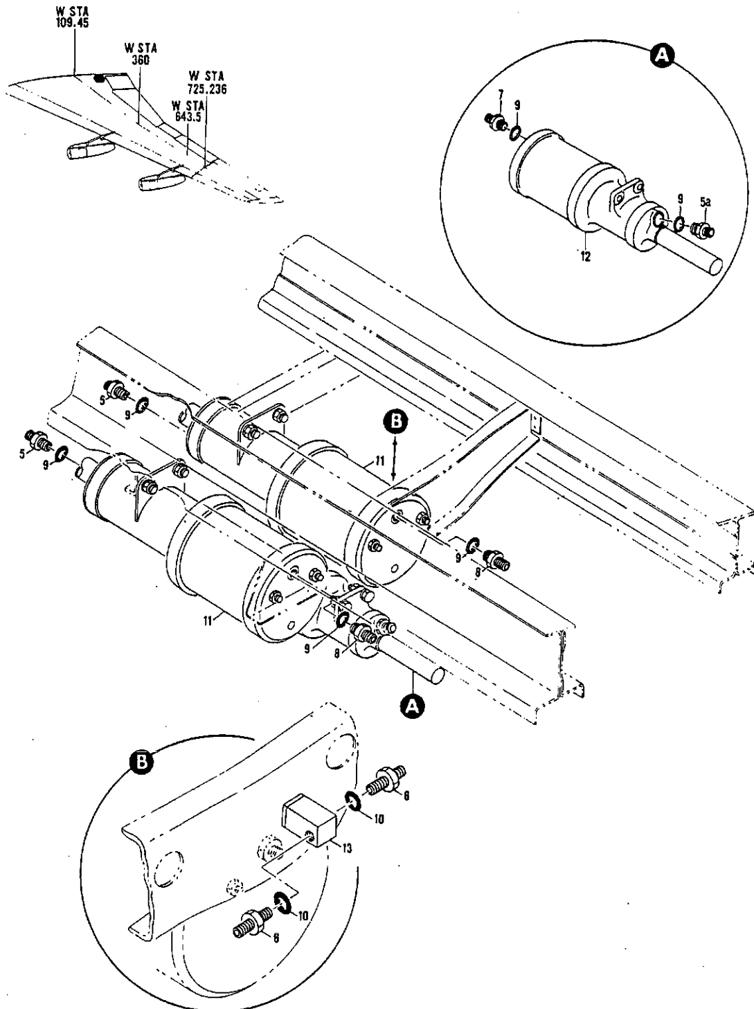
FIGURE 11. VALVE INSTL, BRAKE DEBOOST (LANDING GEAR ONLY)
