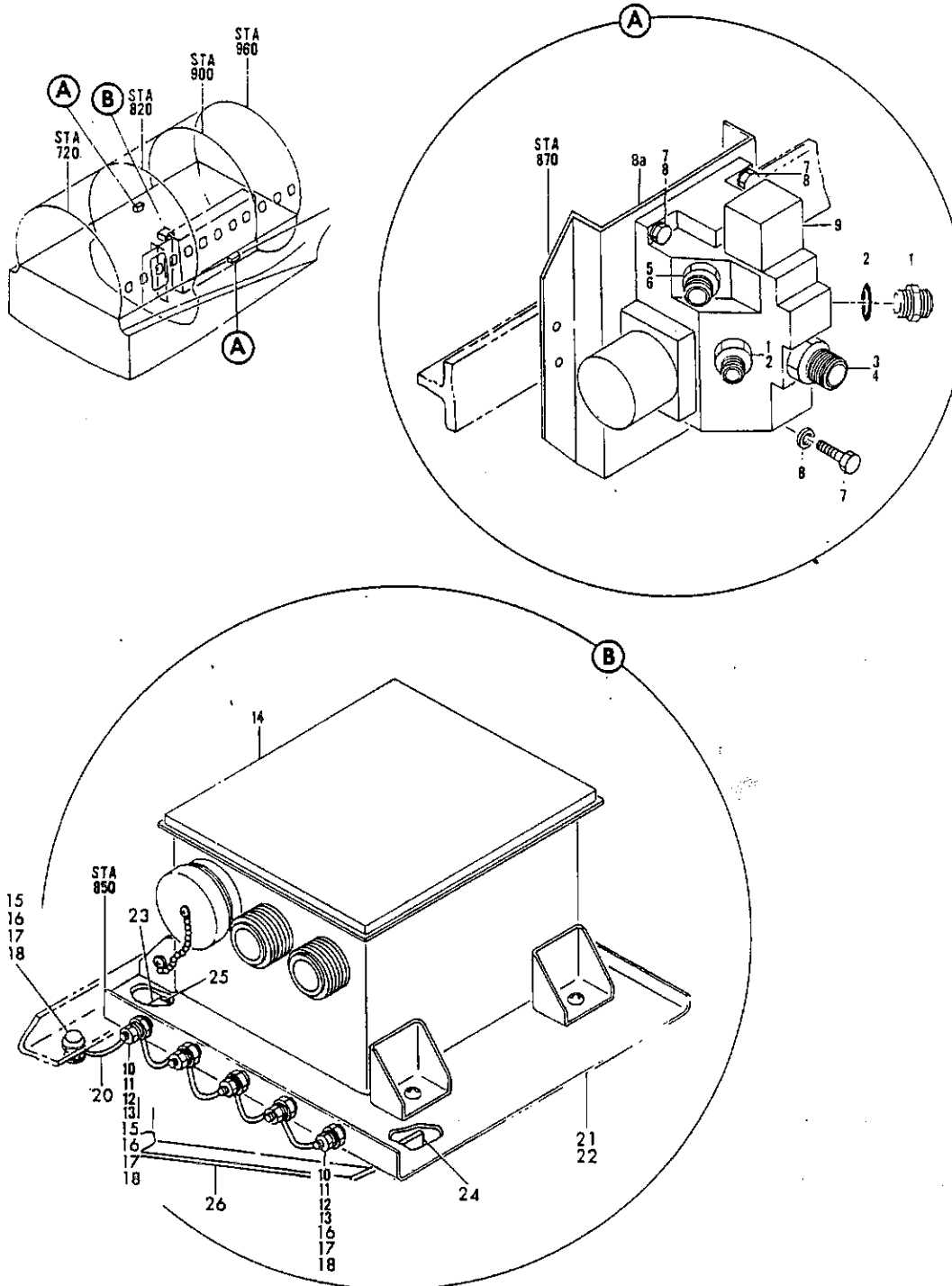
VALVE INSTL, HYDRAULIC BRAKE ANTI-SKID SHIELD INSTL, SKID DETECTOR CONTROL FIGURE 9. SUPPORT INSTL, SKID DETECTOR CONTROL
