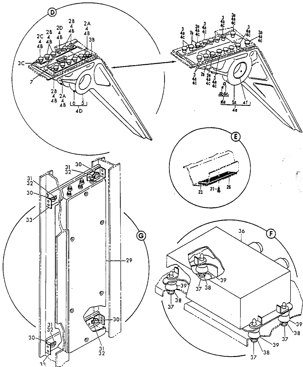
FIGURE 22. WHEEL WELL INSTL, NOSE GEAR (SHEET 2)
