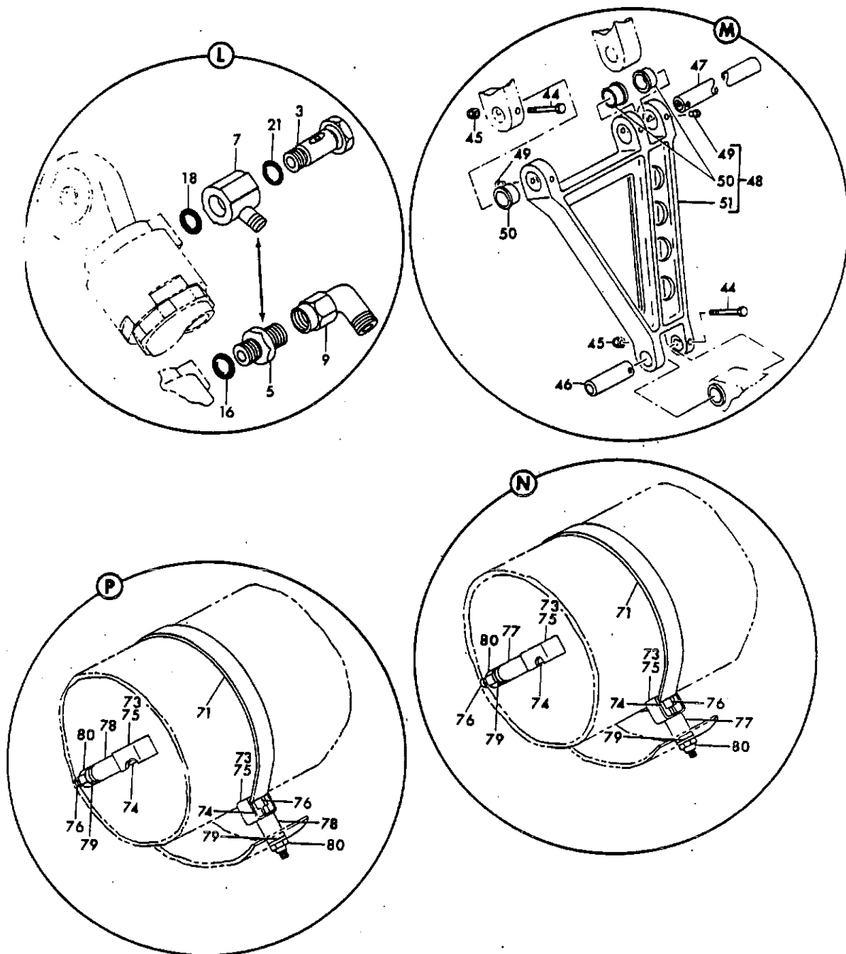
FIGURE 2B. GEAR INSTL, SECTION 61 MAIN LANDING (RH) MAIN GEAR, BUILD-UP (RH) (SHEET 3)
