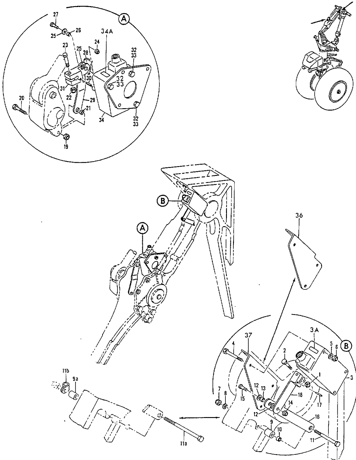
FIGURE 16. SWITCH INSTL, NOSE GEAR POSITION AND LOCK BRACKET INSTL, NOSE GEAR POSITION SWITCH
