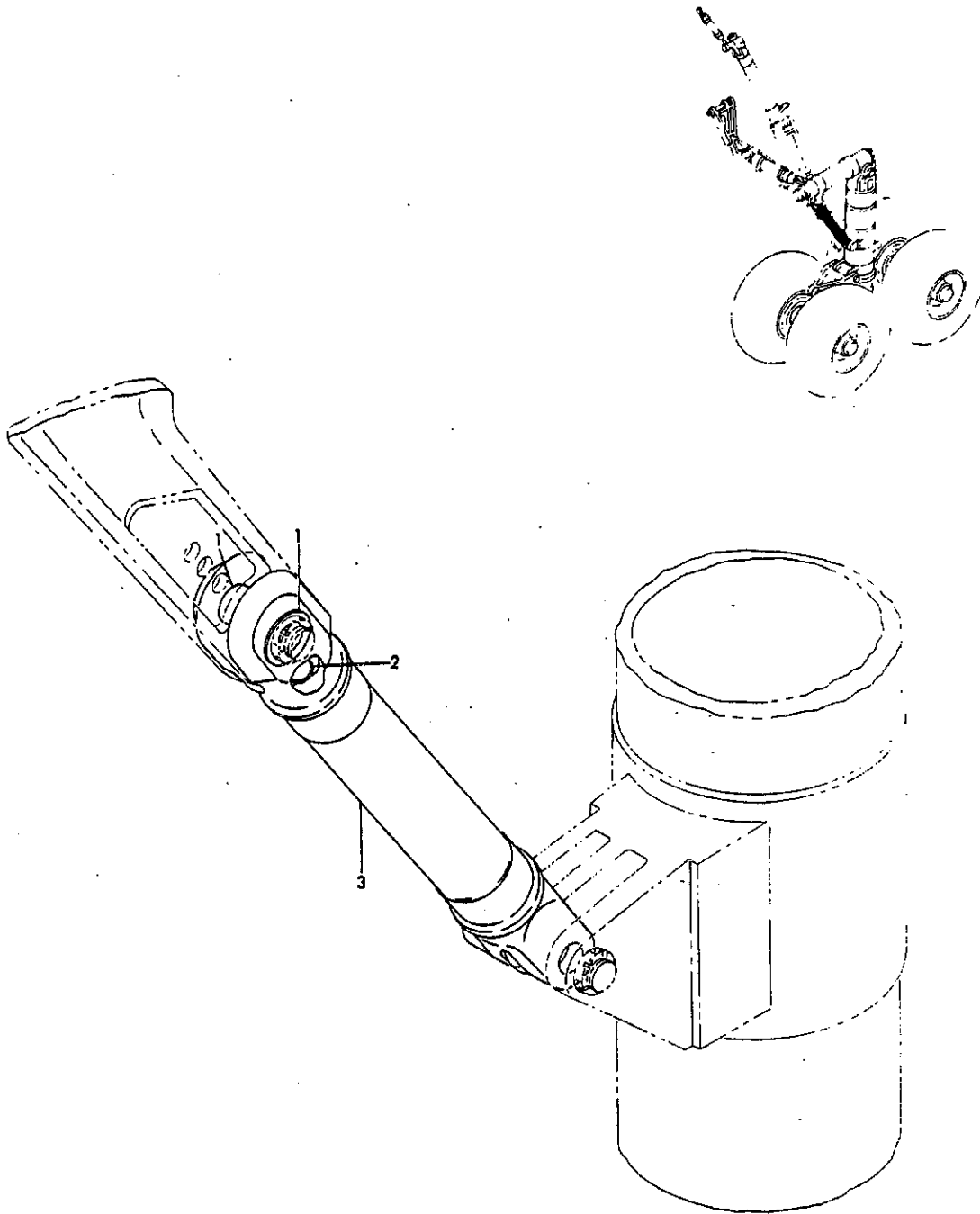
FIGURE 24. STRUT ASSY, MAIN GEAR DRAG
