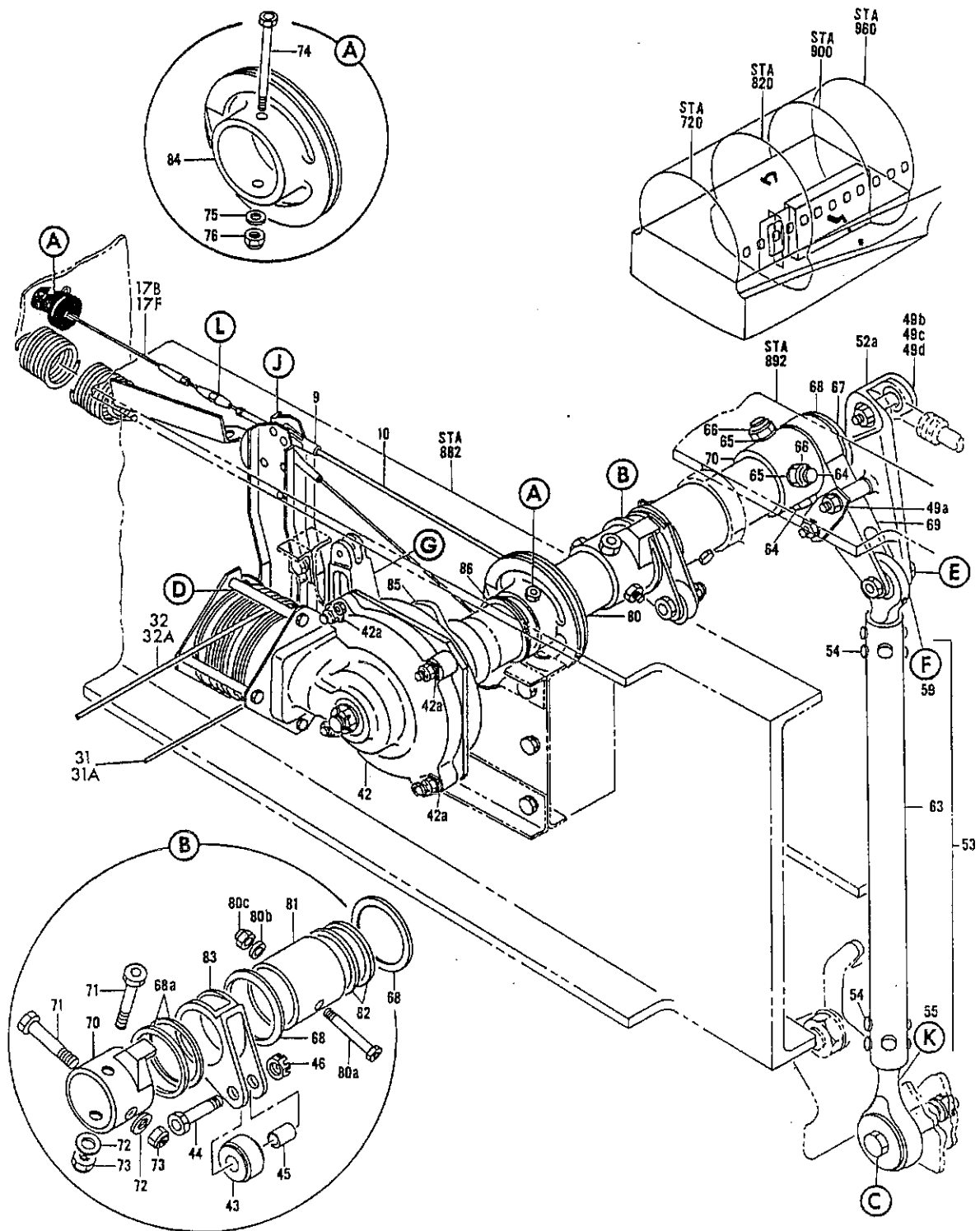
FIGURE 11. RELEASE INSTL, MAIN GEAR EMERGENCY (SHEET 1)
