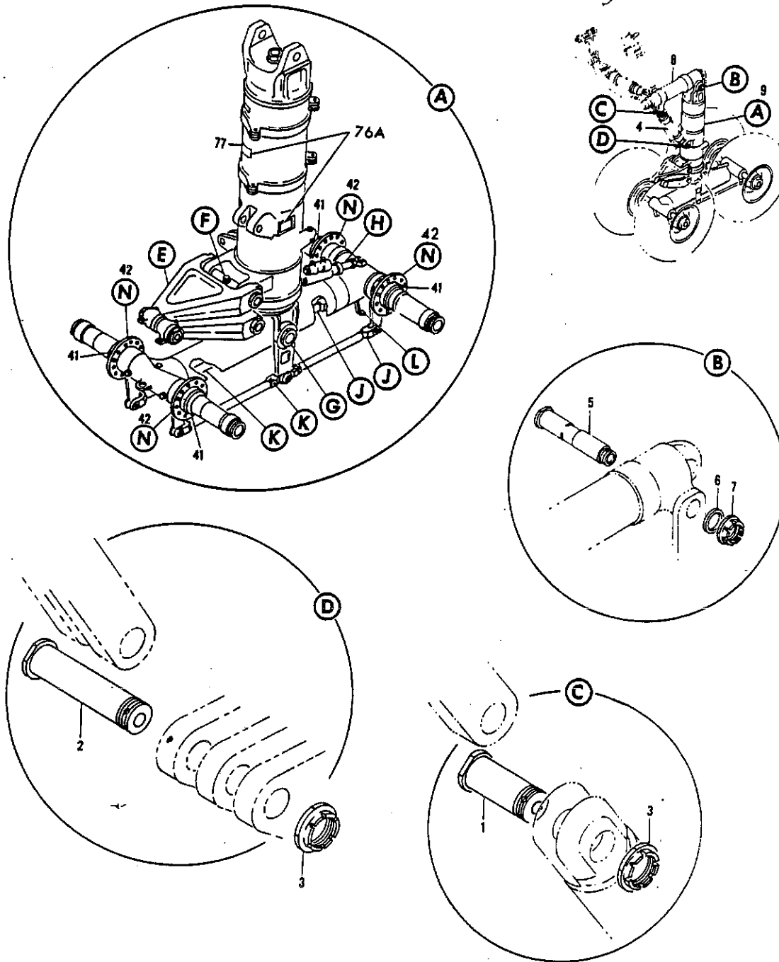
FIGURE 9. COMPONENT ASSY, MAIN GEAR (SHEET 1)
