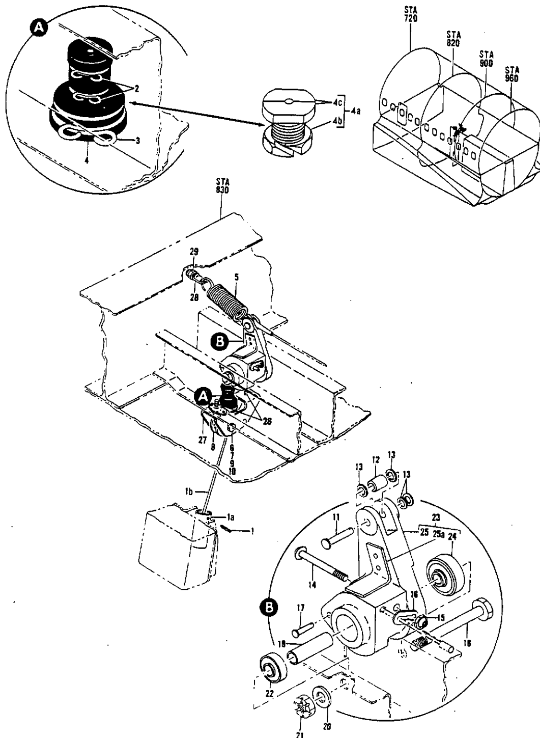
FIGURE 13. BELLCRANK INSTL, MAIN WHEEL WELL EMERGENCY DOOR RELEASE
