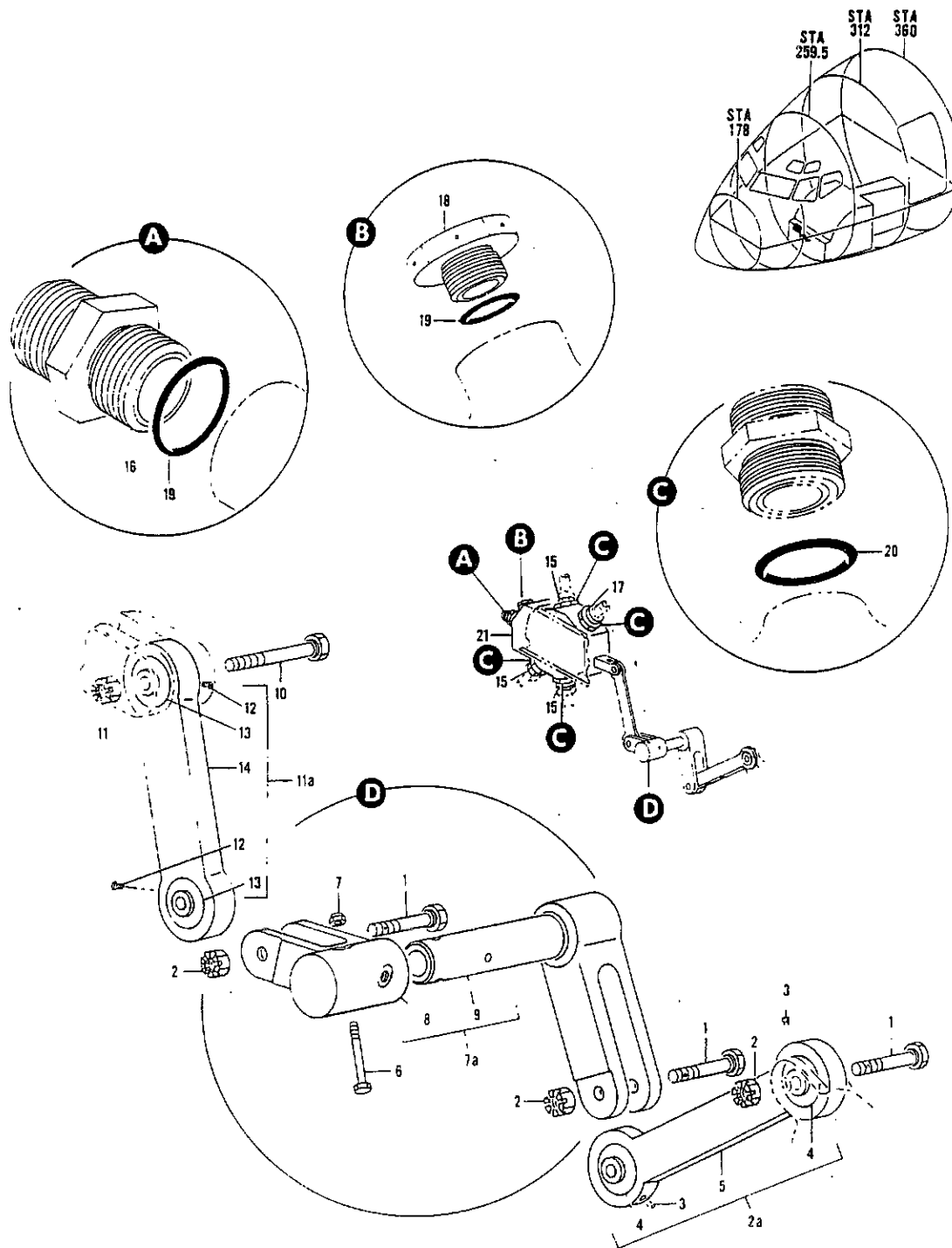
FIGURE 12. MECHANISM INSTL, NOSE GEAR DOOR OPERATED SEQUENCE VALVE
