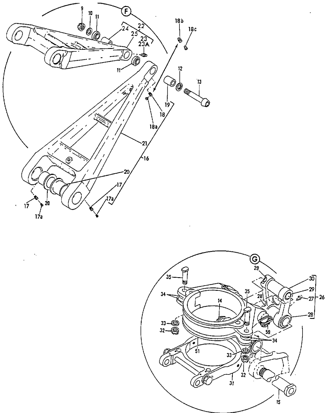
FIGURE 4. GEAR ASSY, SECTION 62 NOSE (SHEET 2)
