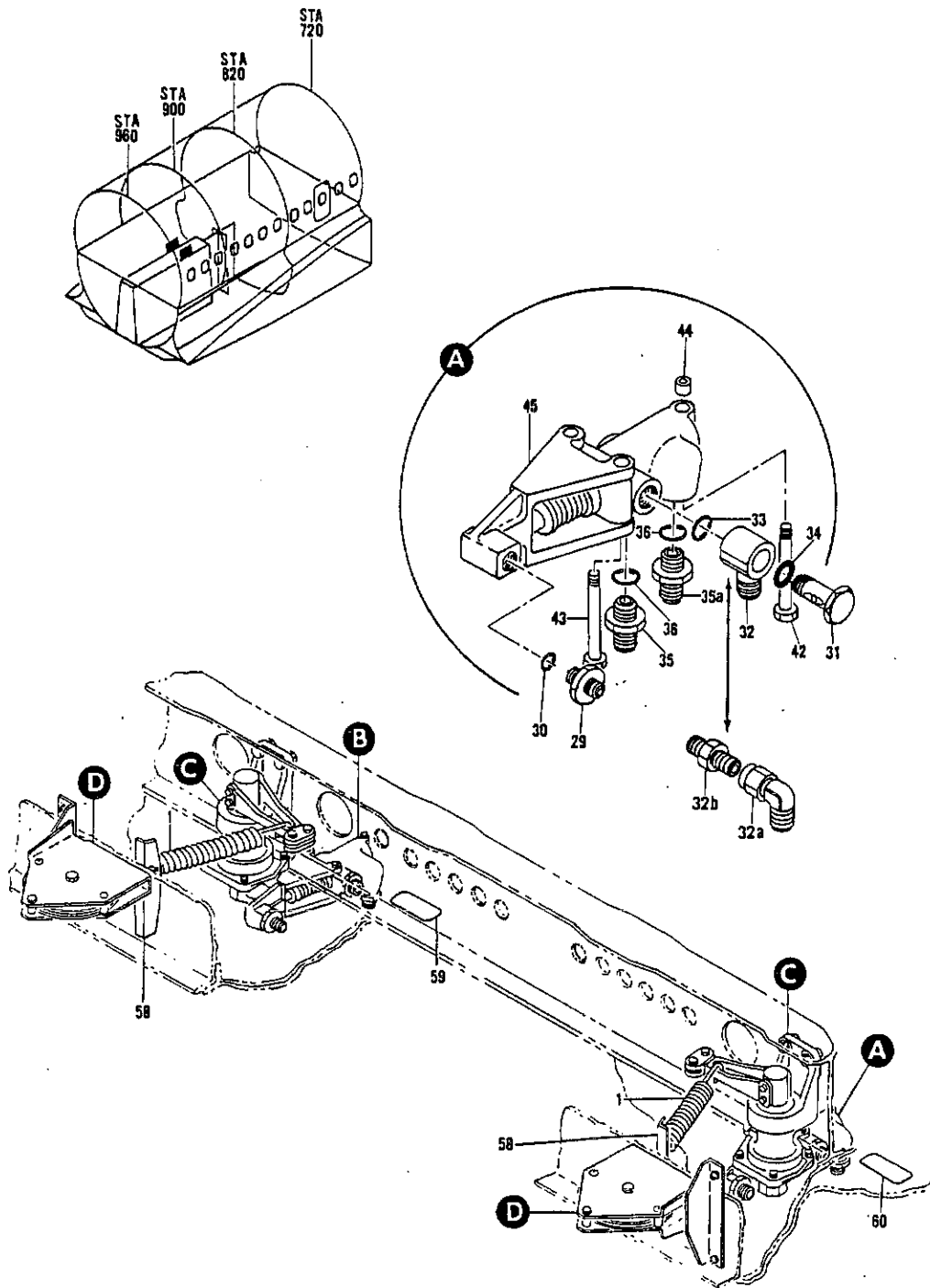
FIGURE 7. CONTROL INSTL, STATION 830 BRAKE (SHEET 1)
