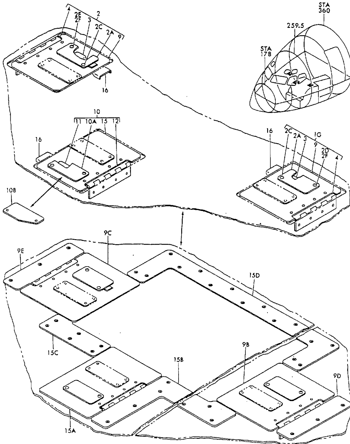
FIGURE 3. DOOR INSTL, EMERGENCY MAIN AND NOSE GEAR EXTENSION
