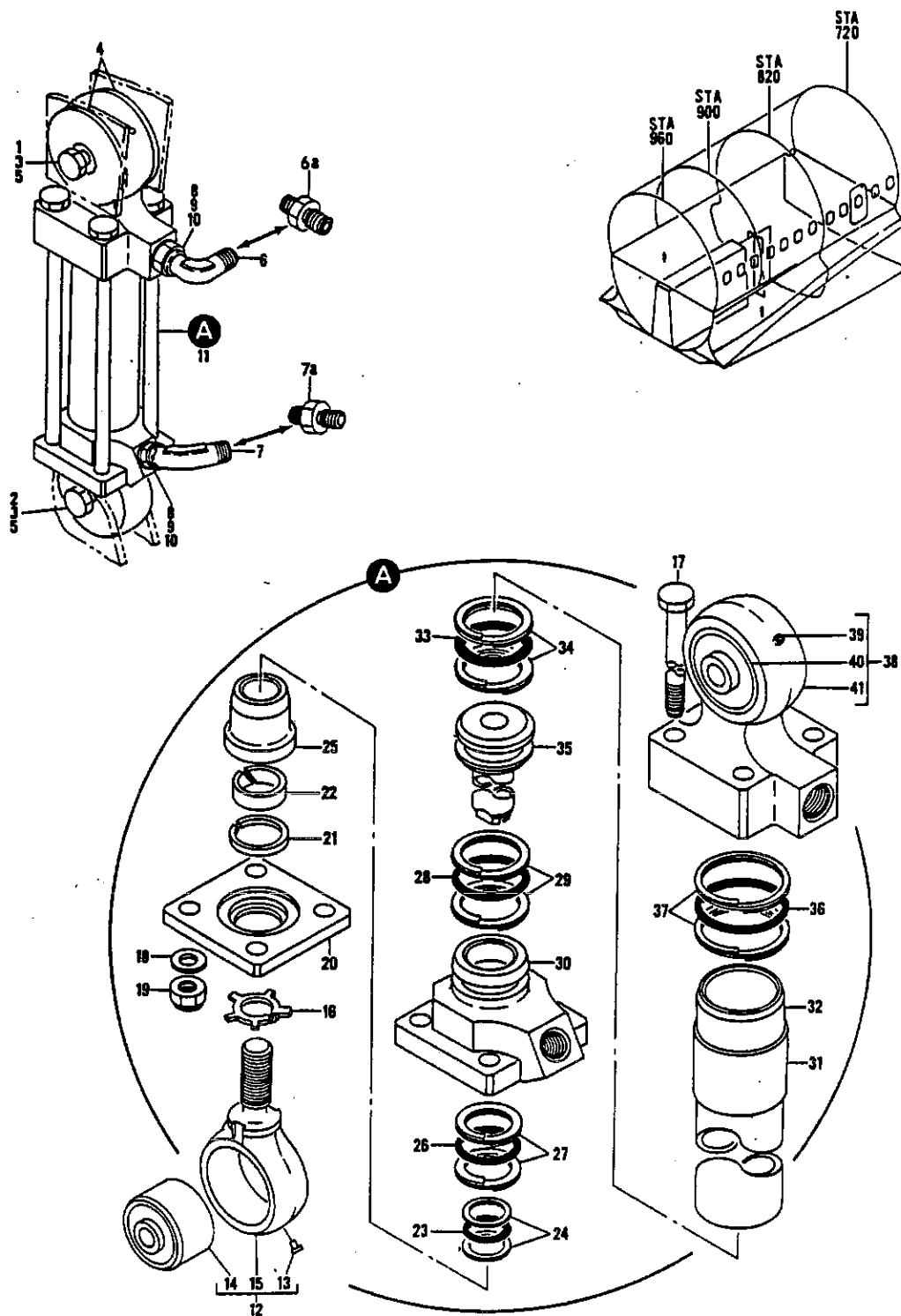
FIGURE 37. ACTUATOR INSTL, MAIN GEAR LOCK
