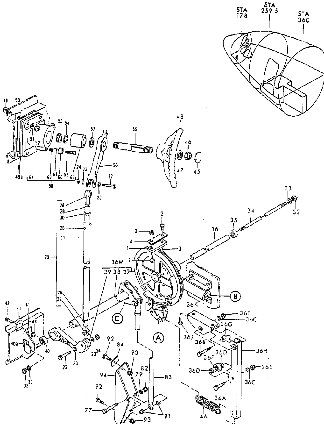
FIGURE 5. WHEEL INSTL, NOSE WHEEL STEERING (LANDING GEAR ONLY) (SHEET 1)
