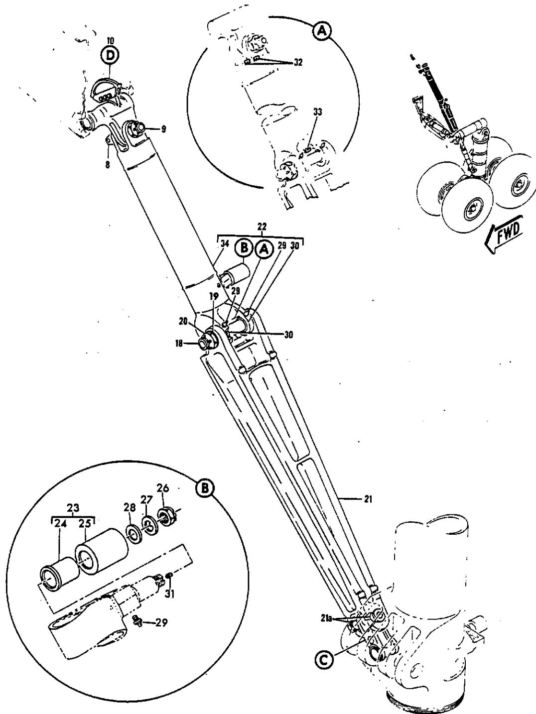
FIGURE 5. STRUT ASSY, SECTION 61 MAIN GEAR SIDE (SHEET 1)
