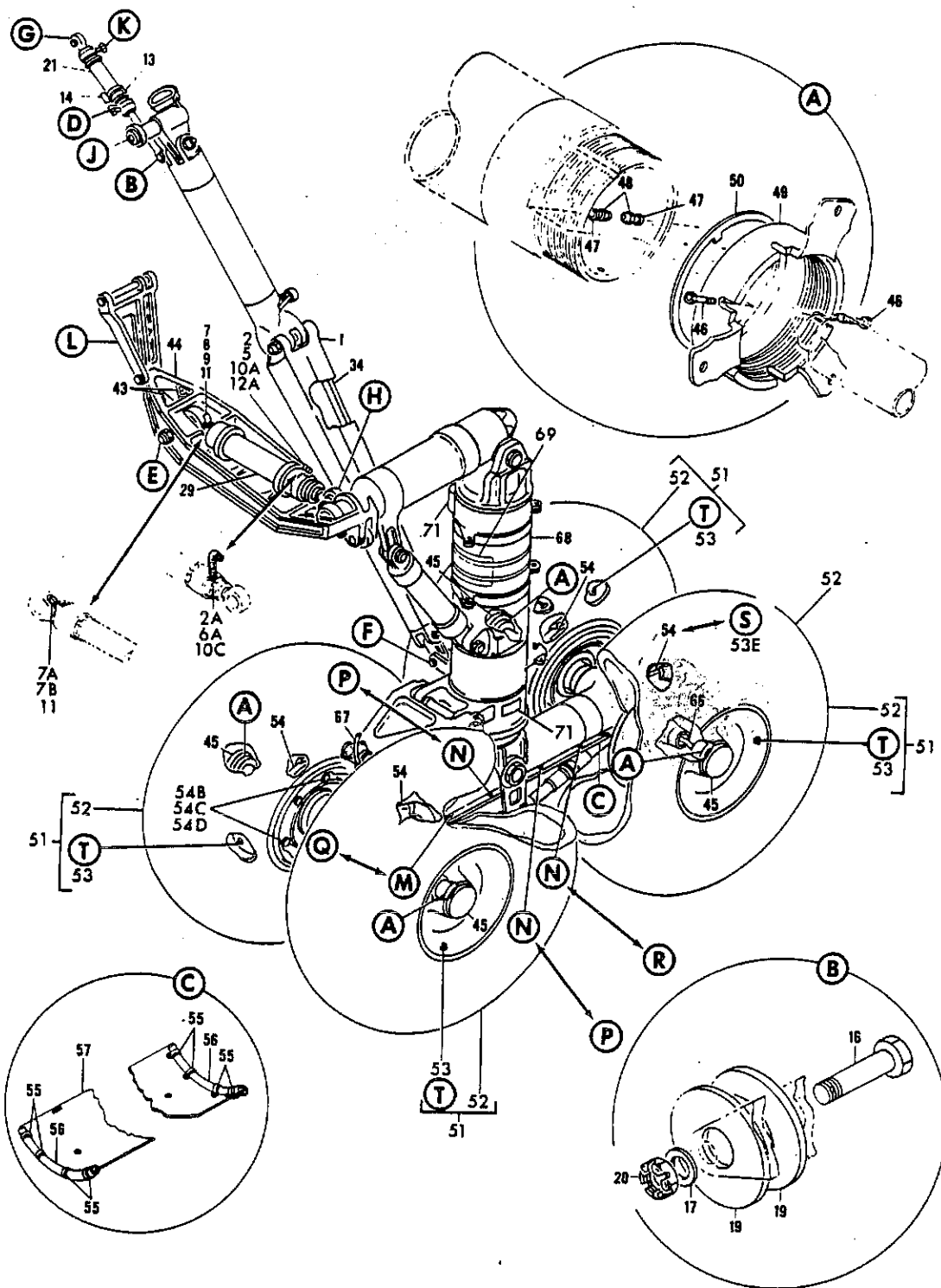
GEAR INSTL, SECTION 61 MAIN LANDING (LH) FIGURE 2. MAIN GEAR, BUILD-UP (LH) (SHEET 1)
