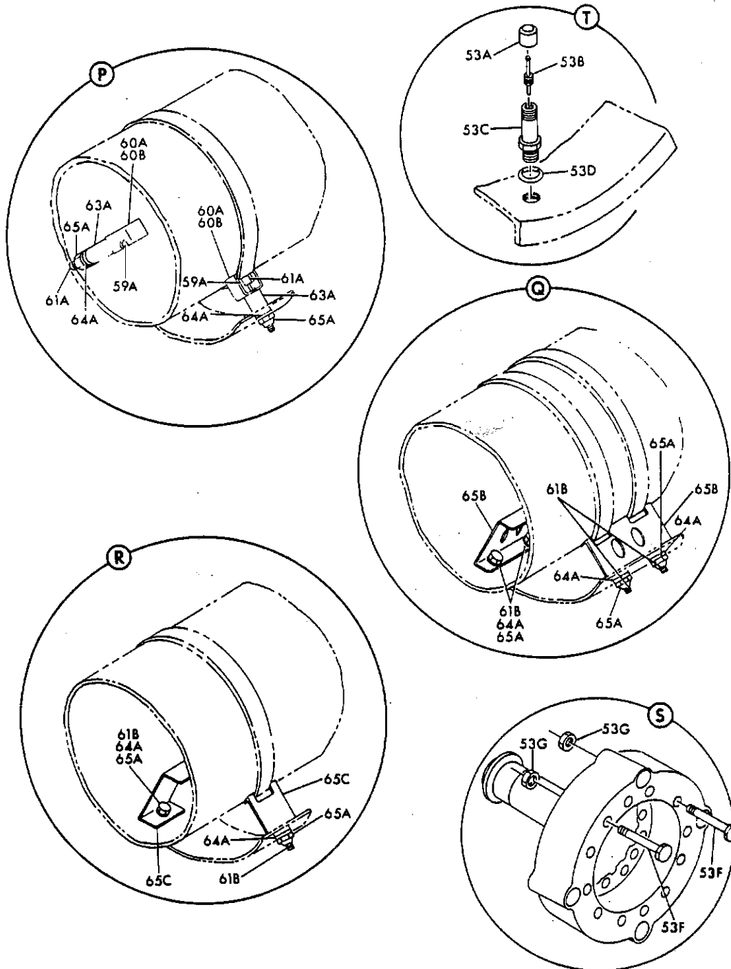
GEAR INSTL, SECTION 61 MAIN LANDING (LH) FIGURE 2. MAIN GEAR, BUILD-UP (LH) (SHEET 4)
