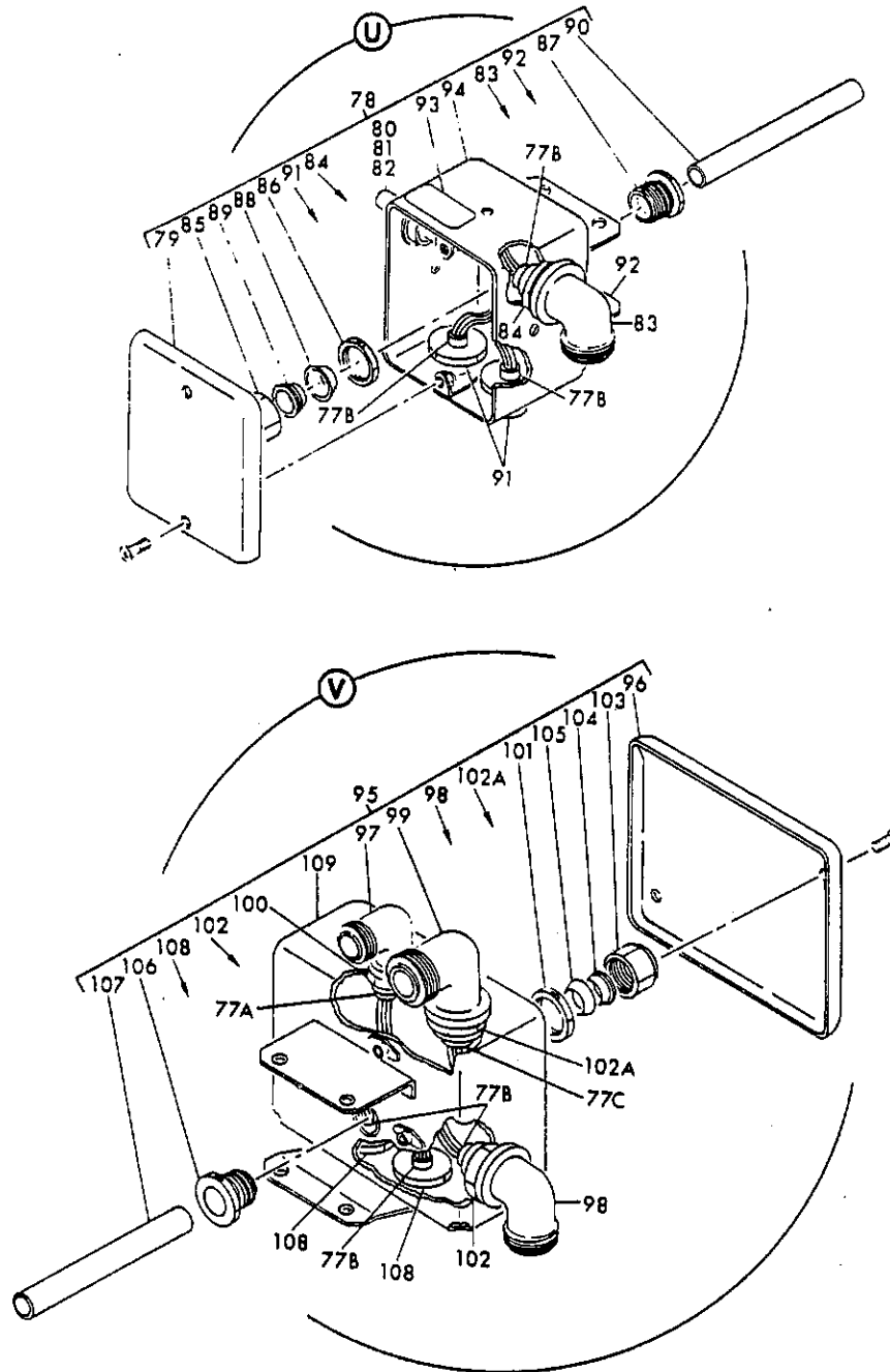
FIGURE 28. ELECTRICAL INSTL, MAIN LANDING GEAR (SHEET 6)
