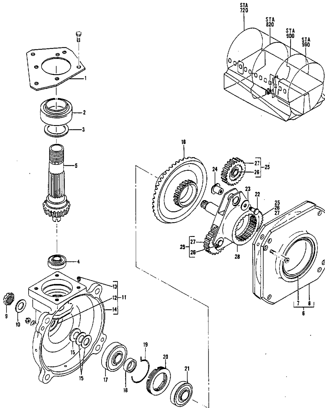
FIGURE 11A. GEAR BOX ASSY, EMERGENCY LANDING GEAR EXTENSION
