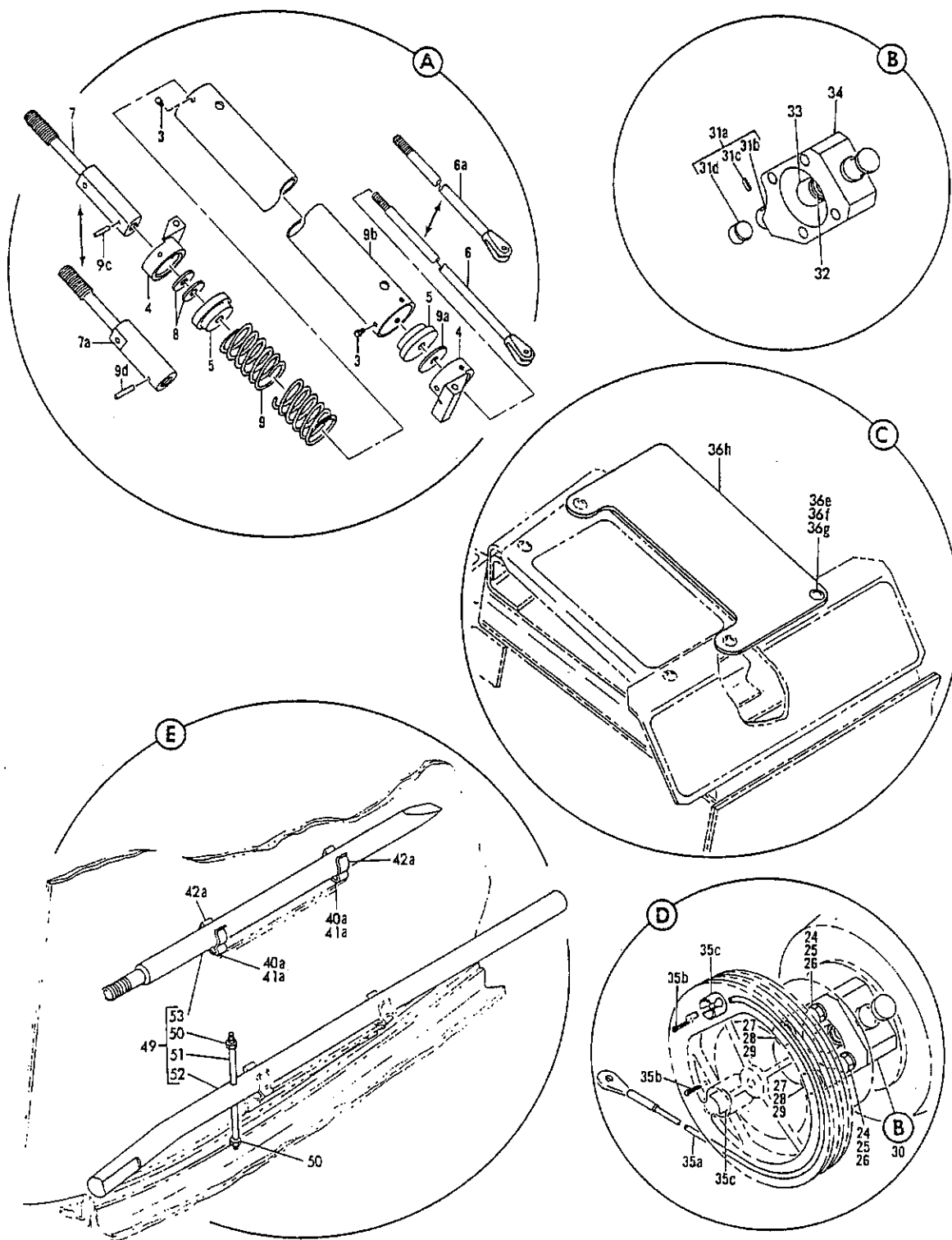
FIGURE 5. DRUM INSTL, EMERGENCY NOSE GEAR EXTENSION RELEASE (LANDING GEAR ONLY) (SHEET 2)
