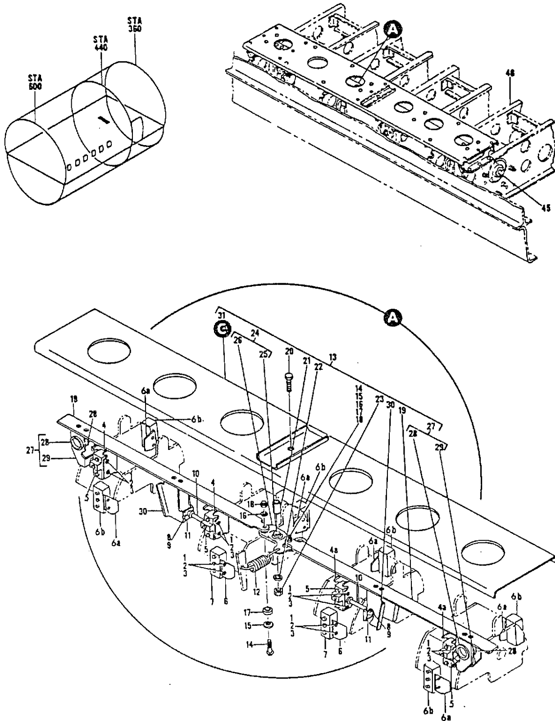
FIGURE 12. SWITCH INSTL, STATION 400 TO 420 THROTTLE OPERATED (SHEET 1)
