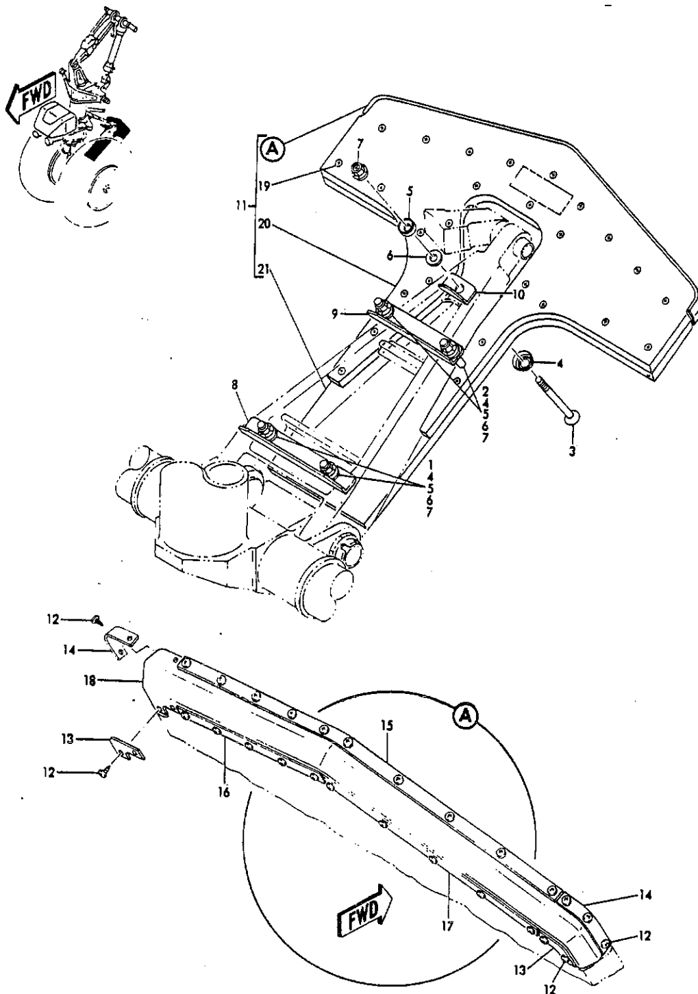
FIGURE 25. DEFLECTOR INSIL, NOSE GEAR AIR (LANDING GEAR ONLY)
