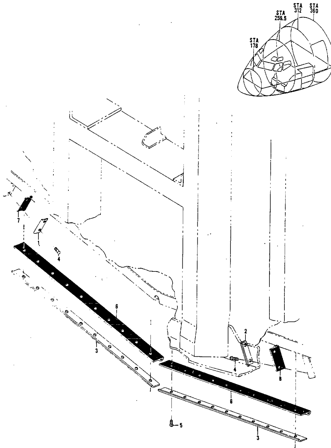
FIGURE 13. SEAL INSTL, NOSE GEAR DOOR
