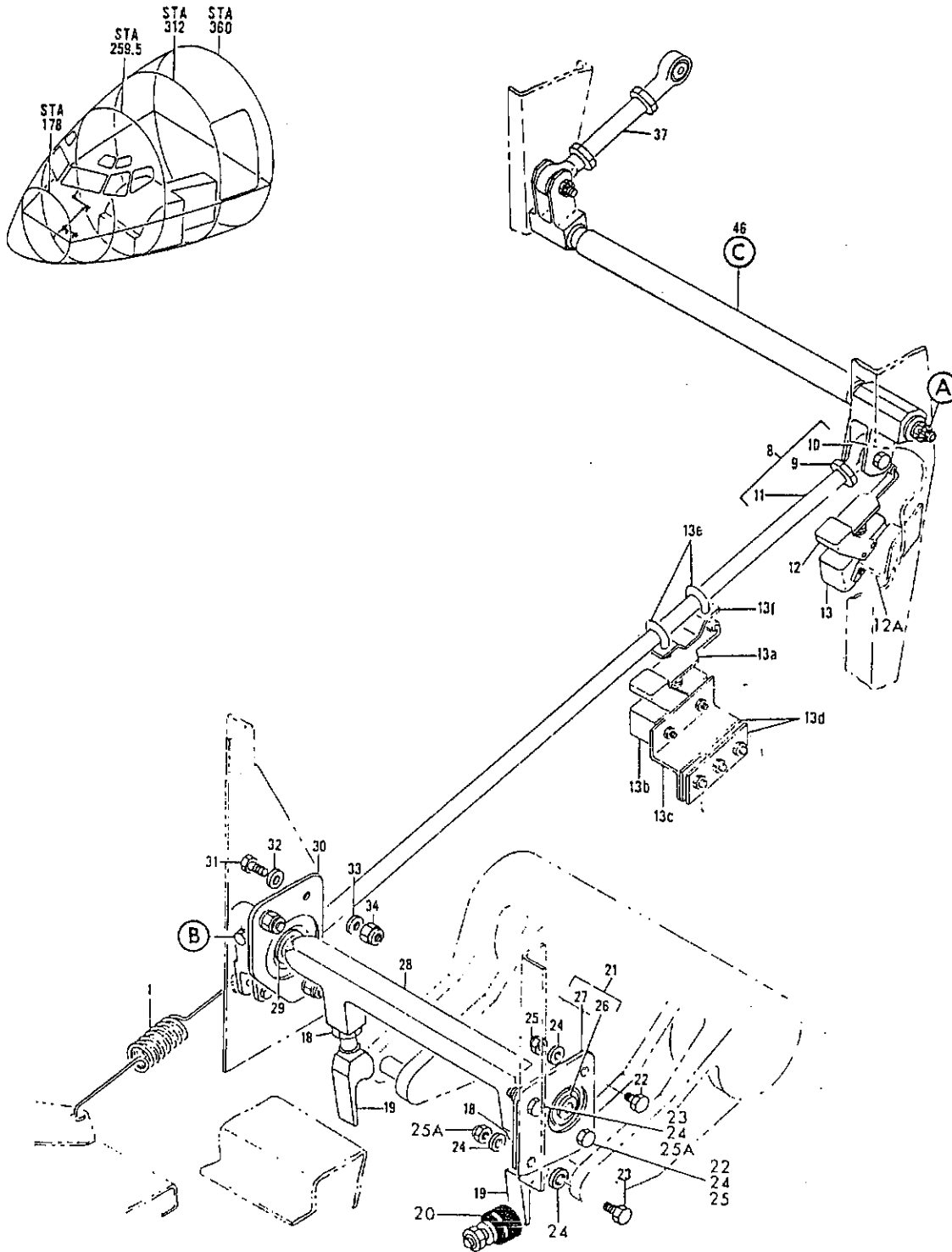
FIGURE 2. MECHANISM INSTL, PARKING BRAKE (SHEET 1)
