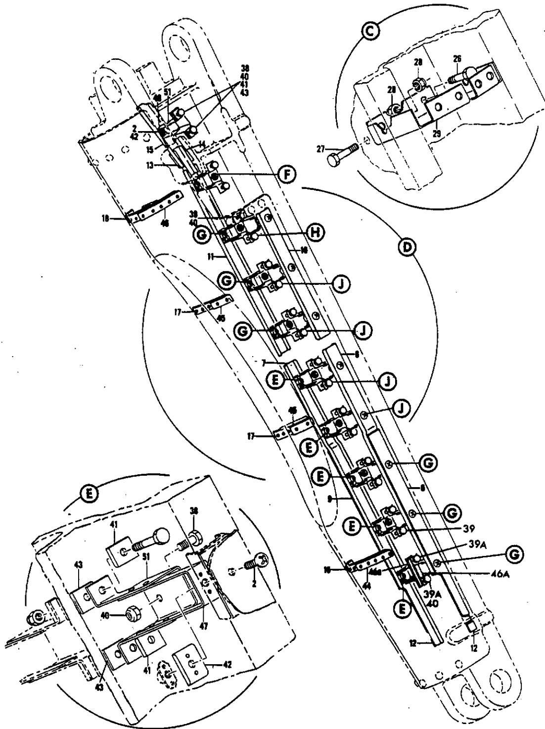
FIGURE 23. FAIRING INSTL, MAIN GEAR SIDE STRUT (SHEET 2)
