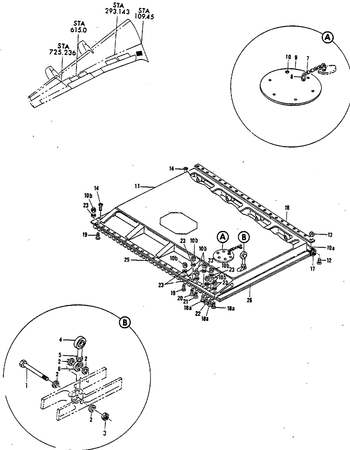
FIGURE 2. DOOR INSTL, LANDING GEAR INBOARD
