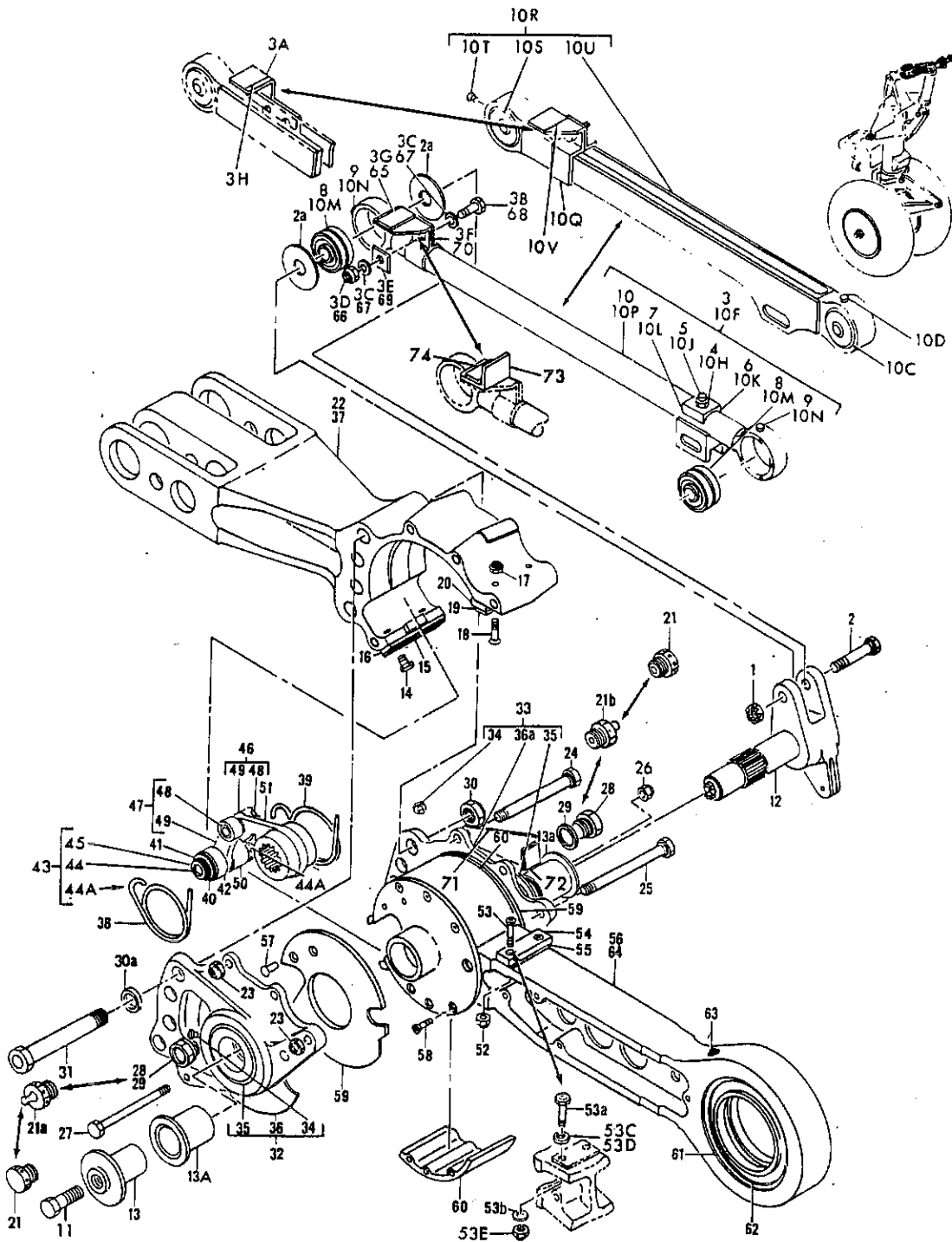
FIGURE 2D. BRACE ASSY., NOSE GEAR DRAG
