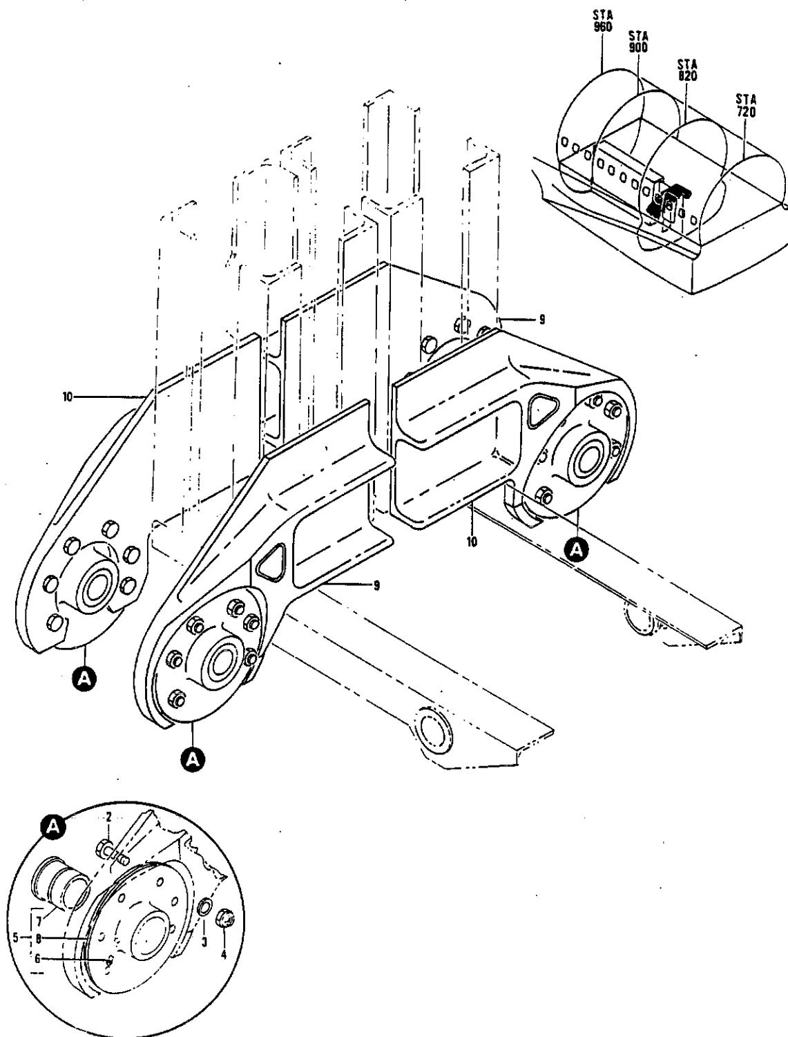
FIGURE 16. SUPPORT INSTL, MAIN GEAR DOOR ACTUATOR
