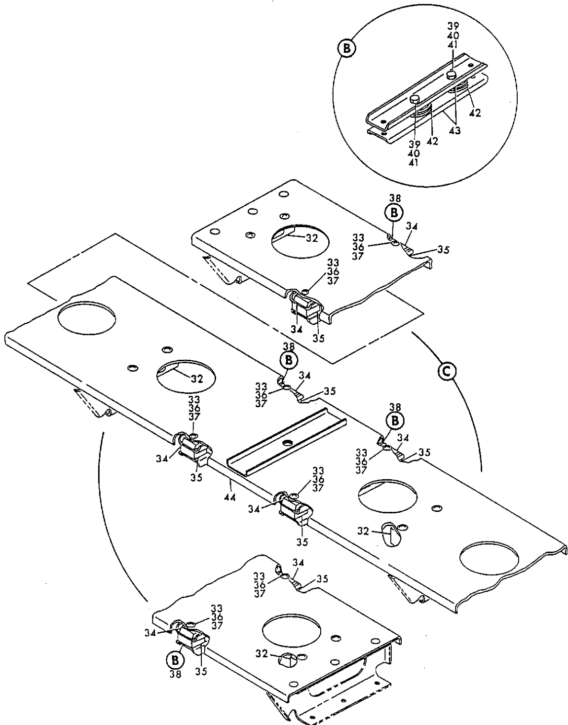
FIGURE 12. SWITCH INSTL, STATION 400 TO 420 THROTTLE OPERATED (SHEET 2)
