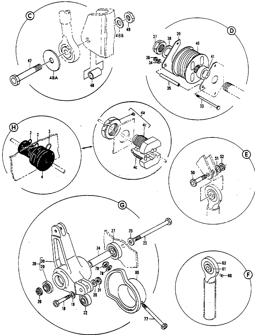
FIGURE 11. RELEASE INSTL, MAIN GEAR EMERGENCY (SHEET 2)
