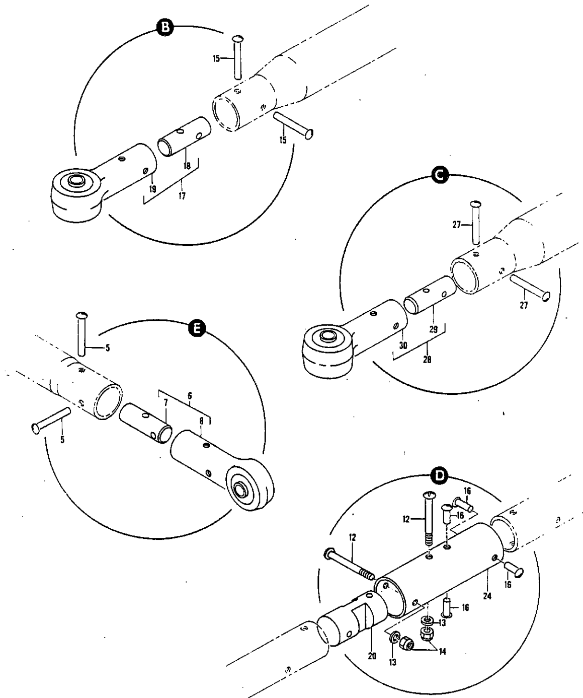
FIGURE 3. BRACKET INSTL, BRAKE PEDAL BUSS (SHEET 2)
