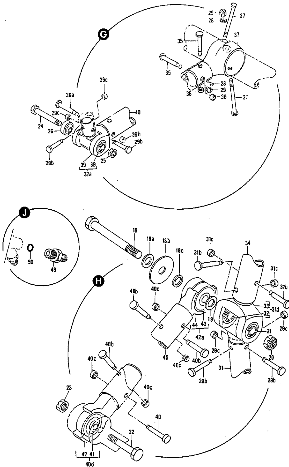
FIGURE 22. MECHANISM INSTL, MAIN GEAR DOOR (SHEET 21)
