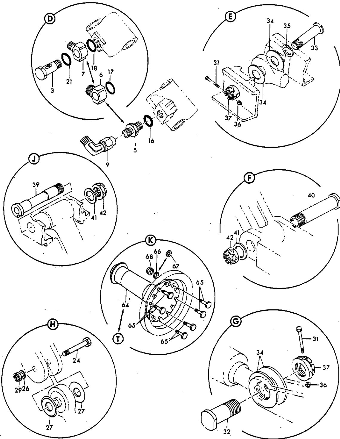
FIGURE 2B. GEAR INSTL. SECTION 61 MAIN LANDING (RH) MAIN GEAR, BUILD-UP (RH) (SHEET 2)
