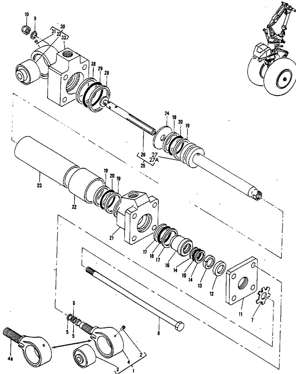
FIGURE 2A. ACTUATOR ASSY, NOSE GEAR LOCK
