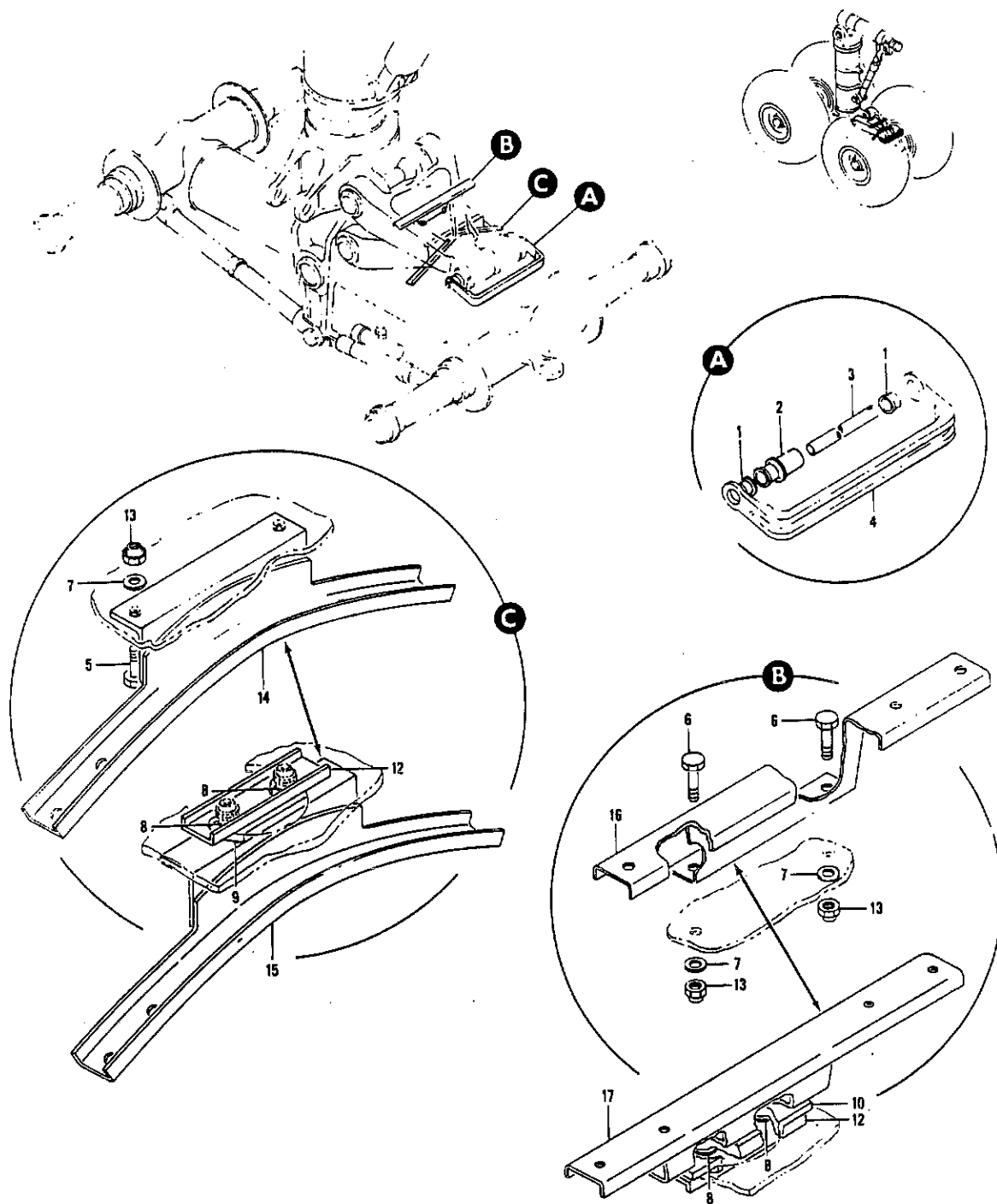
FIGURE 25. SWIVEL INSTL, MAIN LANDING GEAR TORSION LINK
