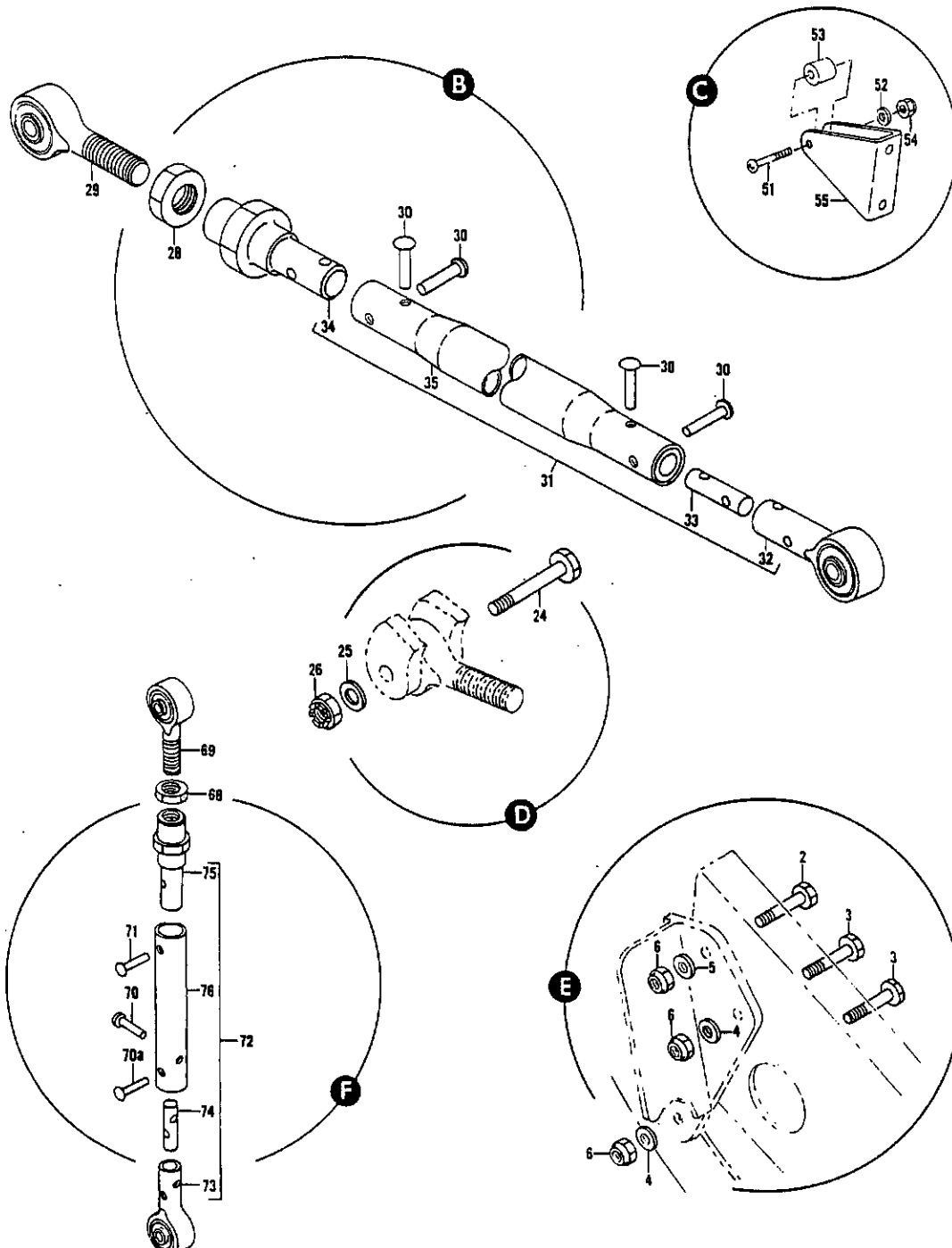
FIGURE 4. CONTROL INSTL, GROUND DOOR RELEASE (SHEET 2)
