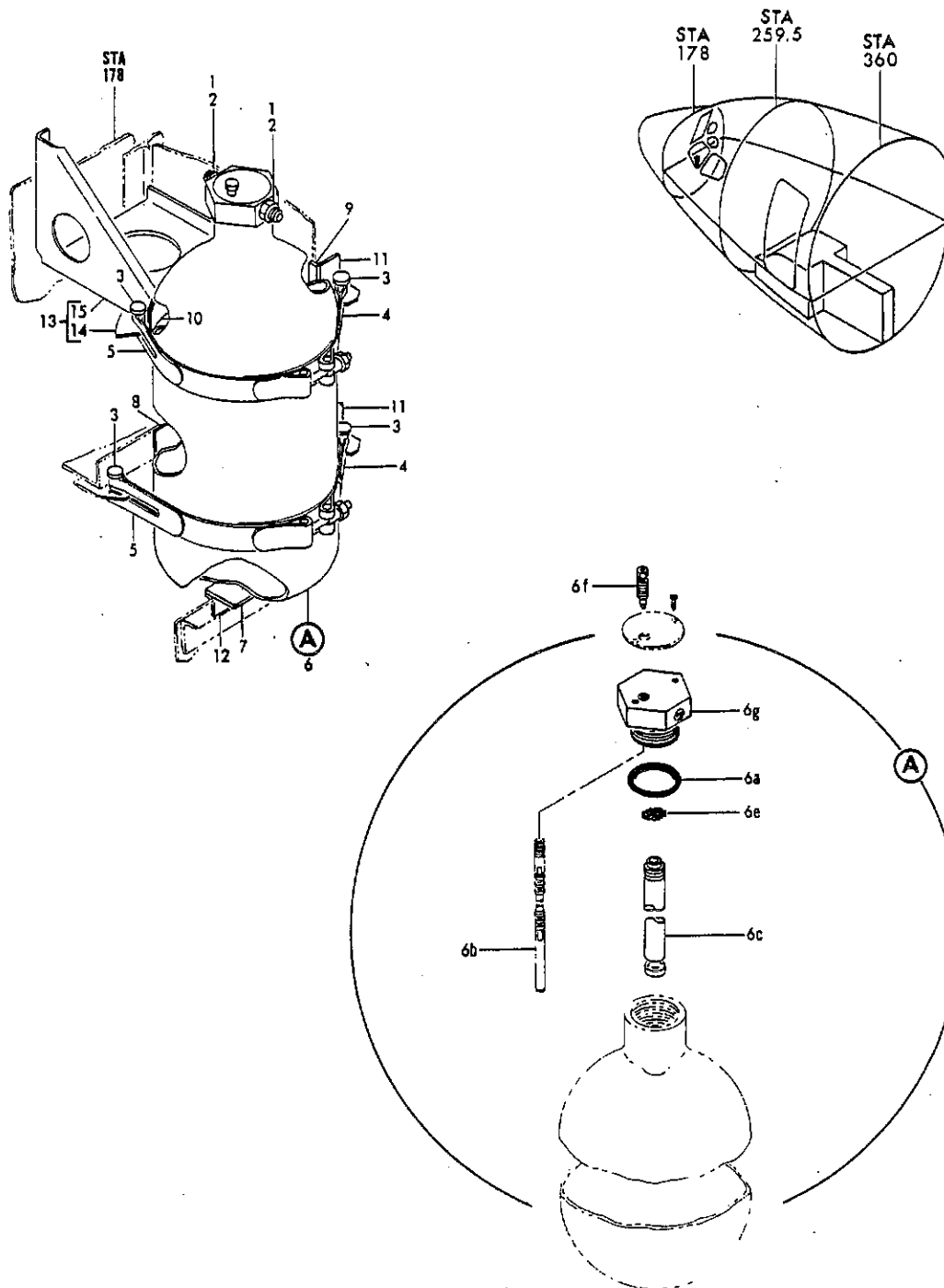
FIGURE 13. BOTTLE INSTL, PNEUMATIC EMERGENCY BRAKE
