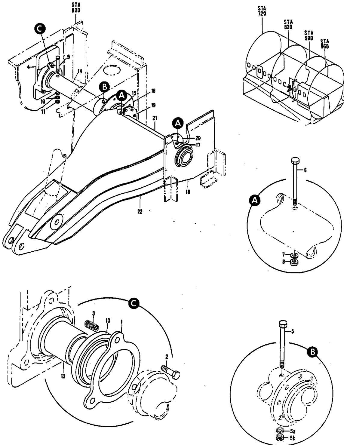
FIGURE 23. BEAM INSTL, MAIN GEAR DOOR WALKING
