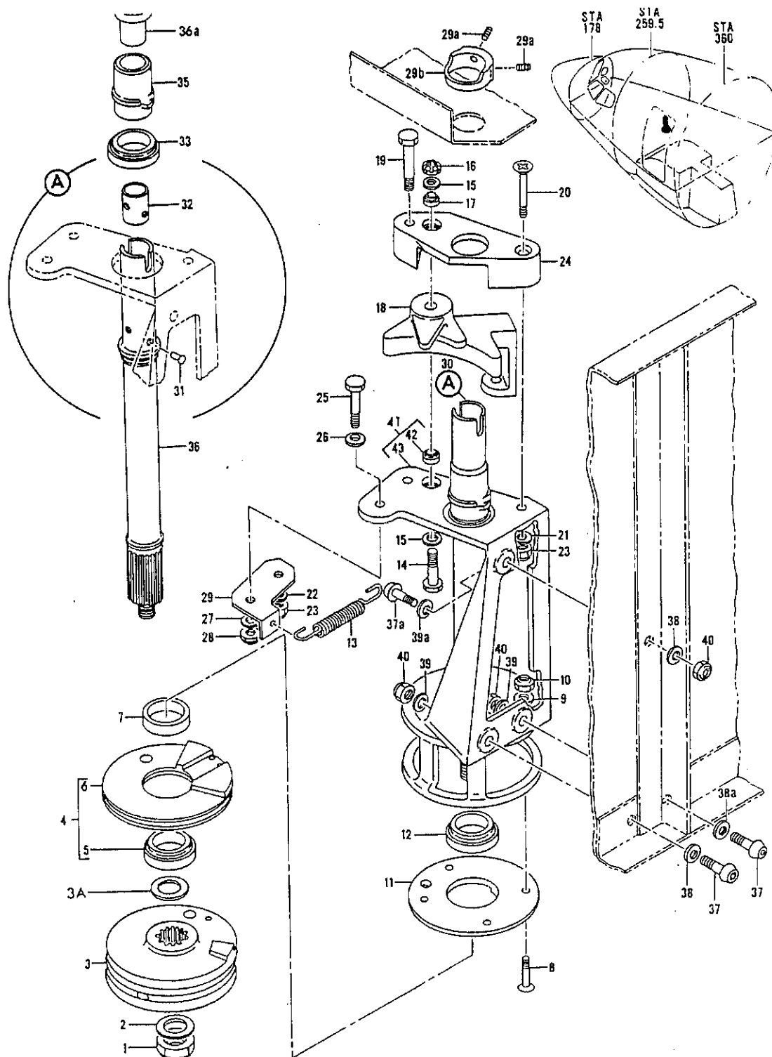
FIGURE 4. DRUM INSTL, STATION 277.0 EMERGENCY NOSE GEAR EXTENSION HANDCRANK
