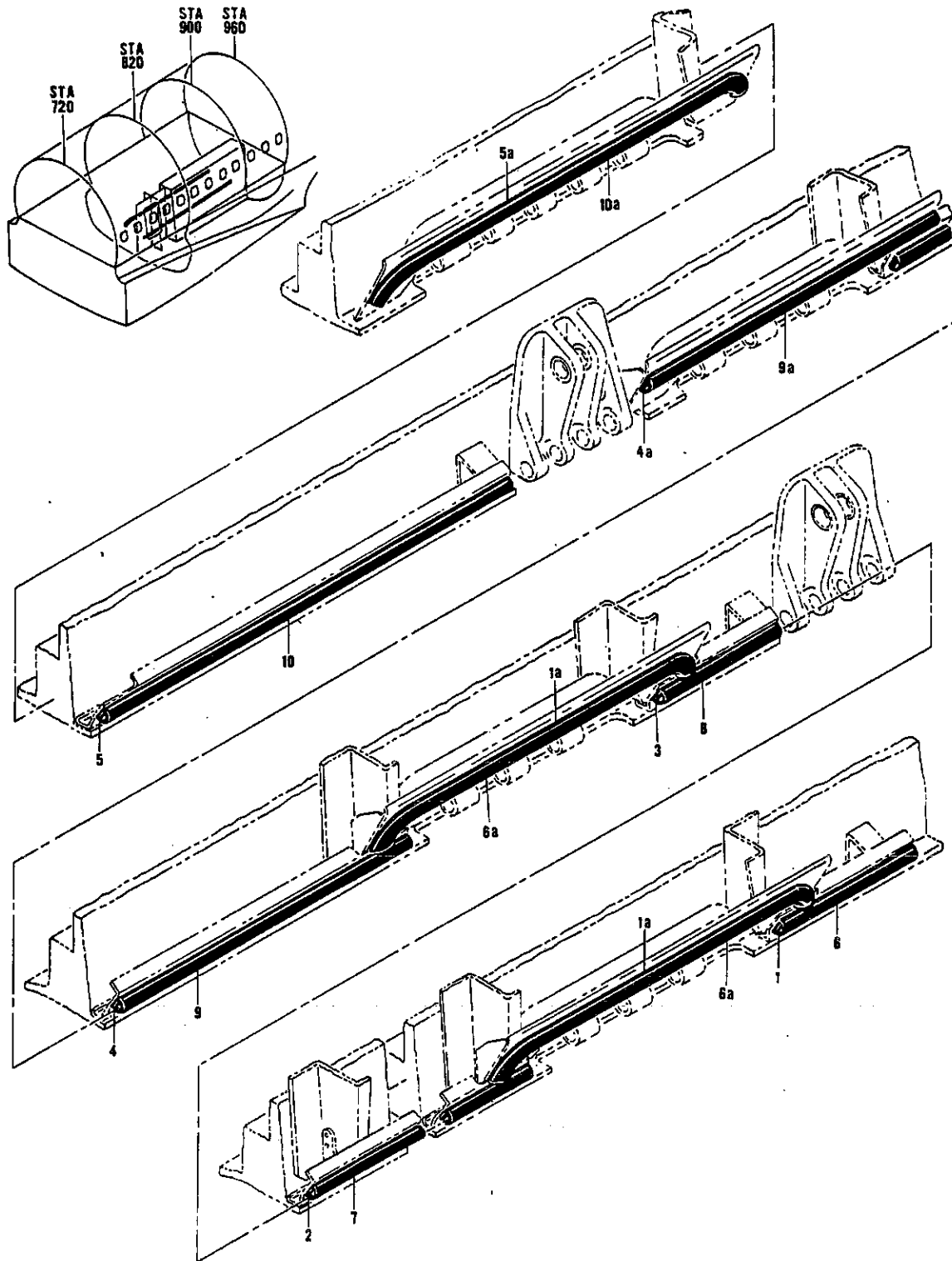
FIGURE 13. SEAL INSTL, MAIN GEAR DOOR
