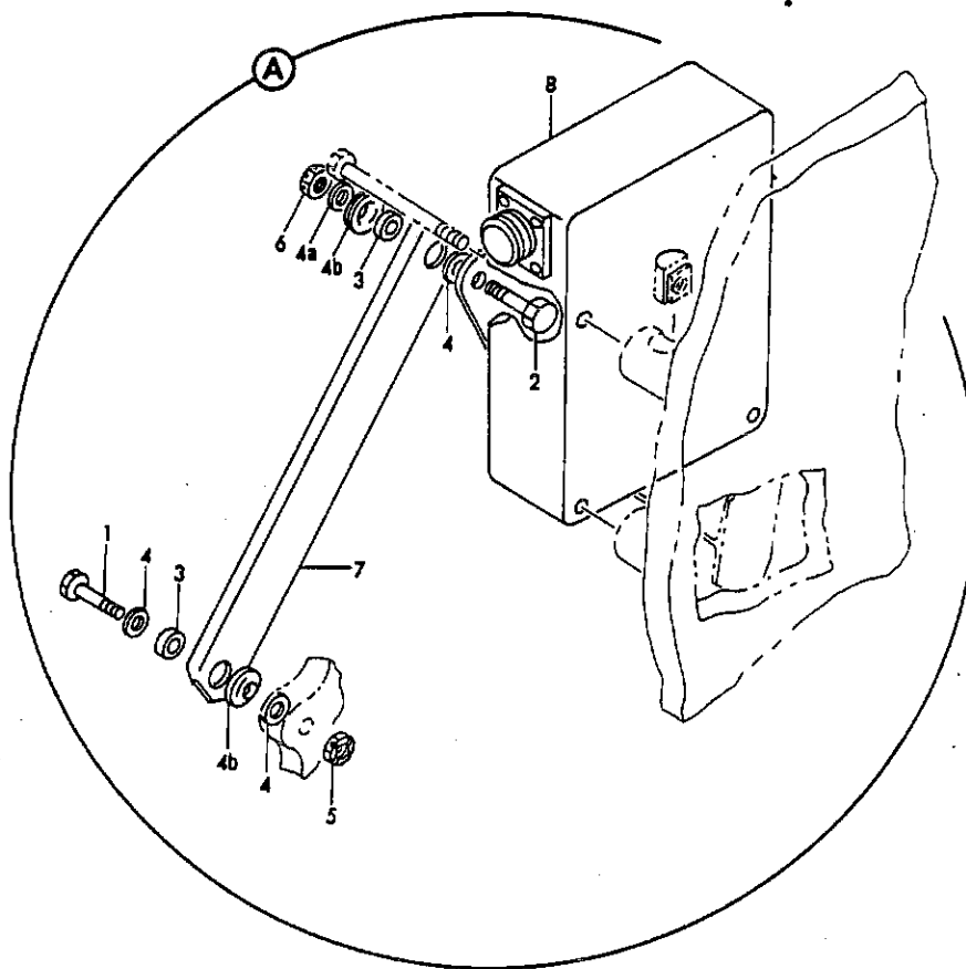
FIGURE 32. SWITCH INSTL, MAIN LANDING GEAR TRUCK CENTERING
