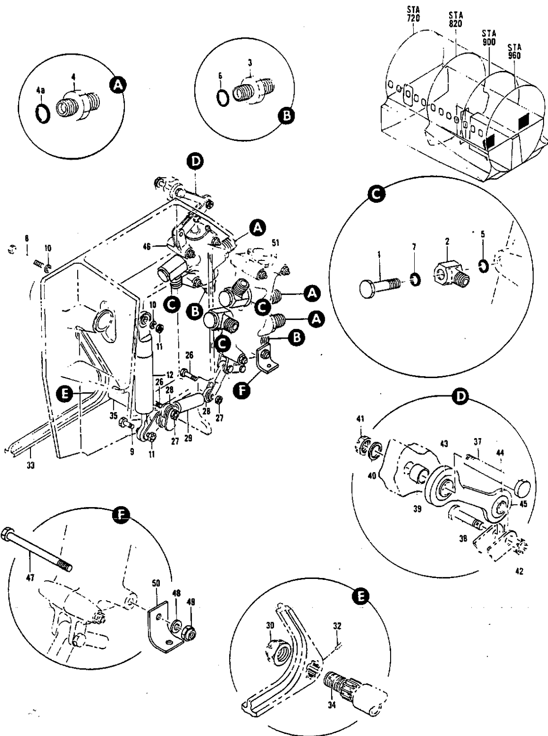
FIGURE 24. VALVE INSTL, MAIN GEAR DOOR CONTROL
