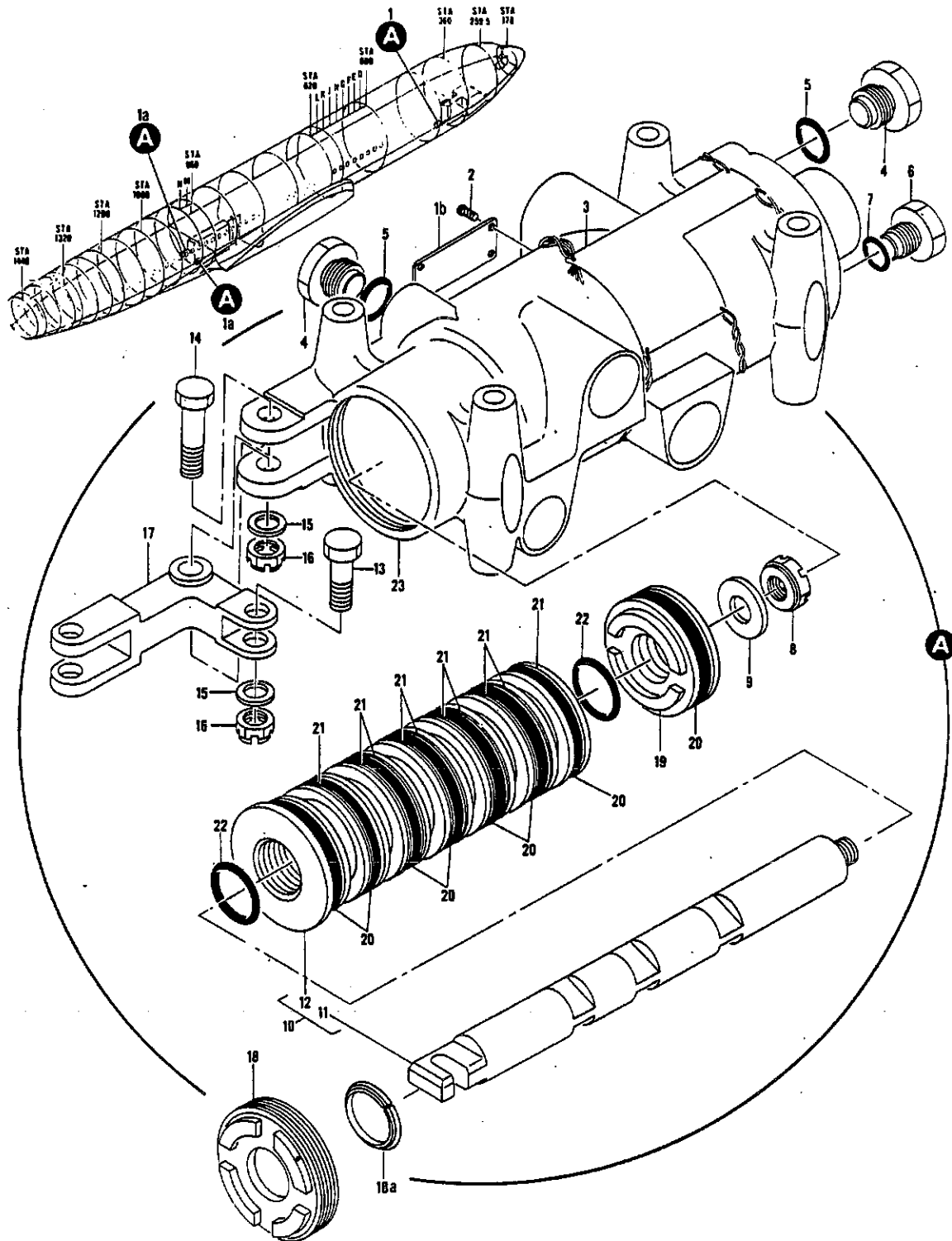
FIGURE 25, VALVE ASSY, LANDING GEAR DOOR CONTROL
