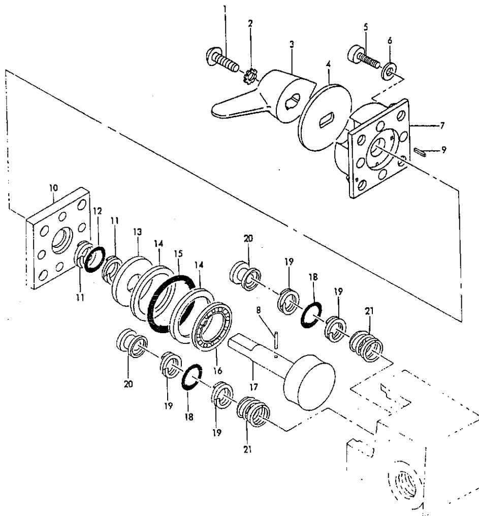
FIGURE 30. VALVE ASSY, MANUALLY OPERATED ROTARY SHUTOFF
