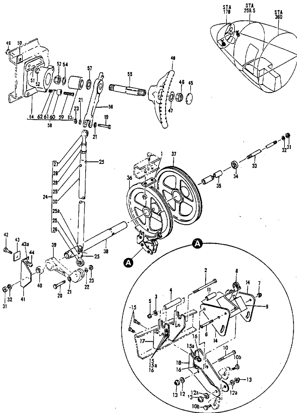
FIGURE 6. WHEEL INSTL, NOSE WHEEL STEERING (LANDING GEAR ONLY)
