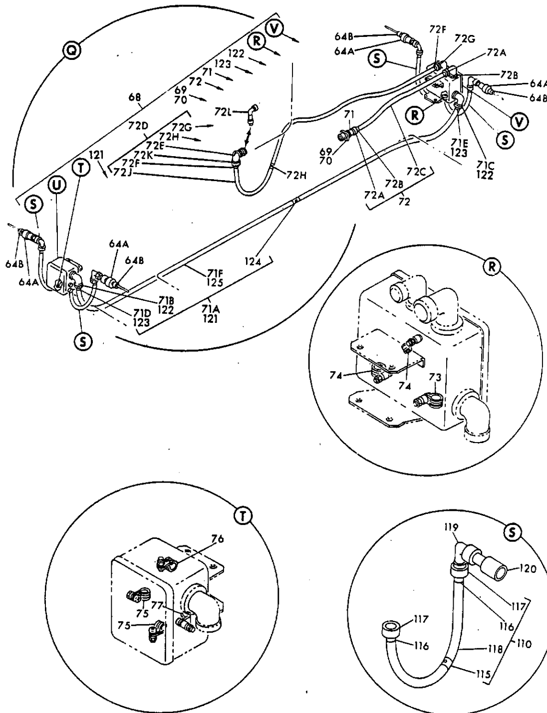
FIGURE 28. ELECTRICAL INSTL, MAIN LANDING GEAR (SHEET 5)
