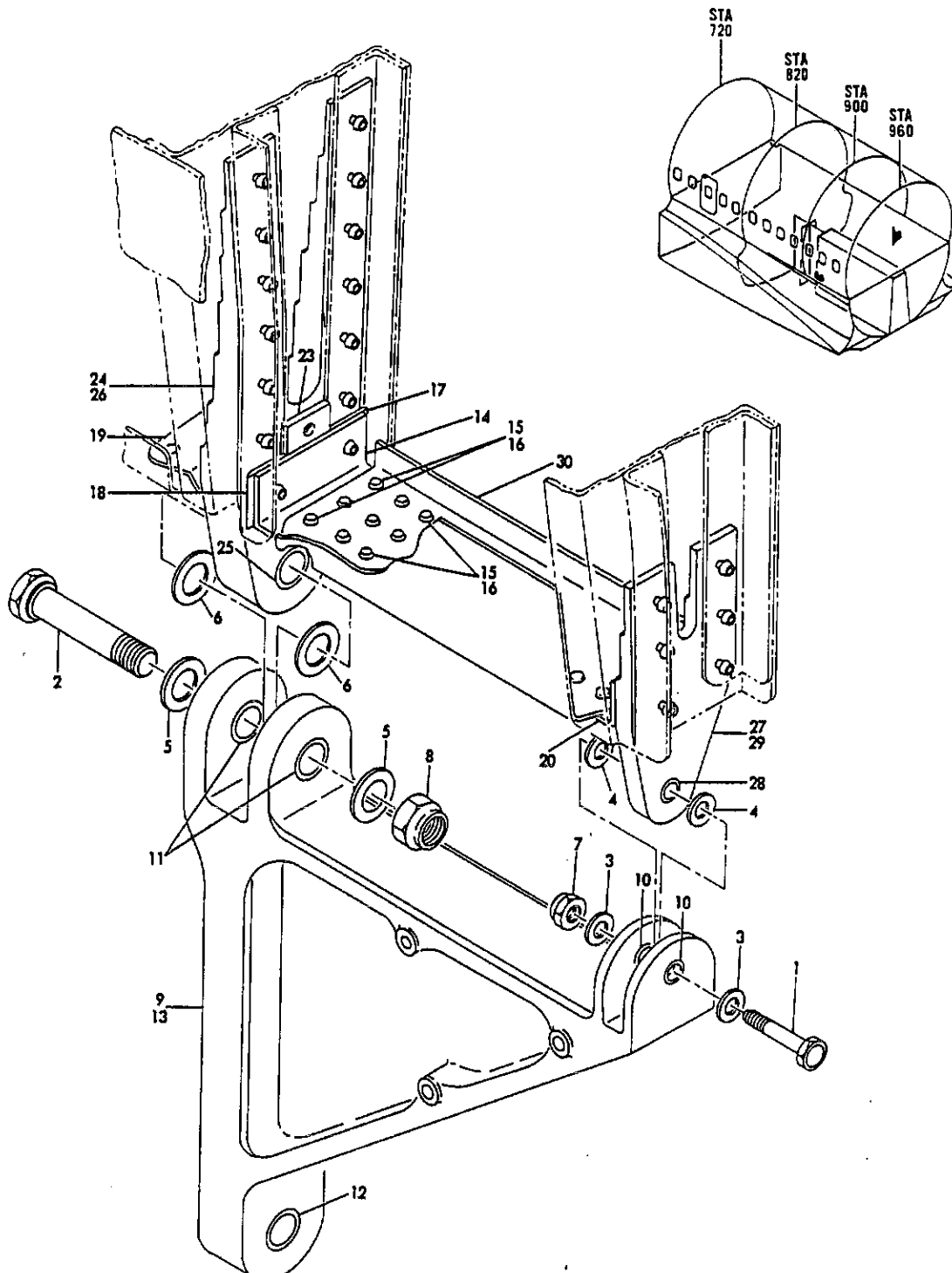
FIGURE 40A. SUPPORT INSIL, STATION 900 TO 910 UPLOCK
