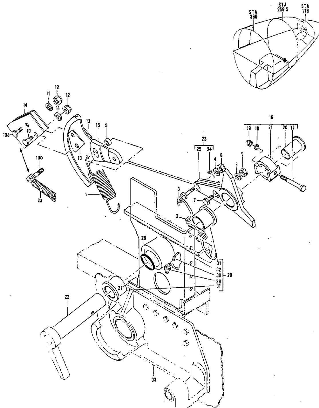
FIGURE 10. RELEASE INSTL, NOSE GEAR DOOR
