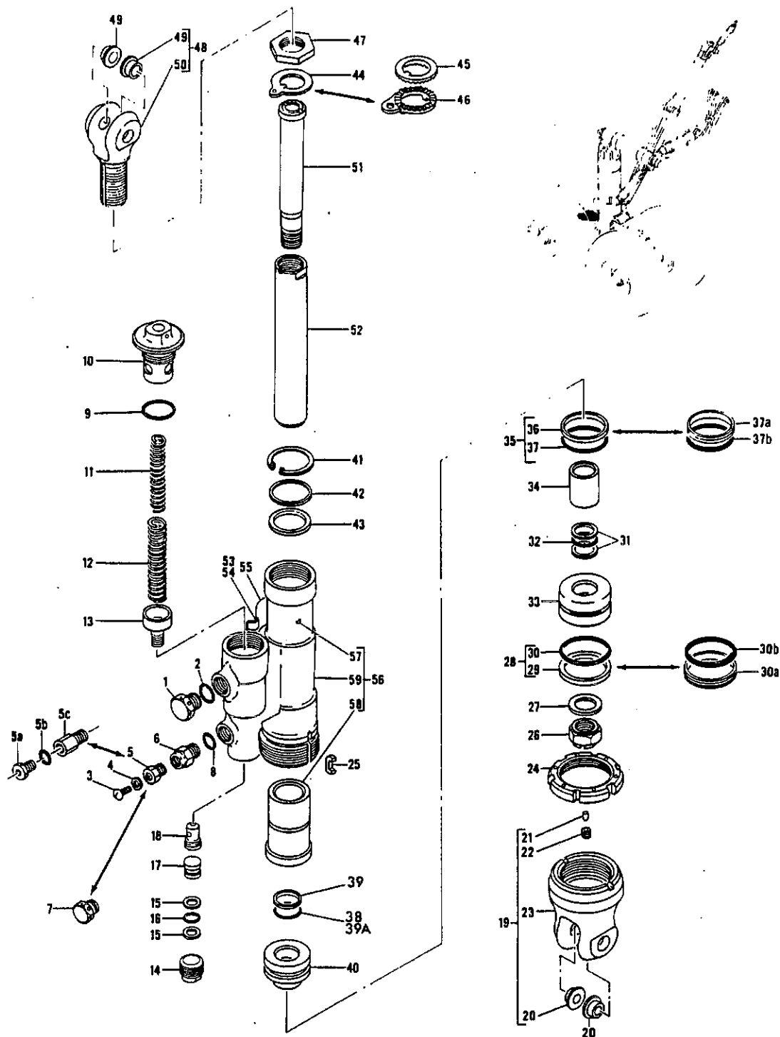
FIGURE 26C. CENTERING CYLINDER AND SNUBBER ASSY, (MAIN GEAR)
