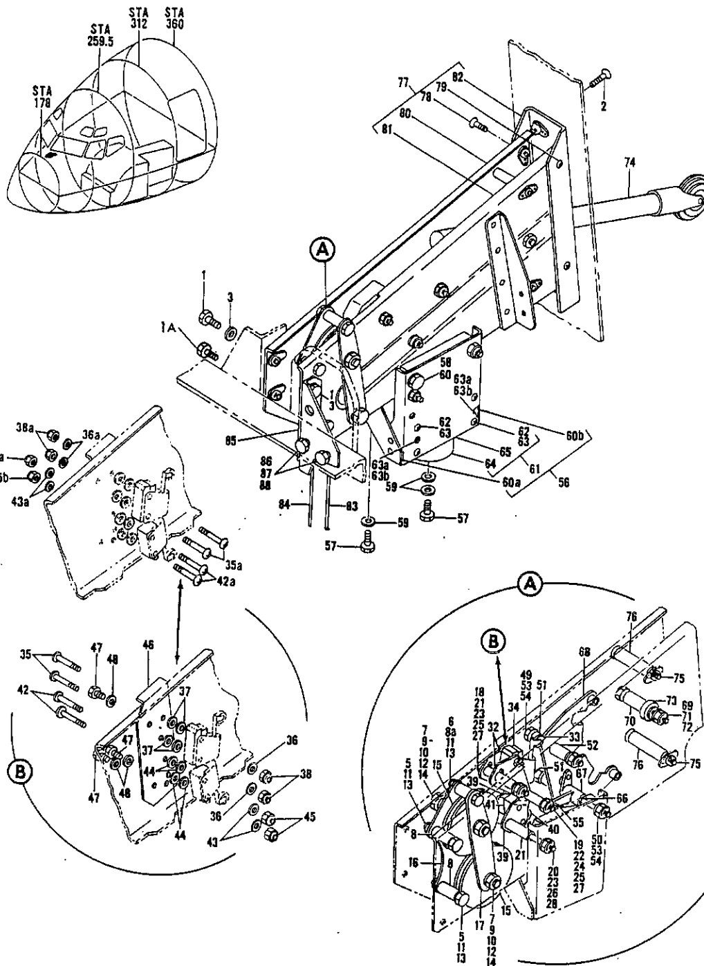
FIGURE 2. LEVER INSTL, LANDING GEAR CONTROL
