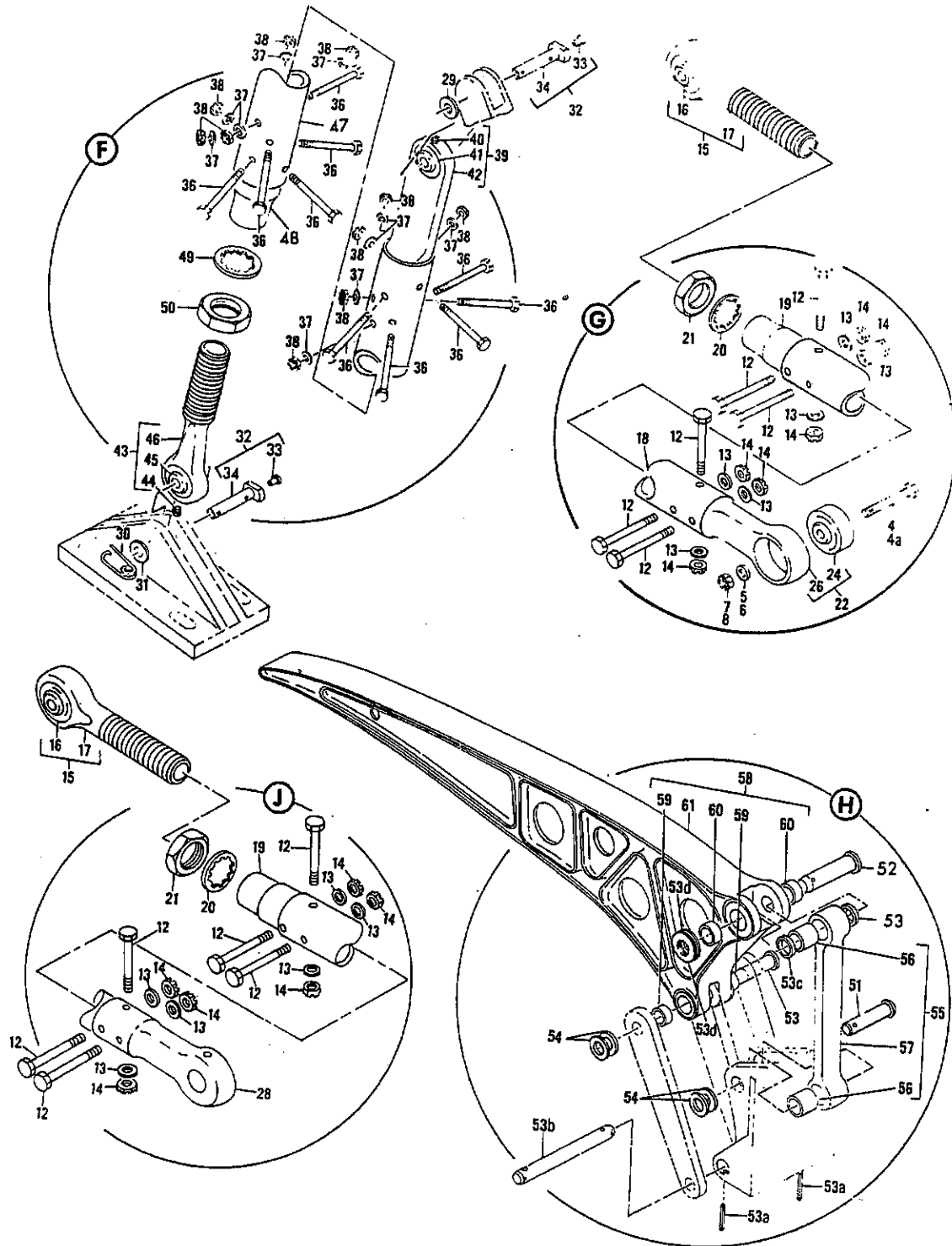
FIGURE 10. DOOR INSTL, MAIN GEAR (SHEET 2)
