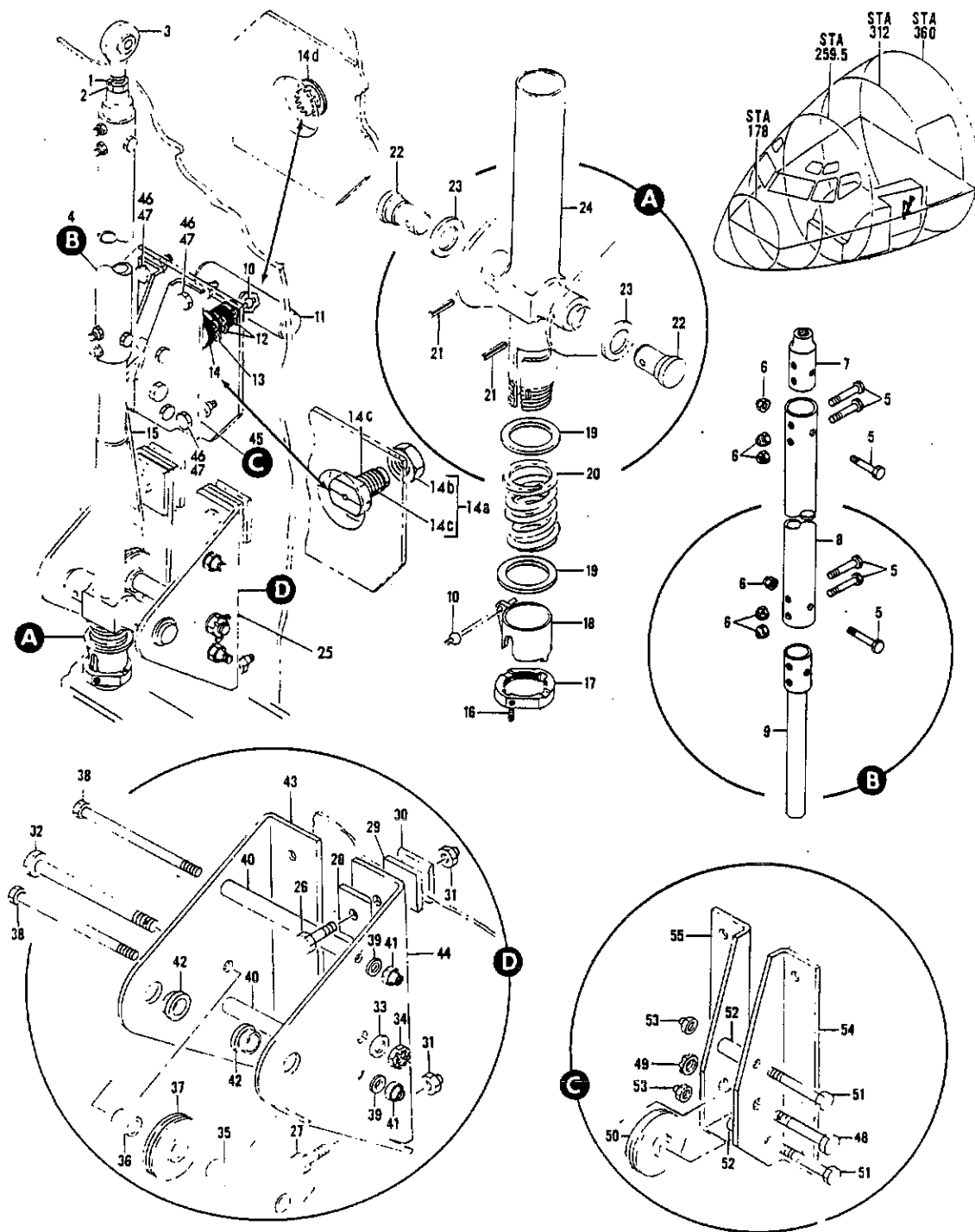
FIGURE 18. LOCK INSTL, NOSE GEAR GROUND
