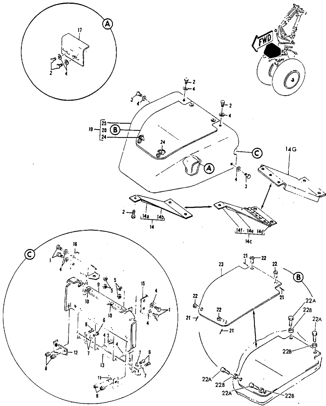
FIGURE 15. LANDING GEAR, NOSE LANDING GEAR
