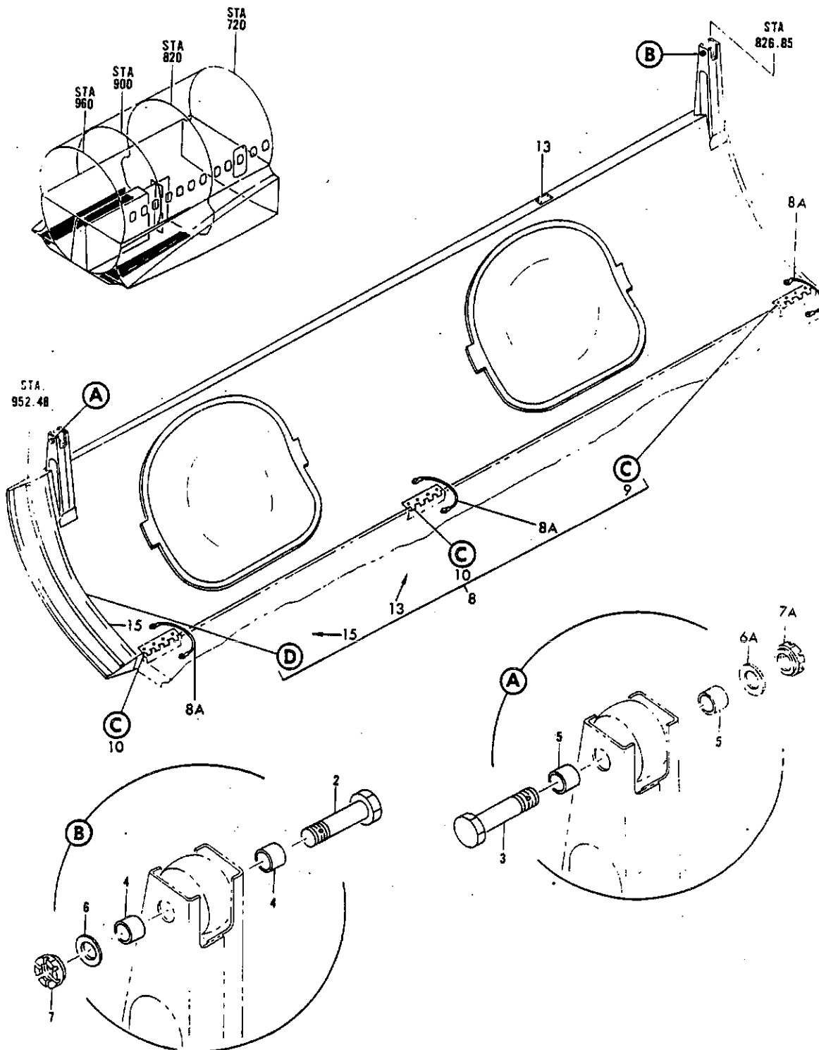
FIGURE 12. DOOR INSTL, MAIN GEAR OUTBOARD (SHEET 1)
