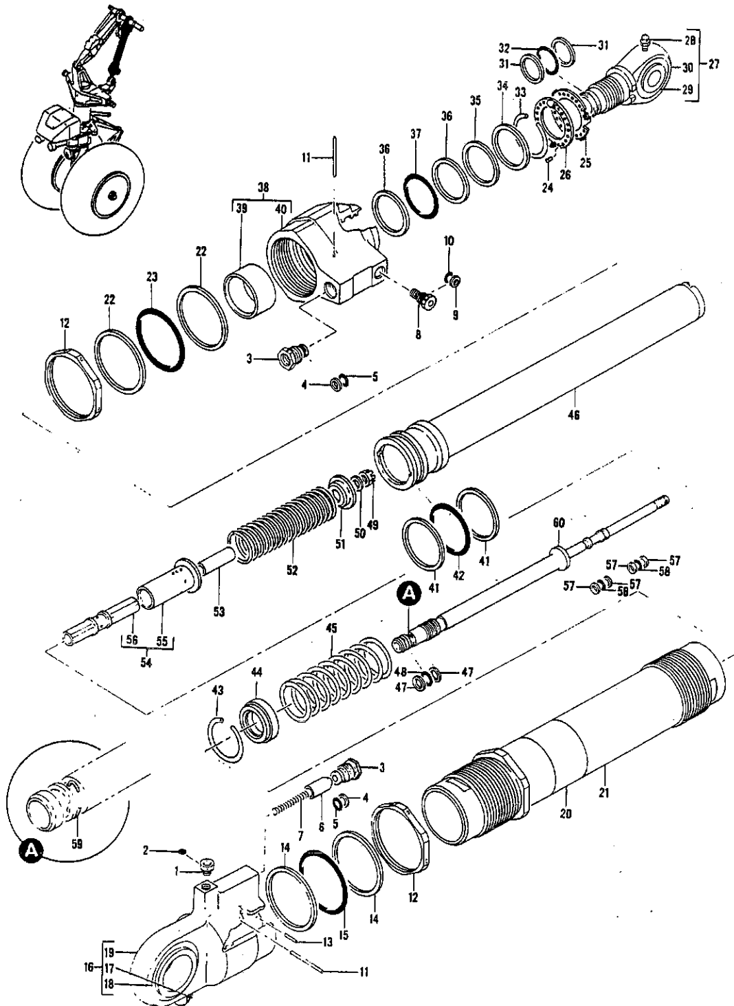
FIGURE 2C. ACTUATOR ASSY, NOSE GEAR HYDRAULIC
