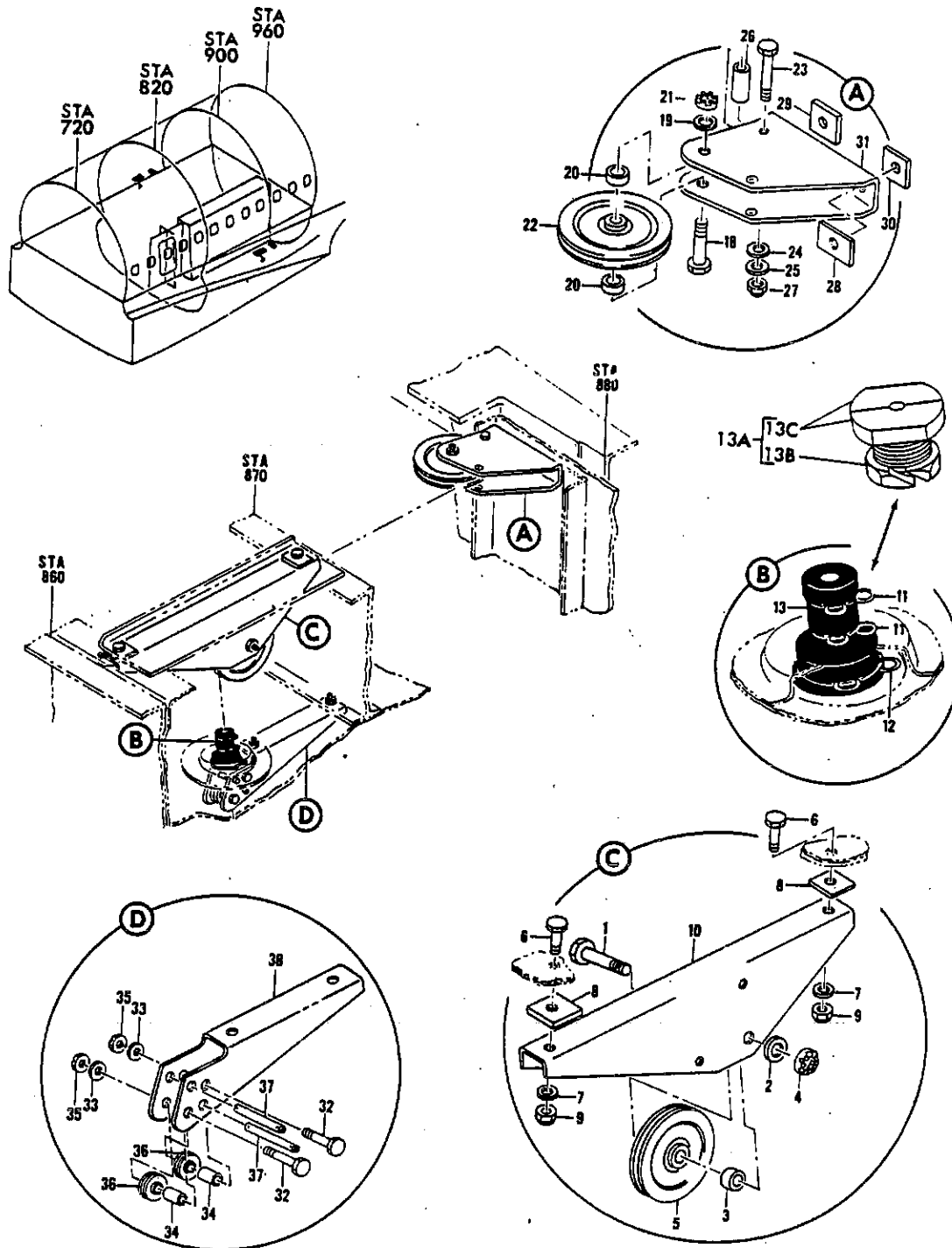
FIGURE 21. BRACKET INSTL, MAIN WHEEL WELL GROUND DOOR RELEASE
