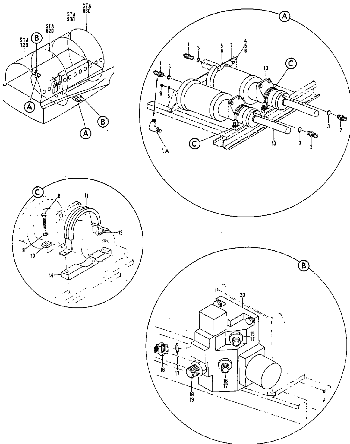
FIGURE 12. VALVE INSTI BRAKE DEBOOST AND ANTI-SKID
