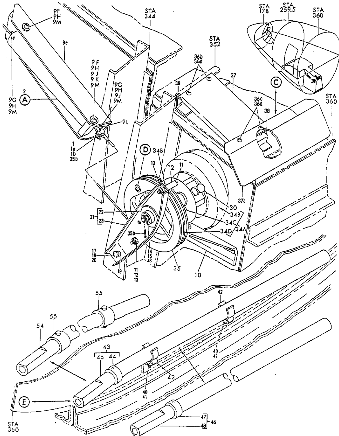
FIGURE 5. DRUM INSTL, EMERGENCY NOSE GEAR EXTENSION RELEASE (LANDING GEAR ONLY) (SHEET 1)
