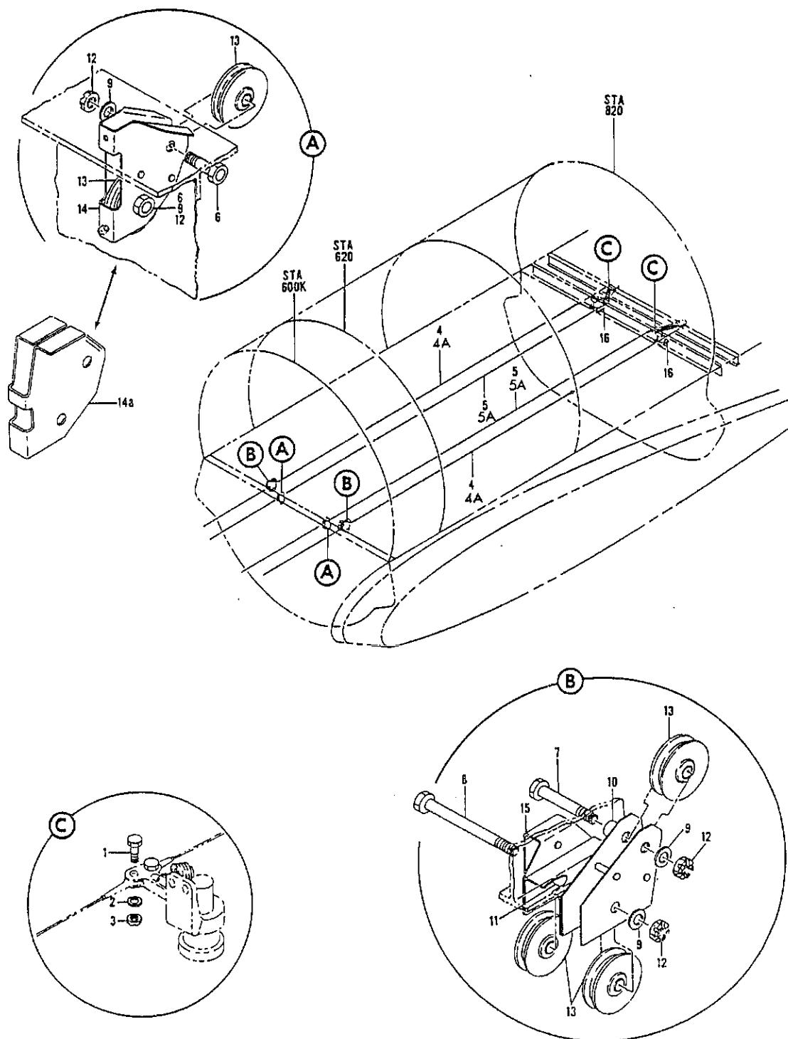
FIGURE 5. CONTROL INSTL, LANDING GEAR BRAKE
