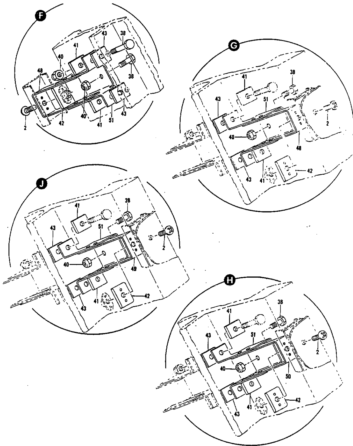
FIGURE 23 FAIRING INSTL, MAIN GEAR SIDE STRUT (SHEET 3)
