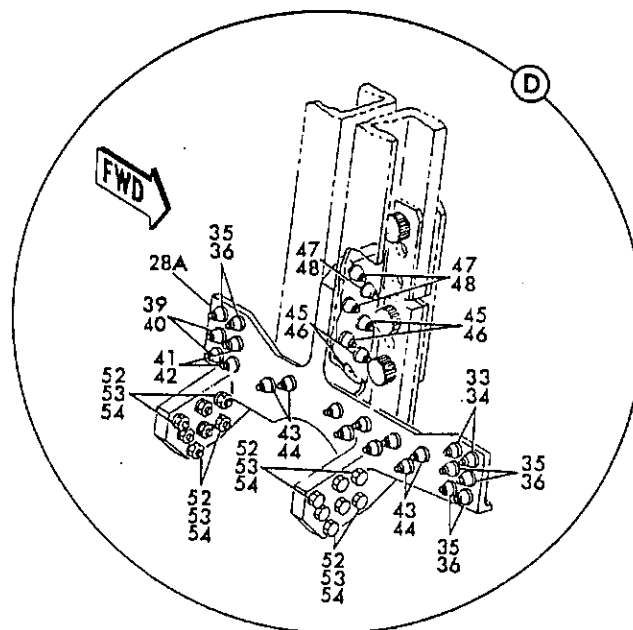
FIGURE 23. PANEL INSTL, STATION 312 TO 360 NOSE GEAR WHEEL WELL SIDE (SHEET 2)
