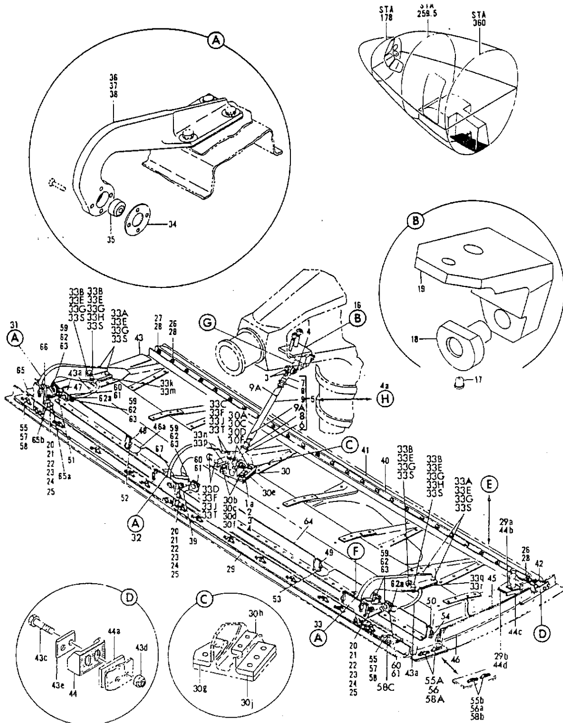
FIGURE 3 DOOR AND FAIRING INSTL, STATION 310 TO 360 NOSE WHEEL WELL (SHEET 1)
