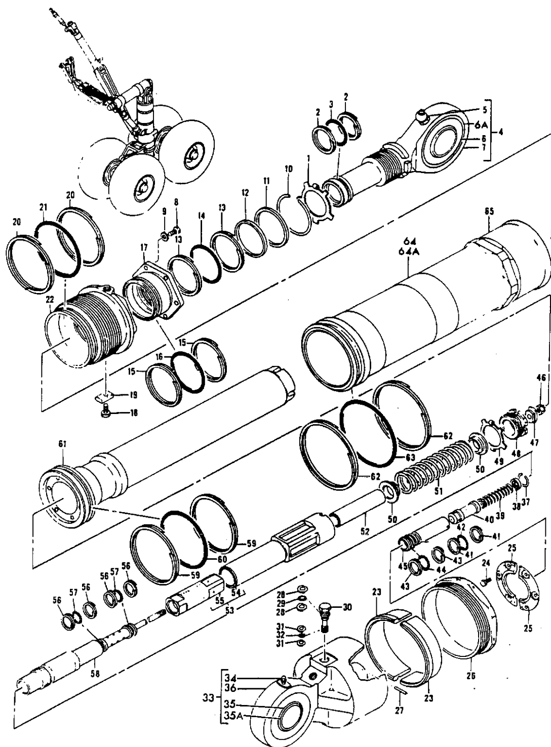
FIGURE 5A. ACTUATOR ASSY, MAIN LANDING GEAR
