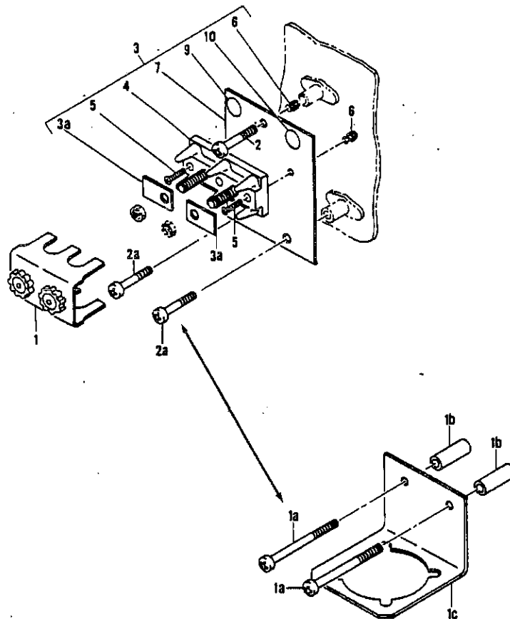
FIGURE 17. STRIP INSTL. PILOTS AND COPILOTS OXYGEN REGULATOR TERMINAL
