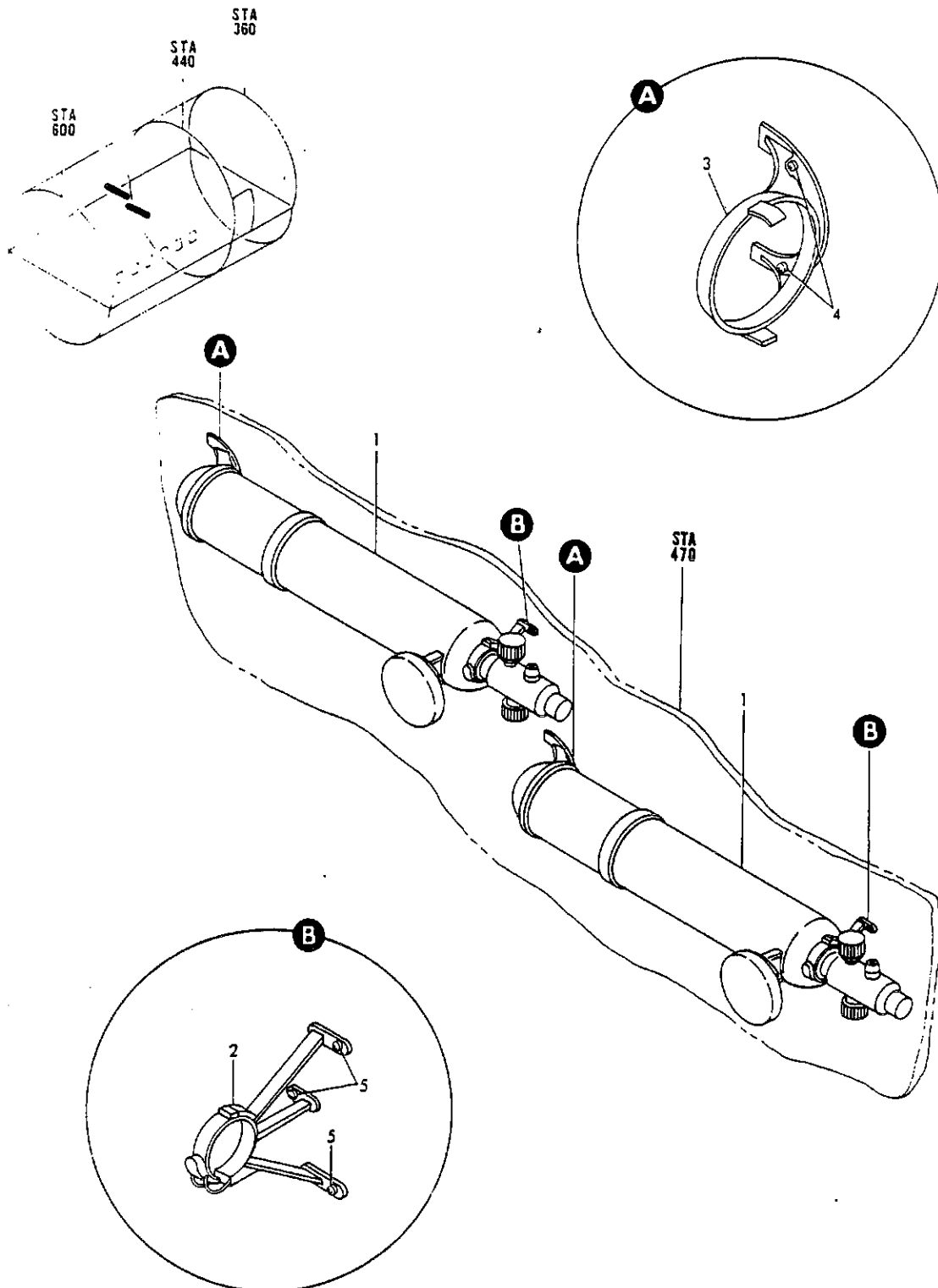
FIGURE 37D. OXYGEN BOTTLE AND FIRST AID KIT INSTL. (OXYGEN ONLY)
