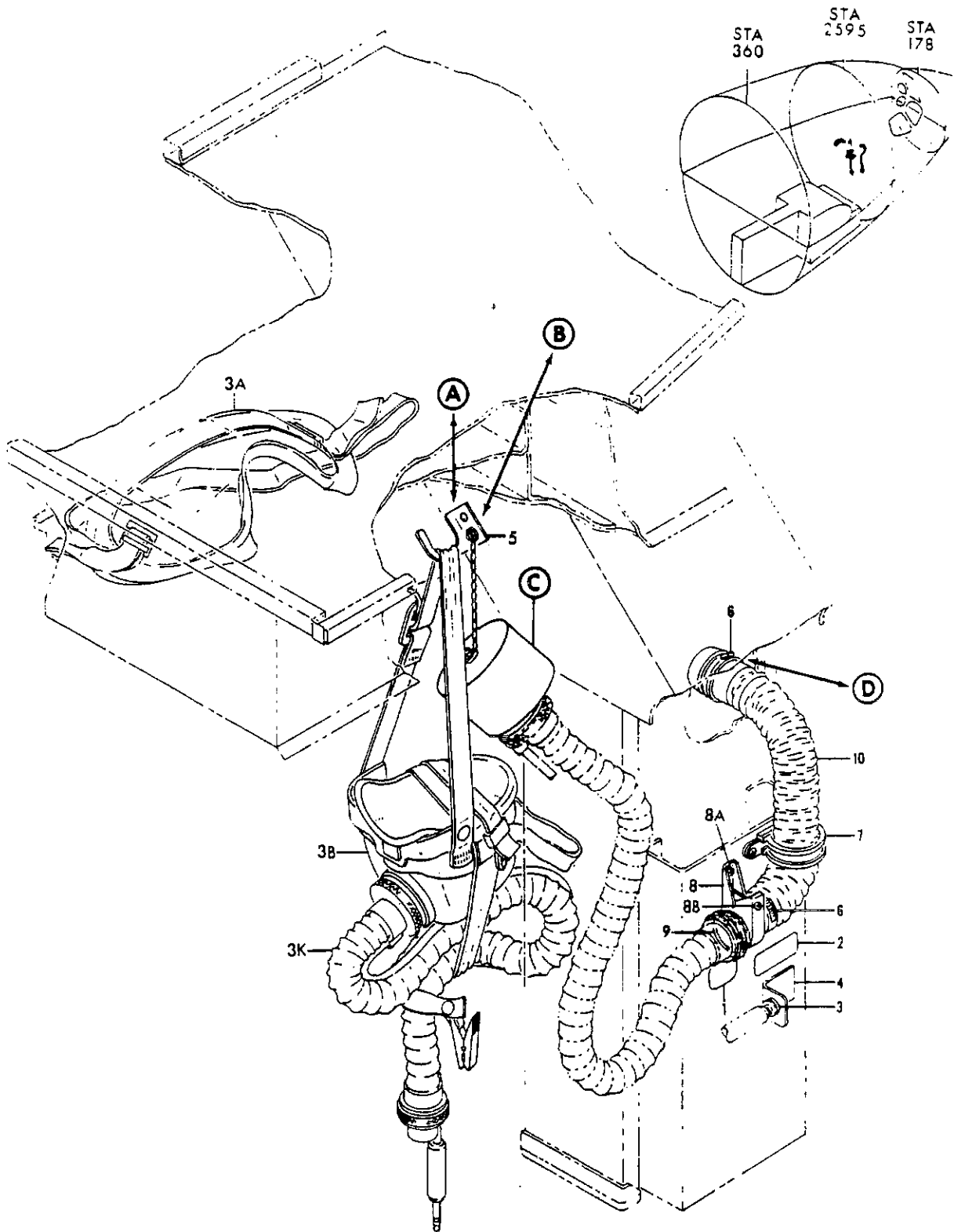
FIGURE 7. STOWAGE INSTL, FLIGHT ENGINEERS OXYGEN MASK (SHEET 1)
