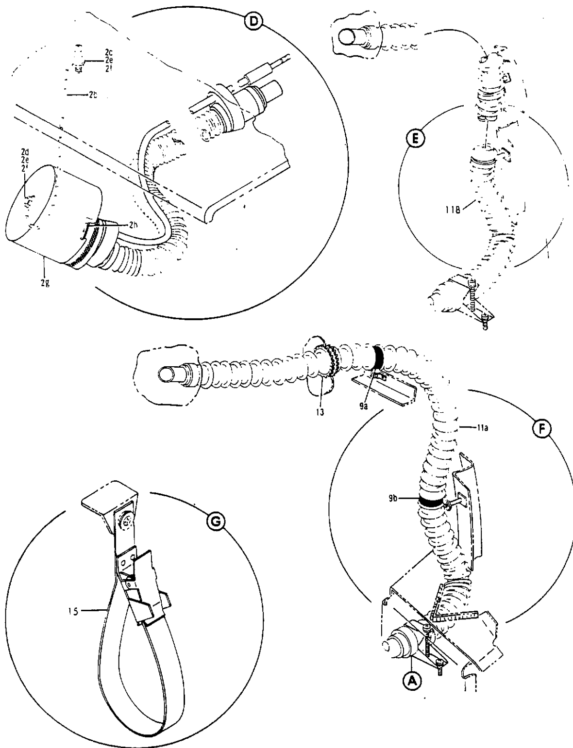
MASK INSTL, NAVIGATOR OXYGEN FIGURE 9. HOOK INSTL, NAVIGATOR OXYGEN (SHEET 2)
