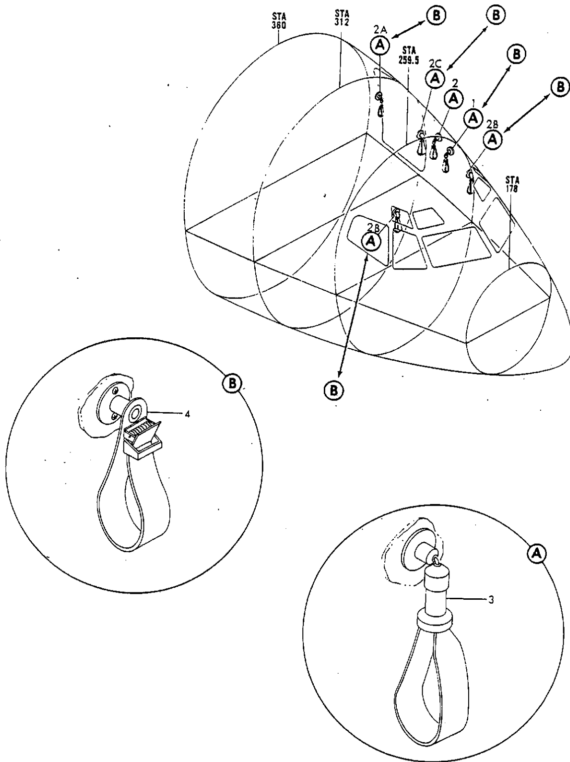
FIGURE 18. HANGER INSTALLATION, OBSERVERS OXYGEN MASK
