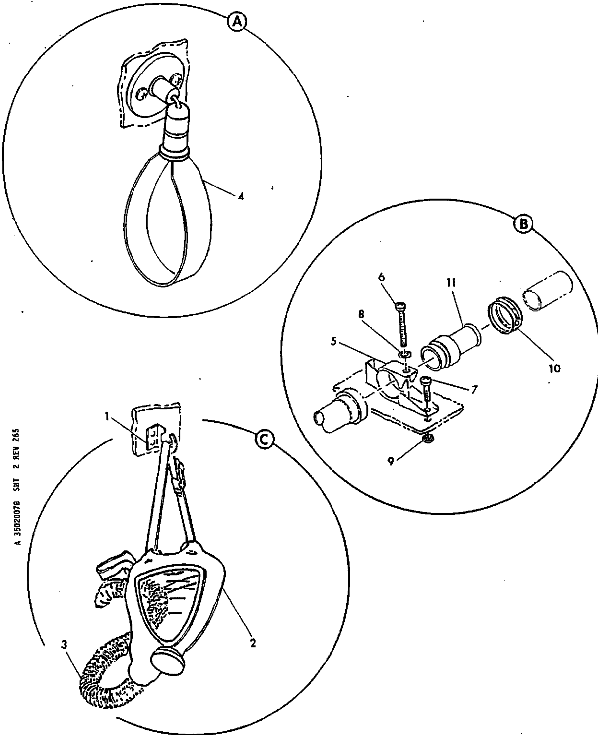
FIGURE 7B. STOWAGE INSTL. MODIFICATION FLIGHT ENGINEERS OXYGEN MASK (SHEET 2)
