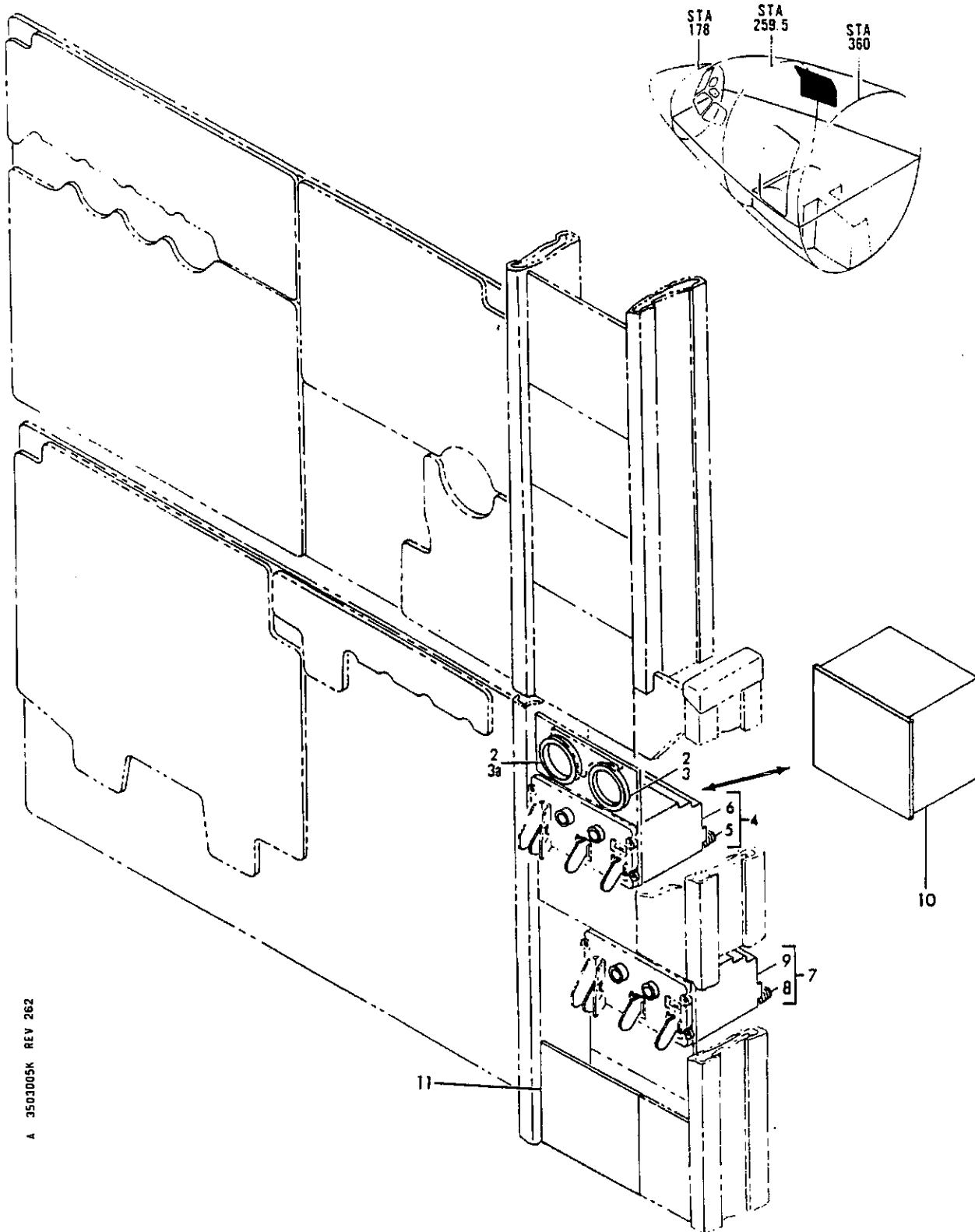
FIGURE 5K. PANEL INSTL, FLIGHT ENGINEERS AUXILIARY (OXYGEN ONLY)
