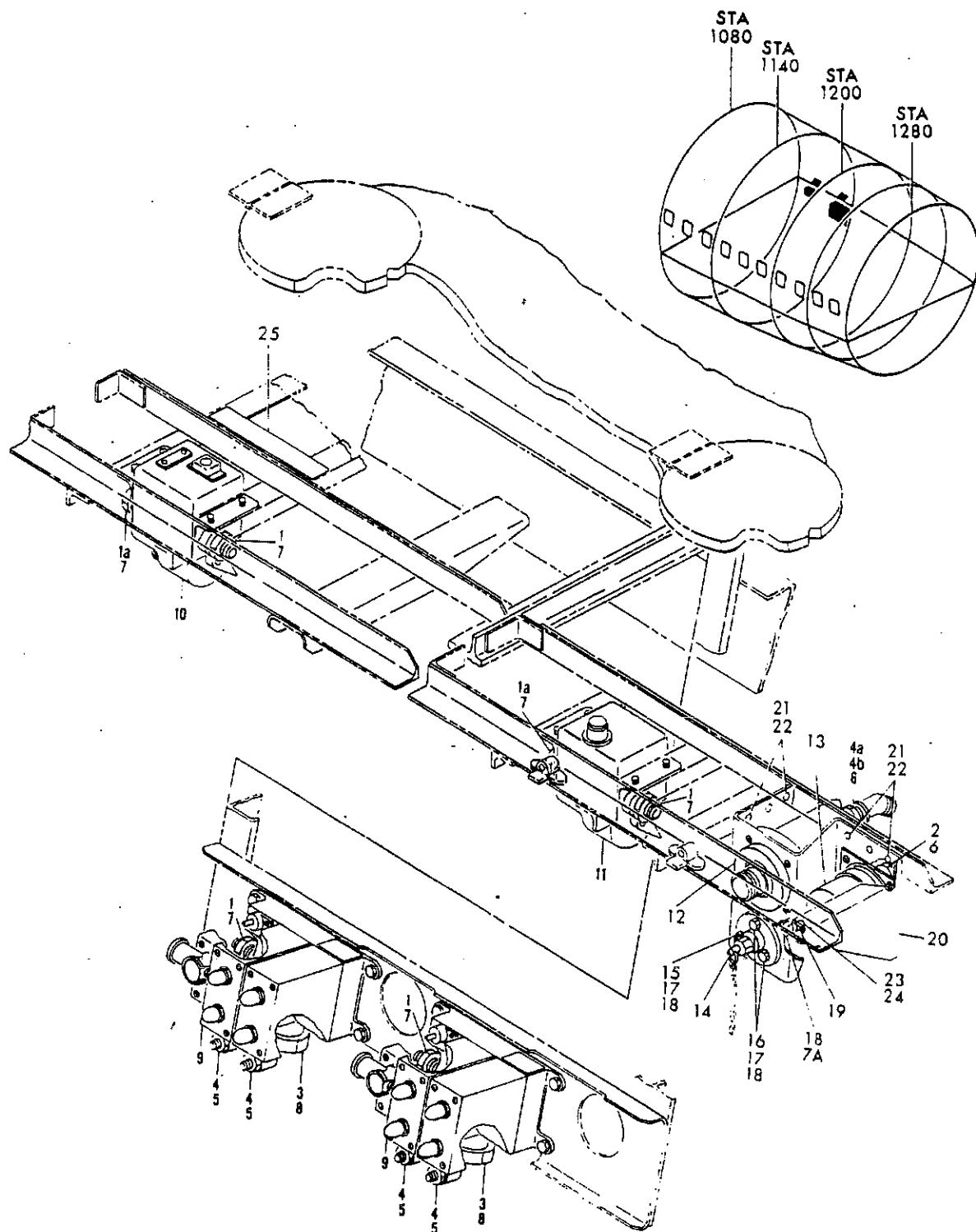
FIGURE 32. EQUIPMENT INSTL, PASSENGER OXYGEN (OXYGEN ONLY)
