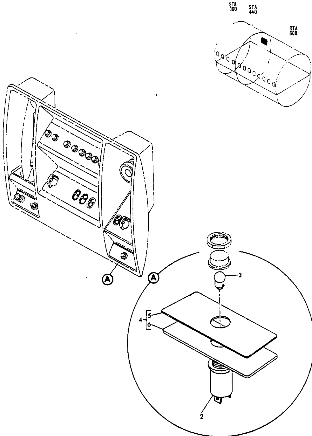
FIGURE 11A. PANEL INSTL. FORWARD GALLEY ATTENDANTS (OXYGEN ONLY)
