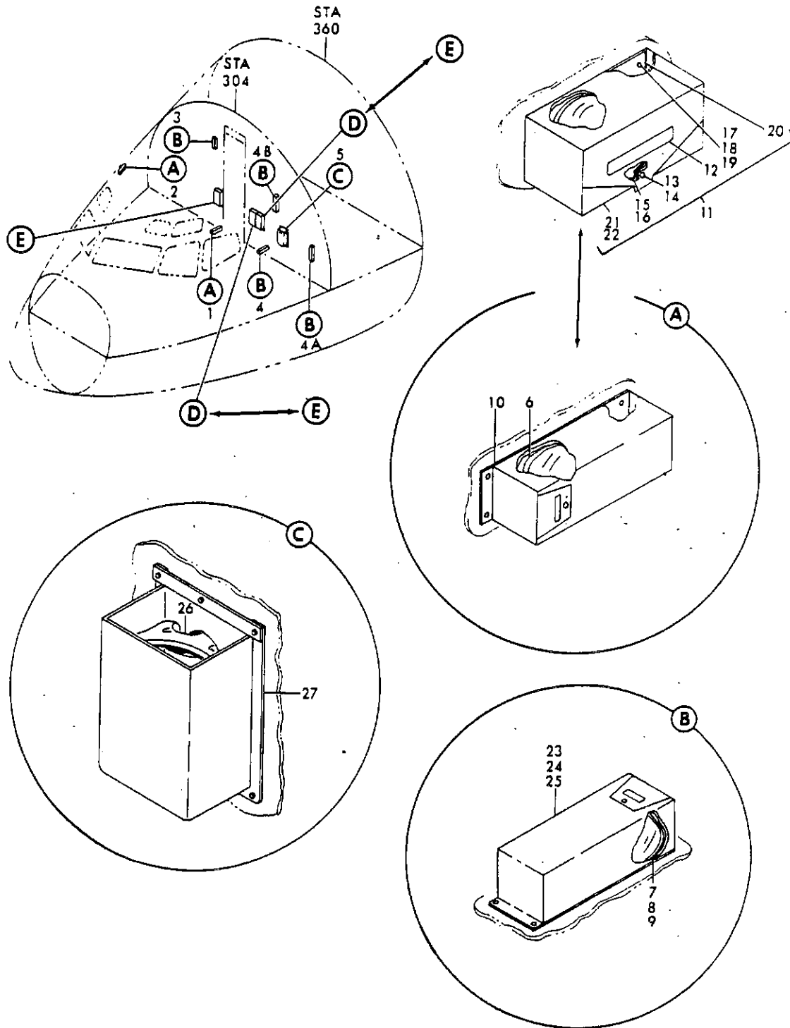
FIGURE 1A. POUCH INSTL, CAPTAINS AND FIRST OFFICERS SMOKE GOGGLE AND OXYGEN MASK (SHEET 1)
