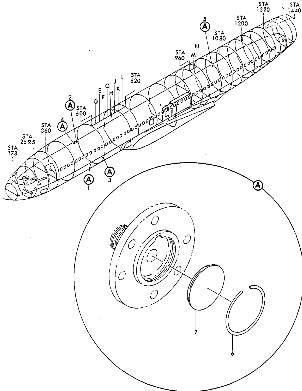
FIGURE 92, INDICATOR ASSY, OXYGEN THERMAL DISCHARGE
