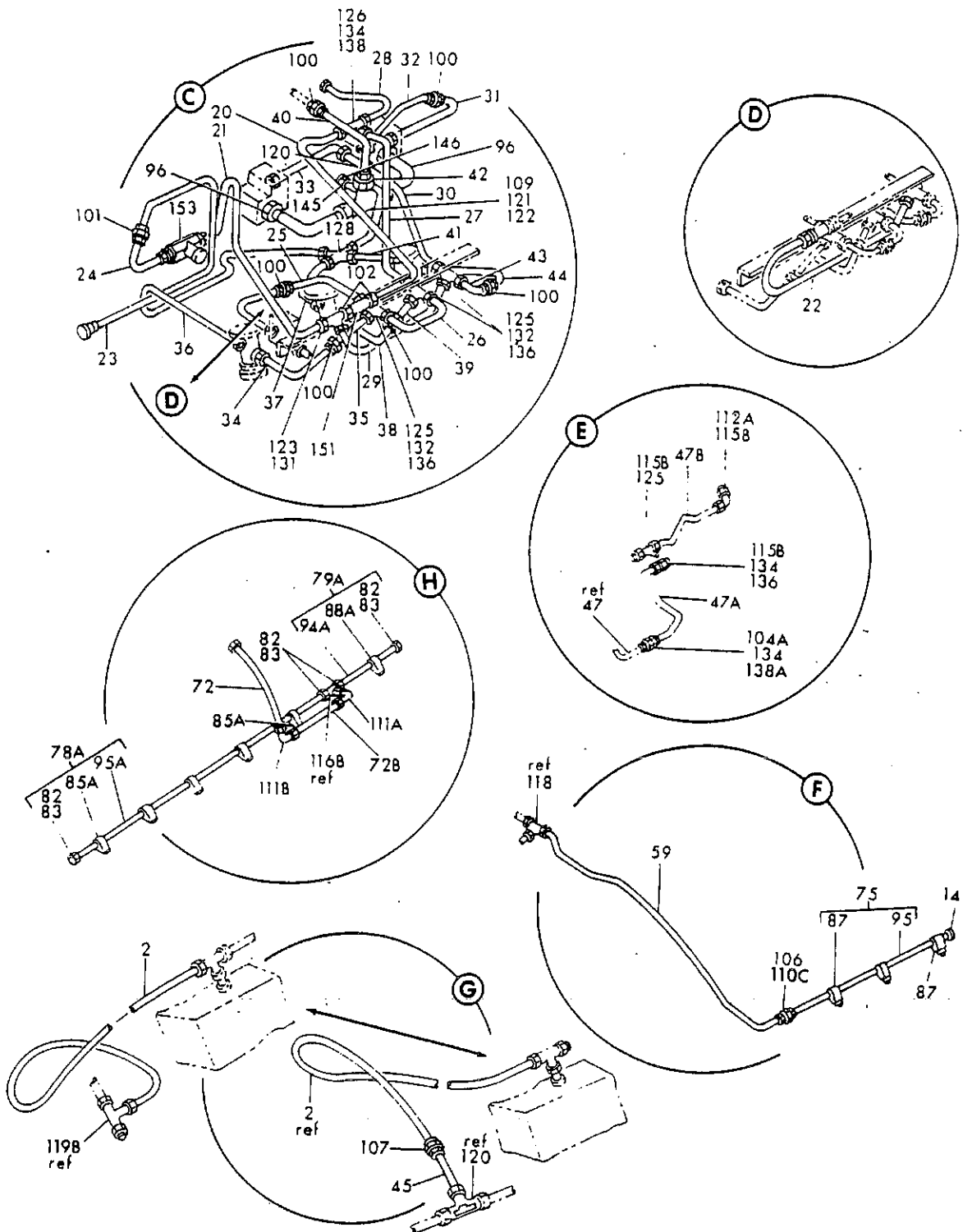
FIGURE 14C. TUBING INSTL, SECTION 43 OXYGEN (OXYGEN ONLY) (SHEET 3)
