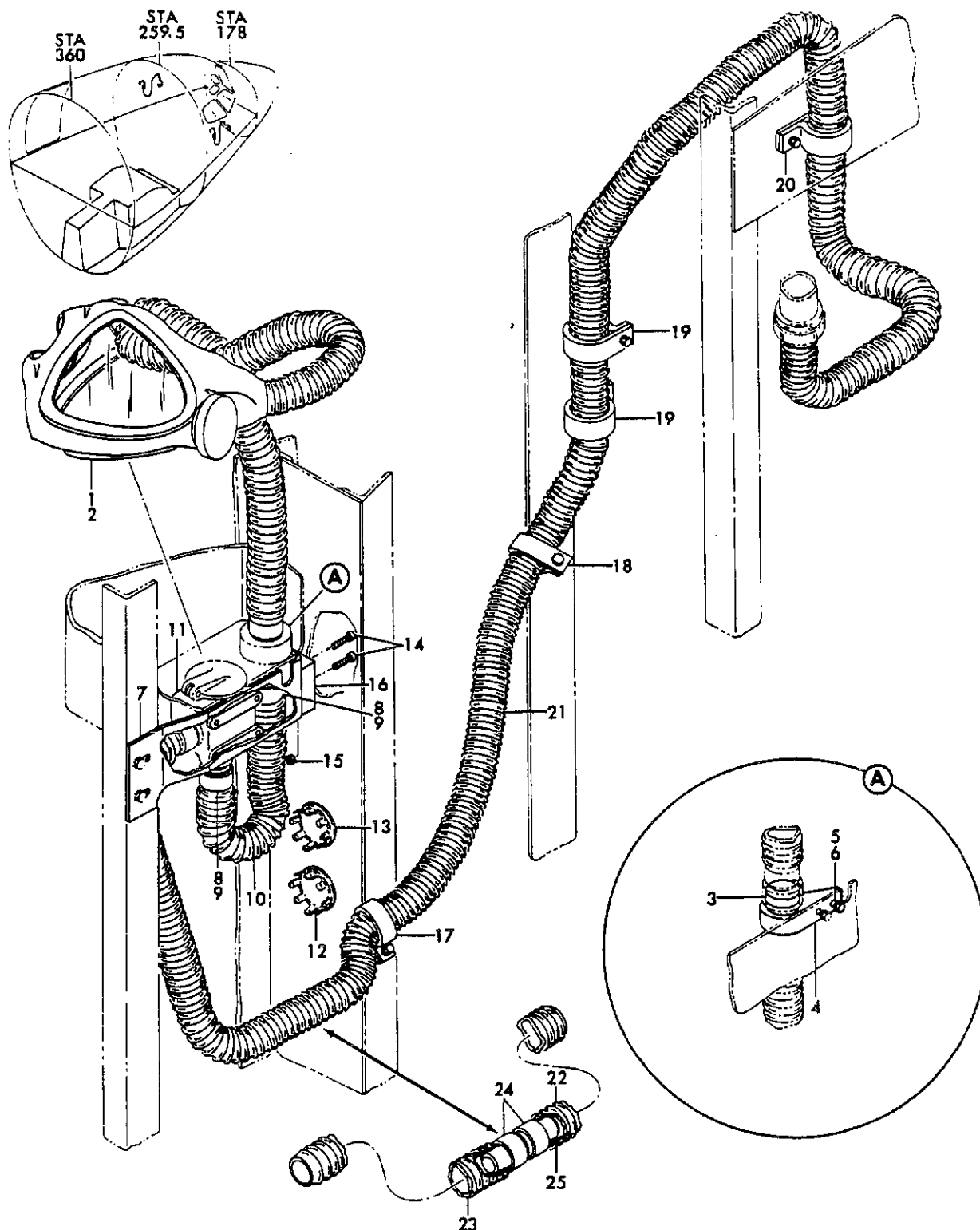
FIGURE 48. HOSE AND VALVE INSTL, PILOT AND COPILOT OXYGEN MASK
