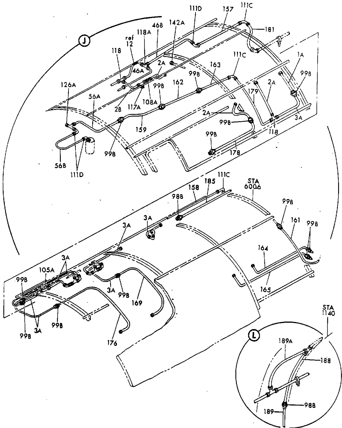
FIGURE 14G. TUBING INSTL, SECTION 43 OXYGEN (OXYGEN ONLY) (SHEET 4)
