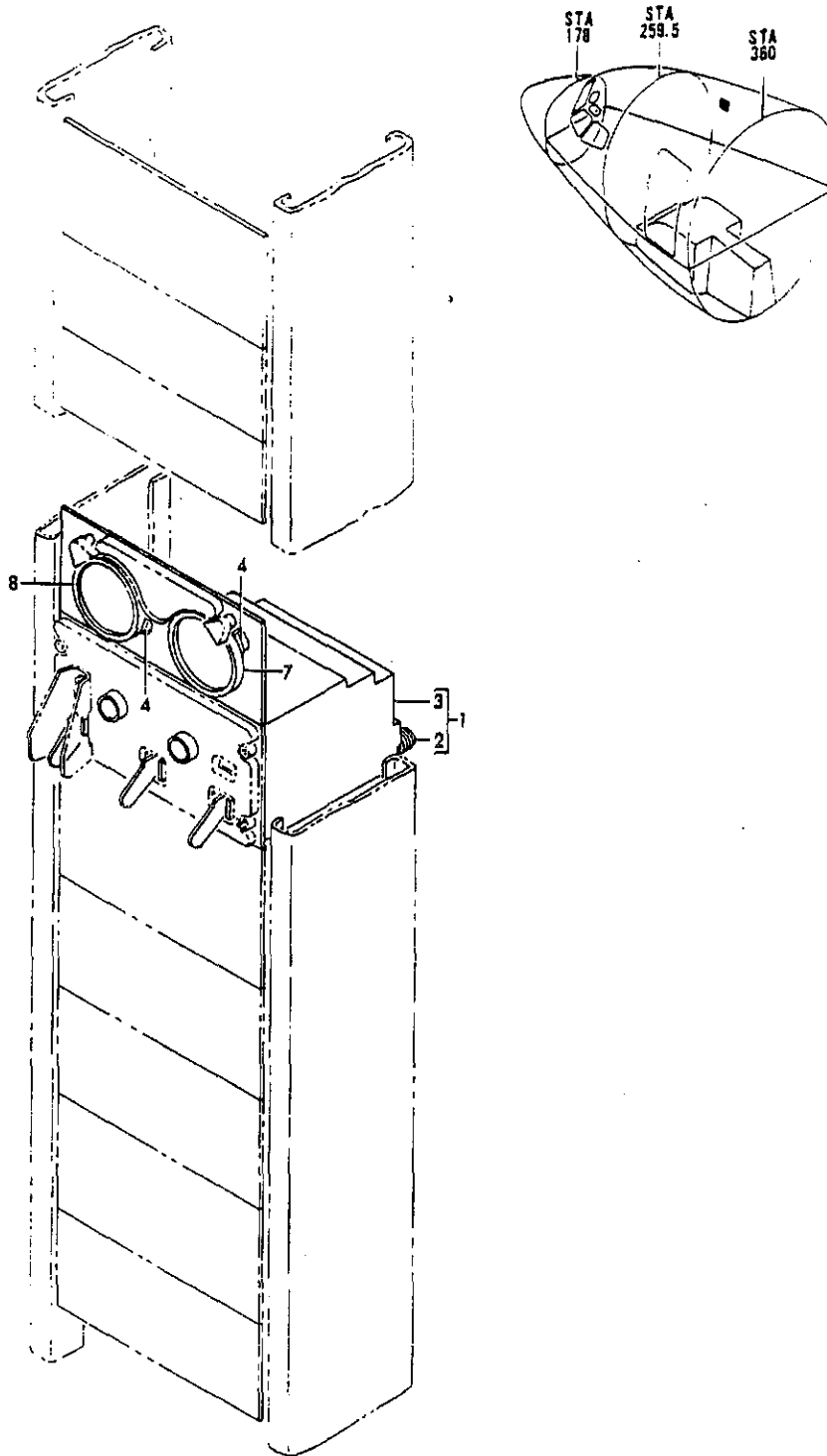
FIGURE 5N. PANEL INSTL, FLIGHT ENGINEERS AUXILIARY (OXYGEN ONLY)
