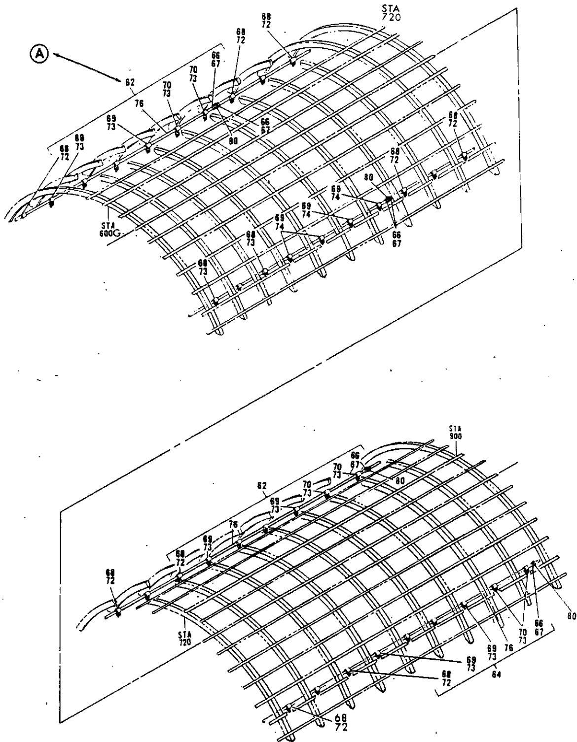
FIGURE 14C. TUBING INSTL. SECTION 43 OXYGEN (OXYGEN ONLY) (SHEET 2)
