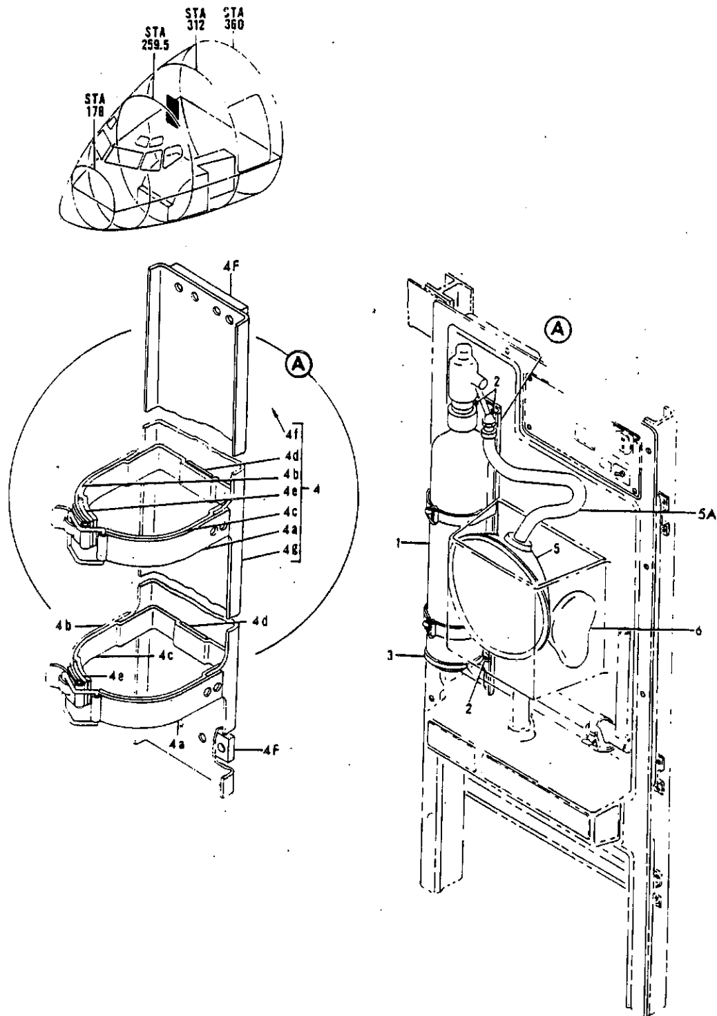
FIGURE 35. EQUIPMENT INSTL. CONTROL CAB EMERGENCY (OXYGEN ONLY)
