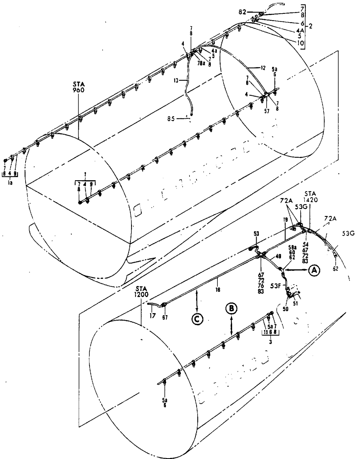
FIGURE 30. TUBING INSTL, SECTION 46 OXYGEN (SHEET 1)
