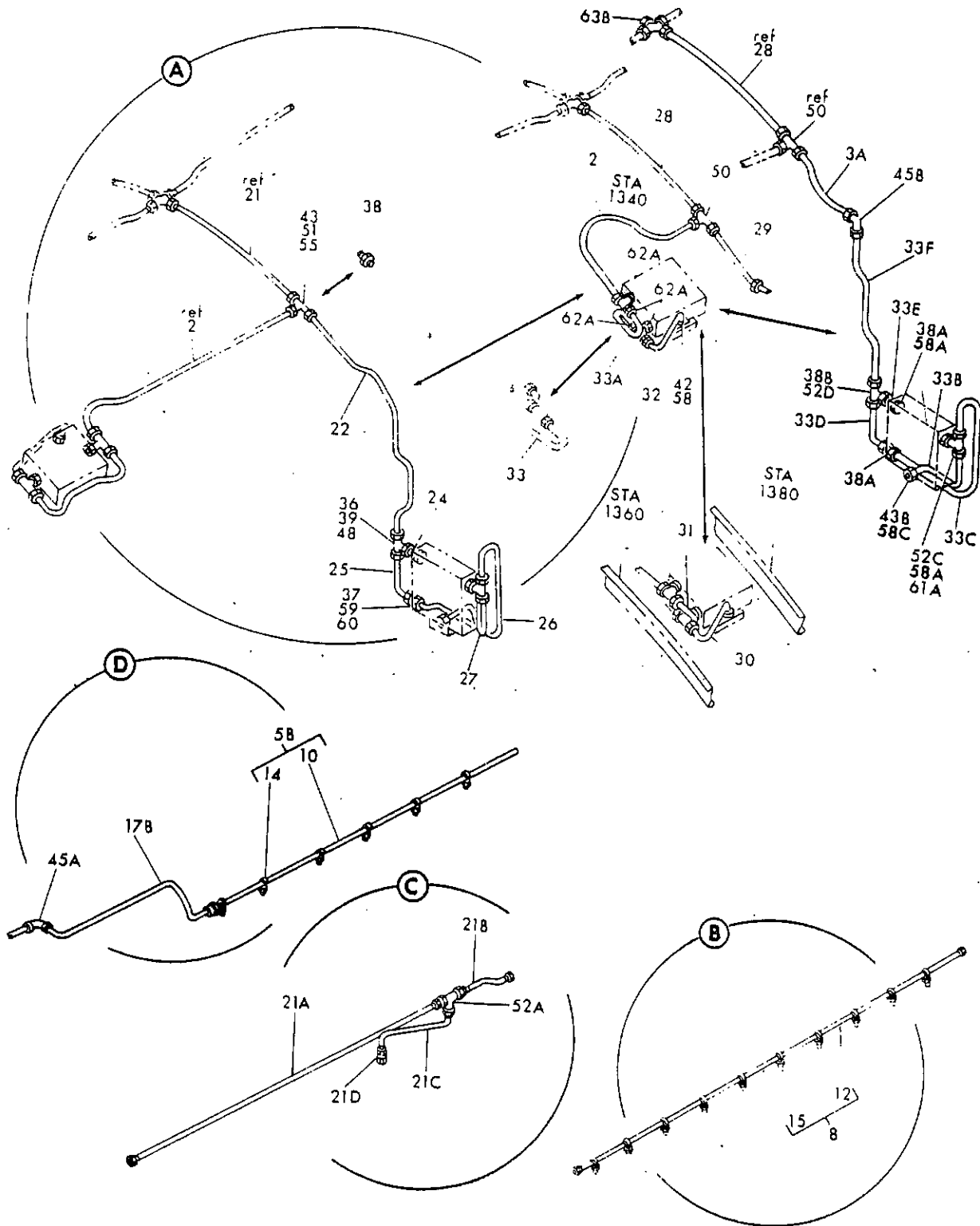
FIGURE 30U. TUBING INSTL. SECTION 46 OXYGEN (SHEET 2)
