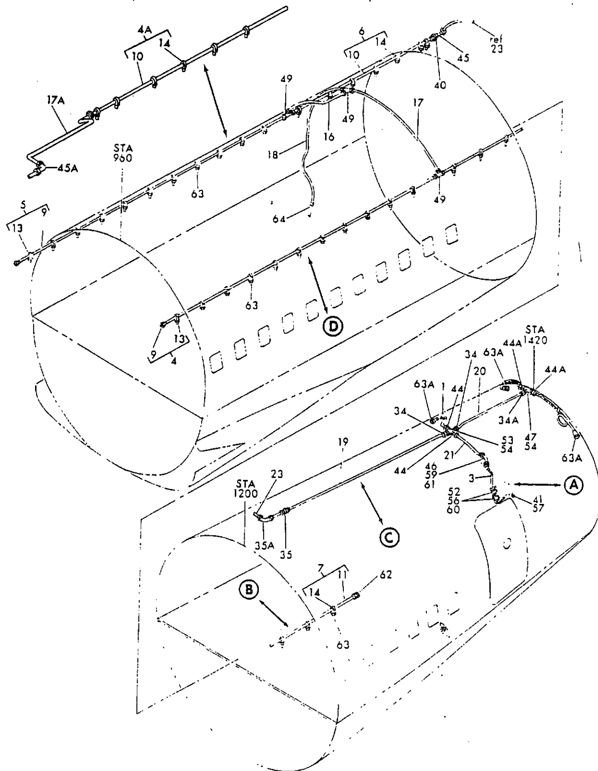
FIGURE 30U. TUBING INSTL. SECTION 46 OXYGEN (SHEET 1)
