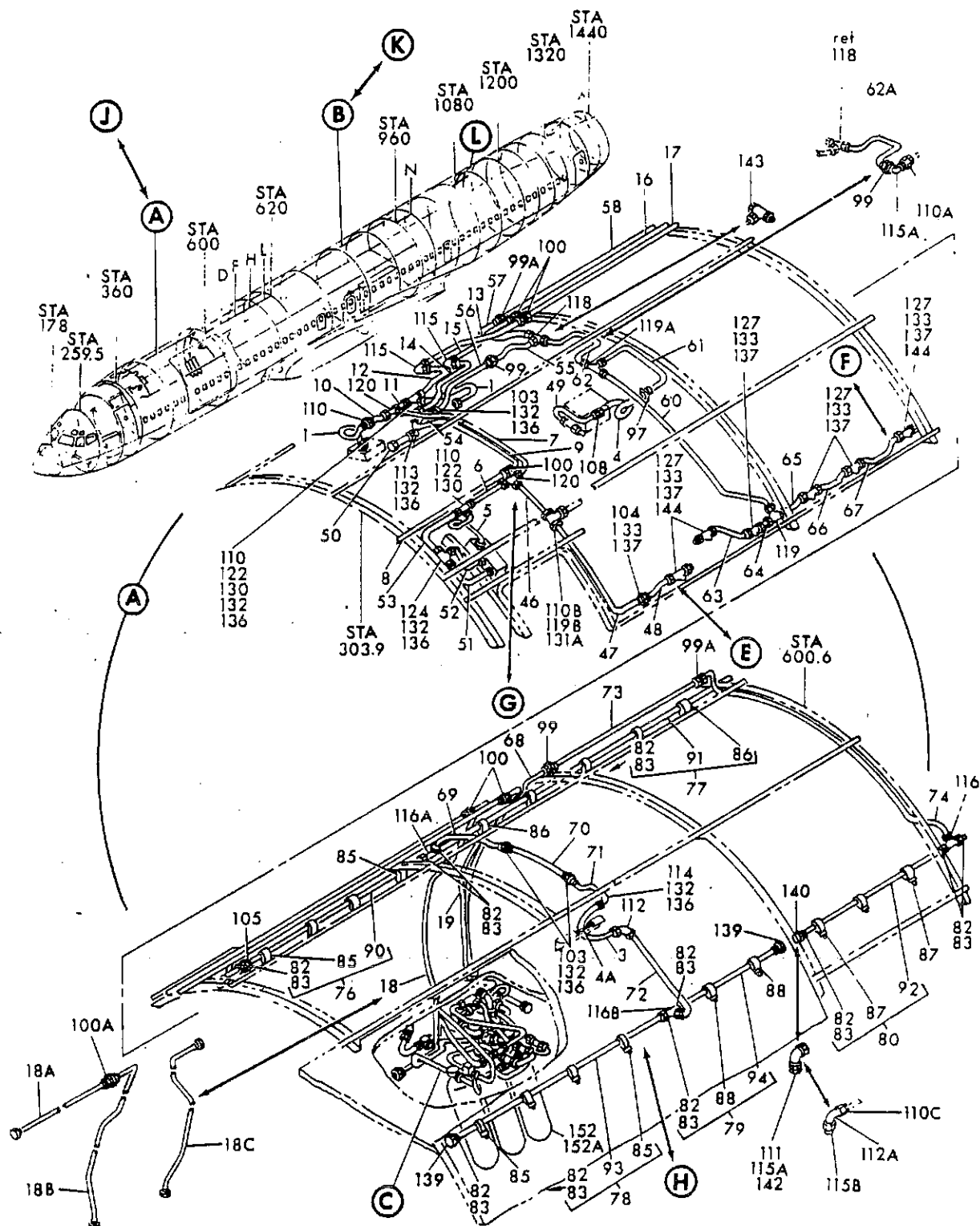
FIGURE 14G. TUBING INSTL, SECTION 43 OXYGEN (OXYGEN ONLY) (SHEET 1)
