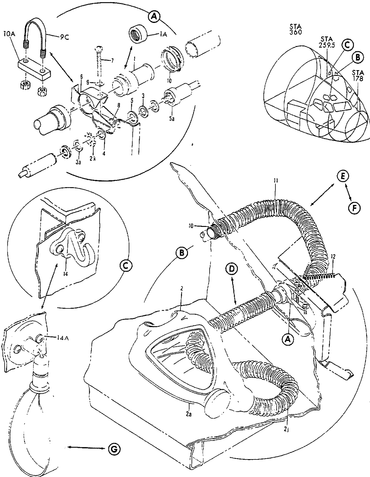
MASK INSTL. NAVIGATOR OXYGEN FIGURE 9. HOOK INSTL. NAVIGATOR OXYGEN (SHEET 1)
