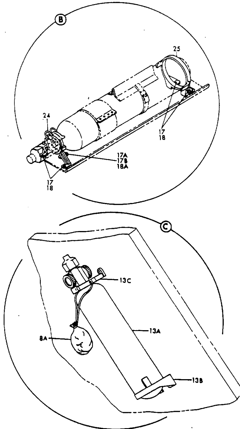
FIGURE 28. BOTTLE INSTL. OXYGEN (SHEET 2)
