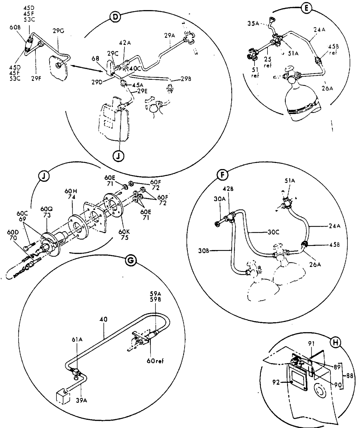
FIGURE 30H. TUBING INSTL, SECTION 46 OXYGEN (OXYGEN ONLY) (SHEET 2)
