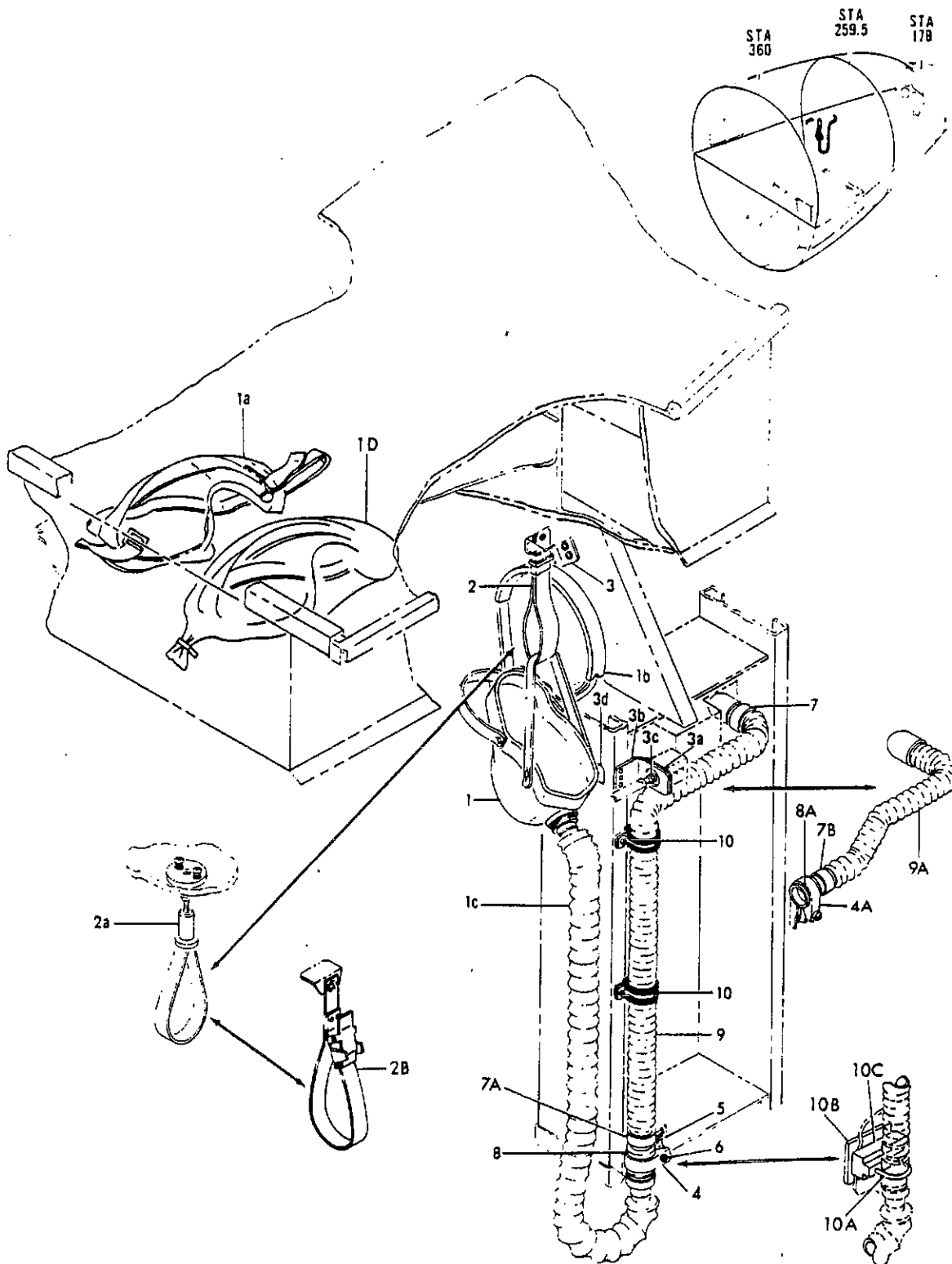
FIGURE 5B. STOWAGE INSTL, FLIGHT ENGINEERS OXYGEN MASK
