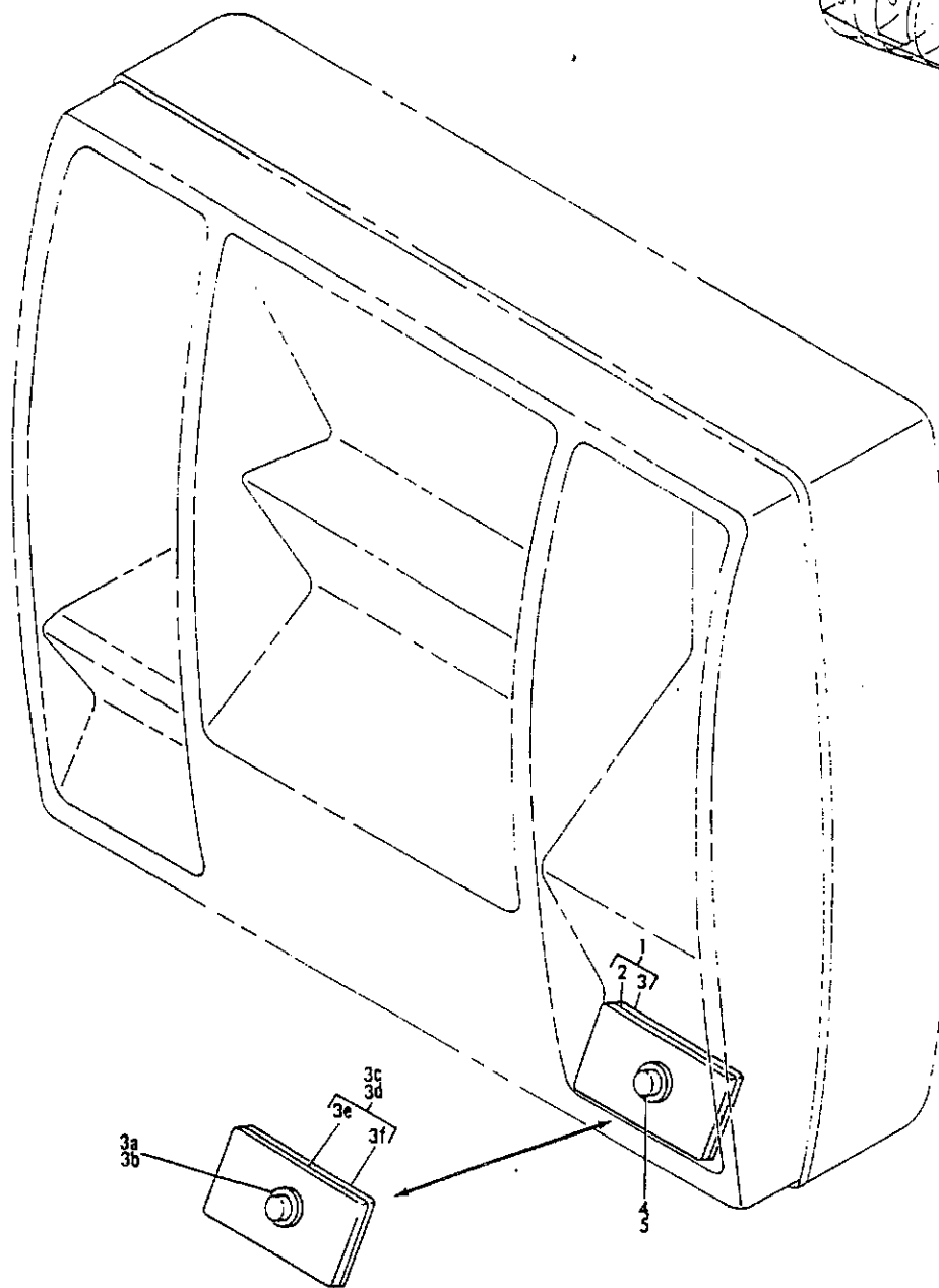
FIGURE 14A. PANEL INSTL, AFT GALLEY ATTENDANTS (OXYGEN ONLY)
