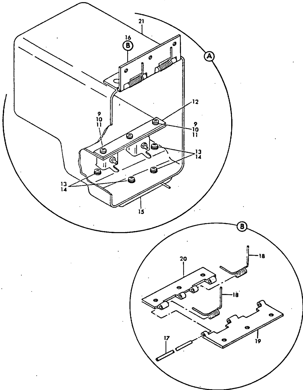
FIGURE 25A. MODULE ASSY, LOW PRESSURE OXYGEN (SHEET 2)
