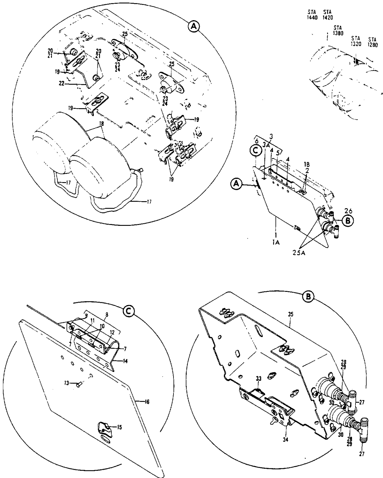
FIGURE 14. MASK AND CONTAINER INSTL, AFT ATTENDANTS OXYGEN
