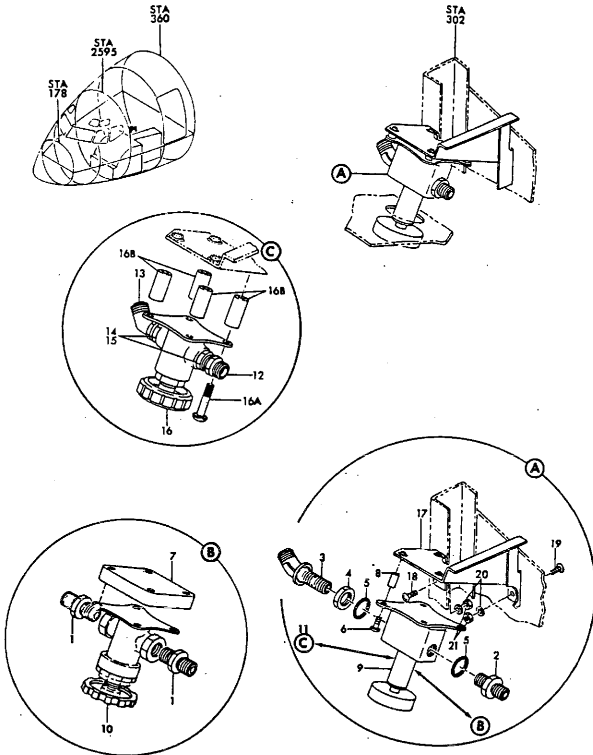
FIGURE 36A. VALVE INSTL, CREW OXYGEN HIGH AND LOW PRESSURE (OXYGEN ONLY)
