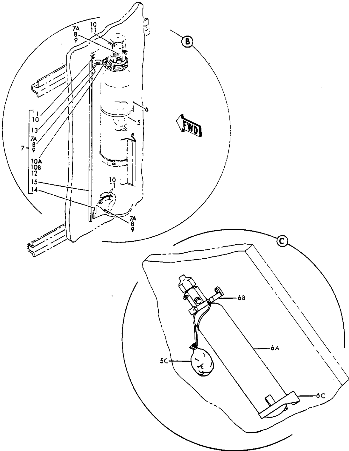
FIGURE 28A. BOTTLE INSTL, OXYGEN (SHEET 2)
