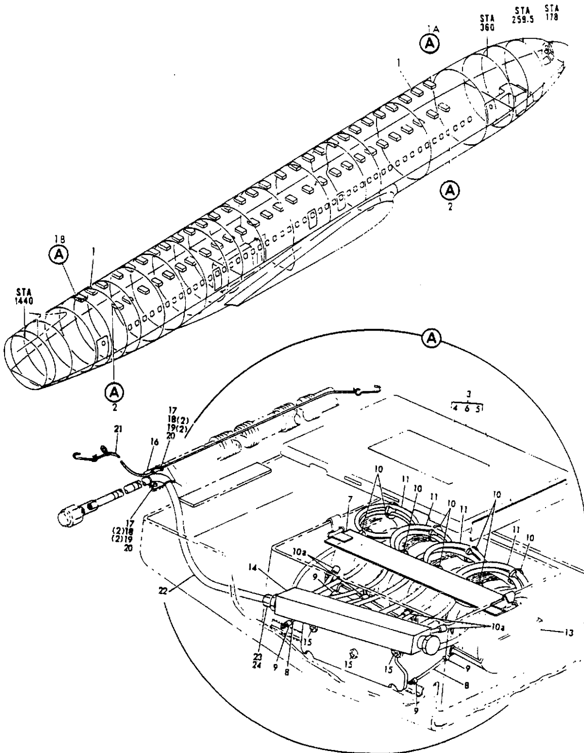
FIGURE 68Z. SERVICE UNIT INSTL, PASSENGER (OXYGEN ONLY)
