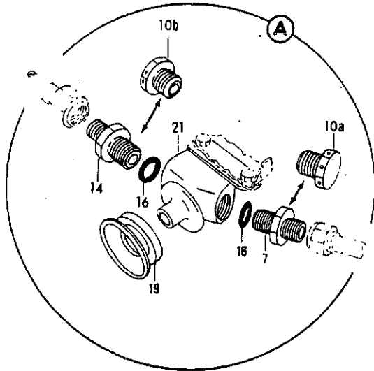
FIGURE 13. DRAIN INSTL, FAN ENGINE (PNEUMATIC ONLY)
