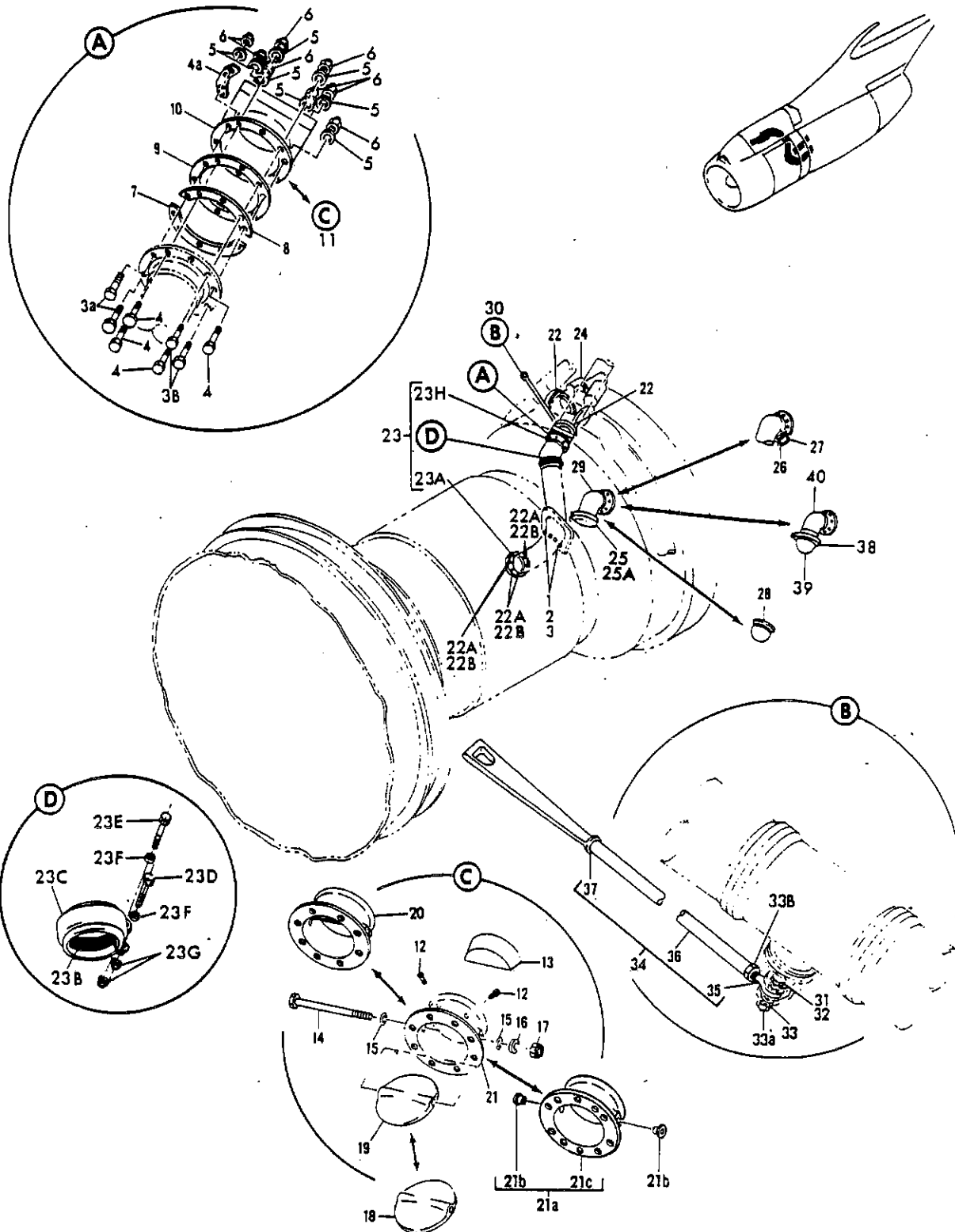
FIGURE 10. DUCT INSTL, WING THERMAL ANTI-ICING AND AIR CONDITIONING
