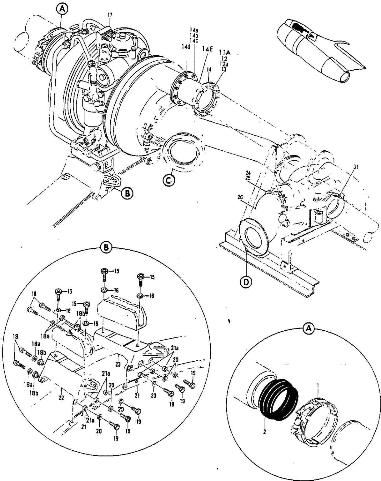
FIGURE 2. TURBOCOMPRESSOR INSTL, FAN ENGINE (SHEET 1)
