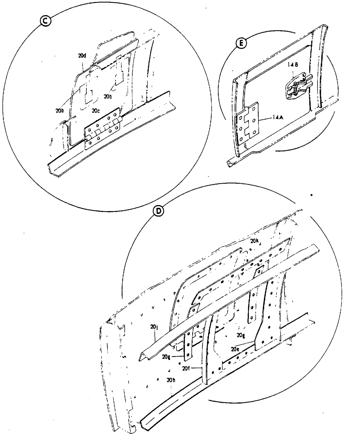
FIGURE 17. FAIRING ASSY, NACELLE TURBO COMPRESSOR FORWARD (PNEUMATIC ONLY) (SHEET 2)
