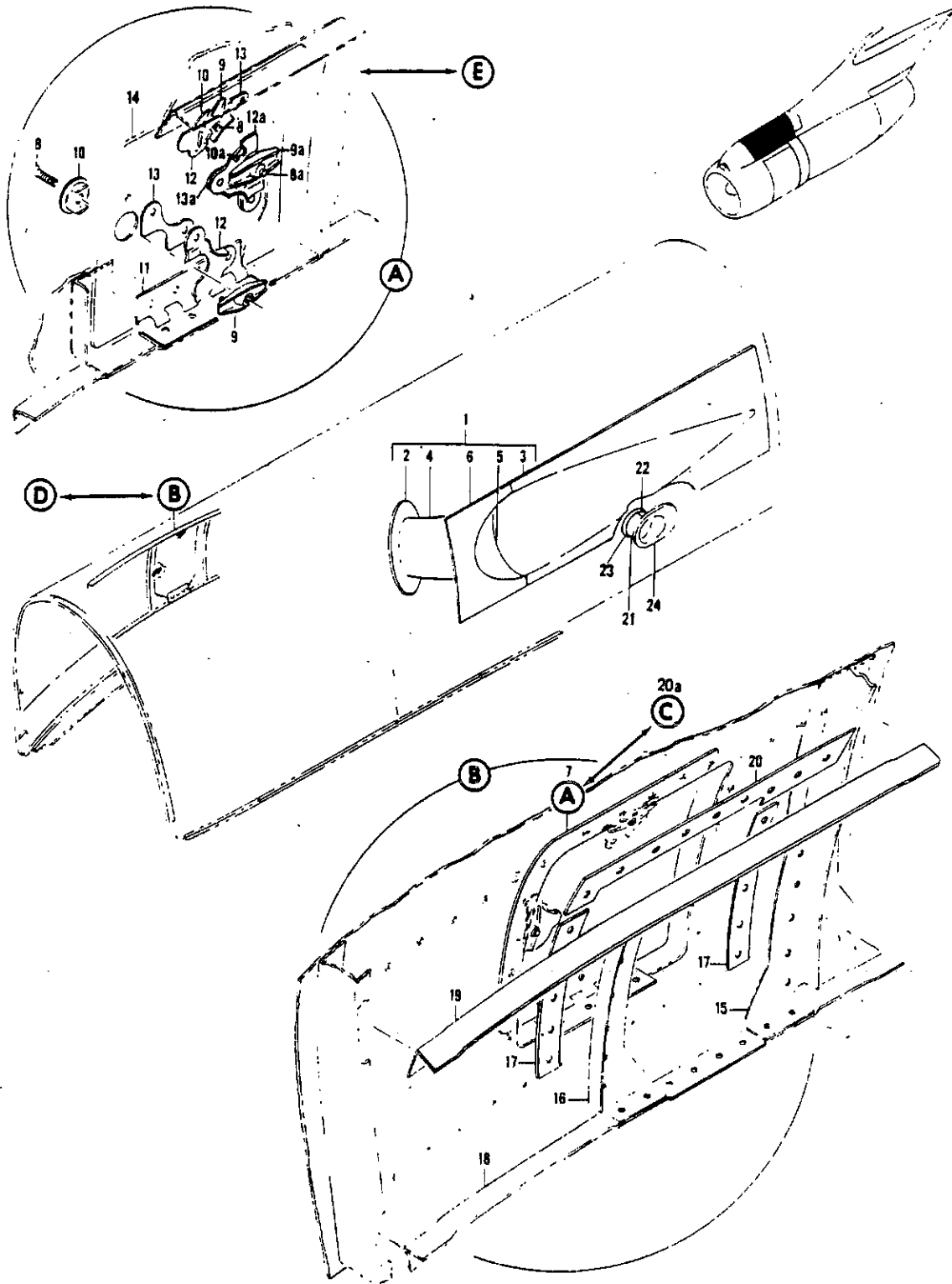
FIGURE 17. FAIRING ASSY, NACELLE TURBO COMPRESSOR FORWARD (PNEUMATIC ONLY) (SHEET 1)
