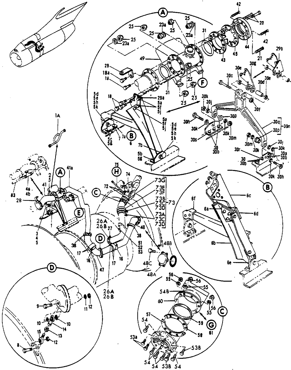
FIGURE 11. DUCT INSTL, WING THERMAL ANTI-ICING AND AIR CONDITIONING (ENGINES NO. 2, 3, AND 4) (SHEET 1)
