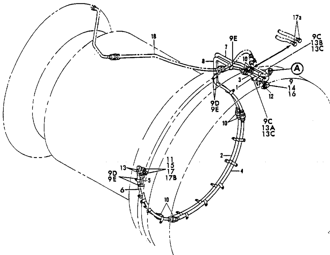
FIGURE 15. PLUMBING INSTL, FAN ENGINE TURBOCOMPRESSOR OIL COOLER AND SUPPLY (PNEUMATIC ONLY)
