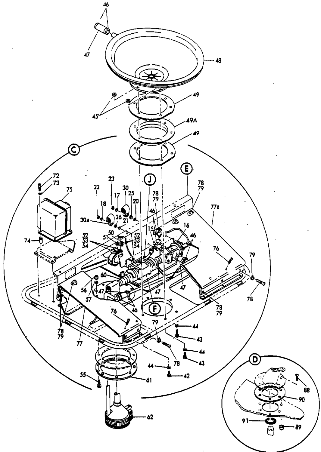
FIGURE 64. TOILET ASSY, AC FLUSH (SHEET 2)
