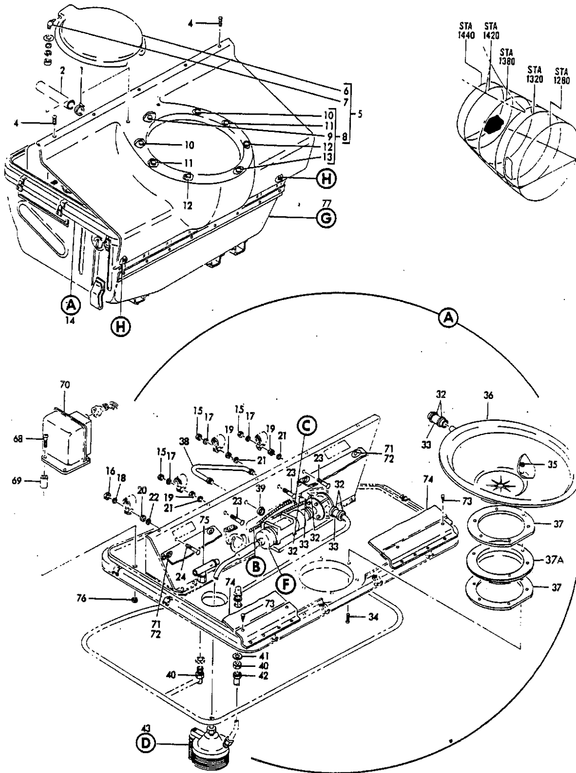
FIGURE 62. TOILET ASSY, AC FLUSH (SHEET 1)
