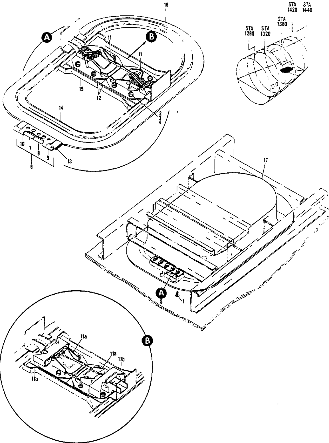
FIGURE 18. PAN AND DOOR INSTL, STATION 1390 AFT TOILET SERVICE
