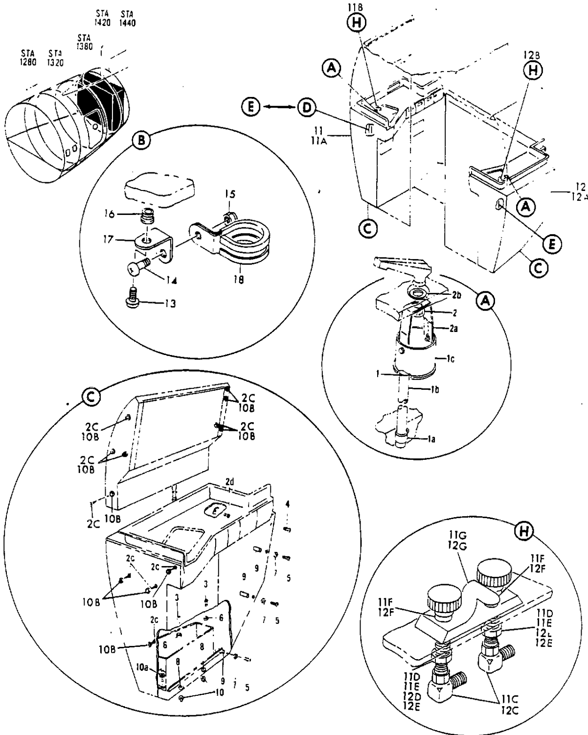
FIGURE 34. LAVATORY INSTL. TOILET C AND D (WATER/WASTE ONLY) (SHEET 1)
