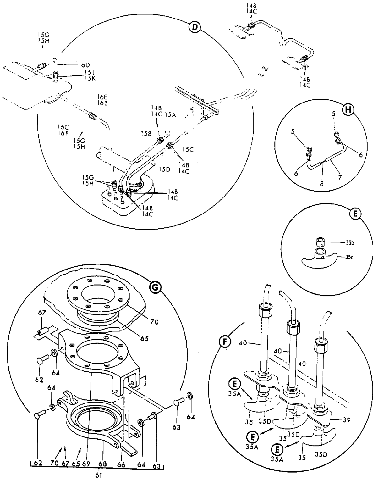
FIGURE 10. DRAIN INSTL, AFT TOILETS (WATER/WASTE ONLY) (SHEET 2)
