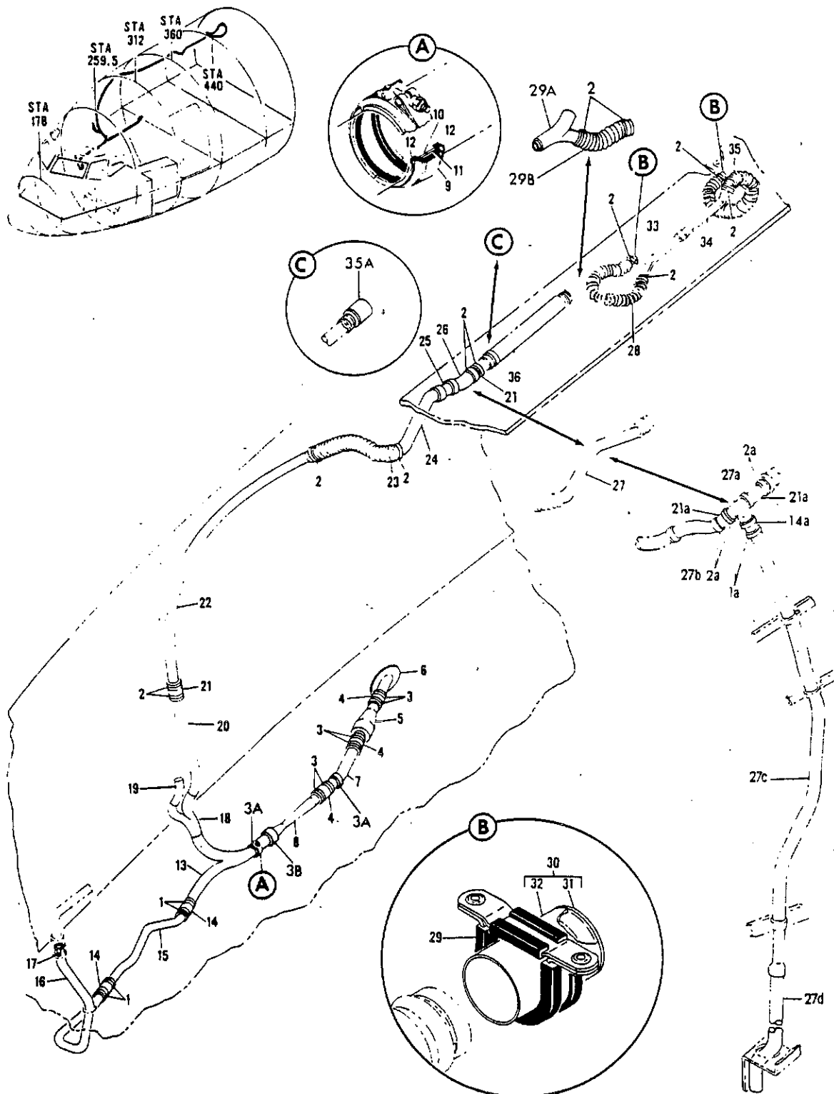
FIGURE 2. TOILET AND GALLEY VENTILATION SYSTEM INSTALLATION (FORWARD)
