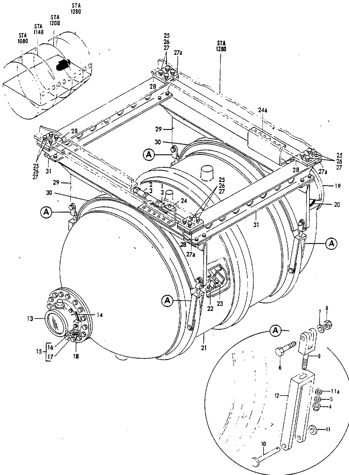
FIGURE 47. TANK INSTL, AFT POTABLE WATER SUPPORT INSTL, AFT POTABLE WATER TANK (WATER/WASTE ONLY)
