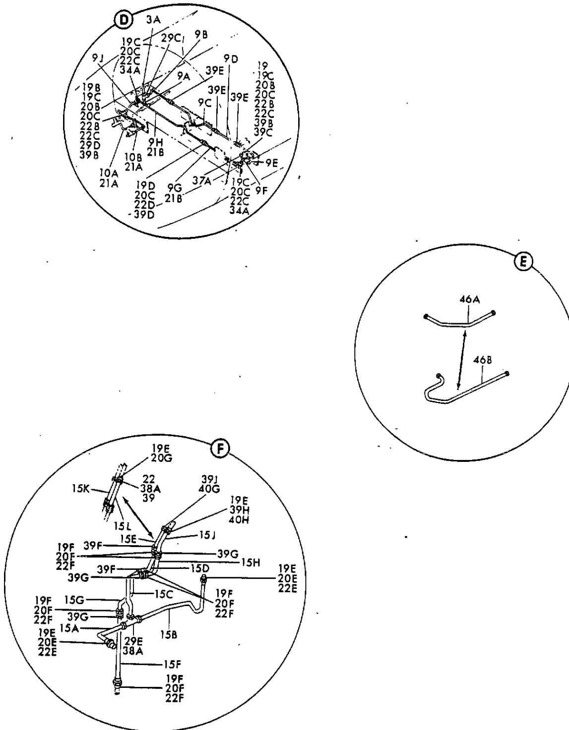
FIGURE 20. WATER SYSTEM INSTL, SECTION 43 FORWARD POTABLE (SHEET 3)
