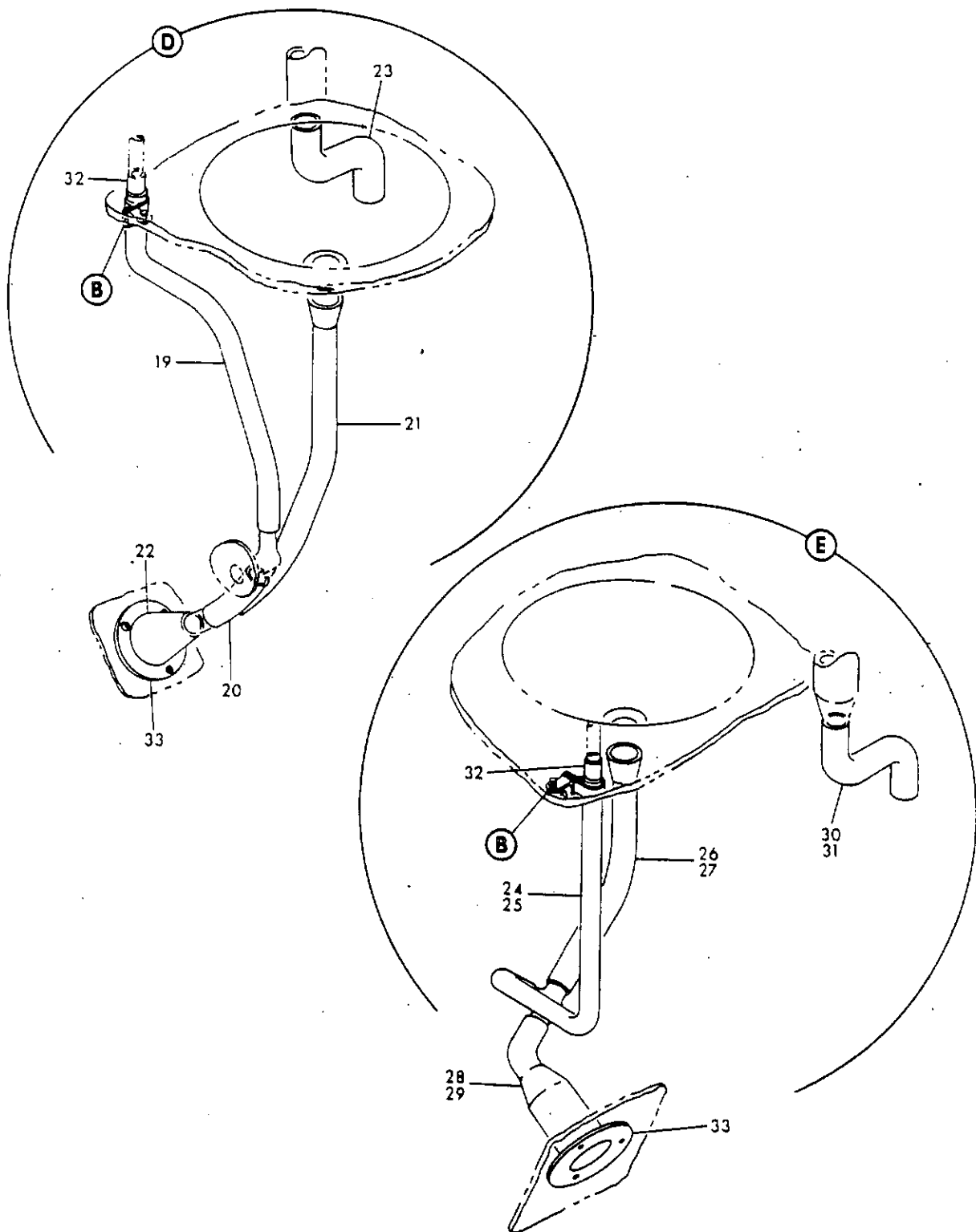
FIGURE 34. LAVATORY INSTL, TOILET C AND D (WATER/WASTE ONLY) (SHEET 2)
