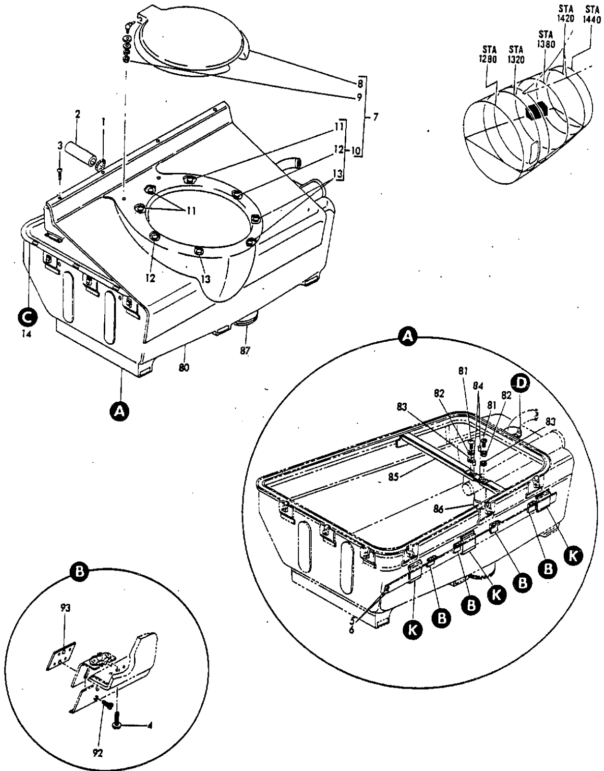
FIGURE 64. TOILET ASSY. AC FLUSH (SHEET 1)
