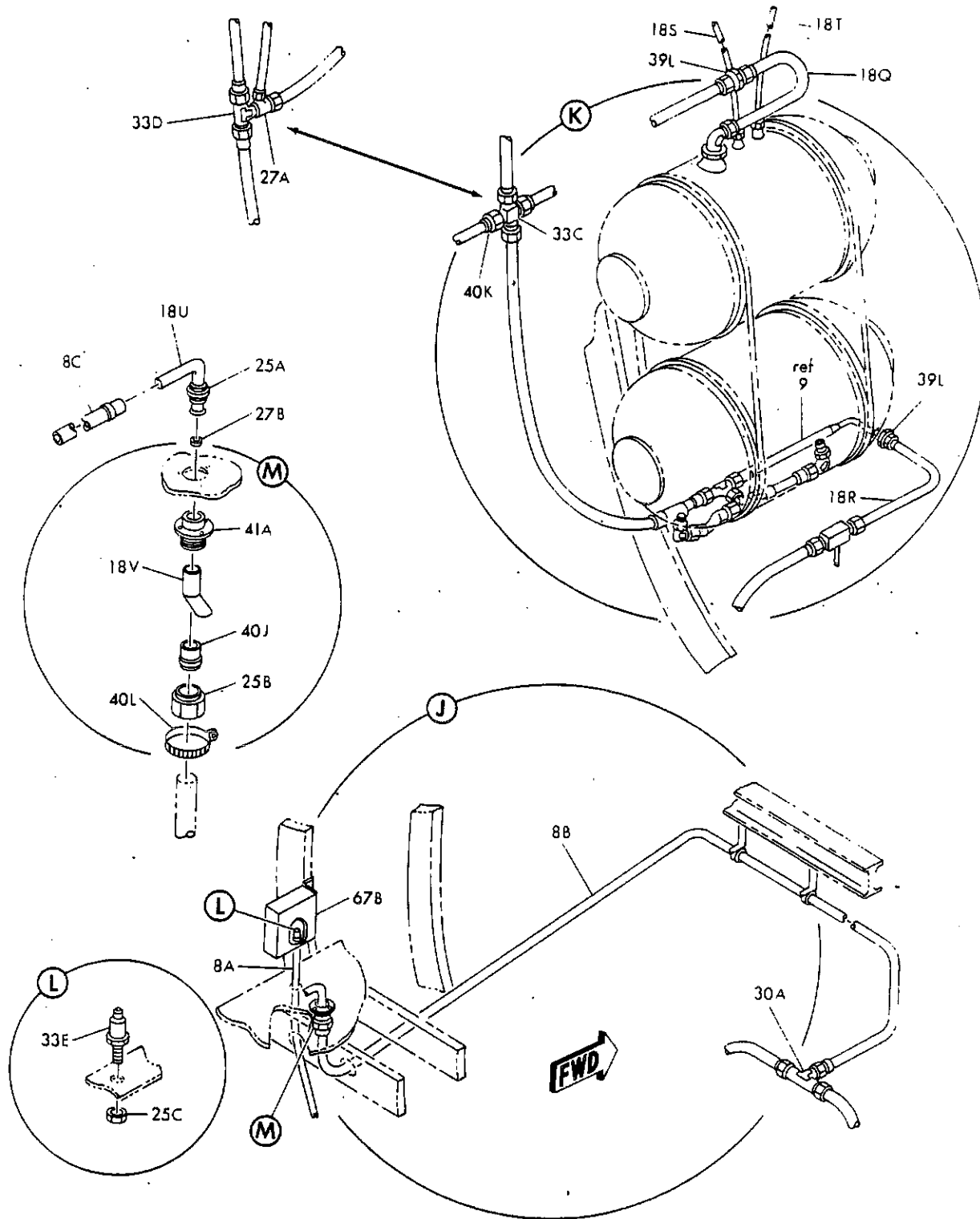
FIGURE 20. WATER SYSTEM INSTL SECTION 43 FORWARD PORTABLE (SHEET 5)
