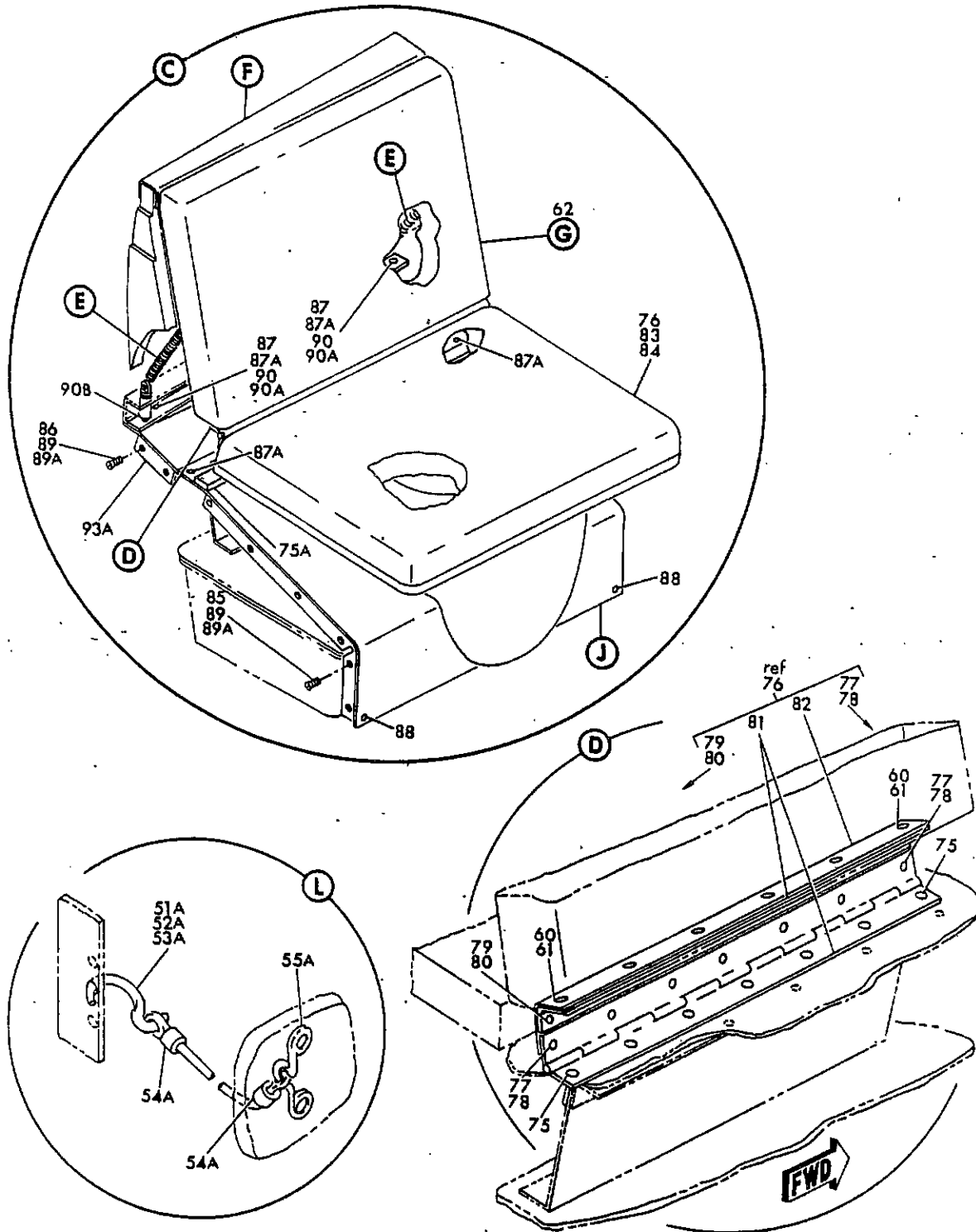
FIGURE 43. TOILET INSTL. FORWARD TOILET COMPARTMENT-B (WATER/WASTE ONLY) (SHEET 2)
