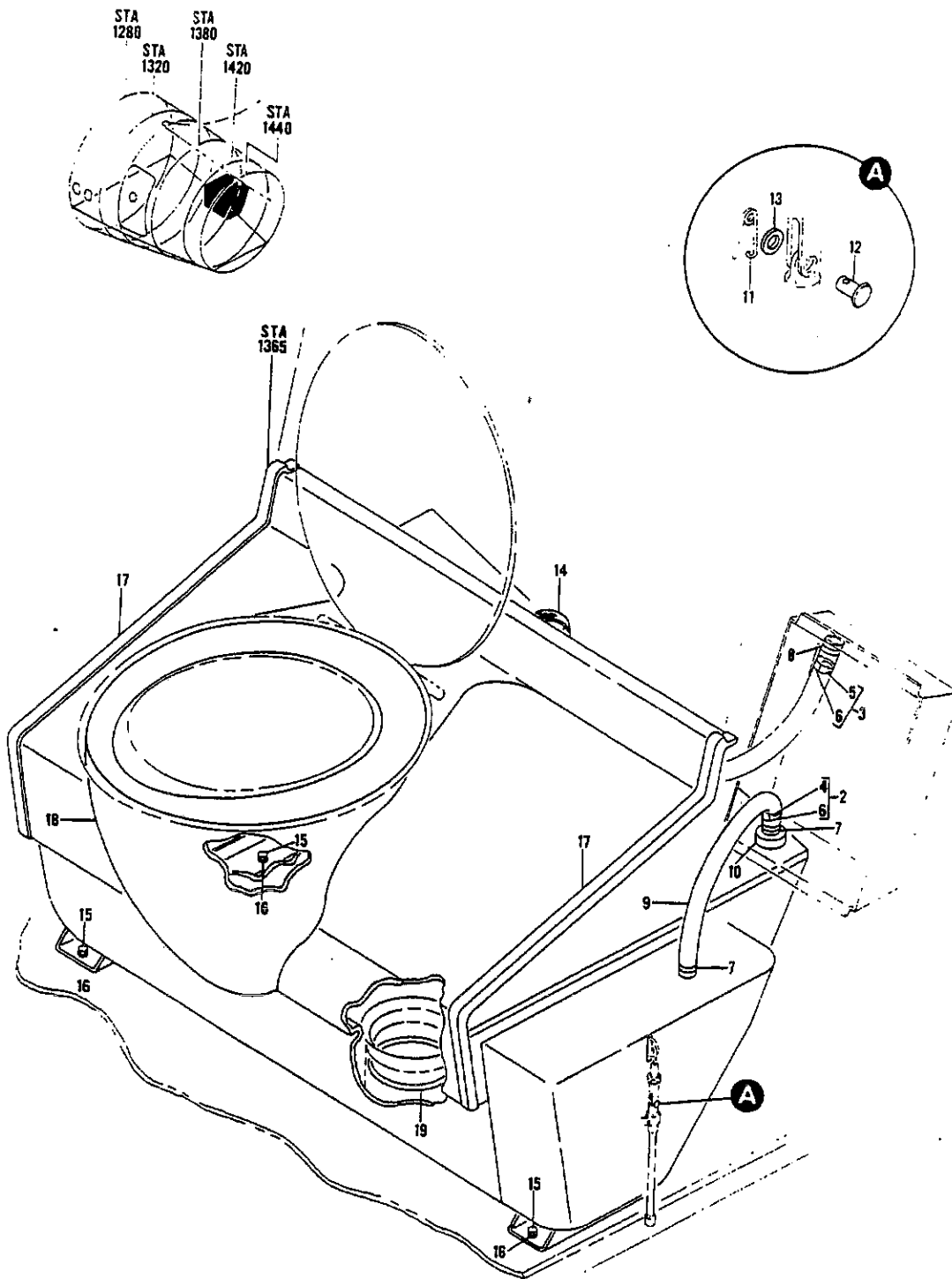
FIGURE 47. TOILET INSTL, AFT COMPARTMENT E (WATER/WASTE ONLY)
