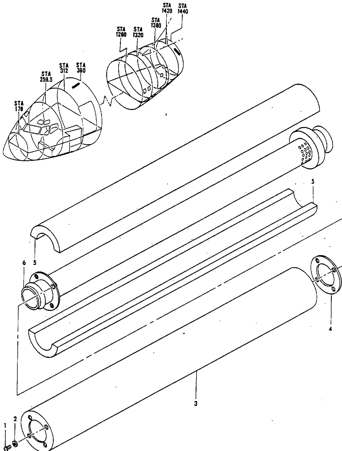
FIGURE 6. MUFLER ASSY. GALLEY VENTILATION
