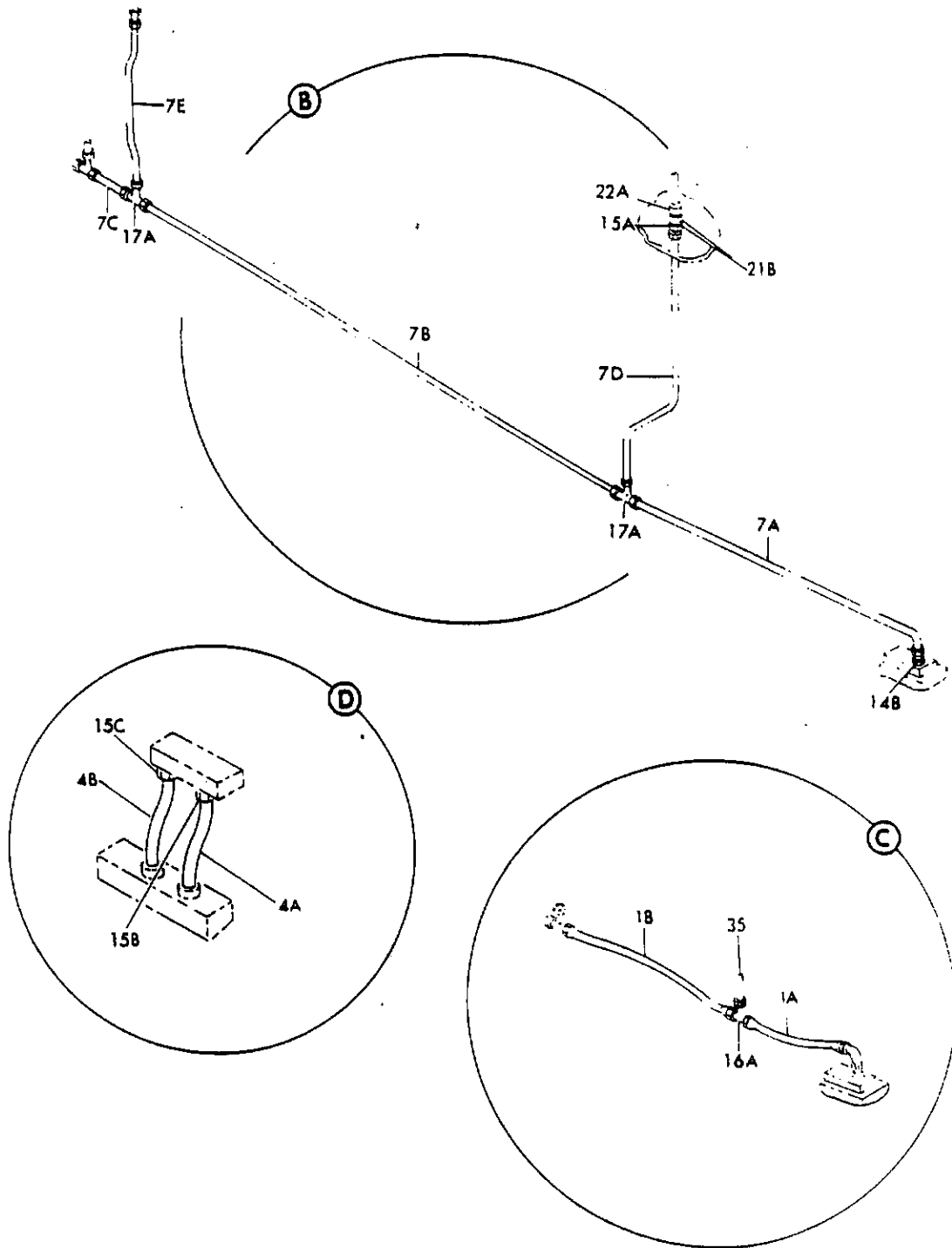
FIGURE 4, WATER SYSTEM INSTL. SECTION 41 FORWARD POTABLE (SHEET 2)
