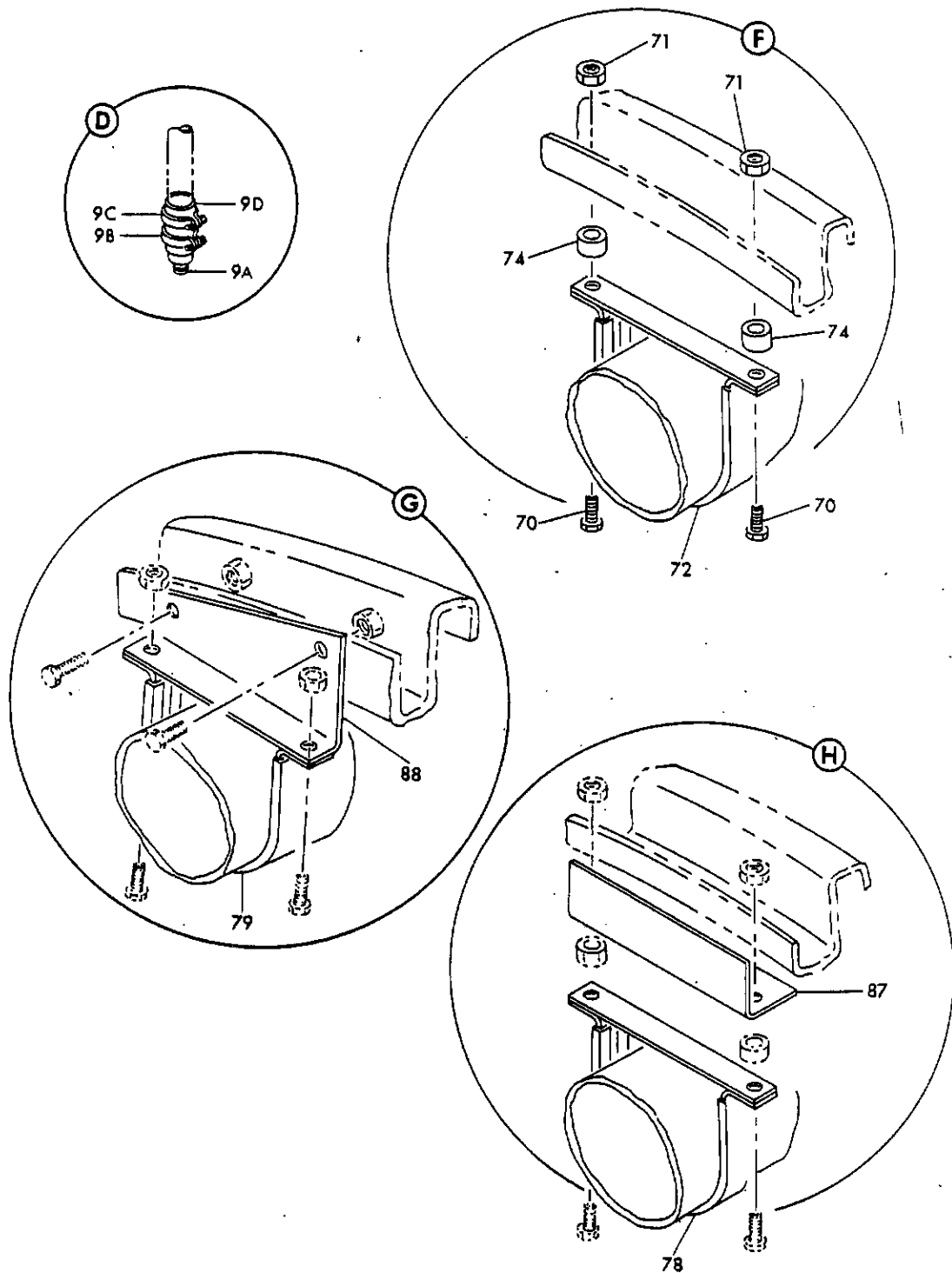
FIGURE 5. VENTILATION SYSTEM INSTL, TOILET AND GALLEY (AFT) (SHEET 2)
