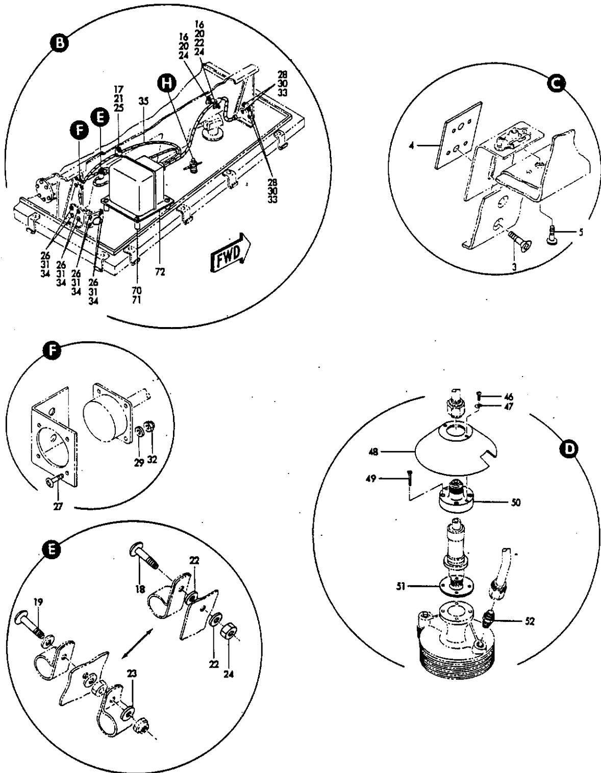
FIGURE 6L. TOILET ASSY, AC FLUSH (SHEET 2)
