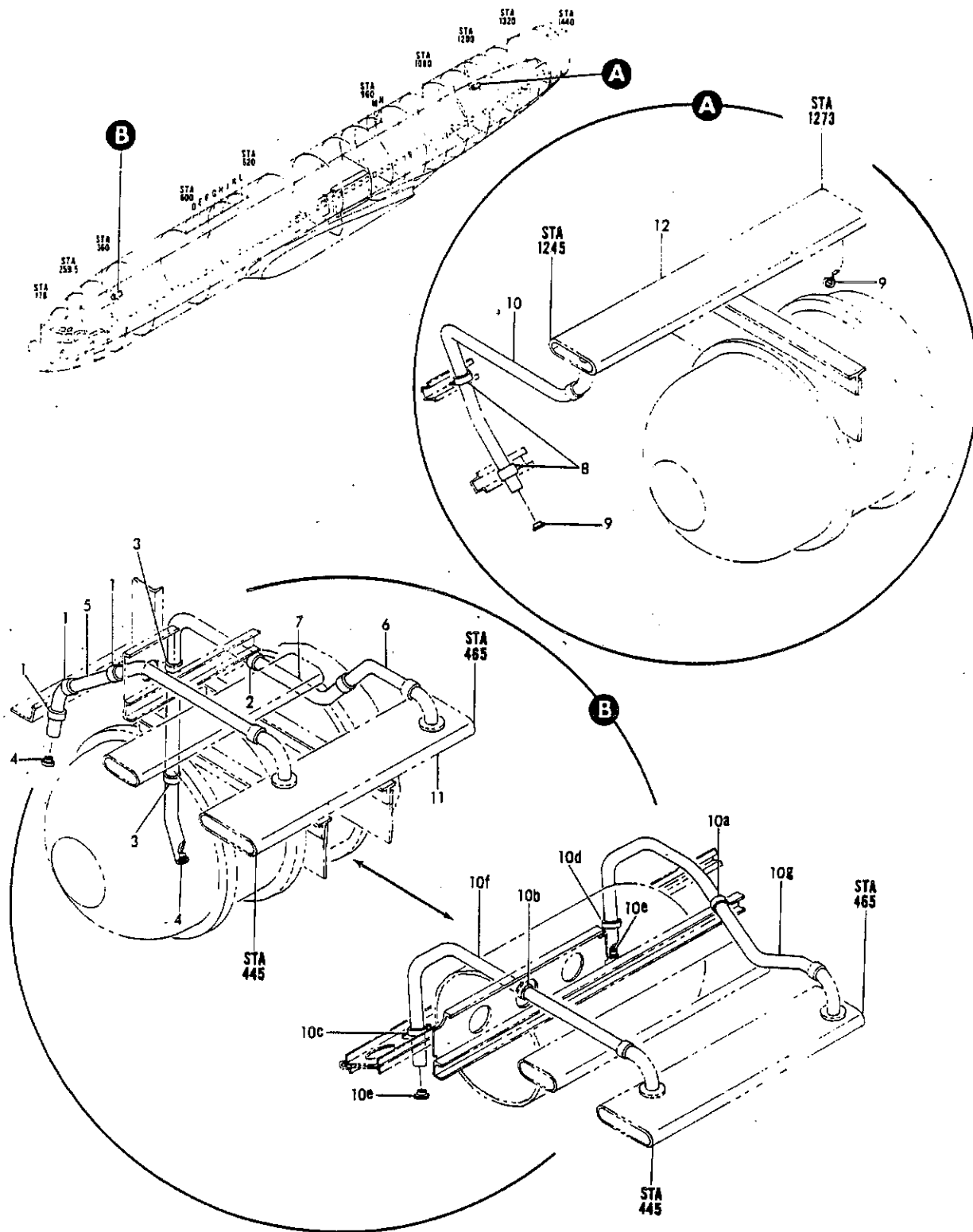
FIGURE 52. DUCT INSTL, FORWARD AND AFT POTABLE WATER TANK HEATING SYSTEM
