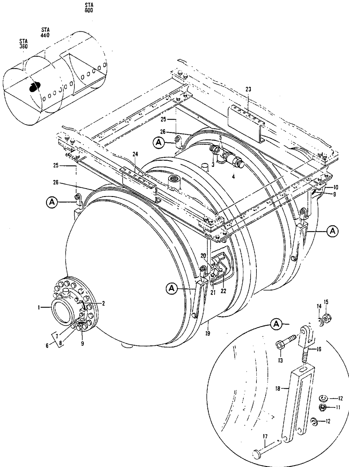
FIGURE 26. TANK INSTL, FORWARD POTABLE WATER SUPPORT INSTL, FORWARD POTABLE WATER TANK (WATER/WASTE ONLY)
