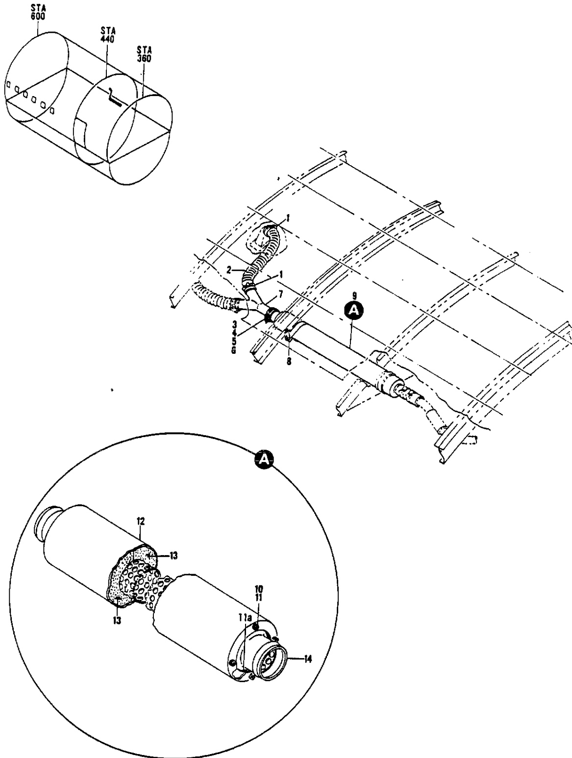
FIGURE 7. MUFFLER INSTL, GALLEY VENTILATION SYSTEM
