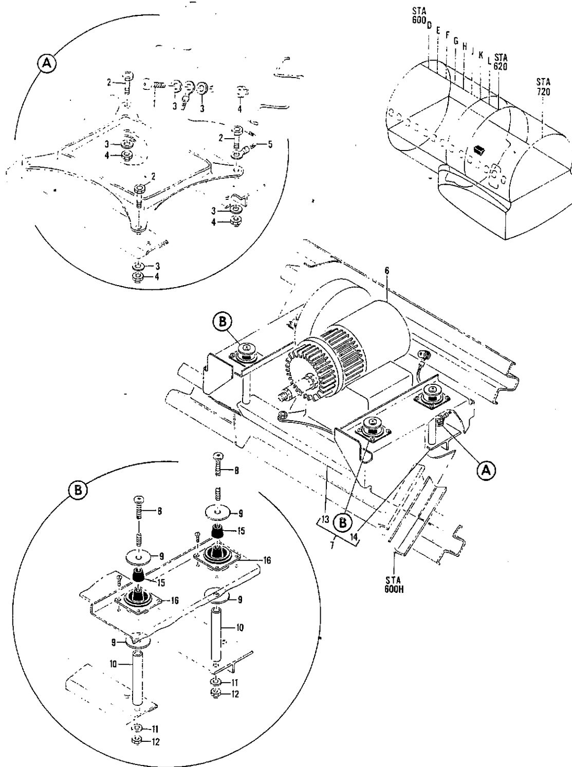
FIGURE 25. COMPRESSOR INSTL, POTABLE WATER SYSTEM (WATER/WASTE ONLY)
