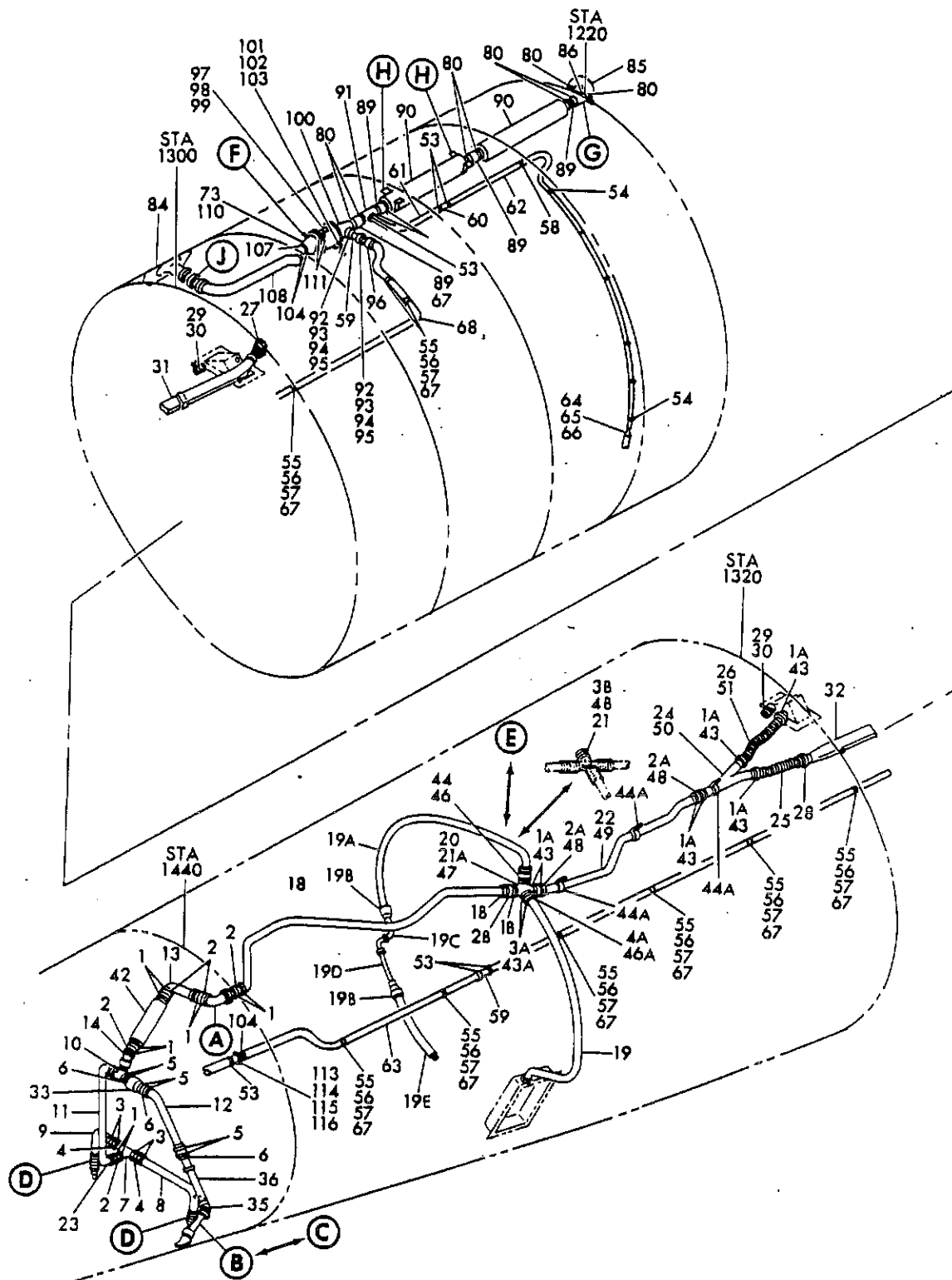
FIGURE 5. VENTILATION SYSTEM INSTL, TOILET AND GALLEY (AFT) (SHEET 1)
