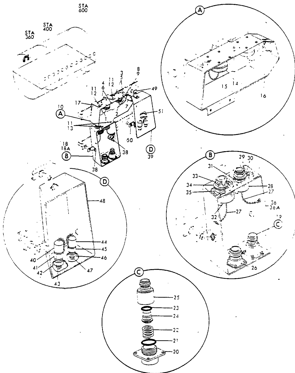
FIGURE 25A. BOX INSTL, GALLEY WATER AND ELECTRICAL
