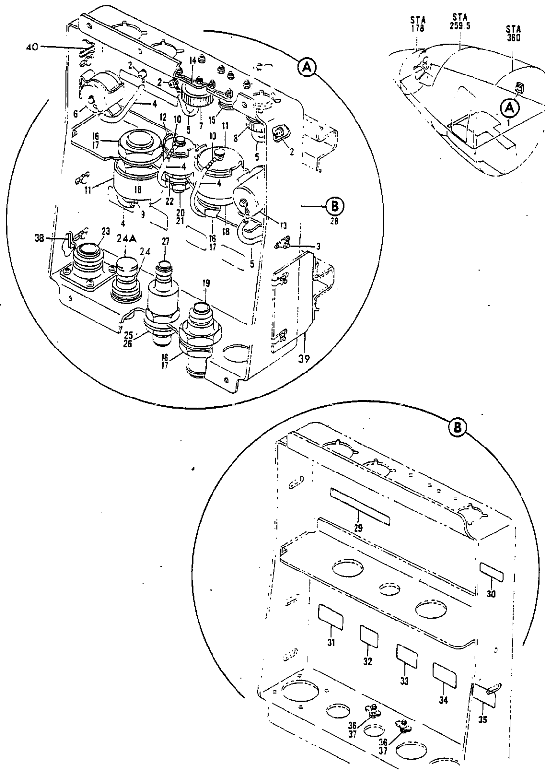
FIGURE 26. BOX INSTL, COMPARTMENT B LAVATORY SERVICES
