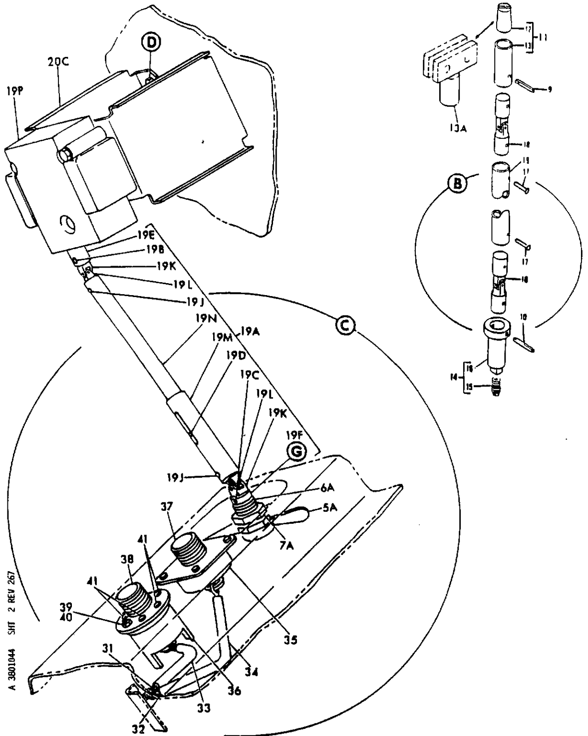
FIGURE 44. VALVE INSTL. AFT PASSENGER WATER FILL AND DRAIN (SHEET 2)
