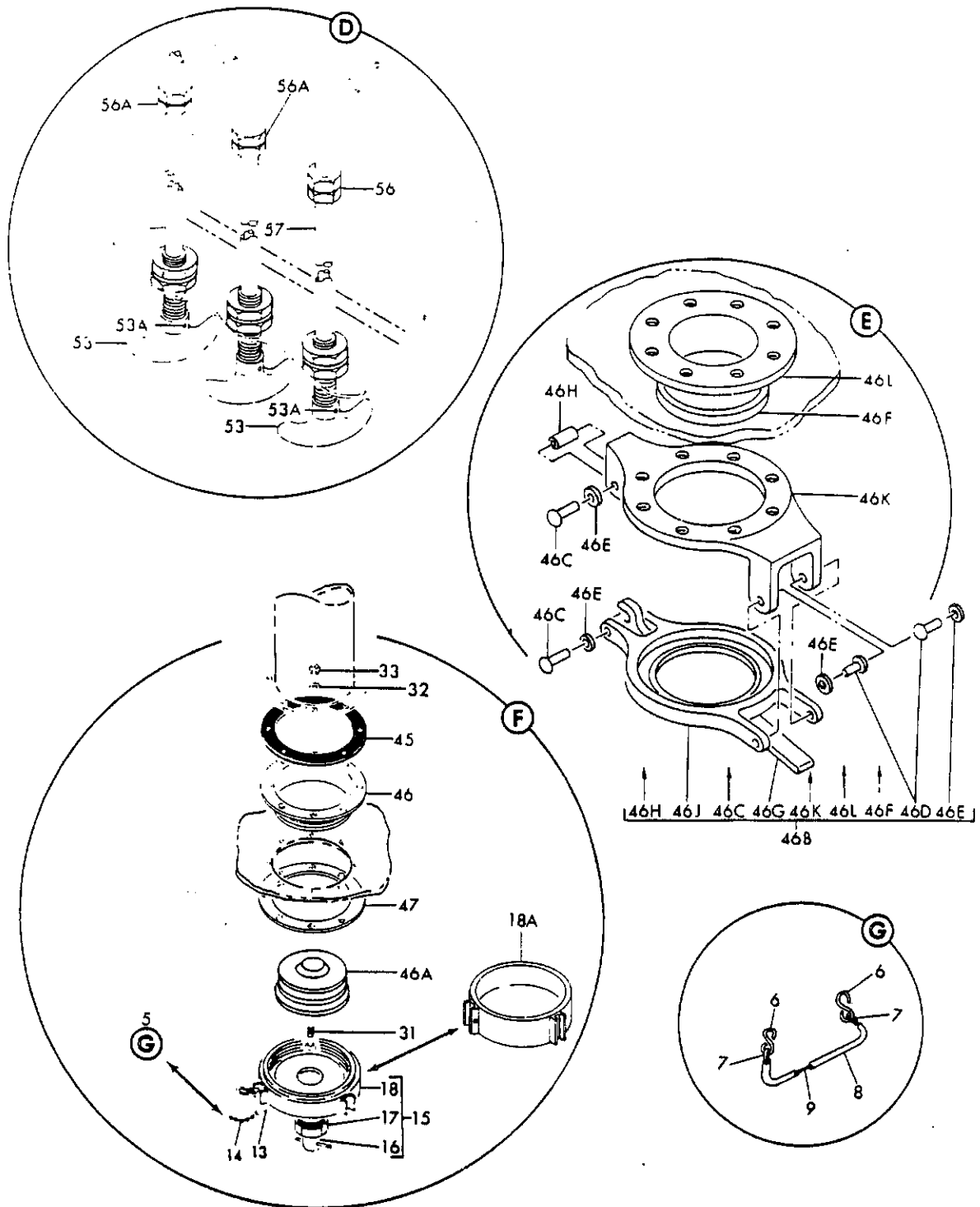
FIGURE 10A. DRAIN INSTL, AFT TOILETS (WATER/WASTE ONLY) (SHEET 2)
