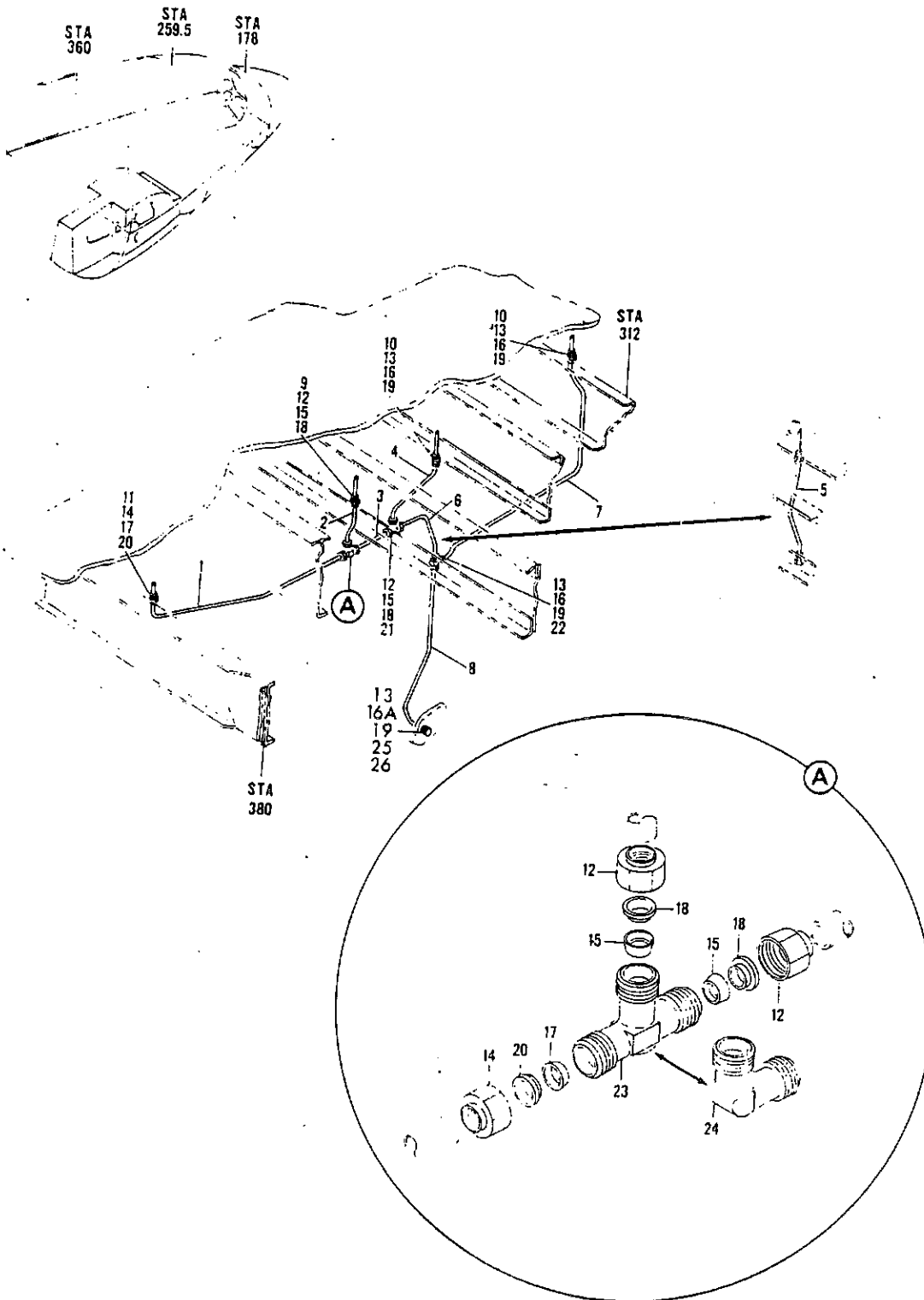
FIGURE 6. DRAIN INSTL, FORWARD TOILET FLOOR
