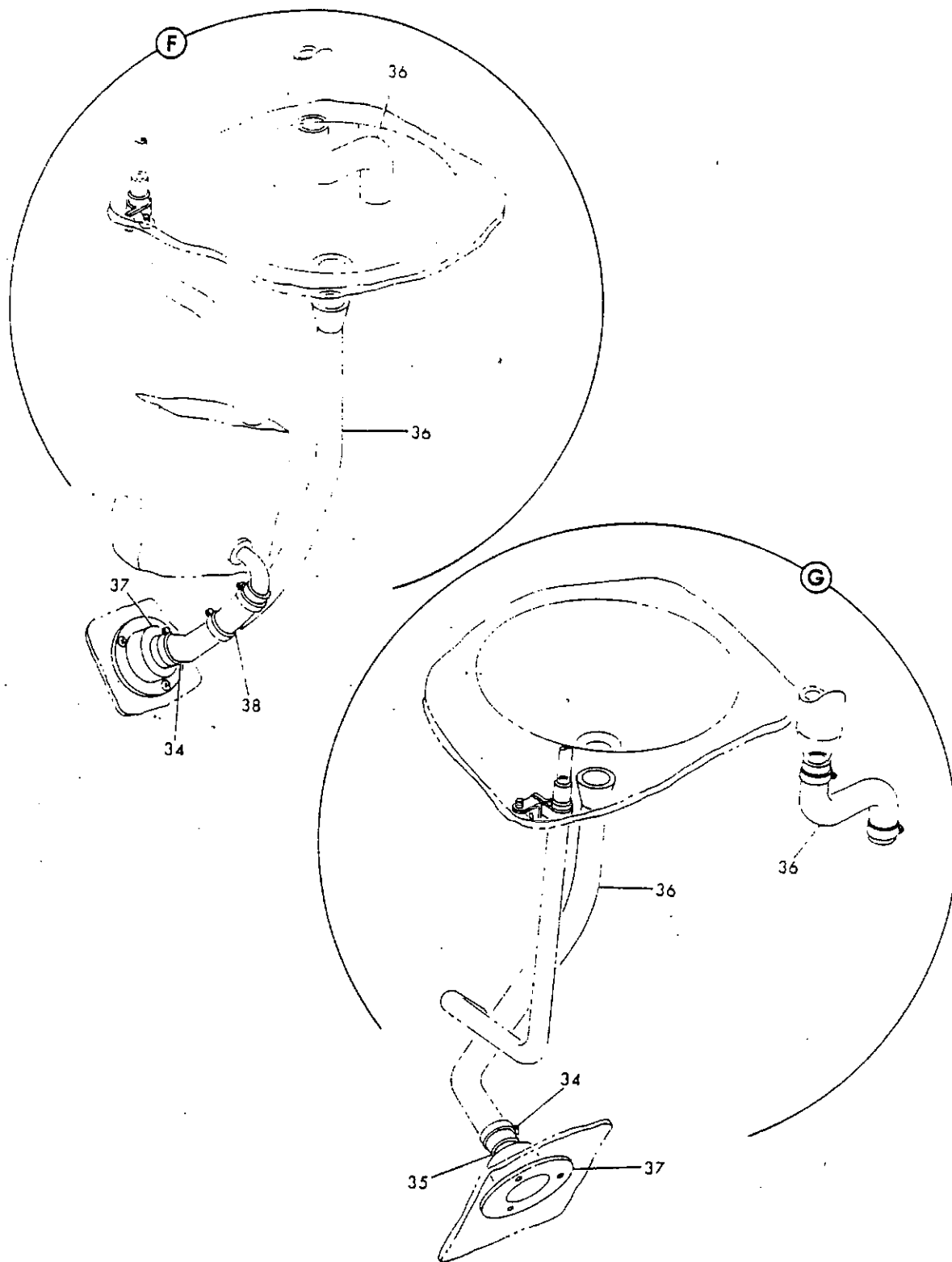
FIGURE 34 LAVATORY INSTL. TOILET C AND D (WATER-WASTE ONLY) (SHEET 3)
