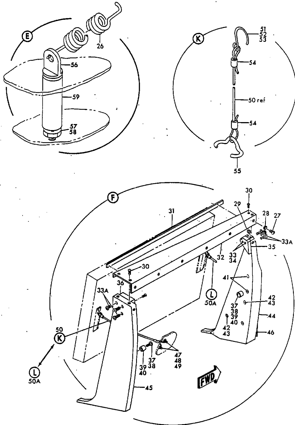
FIGURE 43. TOILET INSTL, FORWARD TOILET COMPARTMENT B (WATER/WASTE ONLY) (SHEET 3)
