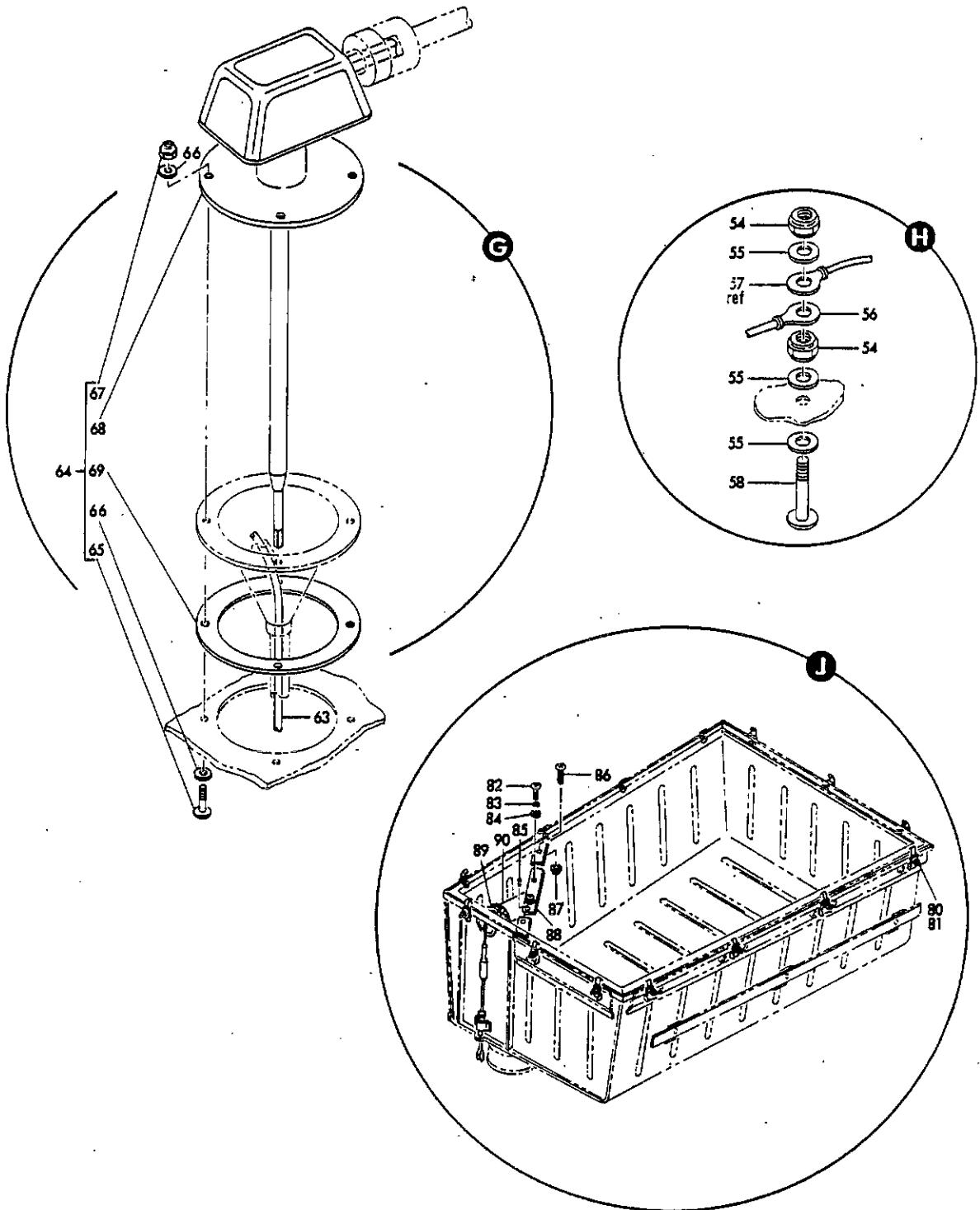
FIGURE 61. TOILET ASSY, AC FLUSH (SHEET 3)
