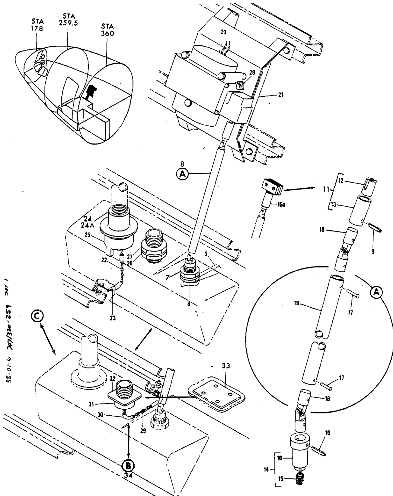
FIGURE 6. VALVE INSTL, FORWARD PASSENGER WATER FILL AND DRAIN (WATER/WASTE ONLY) (SHEET 1)
