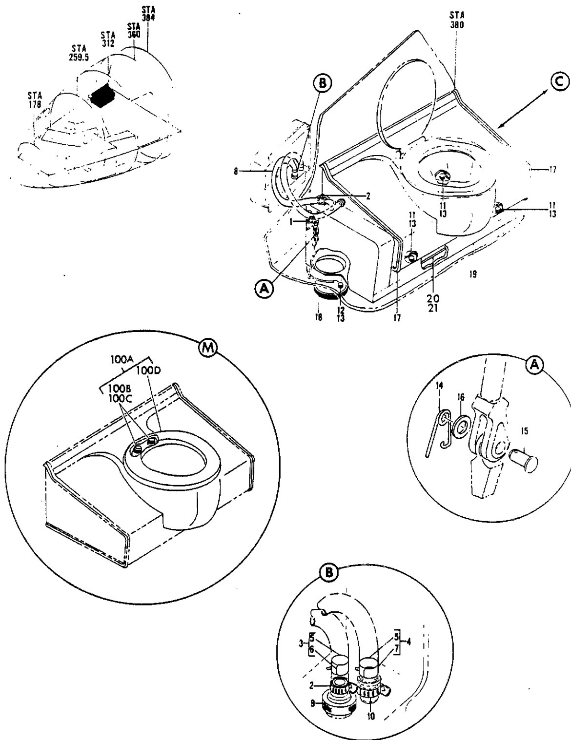
FIGURE 43. TOILET INSTL, FORWARD TOILET COMPARTMENT B (WATER WASTE ONLY) (SHEET 1)
