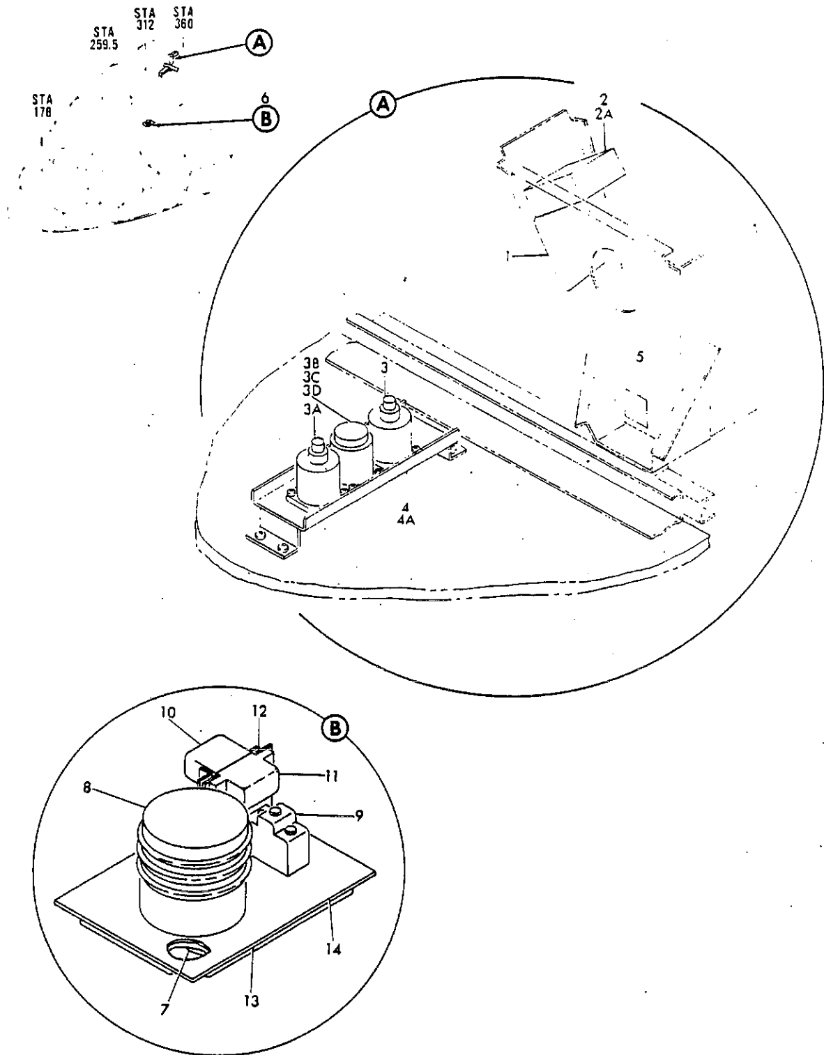
FIGURE 7. QUANTITY INDICATOR AND ISOLATION SWITCH INSTL, POTABLE WATER SYSTEM
