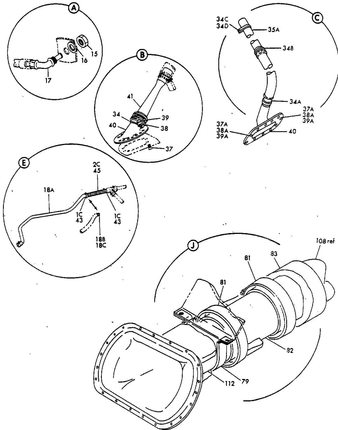
FIGURE 5. VENTILATION SYSTEM INSTL, TOILET AND GALLEY (AFT) (SHEET 3)
