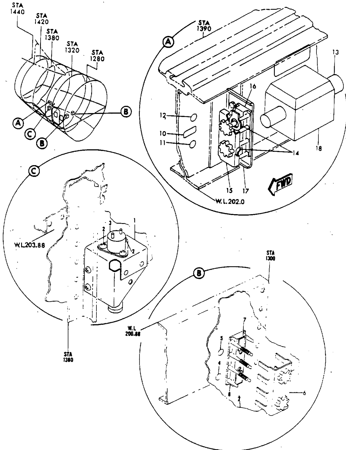
SWITCH INSTL, STATION 1380 POTABLE WATER HEATERS THERMO STRIP INSTL, STATION 1300 POTABLE WATER HEATERS TERMINAL FIGURE 53. SWITCH AND TERMINAL INSTL, STATION 1390 POTABLE WATER HEATERS THERMO
