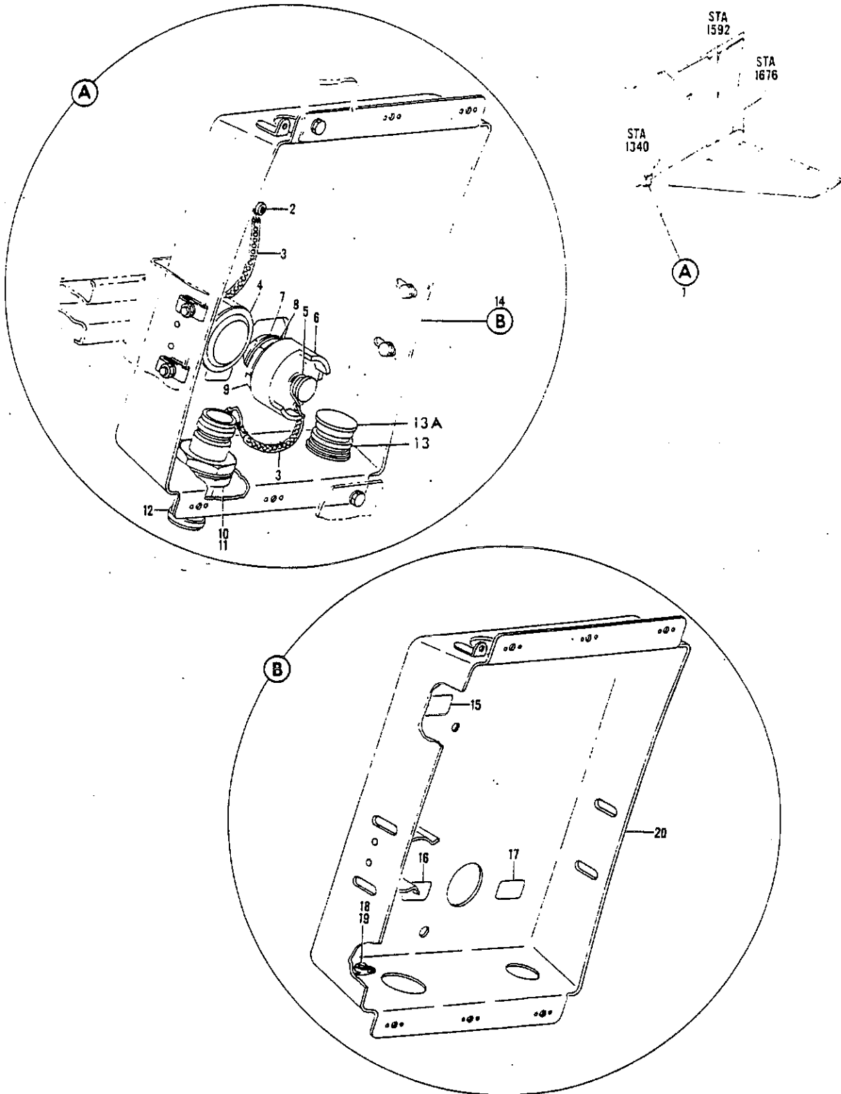
FIGURE 27A. BOX INSTL, COMPARTMENT E LAVATORY SERVICES
