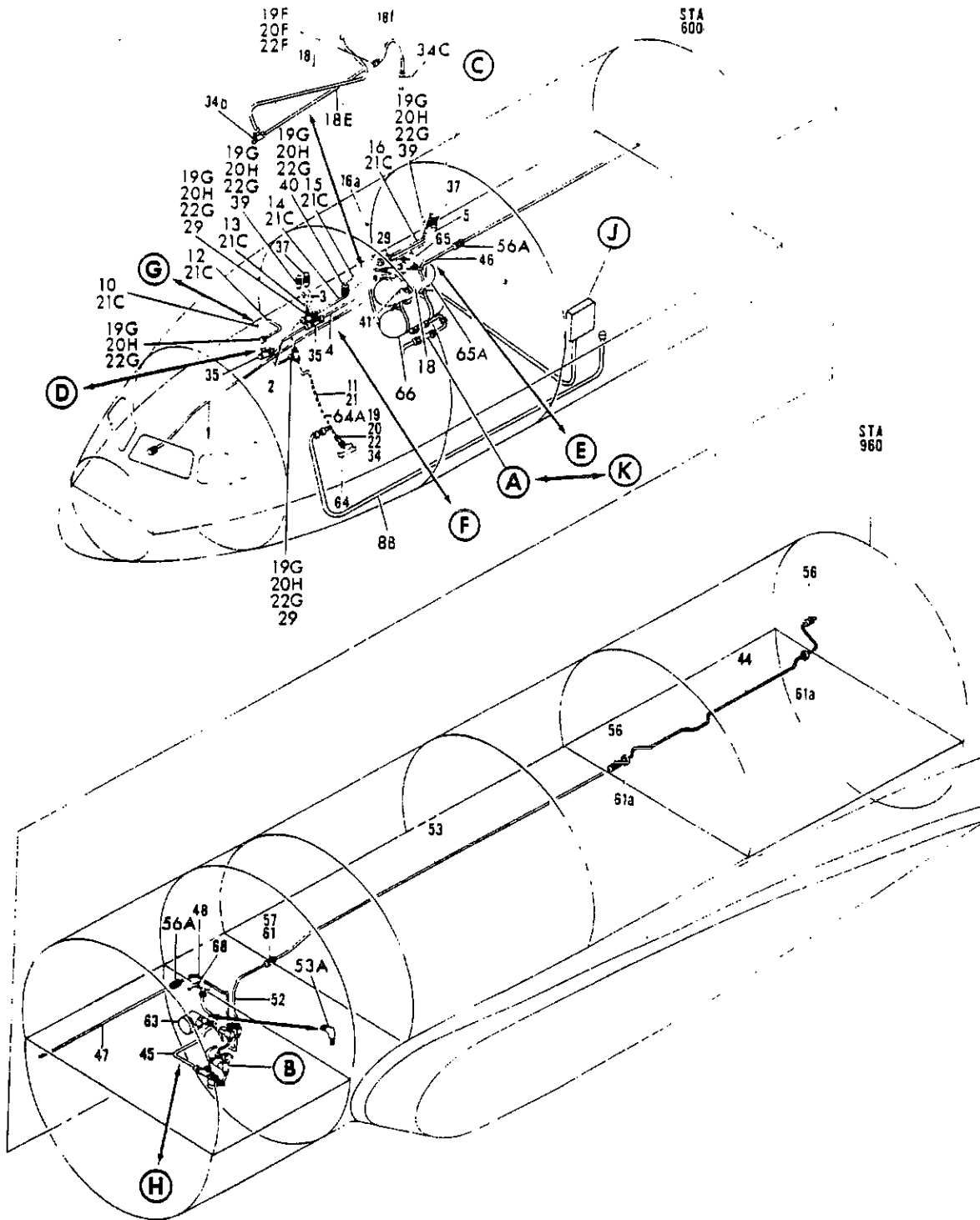
FIGURE 20. WATER SYSTEM INSTL, SECTION 43 FORWARD PORTABLE (SHEET 1)
