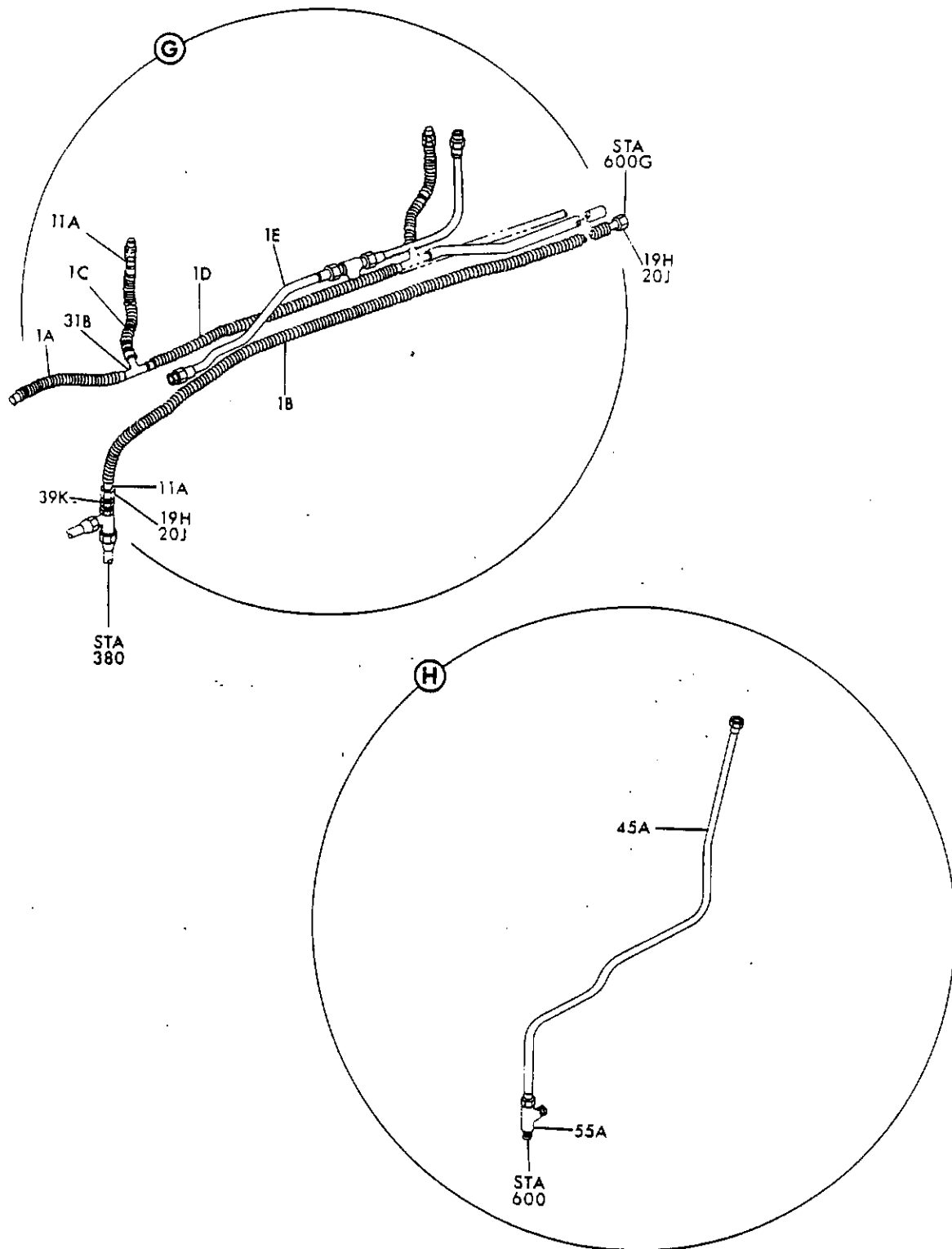
FIGURE 20. WATER SYSTEM INSTL, SECTION 43 FORWARD POTABLE (SHEET 4)
