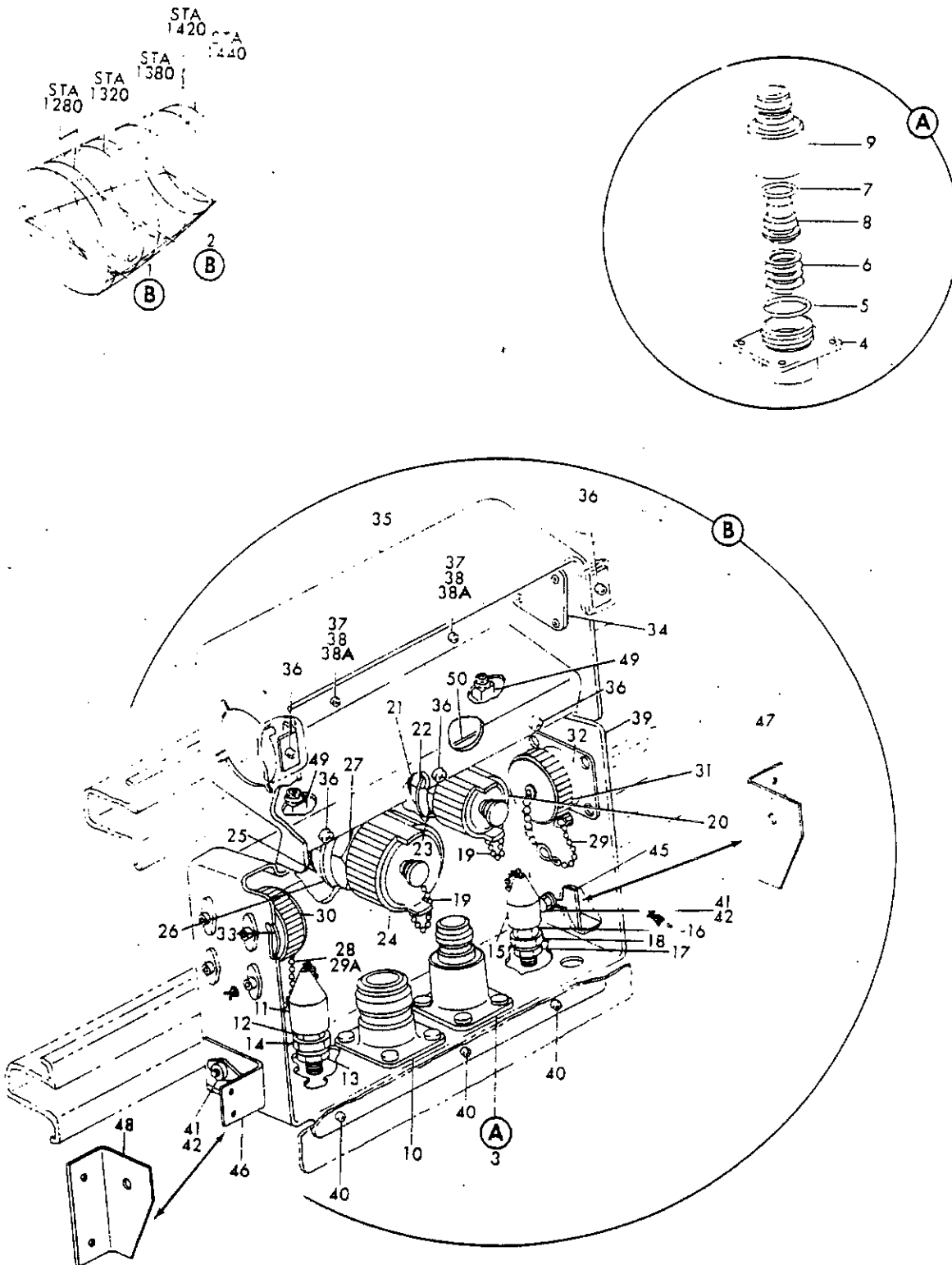
FIGURE 25D. BOX INSTL. GALLEY WATER AND ELECTRICAL SUPPLY
