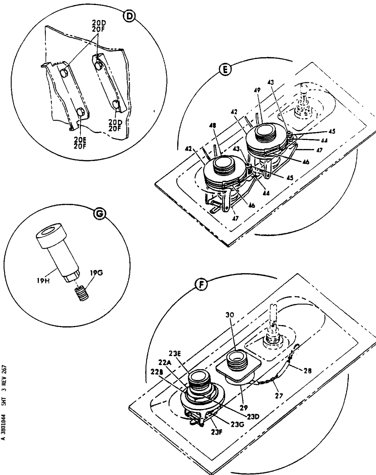
FIGURE 44. VALVE INSTL, AFT PASSENGER WATER FILL AND DRAIN (SHEET 3)
