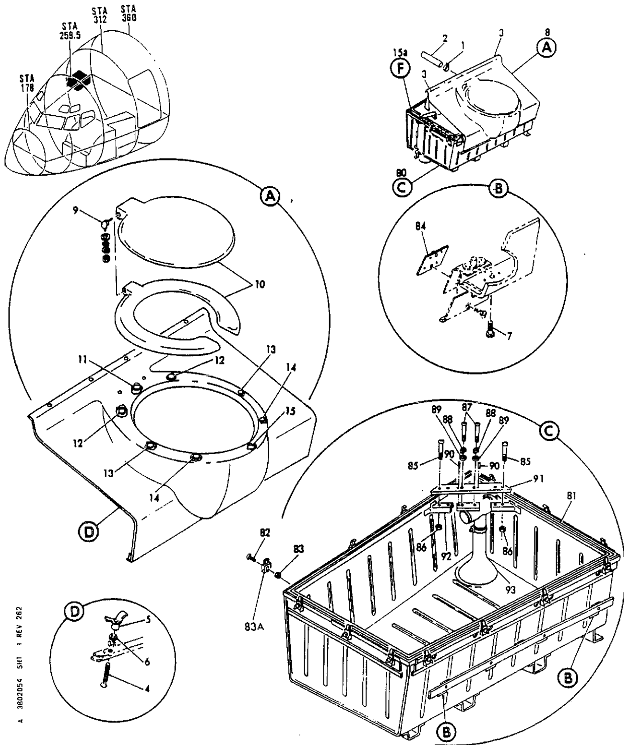
FIGURE 54. TOILET ASSY, DC FLUSH (SHEET 1)
