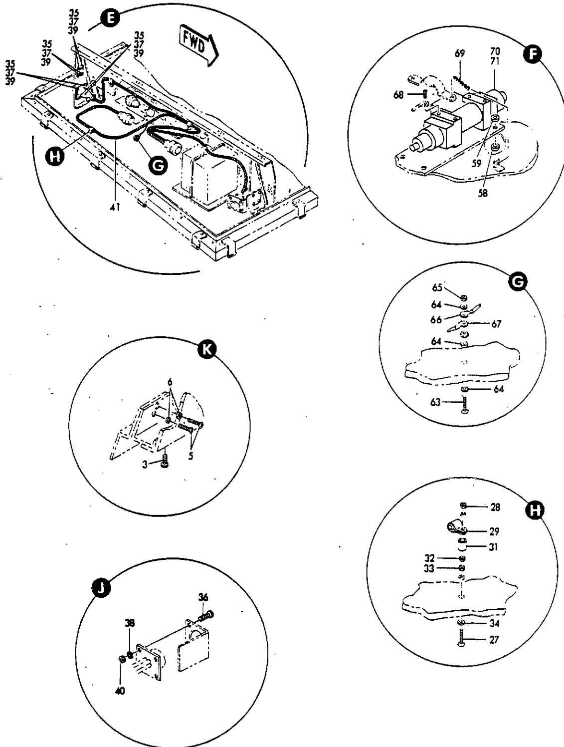
FIGURE 64 TOILET ASSY, AC FLUSH (SHEET 3)
