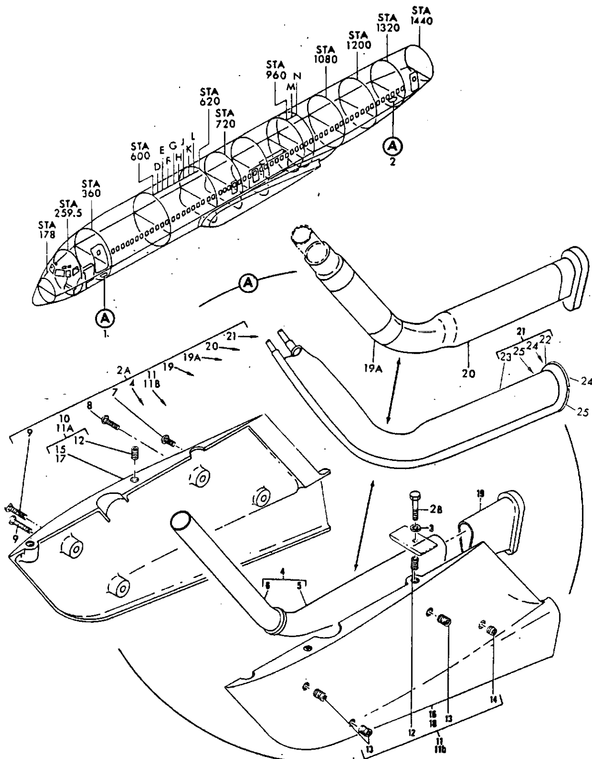
FIGURE 41. MAST INSTALLATION-FORWARD WASTE WATER DRAIN
