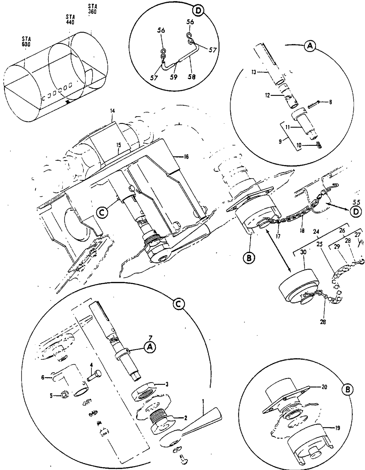
FIGURE 23. VALVE INSTL, FORWARD POTABLE WATER SYSTEM DRAIN (WATER/WASTE ONLY)
