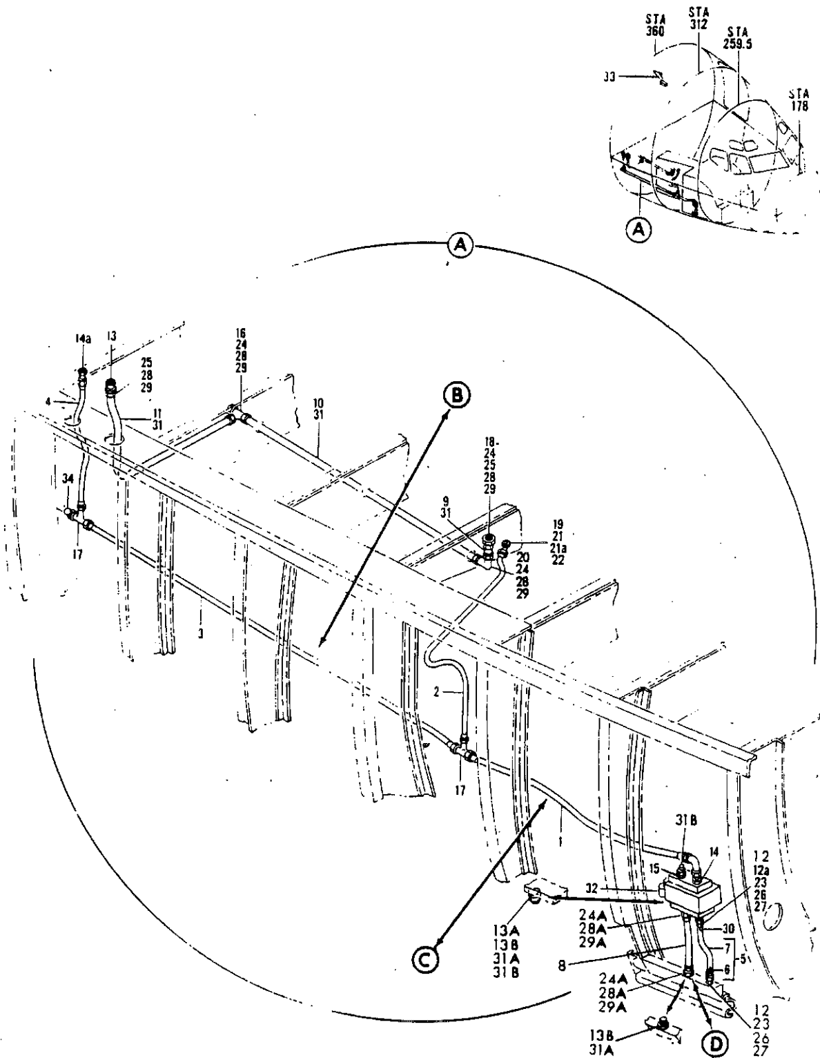
FIGURE 4. WATER SYSTEM INSTL, SECTION 41 FORWARD POTABLE (SHEET 1)
