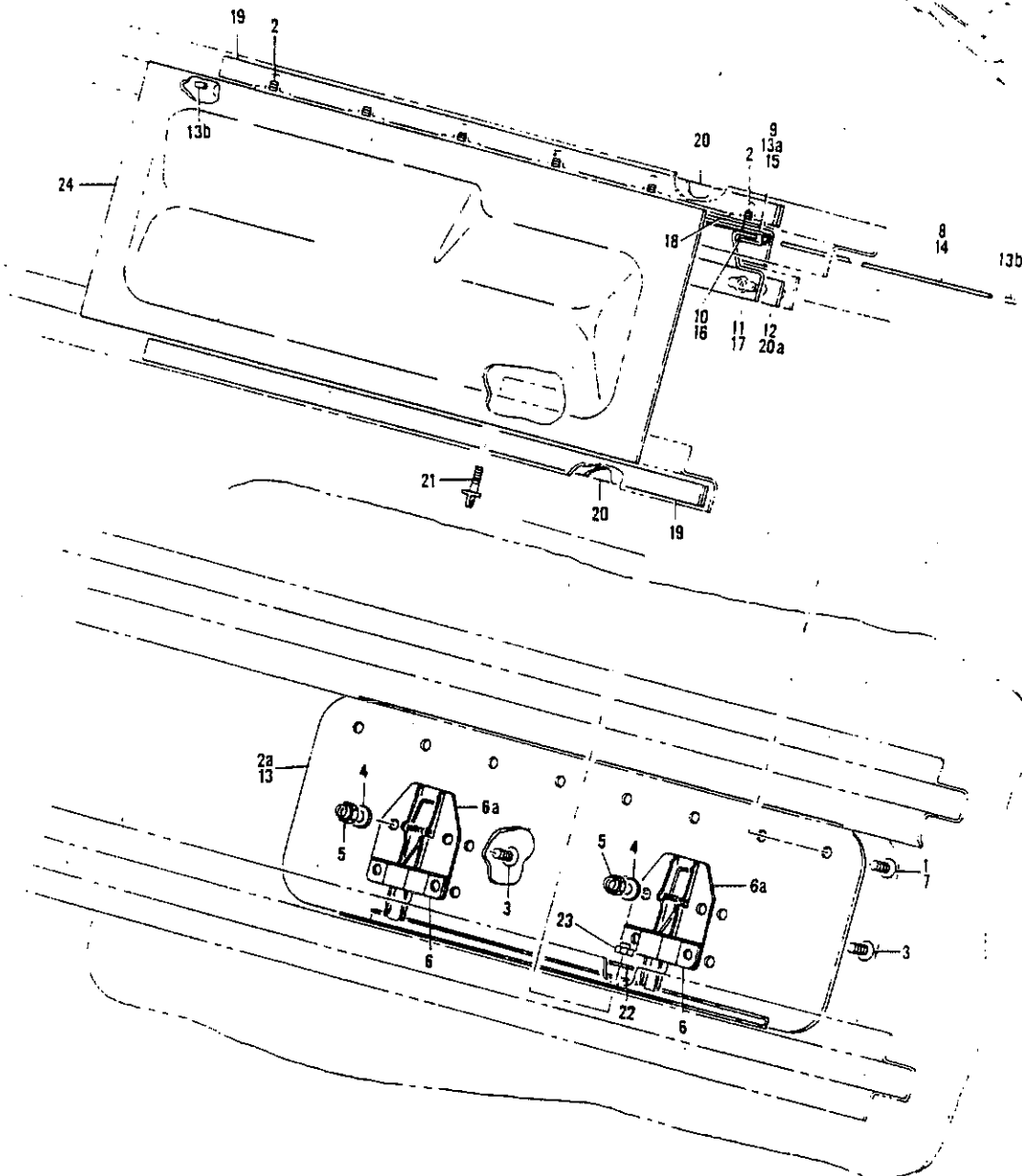
FIGURE 50. PAN AND DOOR INSTL. STATION 259.5 TO 277 FORWARD PASSENGER WATER
