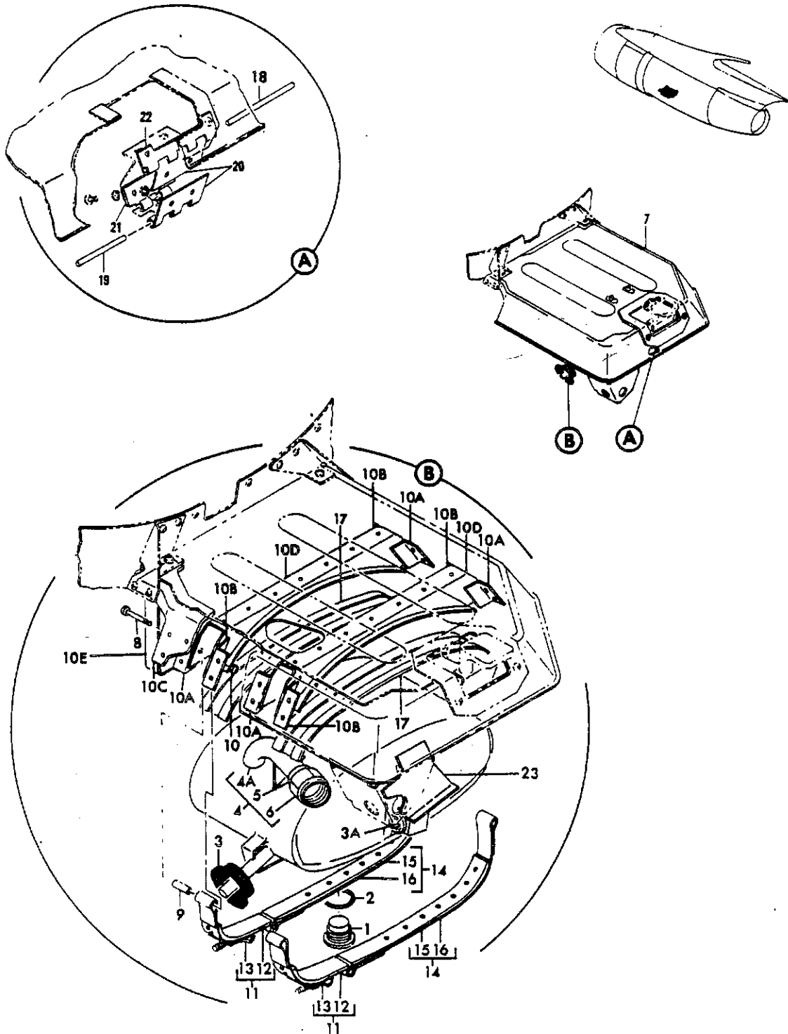
FIGURE 5. TANK INSTL, ENGINE COMBUSTION CHAMBER DRAIN
