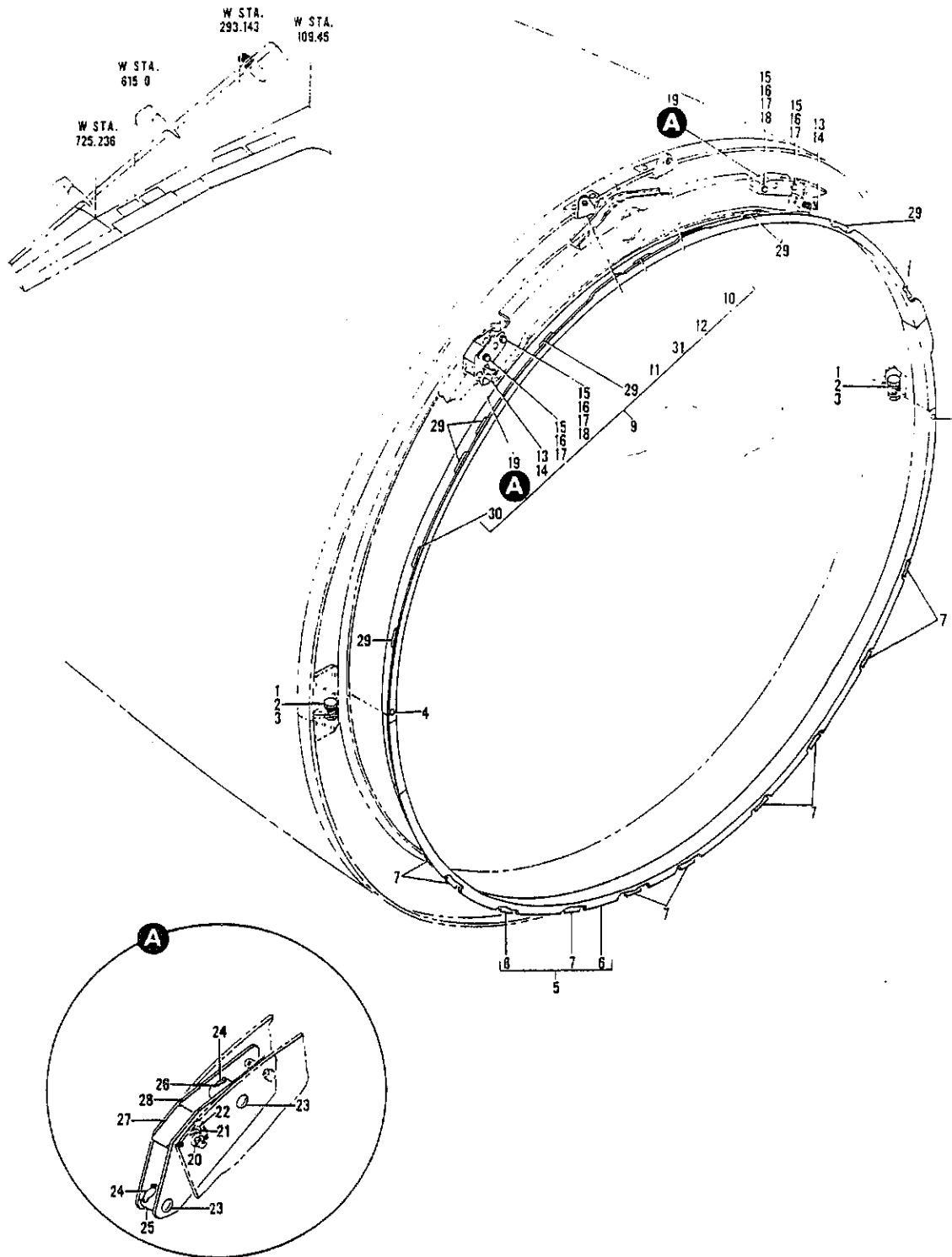
FIGURE 17. COWL ASSY. FAN ENGINE TRANSPORT KIT NOSE
