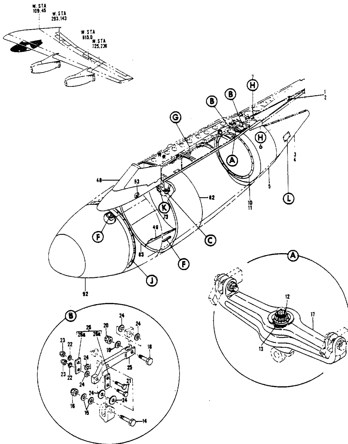
FIGURE 5. KIT AND BUILD-UP INSTL, FAN ENGINE TRANSPORT KIT BEAM TO ENGINE (SHEET 1)
