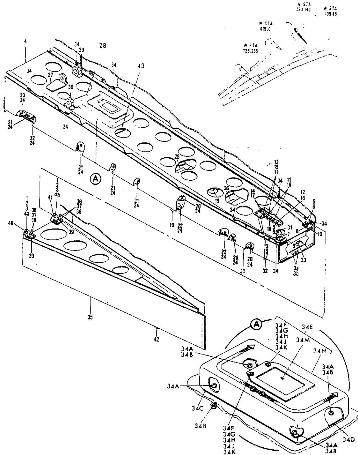
FIGURE 14. BEAM INSTL. SPARE ENGINE TRANSPORT KIT
