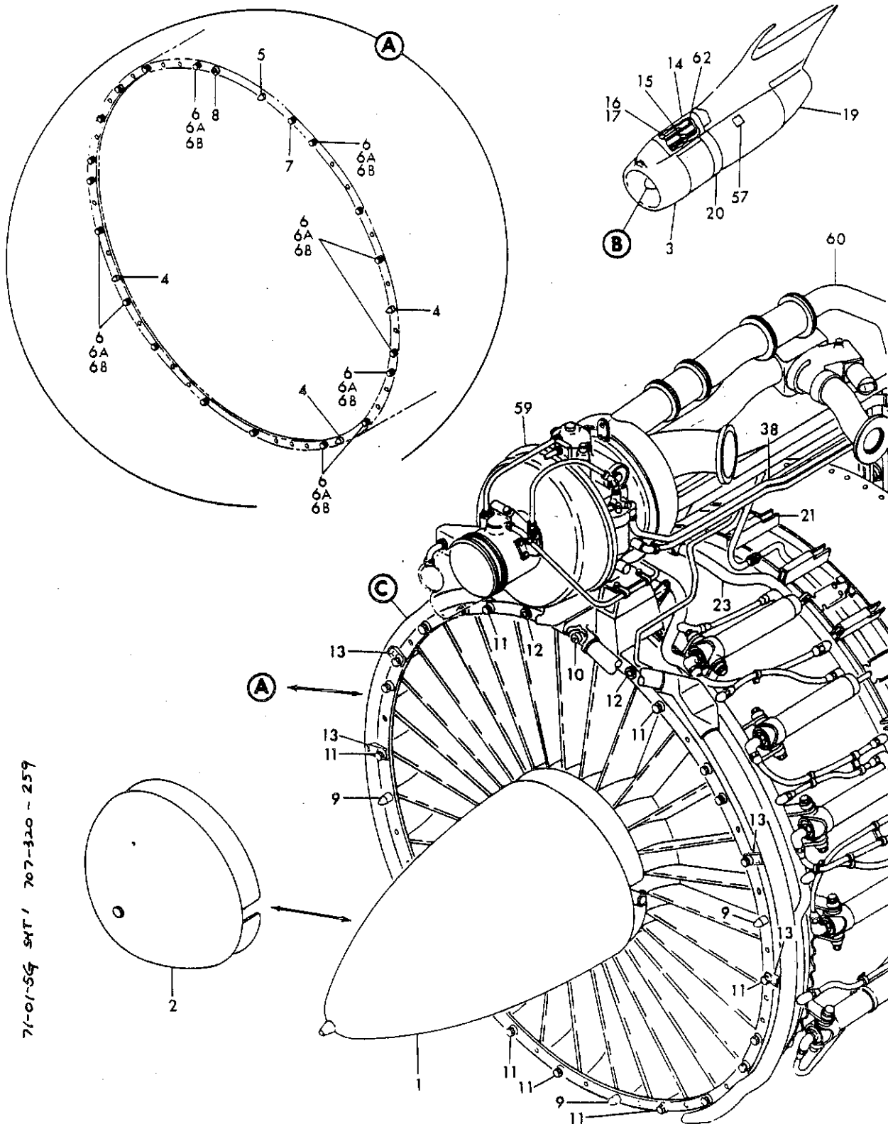
FIGURE 5G. POWER PACK ASSY, FAN ENGINE (SHEET 1)
