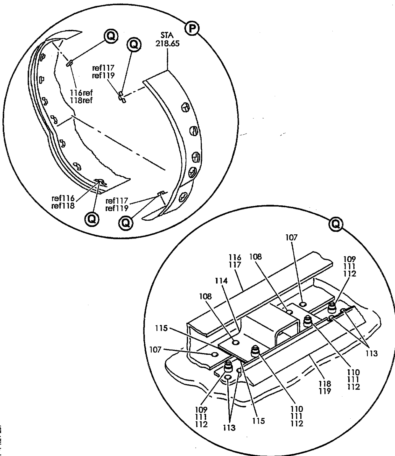
FIGURE 12. PANEL ASSY, ENGINE MACELLE COWL (SHEET 4)
