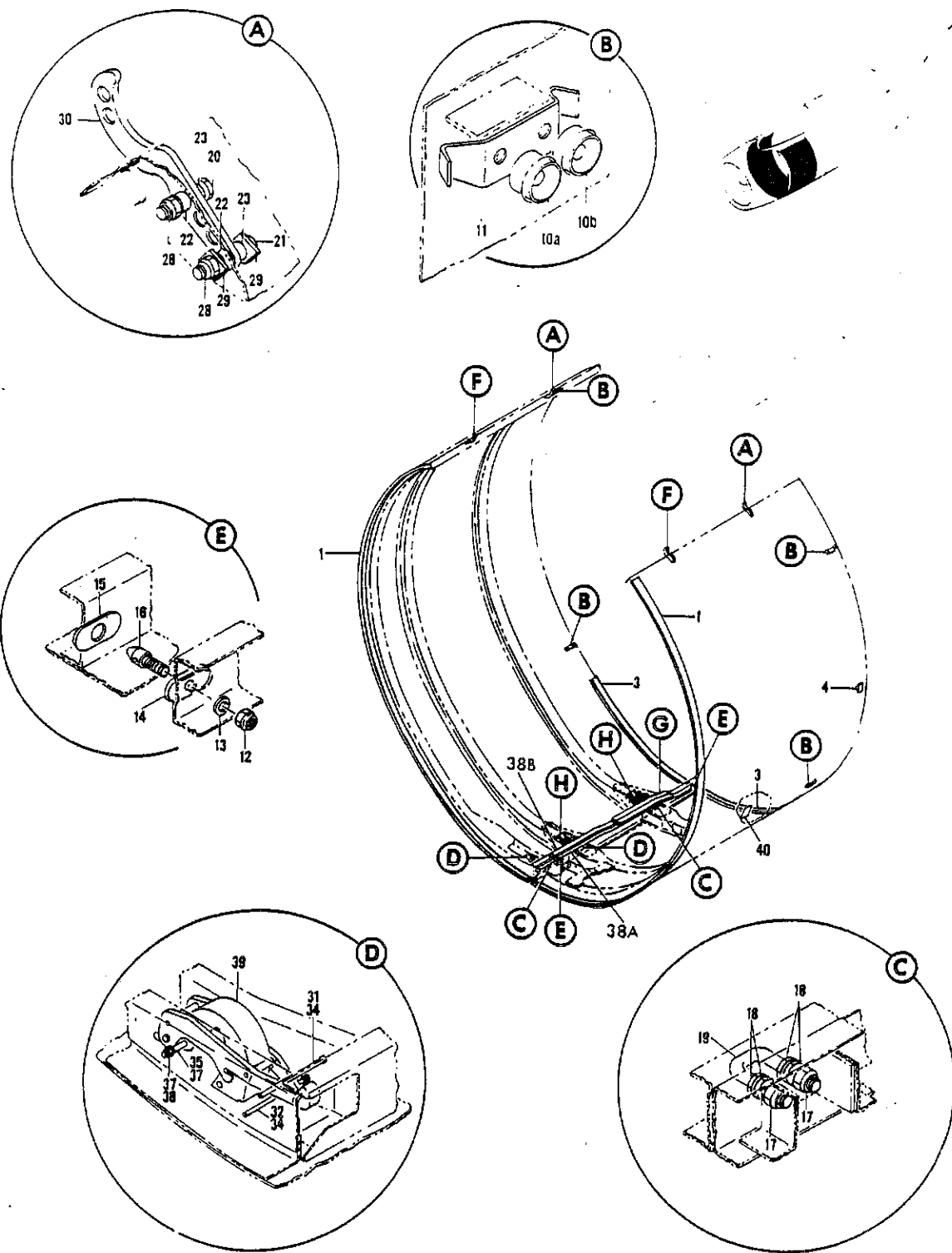
FIGURE 19. PANEL ASSY, ENGINE NACELLE FAN SECTION SIDE COWL (SHEET 1)
