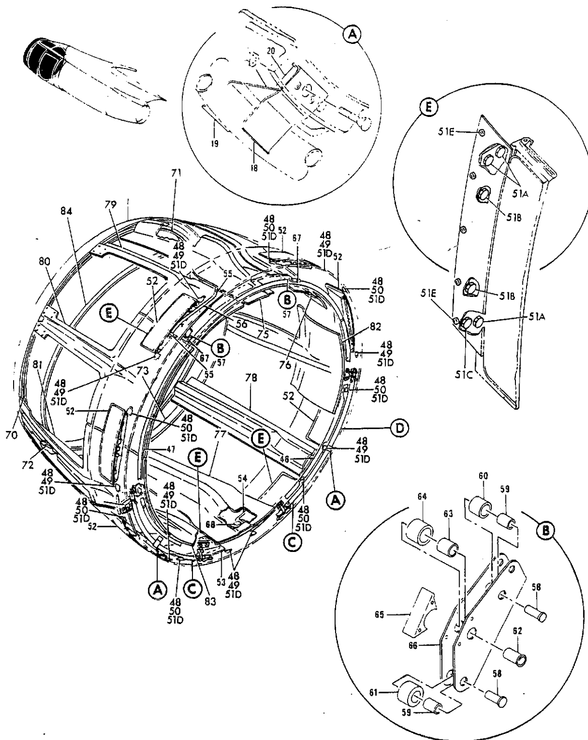
FIGURE 24A. COWL ASSY, LARGE SECONDARY AIR INLET DOORS NOSE (POWER PLANT-GENERAL ONLY) (SHEET 1)
