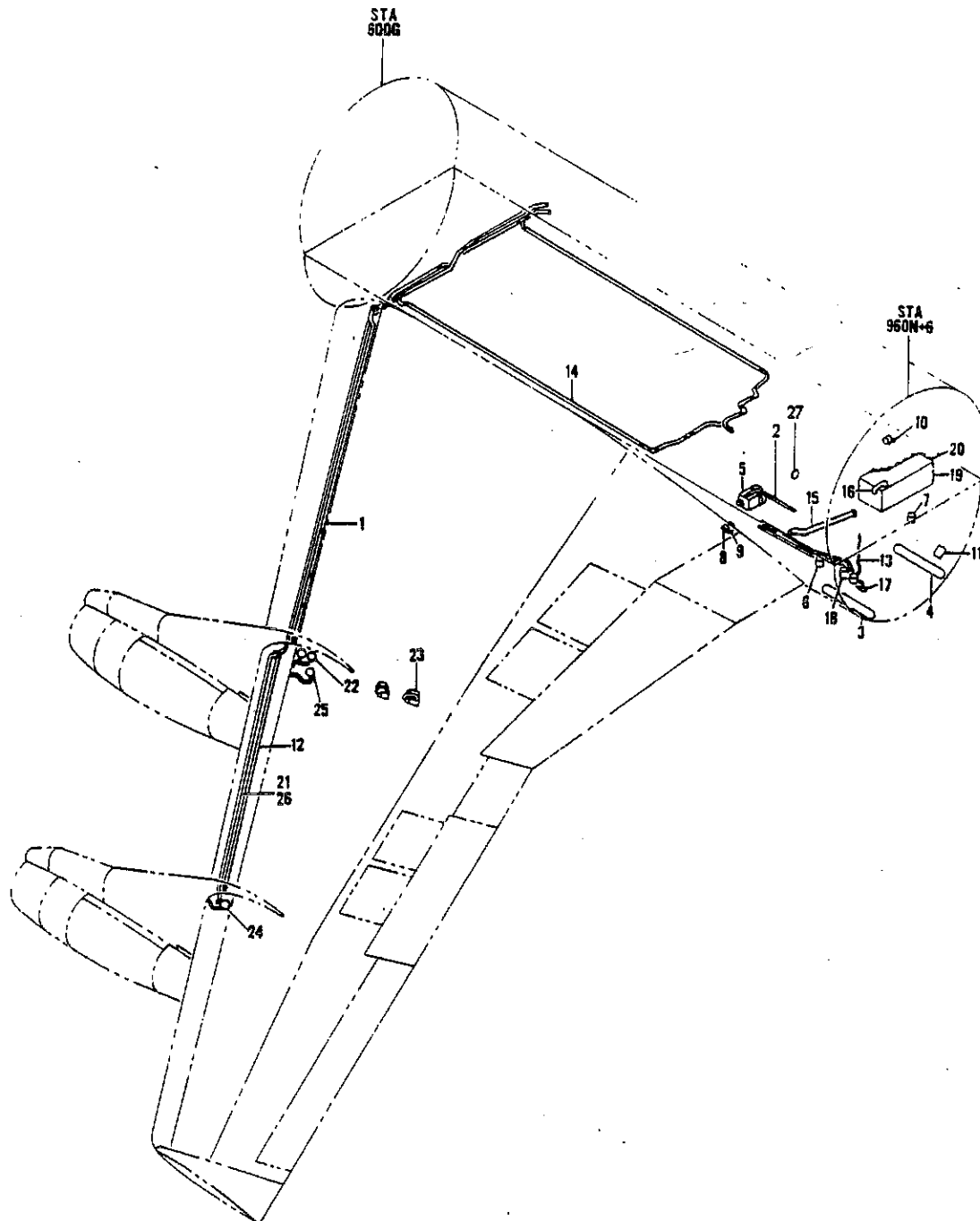
FIGURE 1. EQUIPMENT INSTL, WING AND BODY POWER PLANT
