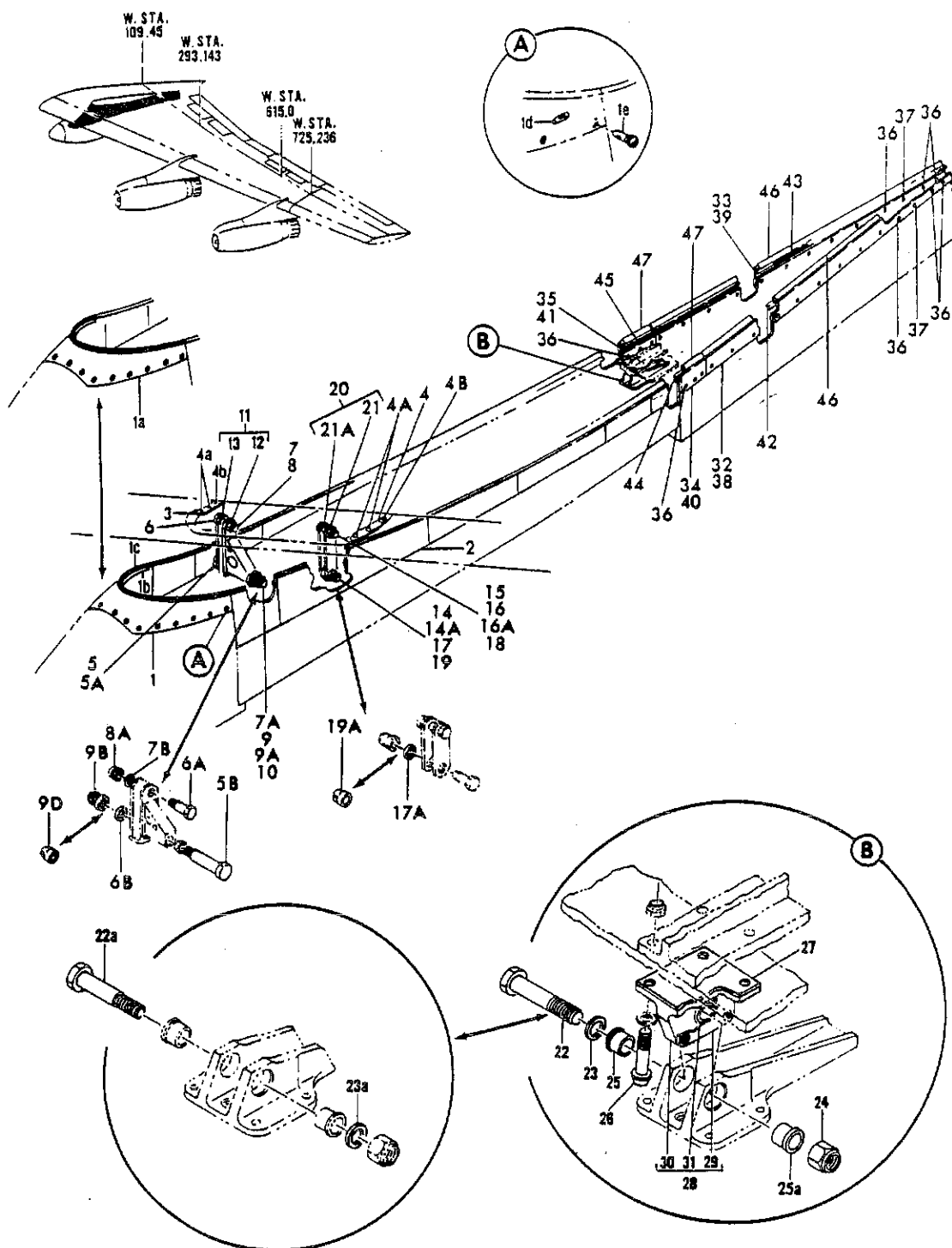
FIGURE 4. KIT, 320/420 SPARE ENGINE TRANSPORT BEAM TO WING FITTINGS AND FAIRINGS
