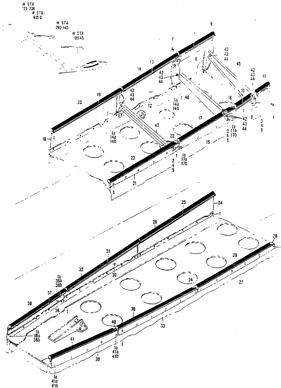
FIGURE 12. FAIRING INSTL. 707/320 SPARE ENGINE KIT BEAM TO WING
