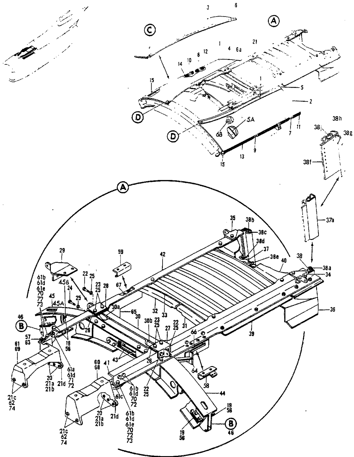
FIGURE 21. PANEL INSTL, FAN ENGINE FORWARD REVERSER SLOT SEAL INSTALLATION (ENGINE NO. 1) (SHEET 1)
