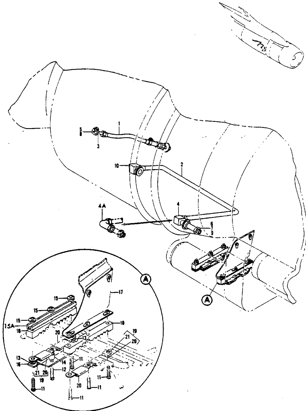
FIGURE 2. DRAIN INSTL, FAN ENGINE (POWER PLANT-GENERAL ONLY)
