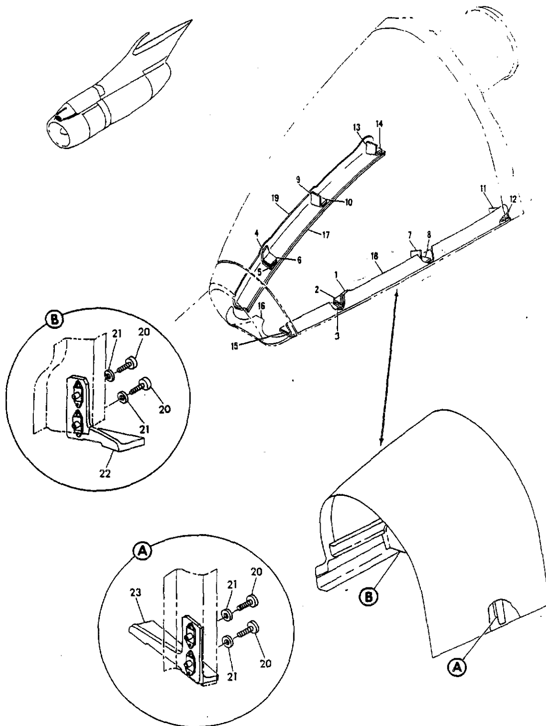
FIGURE 8. FAIRING ASSY, TURBOCOMPRESSOR INLET (ENGINES NO.2,3 AND 4) (POWER PLANT-GENERAL ONLY)
