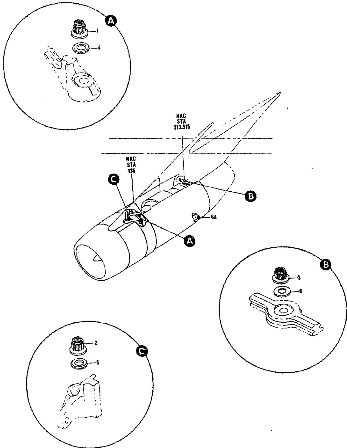
FIGURE 3. POWER PLANT INSTL
