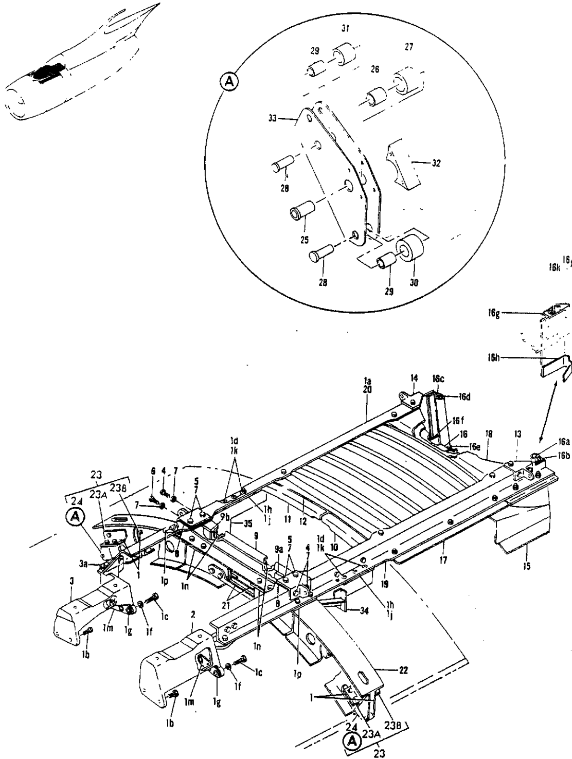
FIGURE 22. SEAL INSTL, FAN ENGINE FORWARD REVERSER SLOT (NEUTRAL)
