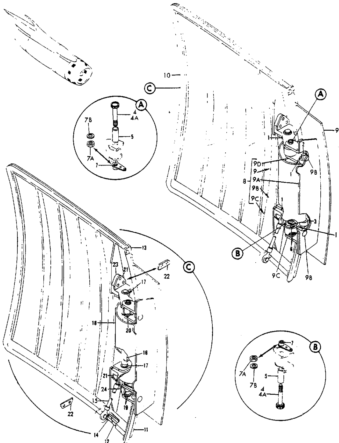
FIGURE 26. DOOR ASSY, NOSE COWL SECONDARY AIR INLET
