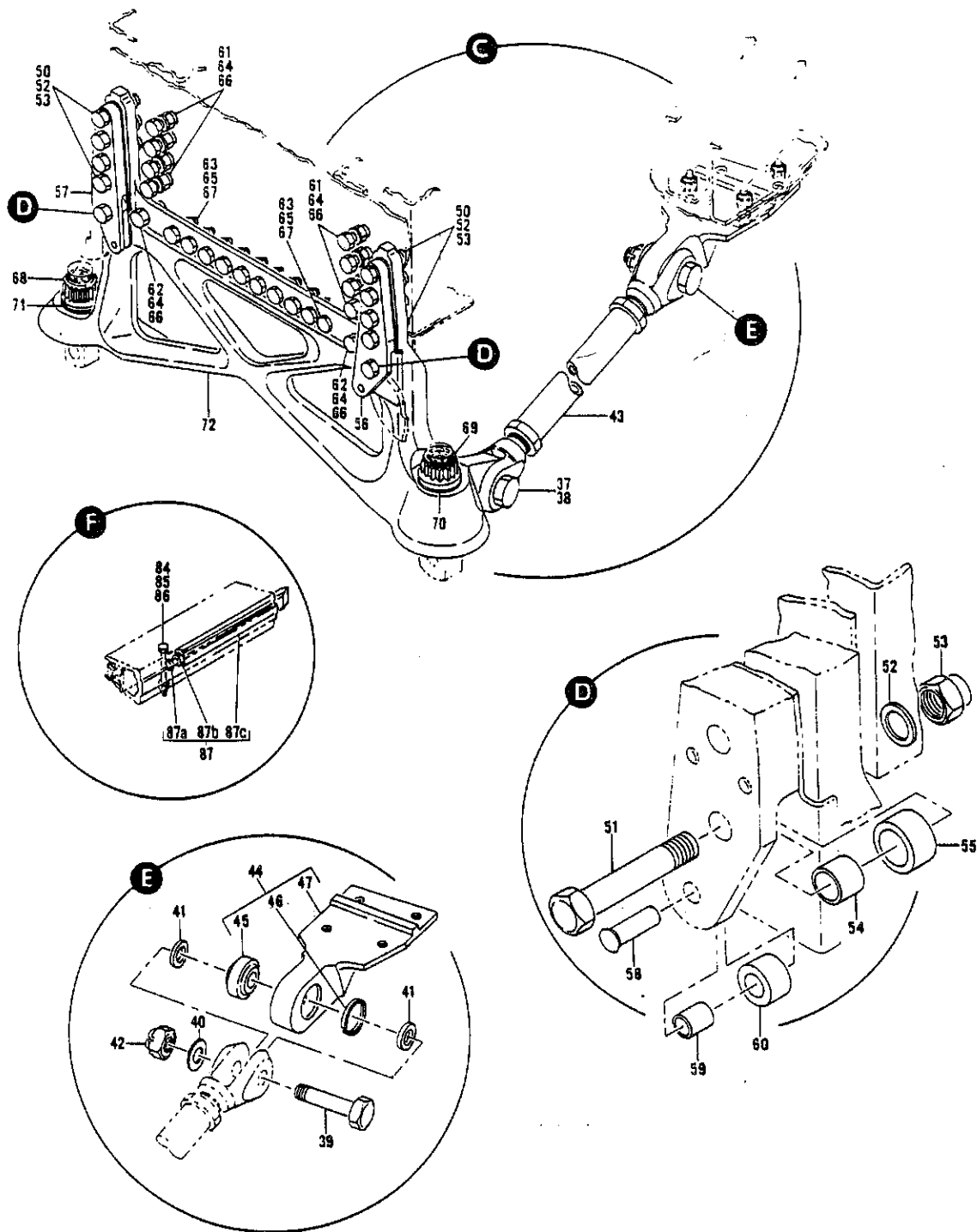
FIGURE 5. KIT AND BUILD-UP INSTL. FAN ENGINE TRANSPORT KIT BEAM TO ENGINE (SHEET 2)
