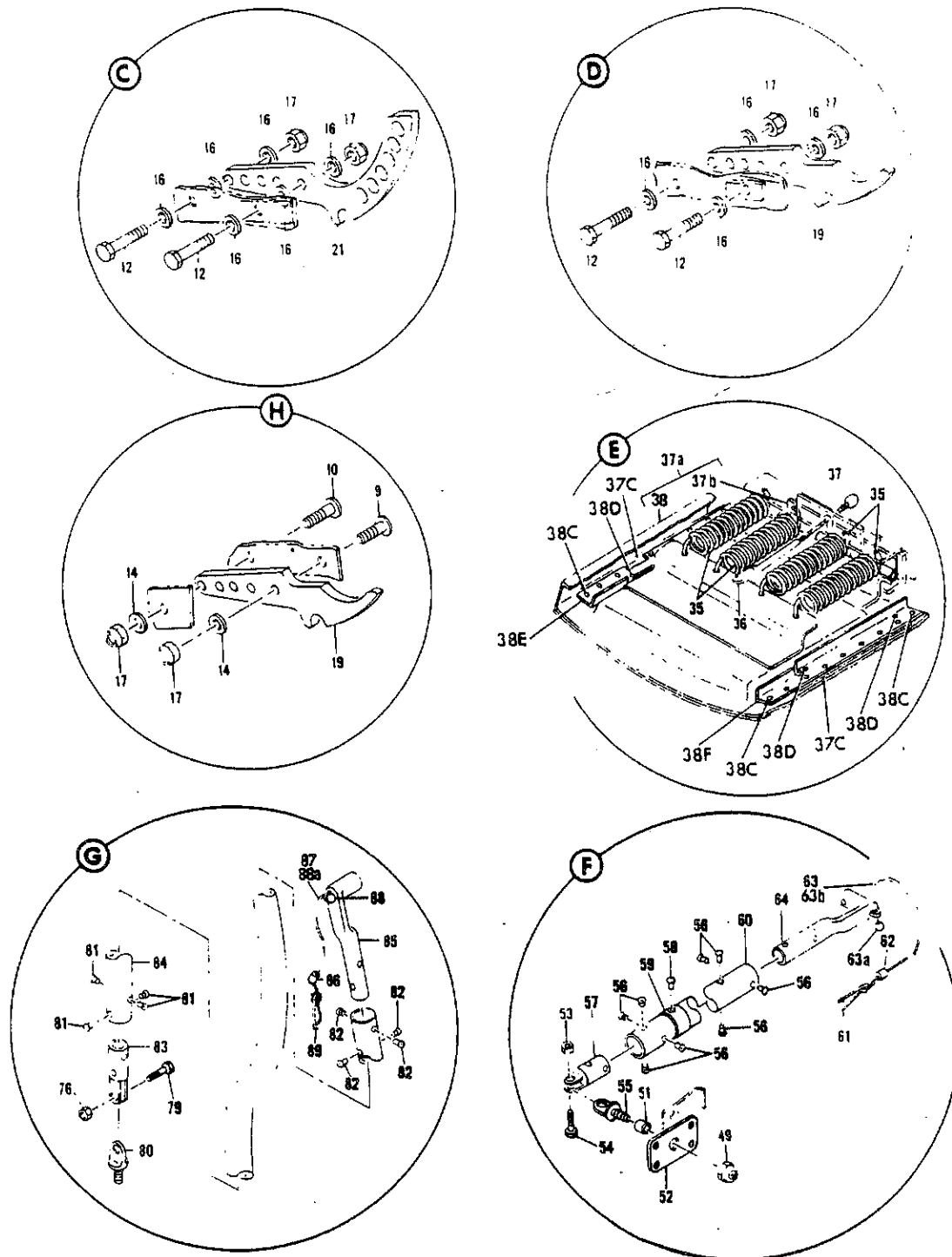
FIGURE 12. PANEL ASSY, ENGINE NACELLE COWL (SHEET 2)
