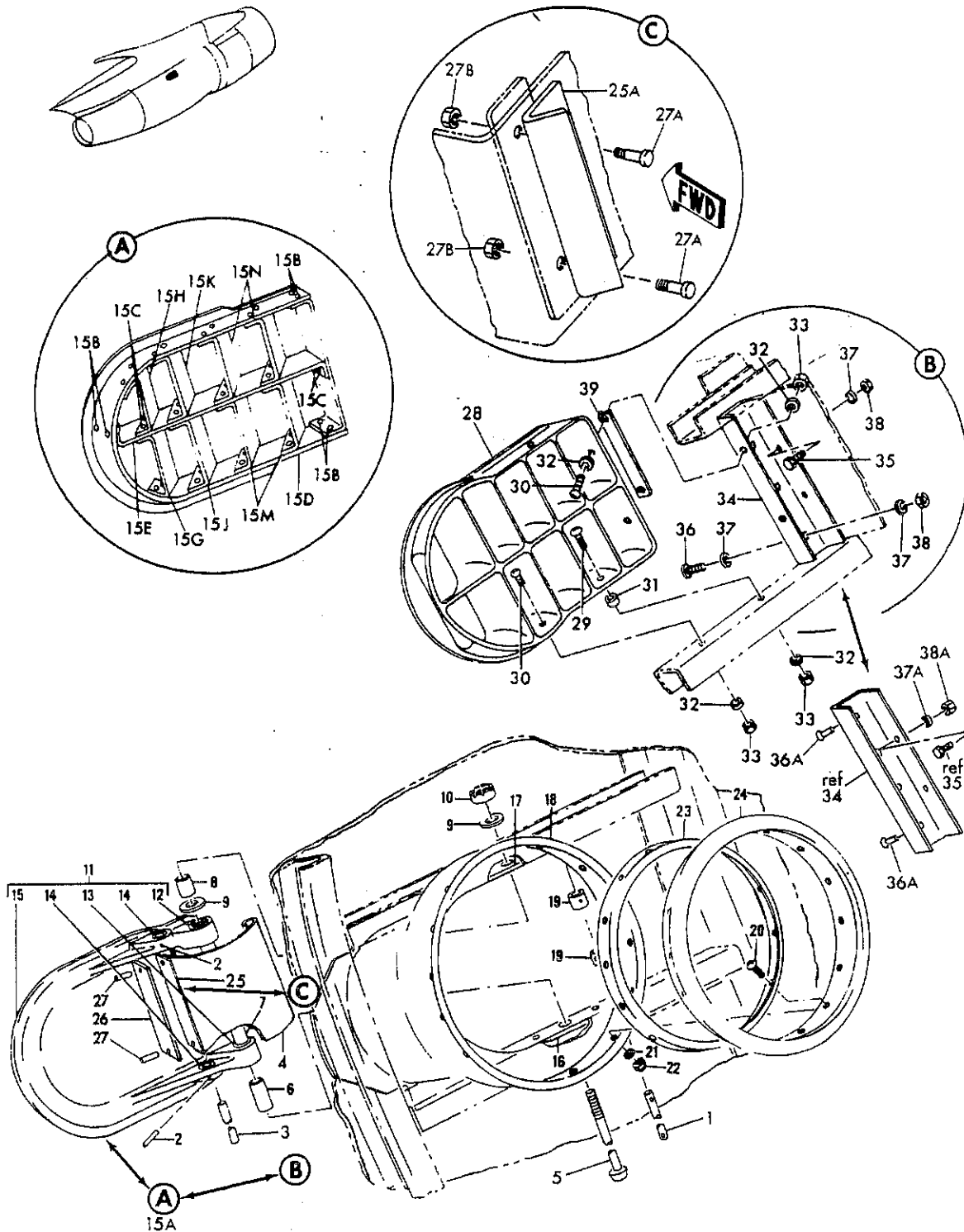
FIGURE 17A. DOOR INSTL, ENGINE SURGE BLEED (LH)
