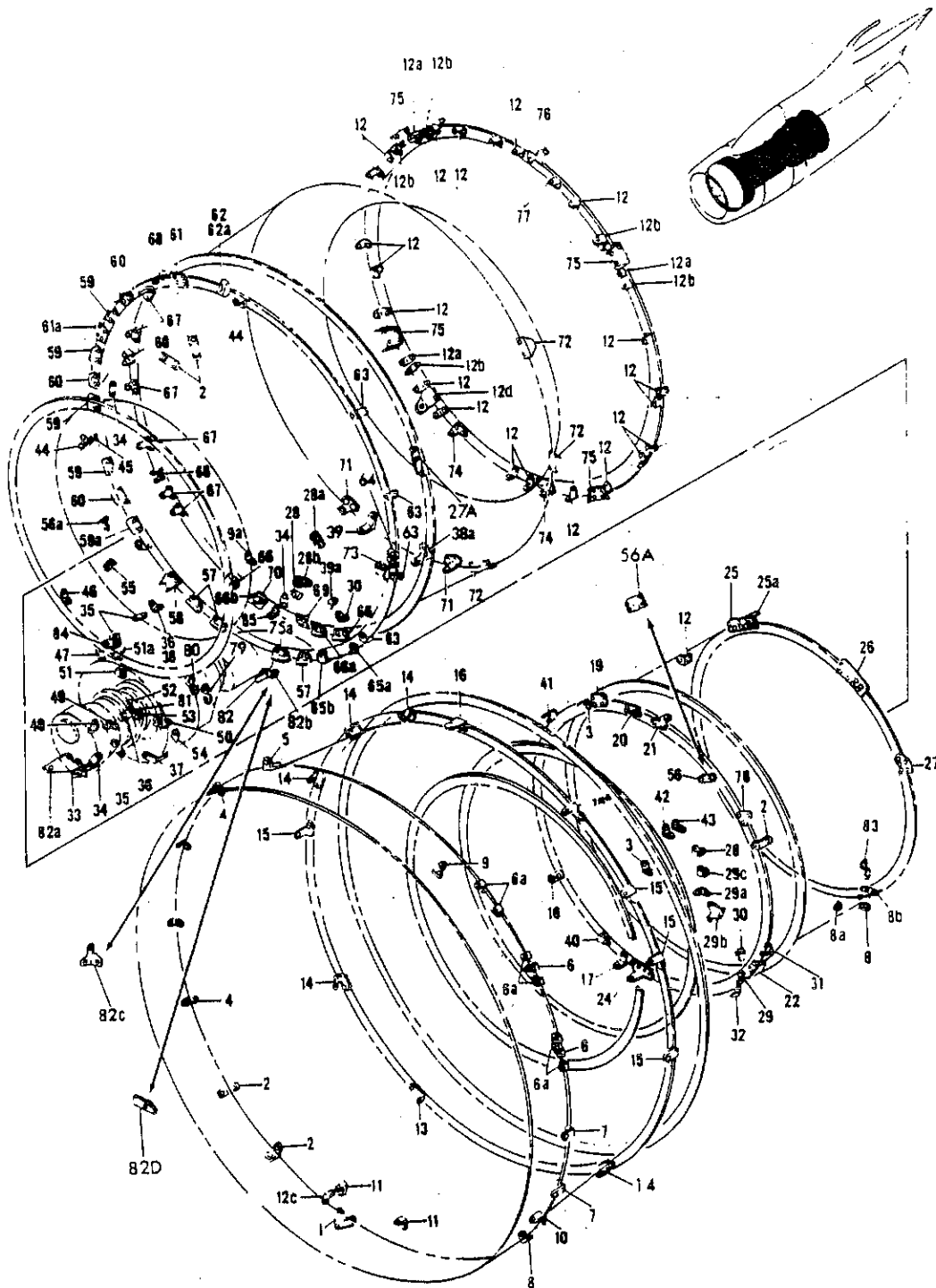
FIGURE 15. BRACKET INSTL, ENGINE
