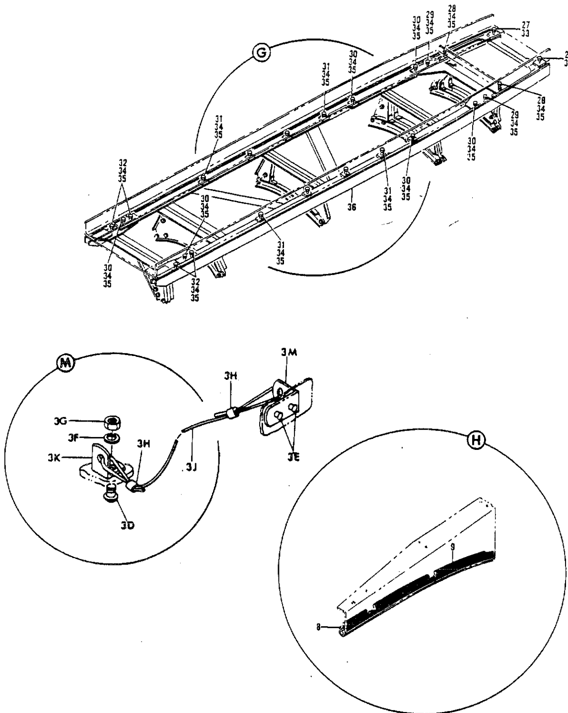
FIGURE 5. KIT AND BUILD-UP INSTL. FAN ENGINE TRANSPORT KIT BEAM TO ENGINE (SHEET 3)
