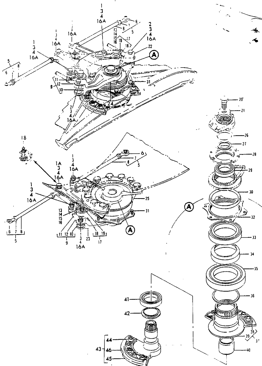
FIGURE 16. HINGE AND MECHANISM INSTL. JT3D ENGINE AFT THRUST REVERSER CLAMSHELL DOOR
