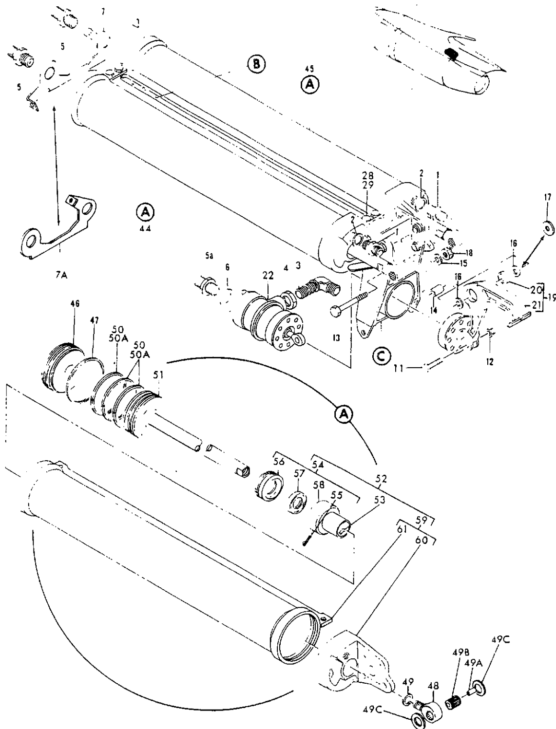
FIGURE 5A. ACTUATOR ASSY. AFT THRUST REVERSER UPPER (SHEET 1)
