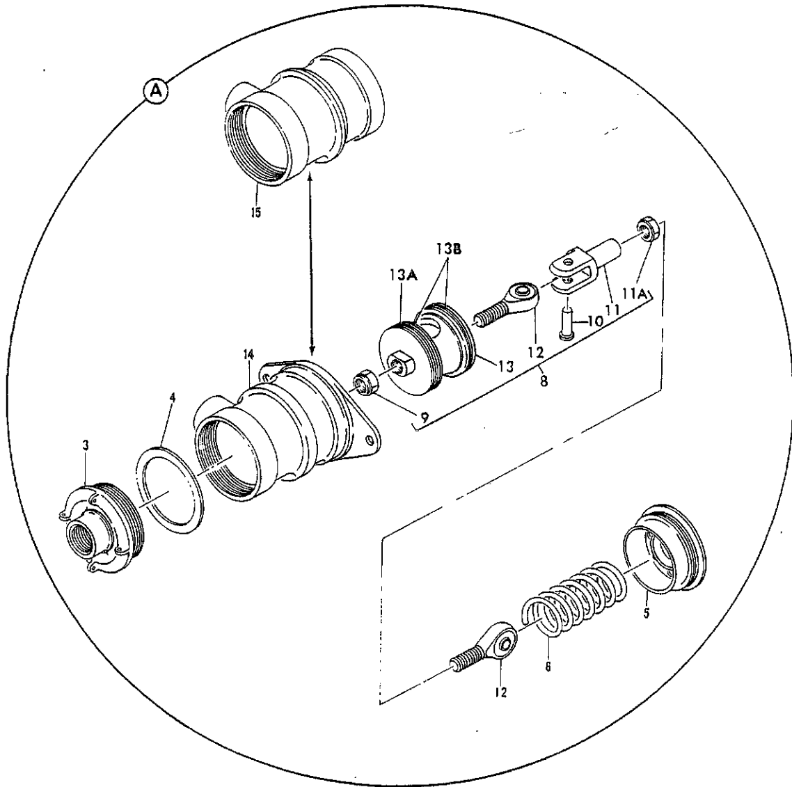
FIGURE 68. LOCK ASSY, AFT THRUST REVERSER ACTUATOR
