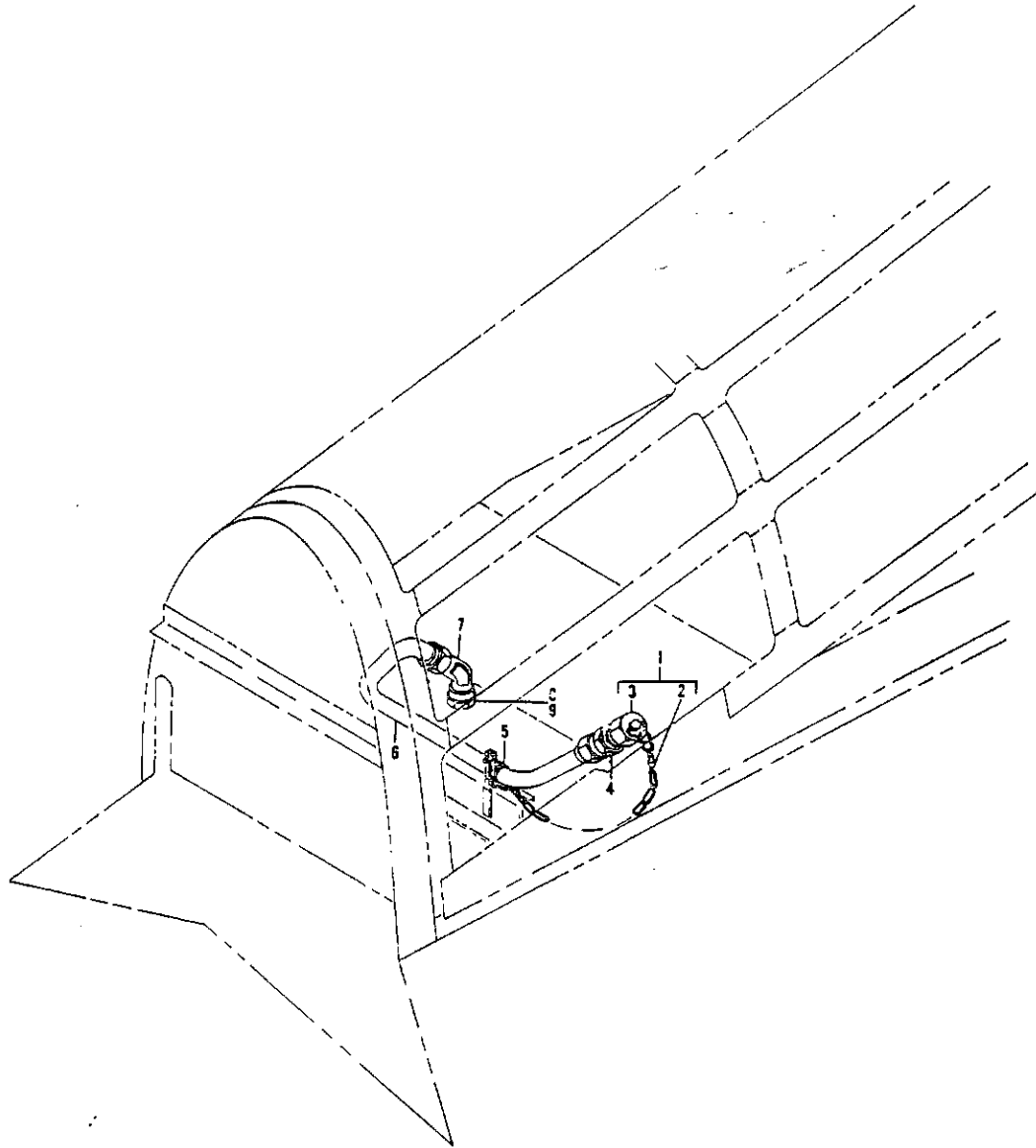
FIGURE 19. TUBE AND EQUIPMENT INSTL, THRUST REVERSER GROUND AIR RECEPTACLE
