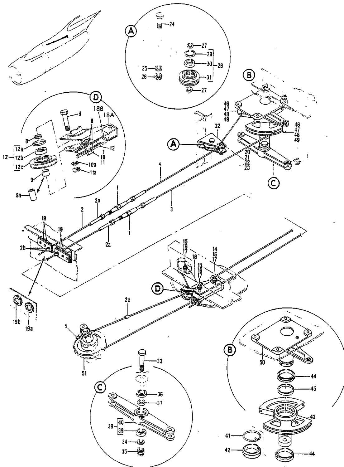
FIGURE 8. FOLLOW-UP INSTL. AFT THRUST REVERSER
