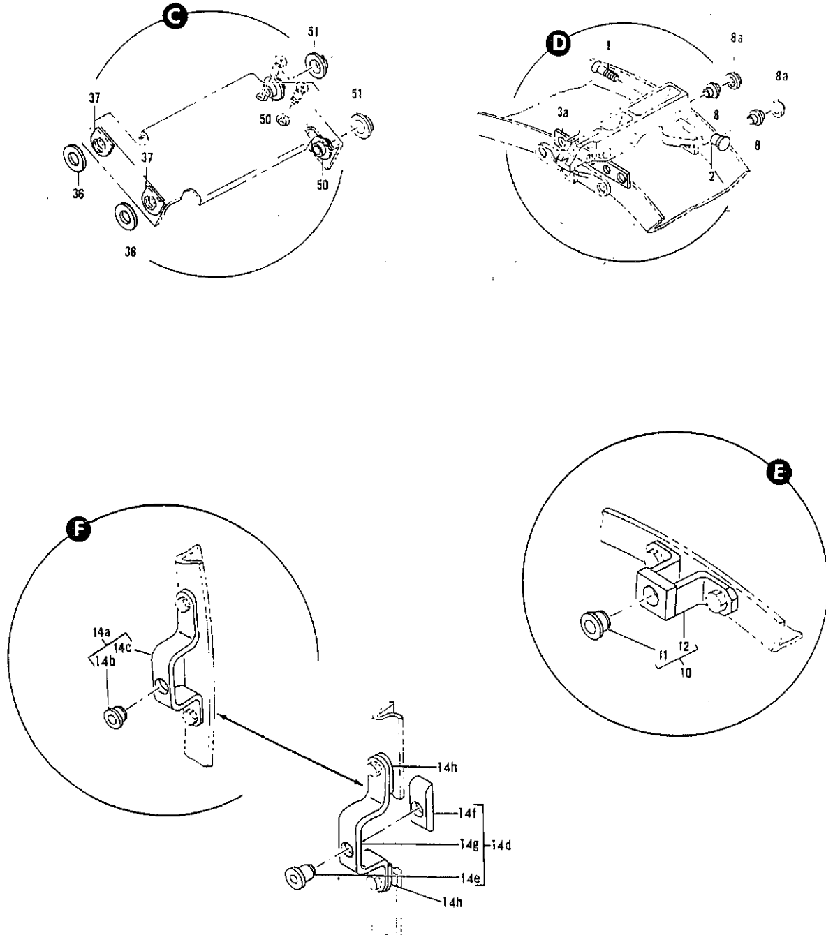
FIGURE 5. BRACKET INSTL, FAN REVERSER (SHEET 2)
