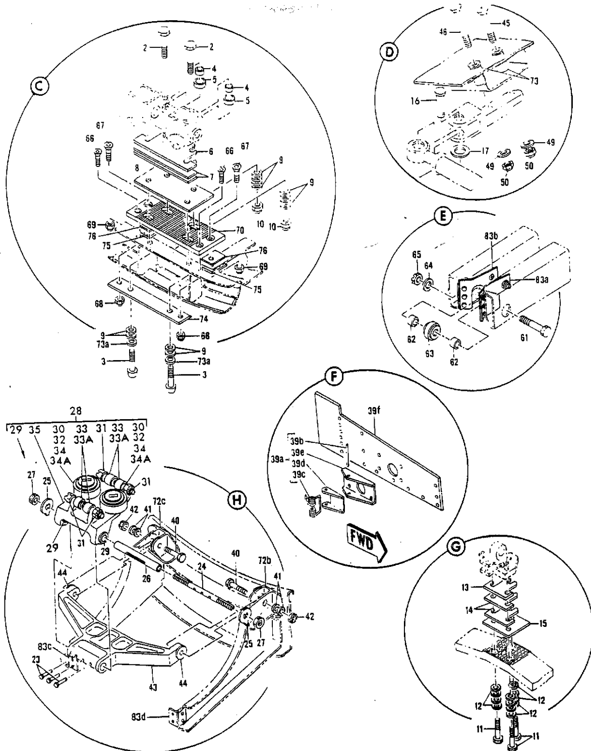
FIGURE 4. SLEEVE INSTL. AFT THRUST REVERSER (SHEET 2)
