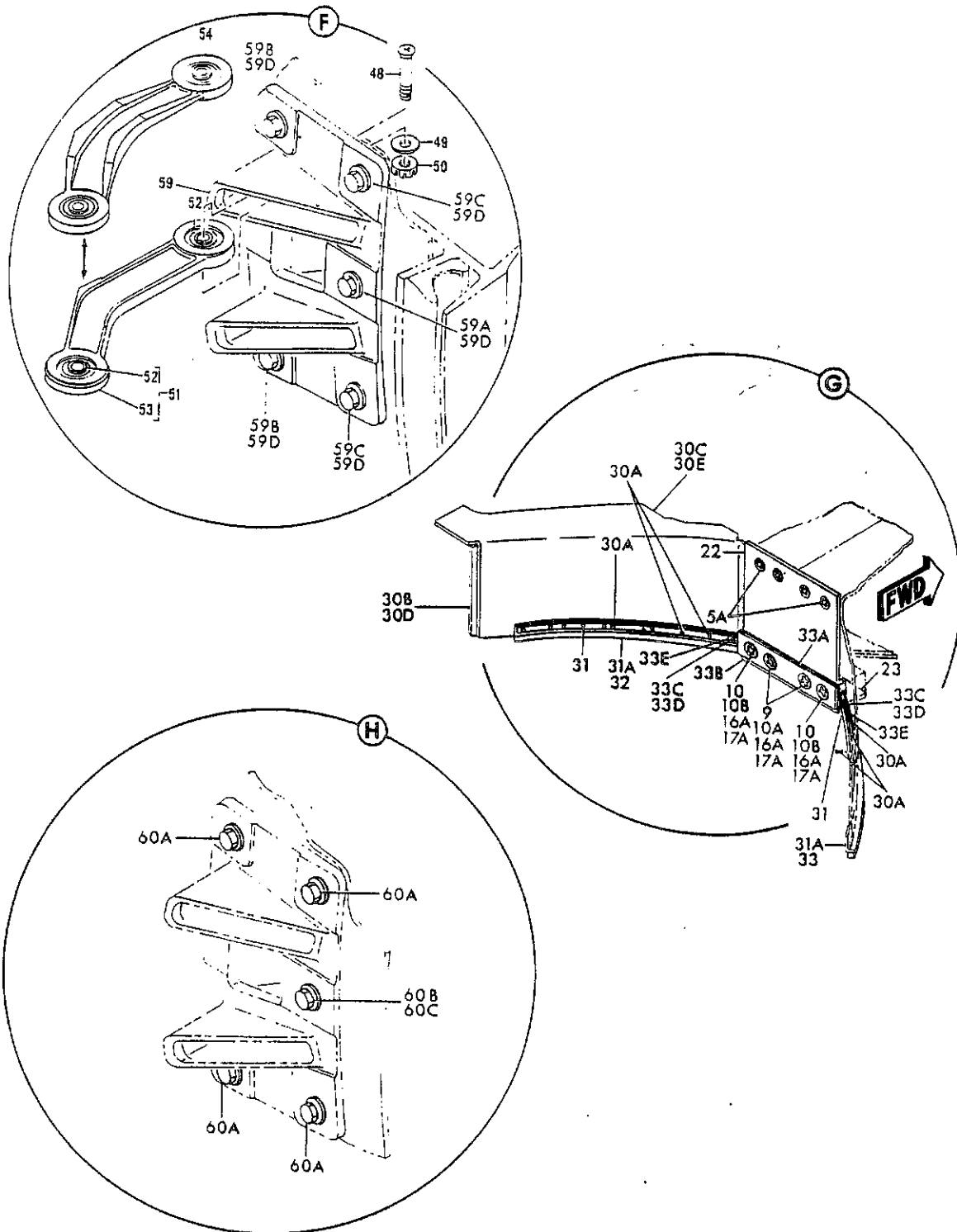
FIGURE 3. RING ASSY, FAN REVERSER COWL (SHEET 3)
