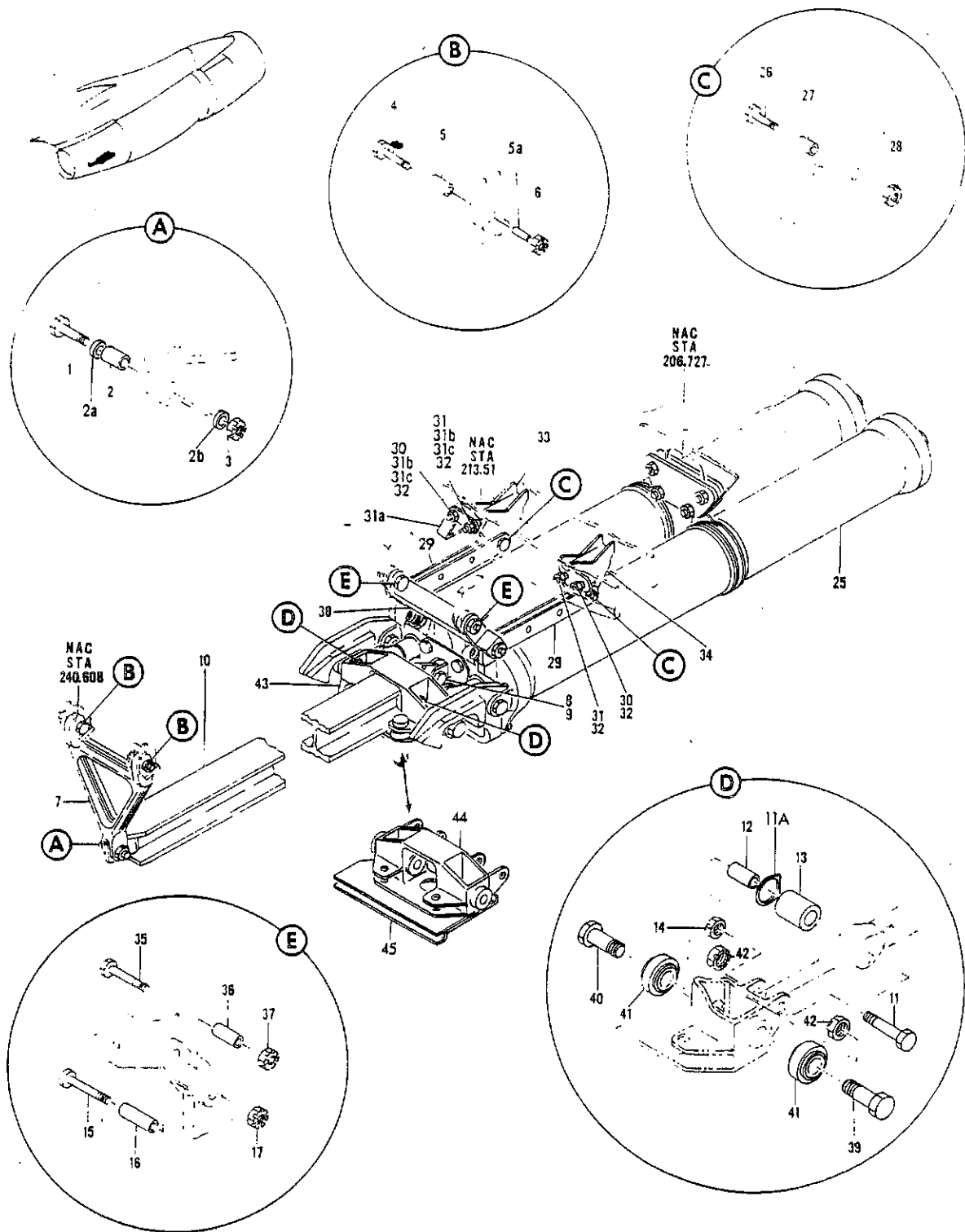
FIGURE 6. ACTUATOR INSTL, AFT THRUST REVERSER LOWER
