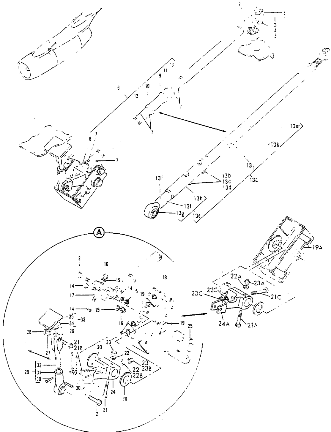
FIGURE 1. FOLLOW-UP INSTL. FAN REVERSER (SHEET 1)
