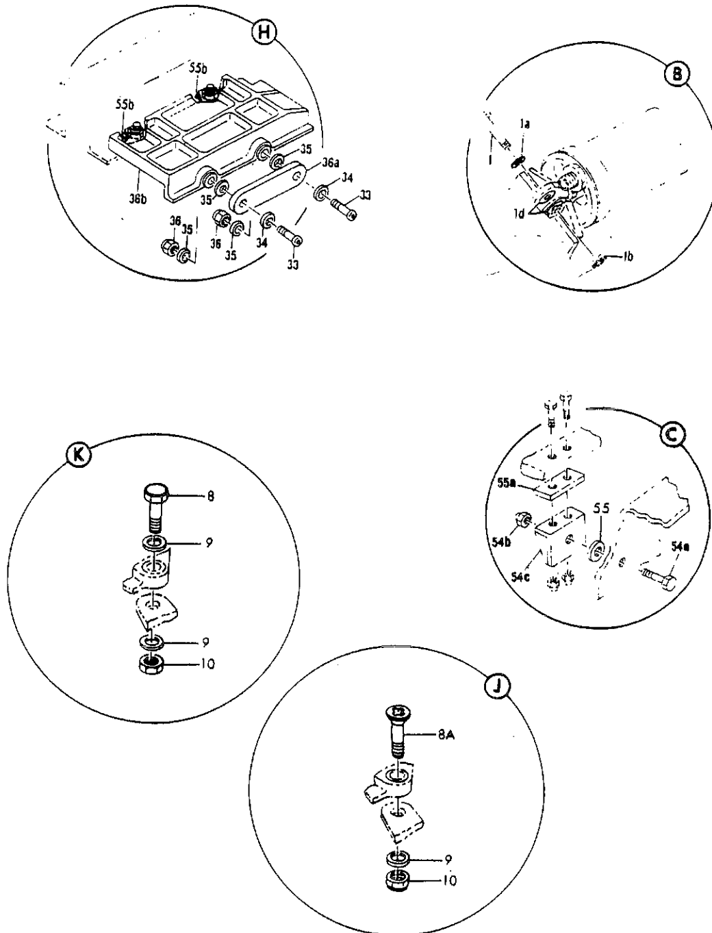
FIGURE L. FAN REVERSER INSTL, FAN ENGINE (SHEET 3)
