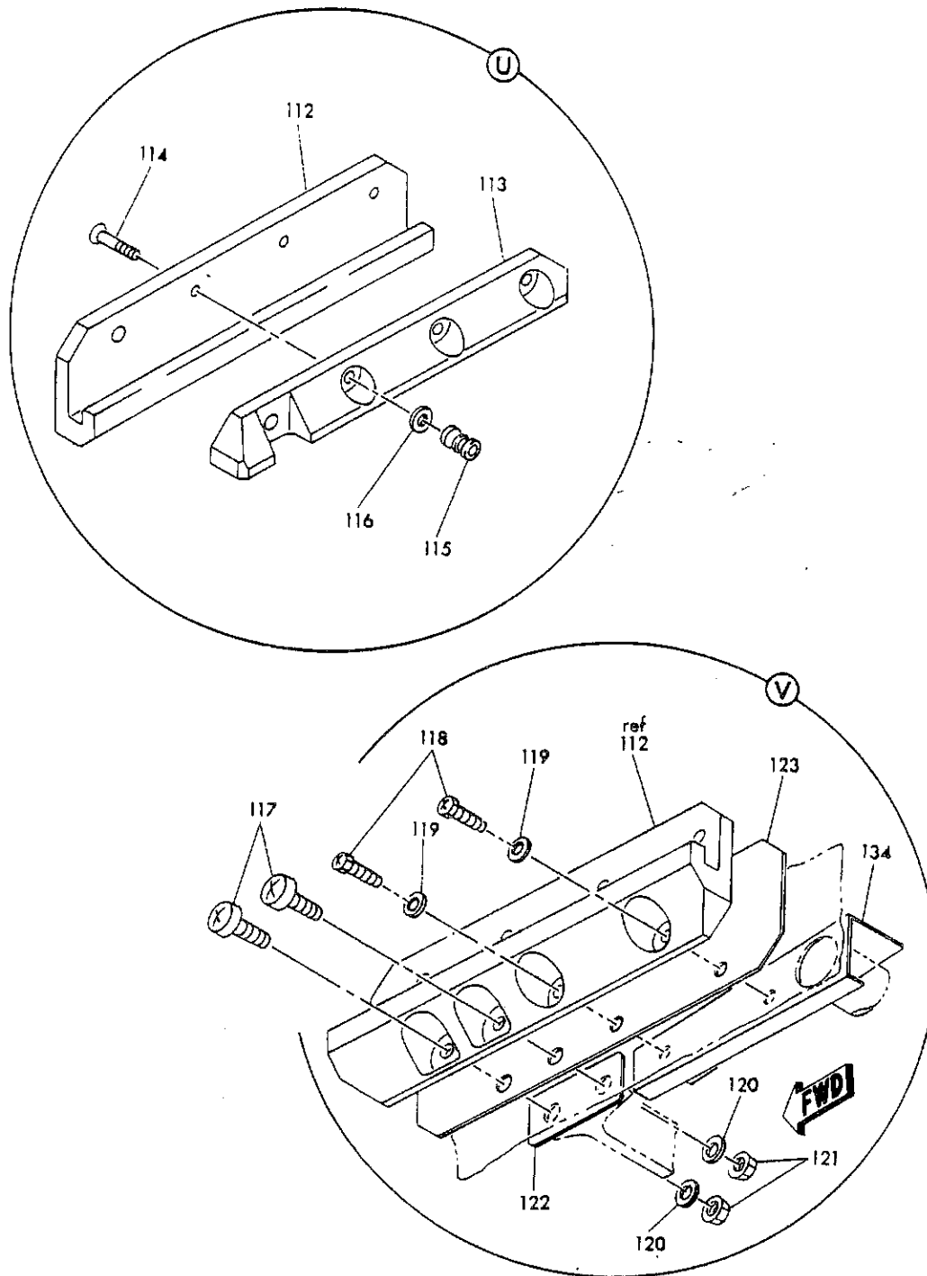
FIGURE 1. FAN REVERSER INSTL, FAN ENGINE (SHEET 7)
