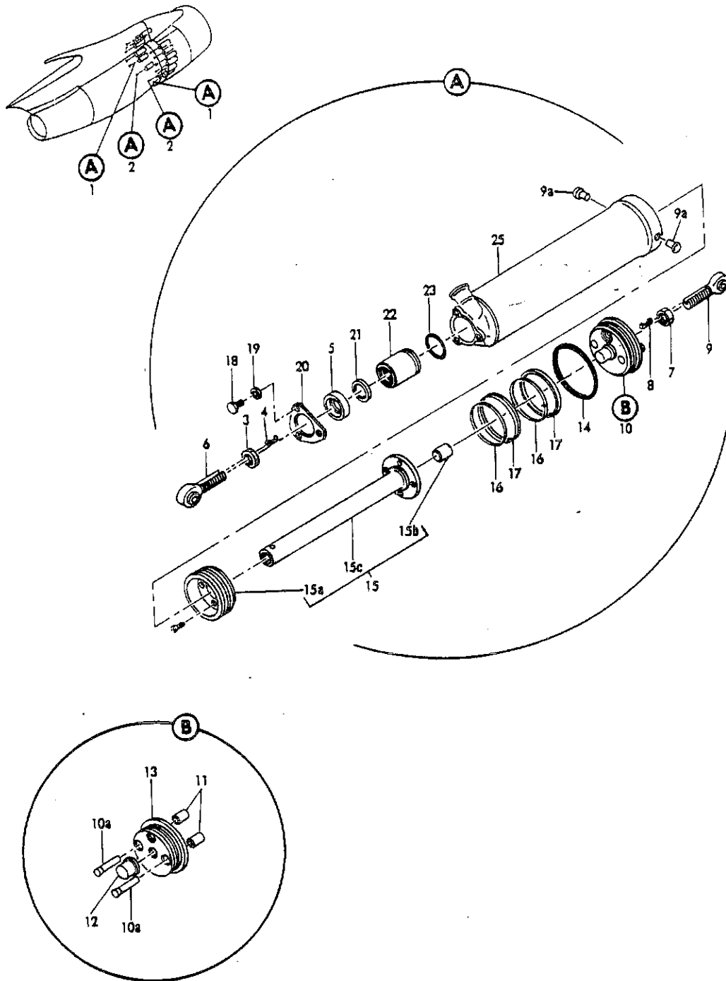
FIGURE 10. ACTUATOR ASSY, FAN REVERSER (EXHAUST ONLY)
