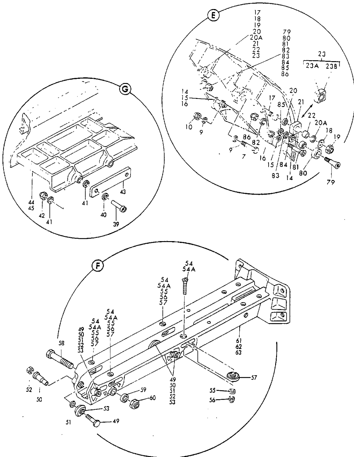
FIGURE 1B. FAN REVERSER (INSTL, FAN ENGINE (SHEET 3))
