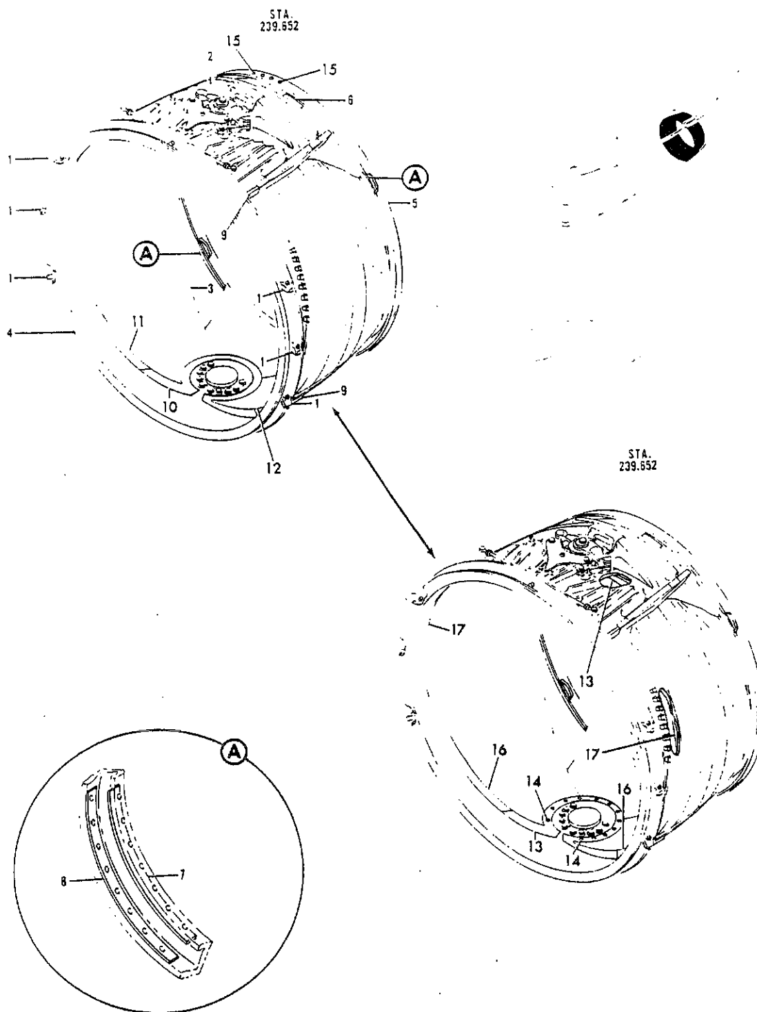
FIGURE 10. THRUST REVERSER ASSY, JT3D
