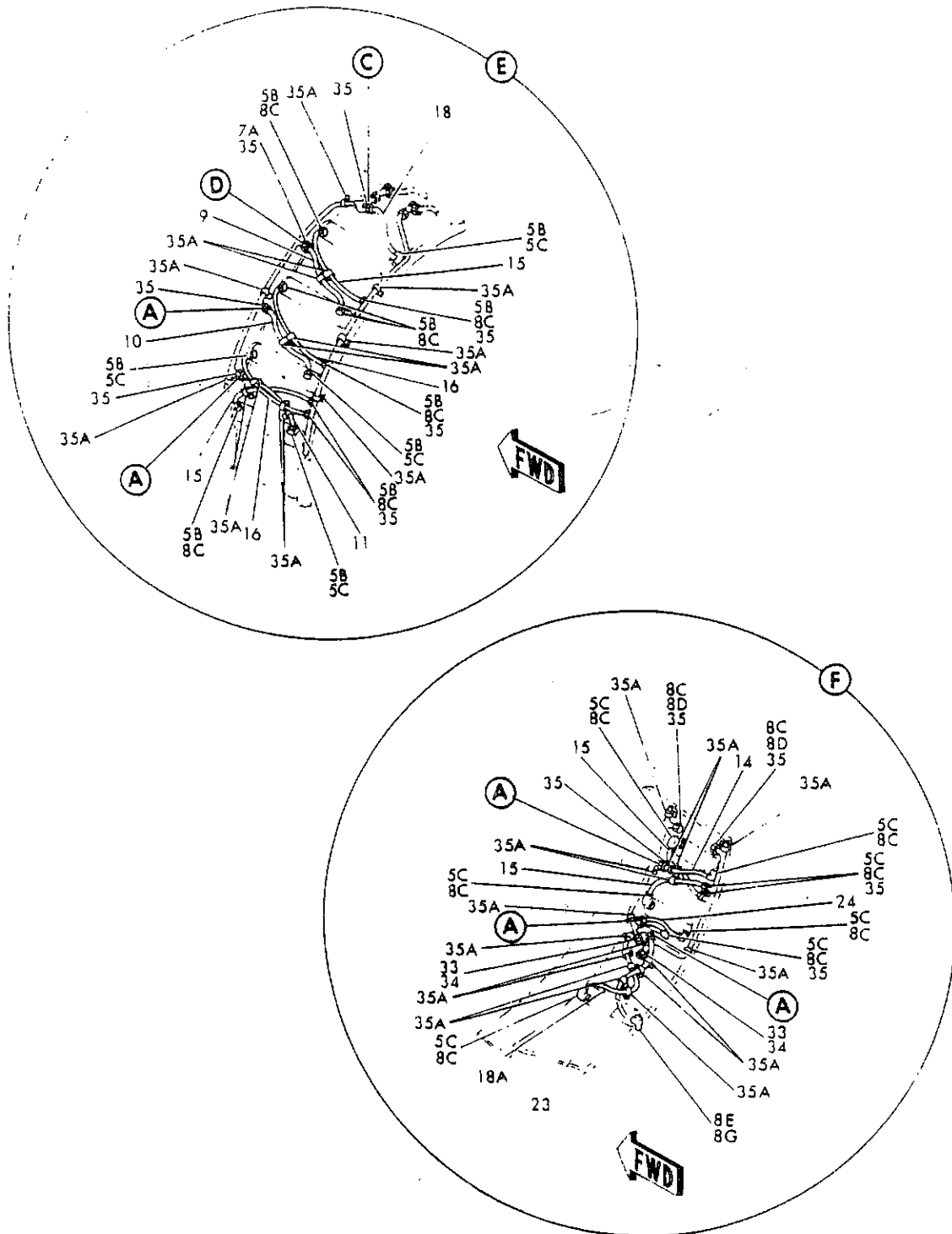
FIGURE 2. PLUMBING INSTL. FAN ENGINE FORWARD REVERSER (SHEET 2)
