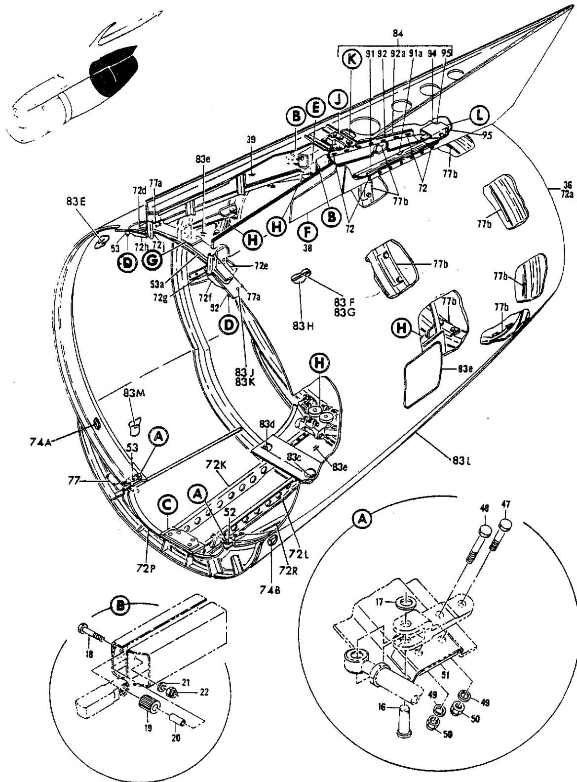
FIGURE 4. SLEEVE INSTL. AFT THRUST REVERSER (SHEET 1)
