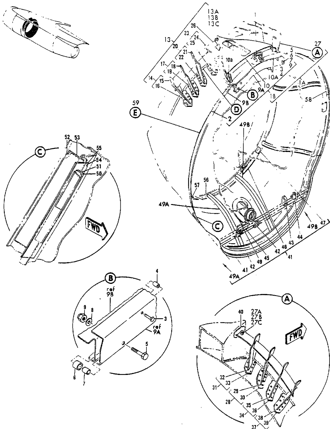
FIGURE 6. DIAPHRAGM INSTL, FAN ENGINE FAN AIR EXHAUST (SHEET 1)
