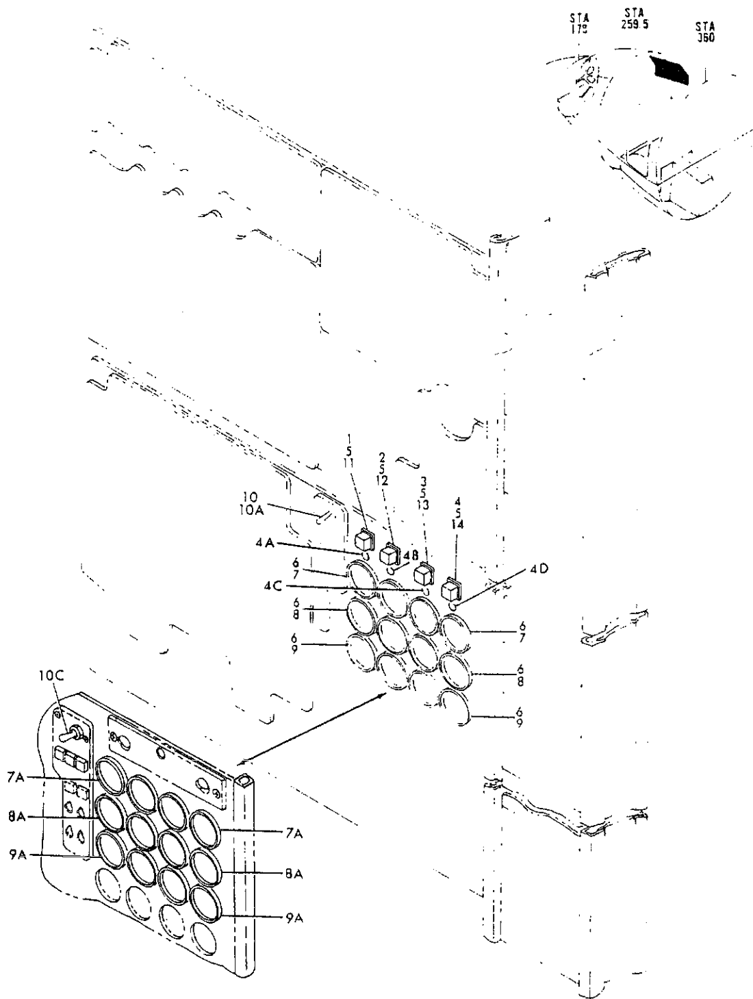
FIGURE 16K. PANEL INSTL, FLIGHT ENGINEERS LOWER (OIL ONLY)
