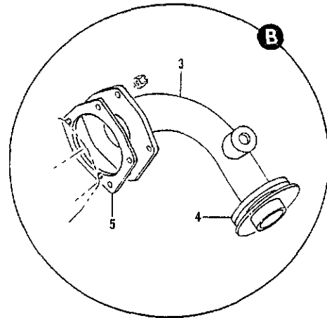
FIGURE 12. BULB INSTL, JT3D1 ENGINE OIL INLET TEMPERATURE BREATHER INSTL, FAN ENGINE
