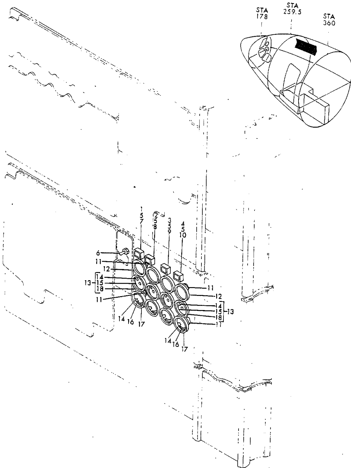
FIGURE 16M. PANEL INSTL, FLIGHT ENGINEERS LOWER (OIL ONLY)
