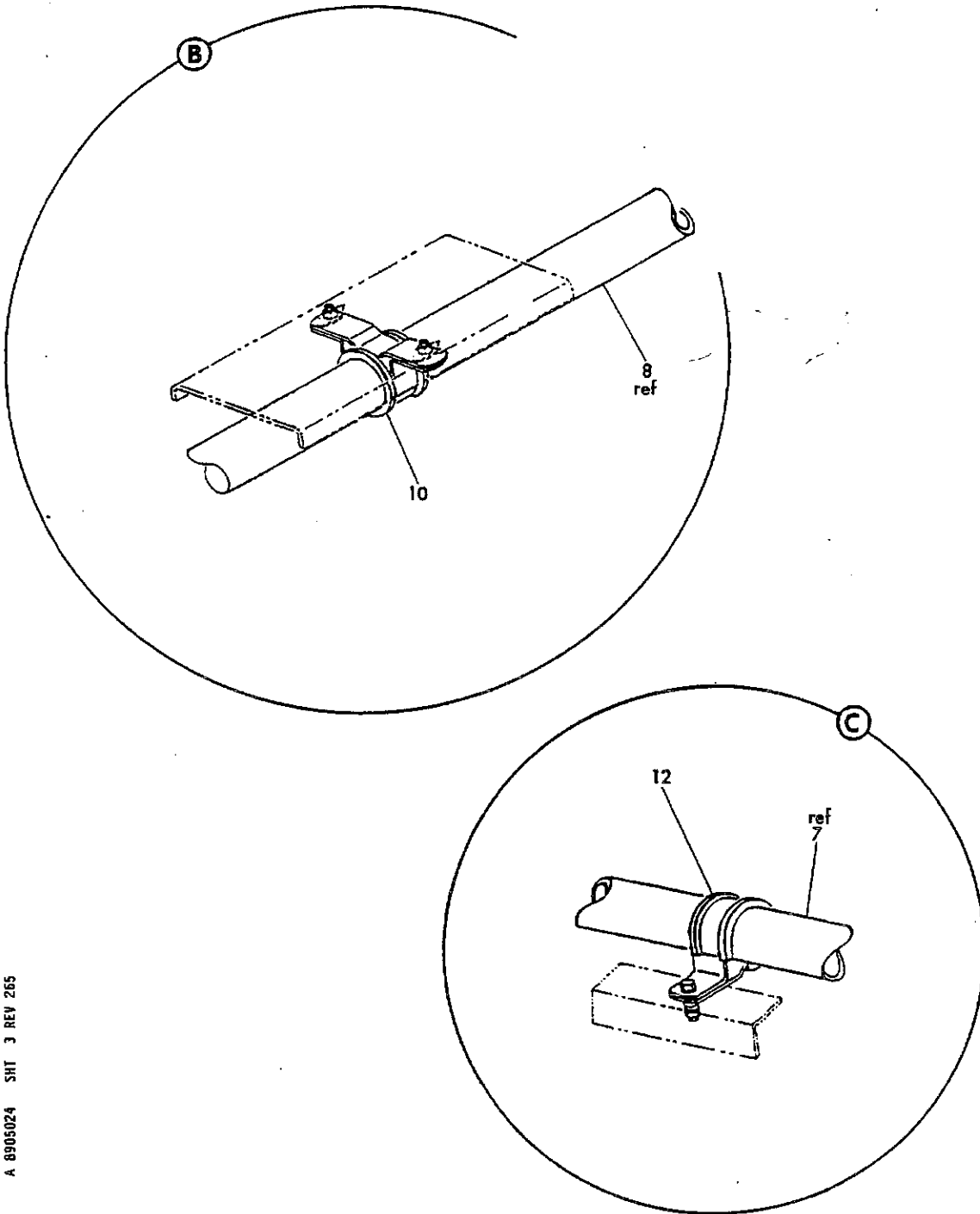
FIGURE 24. TUBE ASSY, HYDRAULIC UT II SUPPLY 1-1/4 IN. (SHEET 3)
