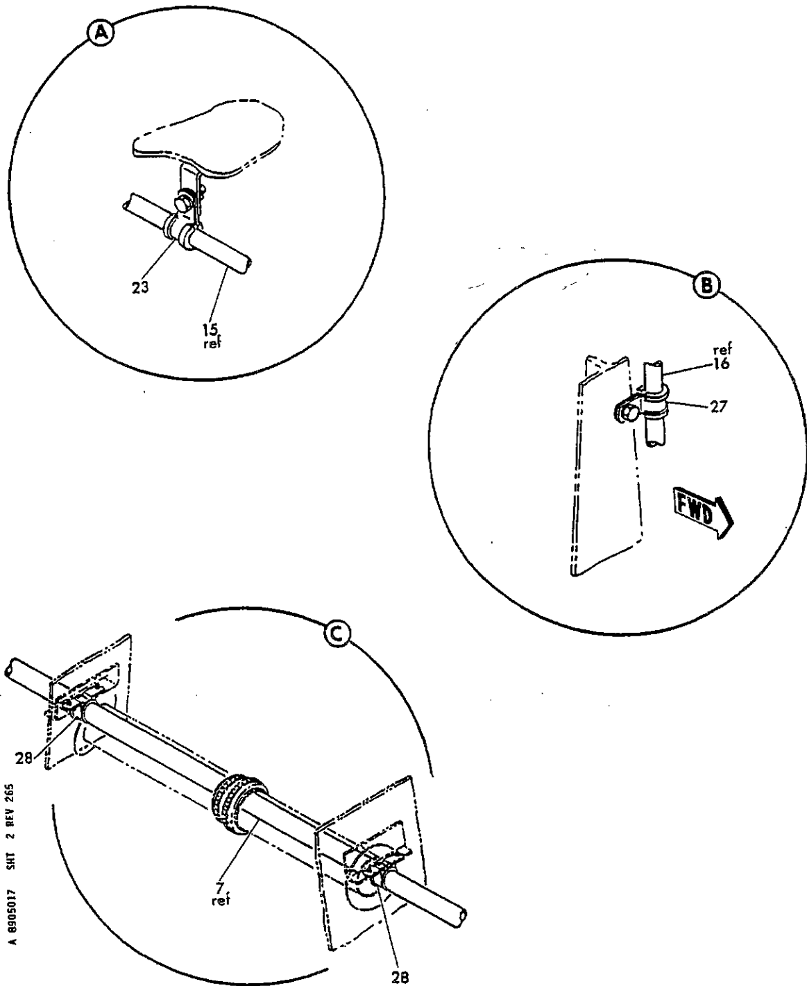
FIGURE 17. SHUT OFF VALVE 1-1/4 IN. INSTL (SHEET 2)
