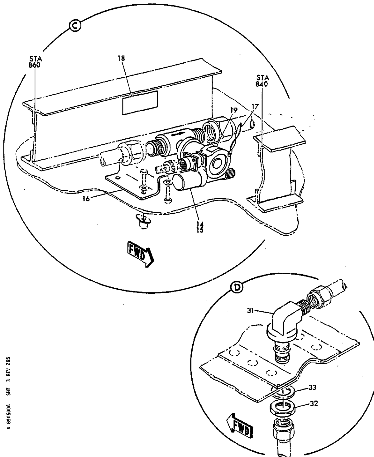
FIGURE 6. F.S. STA 800 TO 880 AREA HYDRAULIC SYSTEM INSTL, AFT A/R PUMP PRESSURE LINE L.H. (SHEET 3)
