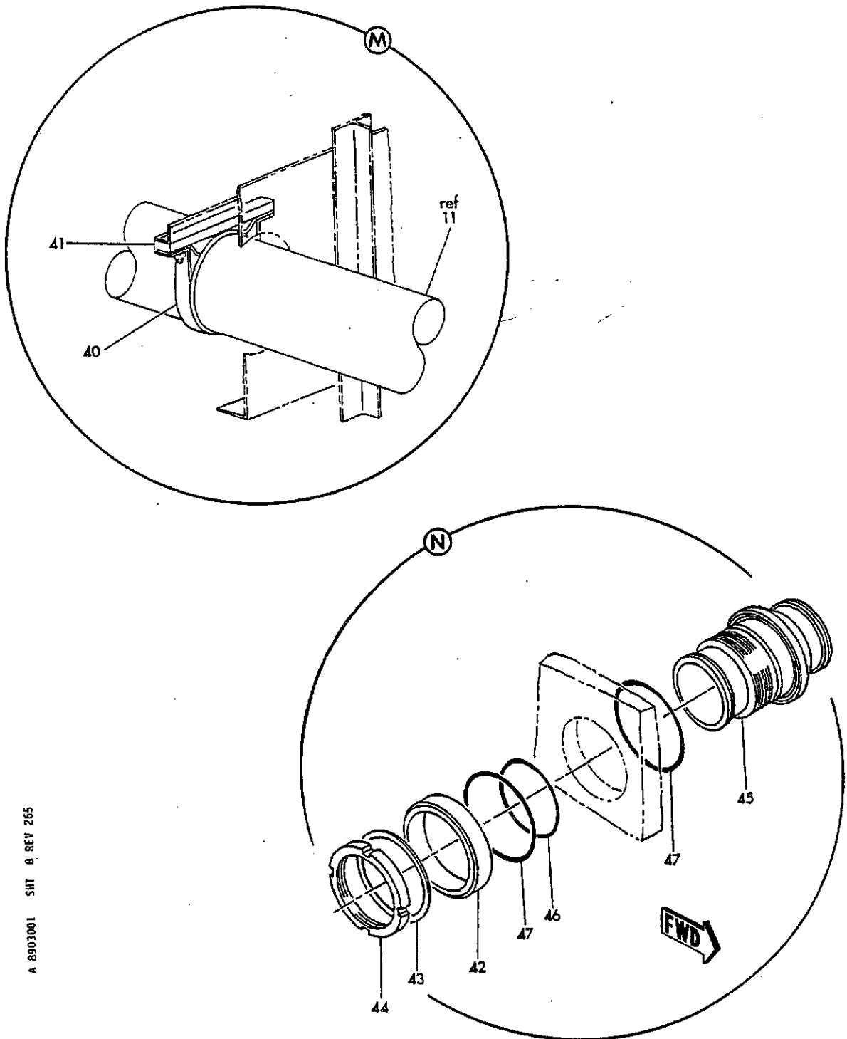
FIGURE 1. WING FUEL SYSTEM INSTL. (SHEET 8)
