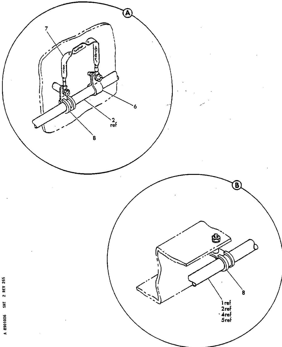
FIGURE 6. SENSING INSTL. (SHEET 2)
