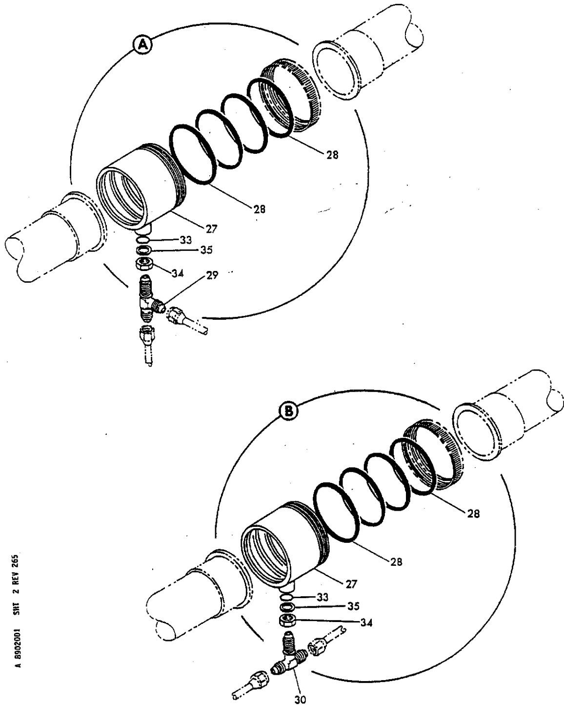
FIGURE 1. FUEL SYSTEM INSTL. SHAKE PIT AREA STA 600K TO 600F (SHEET 2)
