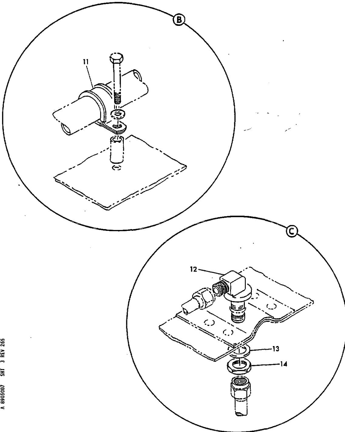
FIGURE 7. F.S. STA 800 TO 880 AREA HYDRAULIC SYSTEM INSTL, AFT A/R PUMP PRESSURE LINE L.H. (SHEET 3)
