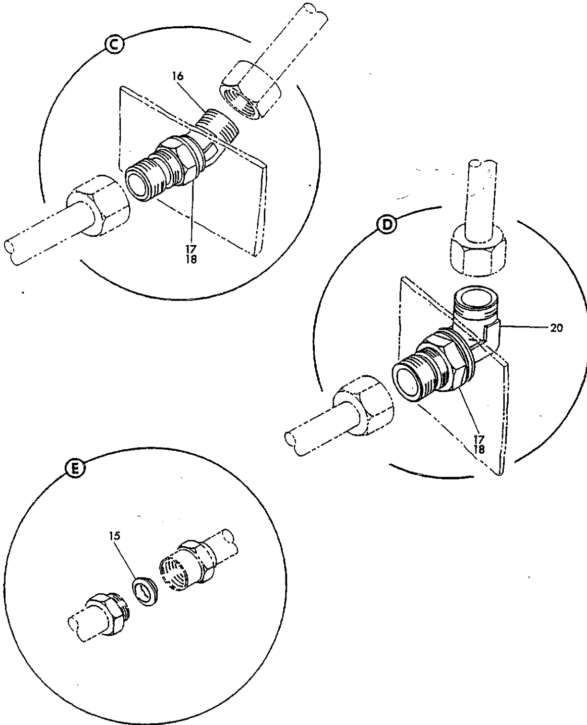
FIGURE 25. HYDRAULIC SYSTEM INSTL WING REAR SPAR (SHEET 3)
