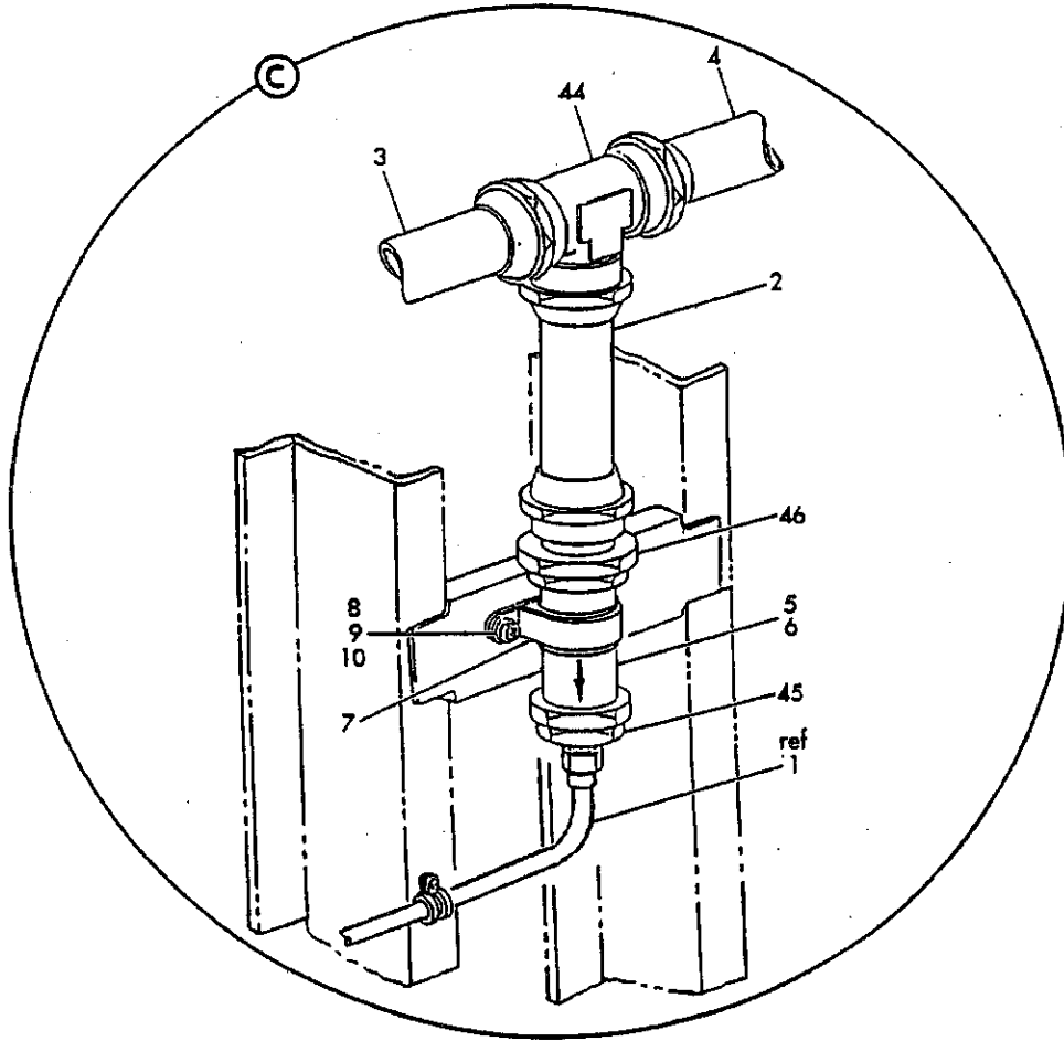
FIGURE 9. PRESSURE SYS INSTL. A/R POD FUEL POSITIVE INLET (SHEET 2)
