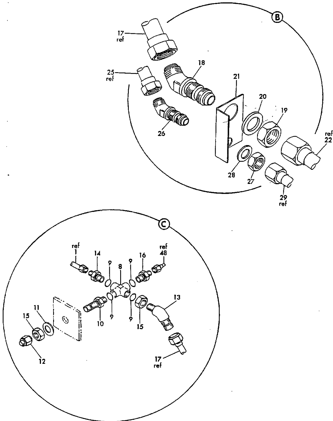
FIGURE 27. HYDRAULIC UT II INSTL, SECT 43(STA 815 TO 840 RH)(HYDRAULIC POWER ONLY)(SHEET 3)
