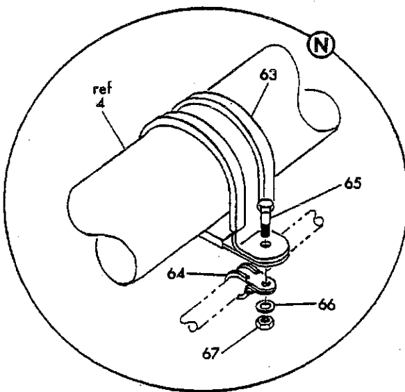
FIGURE 1. FUEL SYSTEM INSTL. SNAKE PIT AREA STA 600K TO 600F (SHEET 7)
