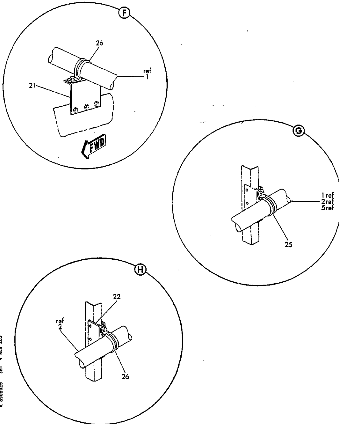
FIGURE 25. HYDRAULIC SYSTEM INSTL WING REAR SPAR (SHEET 4)
