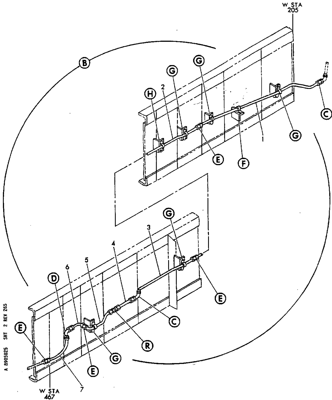
FIGURE 25. HYDRAULIC SYSTEM INSTL WING REAR SPAR (SHEET 2)
