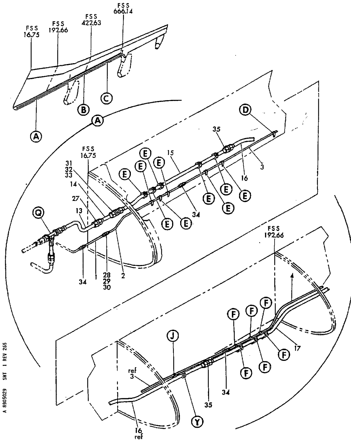
FIGURE 29. WING HYDRAULIC SYSTEM INSTL. FRONT SPAR AREA (SHEET 1)
