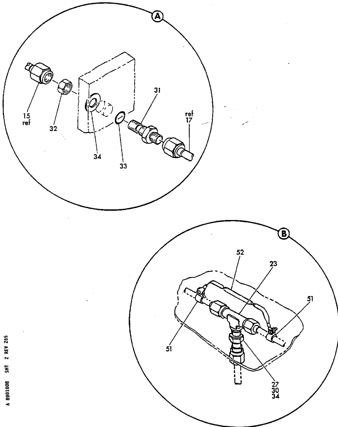
FIGURE 8. DRAIN INSTL, A/R FUEL PUMP SEAL (SHEET 2)
