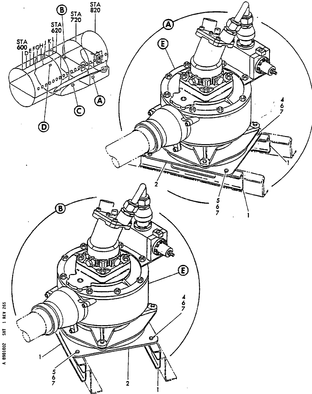
FIGURE 2. A/R FUEL PUMP INSTL. FWD (SHEET 1)
