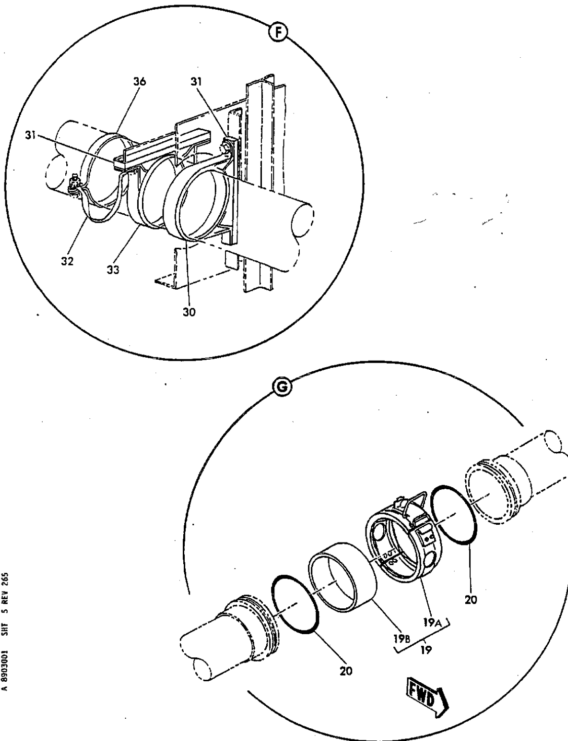
FIGURE 1. WING FUEL SYSTEM INSTL. (SHEET 5)
