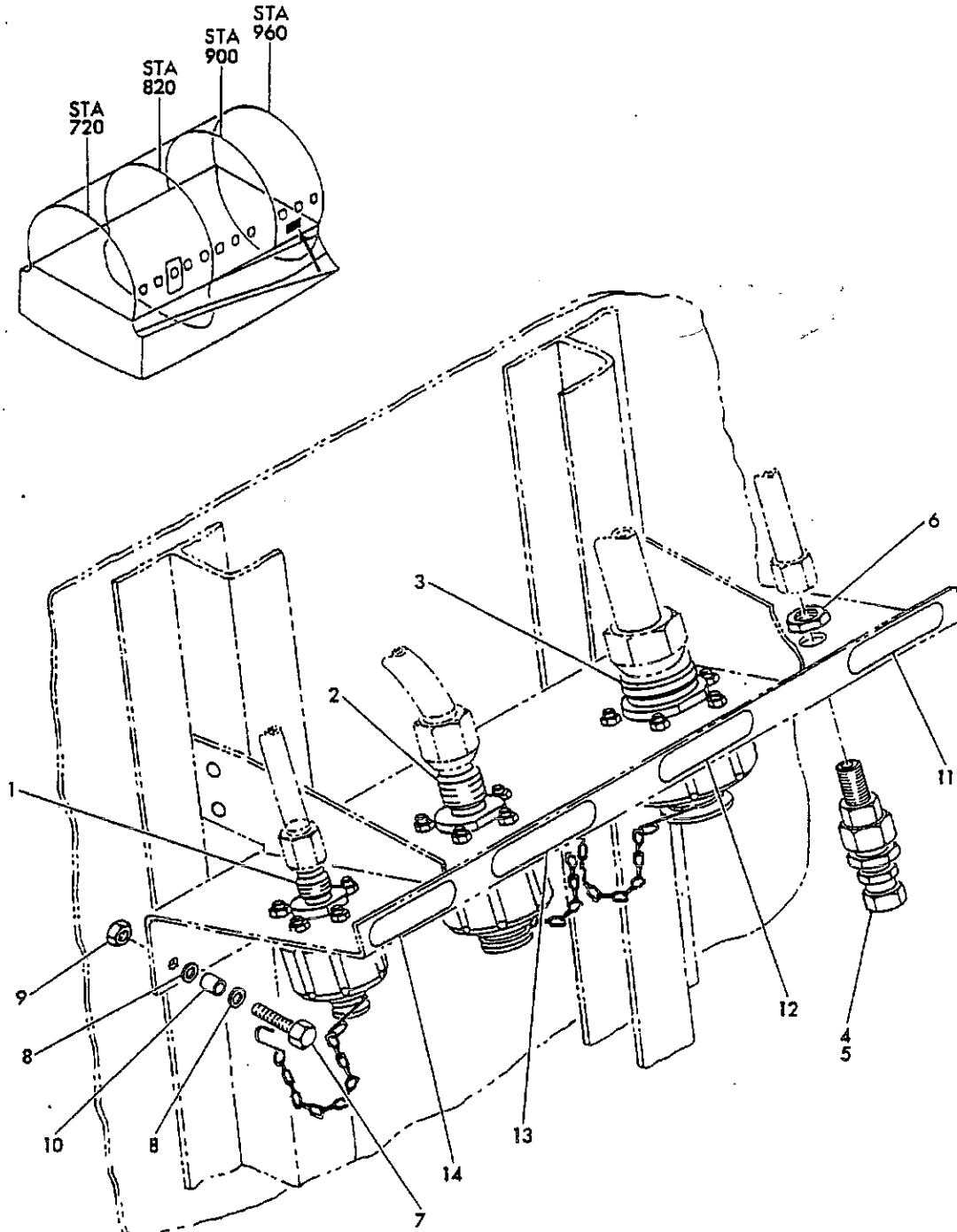
FIGURE 14. CONNECTORS INSTL., HYDRAULIC UT II FILLING AND TEST PORTS
