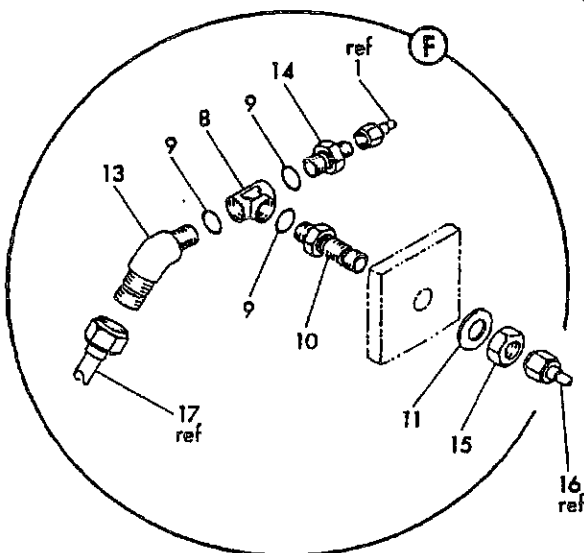
FIGURE 26. HYDRAULIC UT II INSTL, SECT 43(STA 815 TO 840 LH)(HYDRAULIC POWER ONLY)(SHEET 3)
