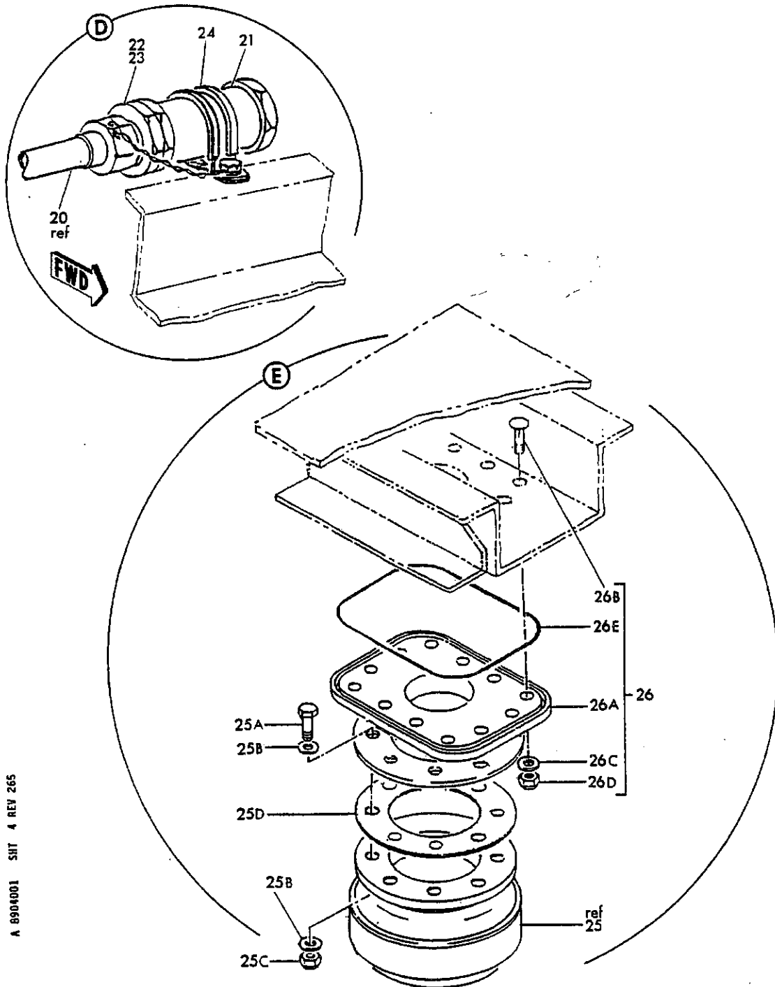
FIGURE 1. ISOLATION VALVE INSTL (SHEET 4)
