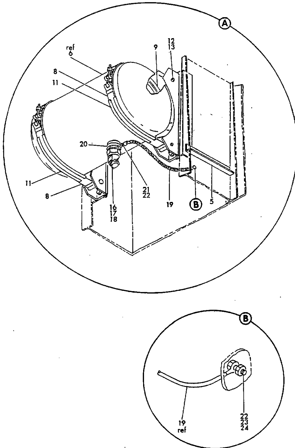
FIGURE 22. TANK INSTL. HYDRAULIC SURGE (SHEET 2)
