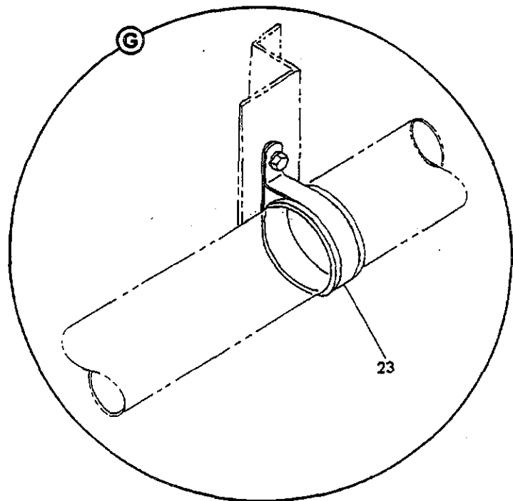
FIGURE 1. FUEL SYSTEM INSTL, WING CENTER SECTION (A/R PUMP PRESSURE LINE ONLY) (SHEET 4)
