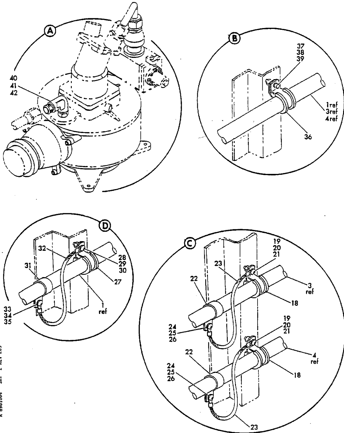
FIGURE 4. LOW FUEL PRESSURE INDICATION SYSTEM INSTL (SHEET 2)
