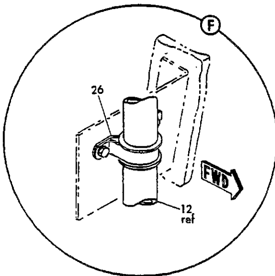
FIGURE 17. SHUT OFF VALVE 1-1/4 IN. INSTL (SHEET 3)
