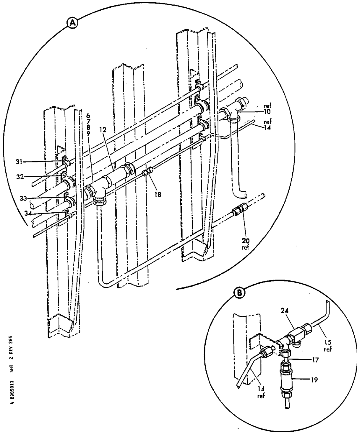
FIGURE 11. WATER TANK AREA HYDRAULIC UT II SYS INSTL, STA 820 TO 960 (SHEET 2)
