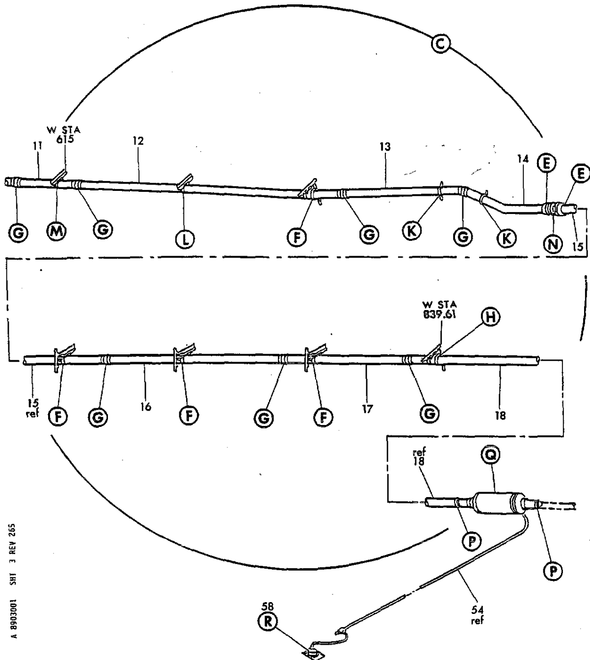
FIGURE 1. WING FUEL SYSTEM INSTL. (SHEET 3)
