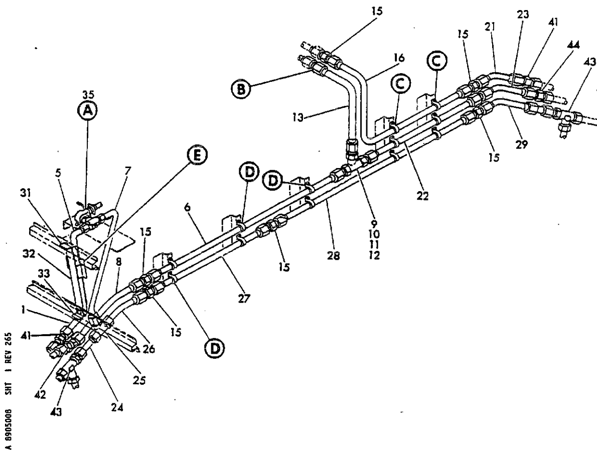
FIGURE 8. HYDRAULIC UT II SYSTEM INSTL. SNAKE PIT ONLY (SHEET 1)
