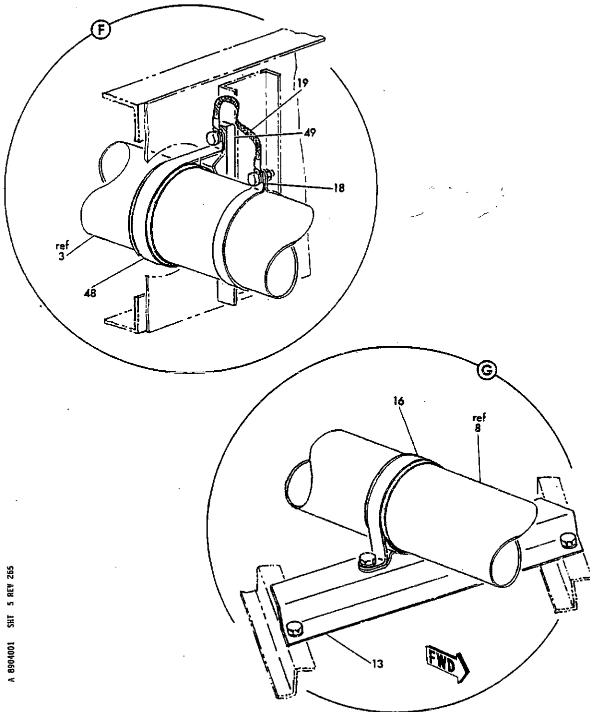
FIGURE 1. ISOLATION VALVE INSTL (SHEET 5)
