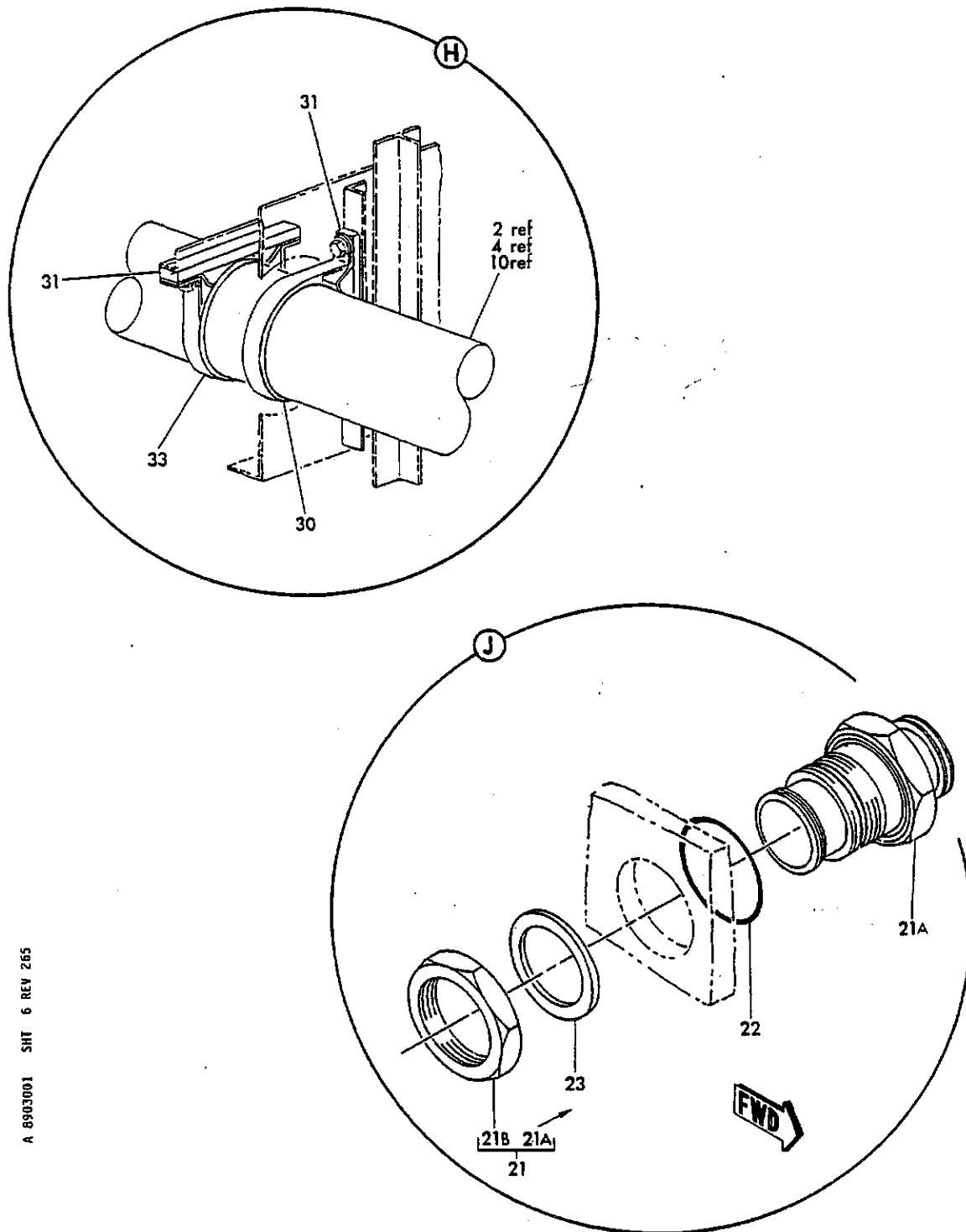
FIGURE 1. WING FUEL SYSTEM INSTL. (SHEET 6)
