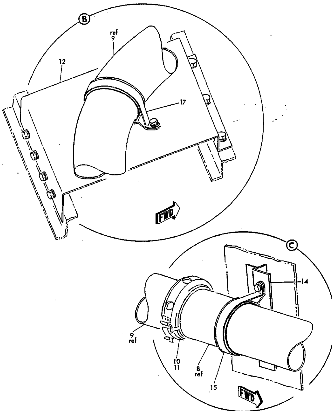
FIGURE 1. ISOLATION VALVE INSTL (SHEET 3)
