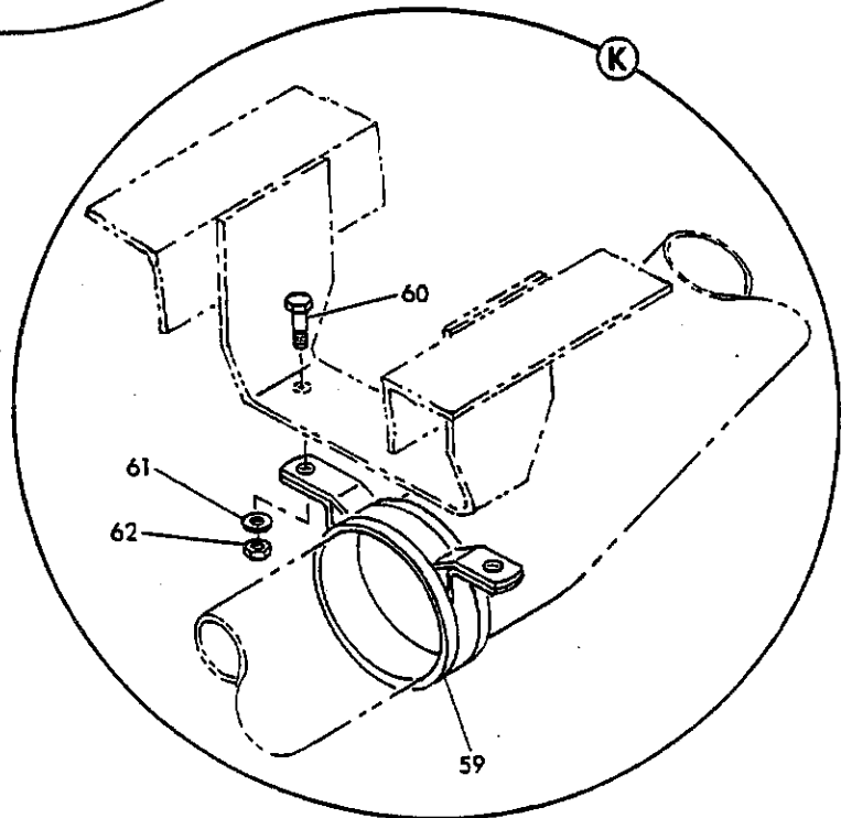
FIGURE 1. FUEL SYSTEM INSTL. SNAKE PIT AREA STA 600K TO 600F (SHEET 6)
