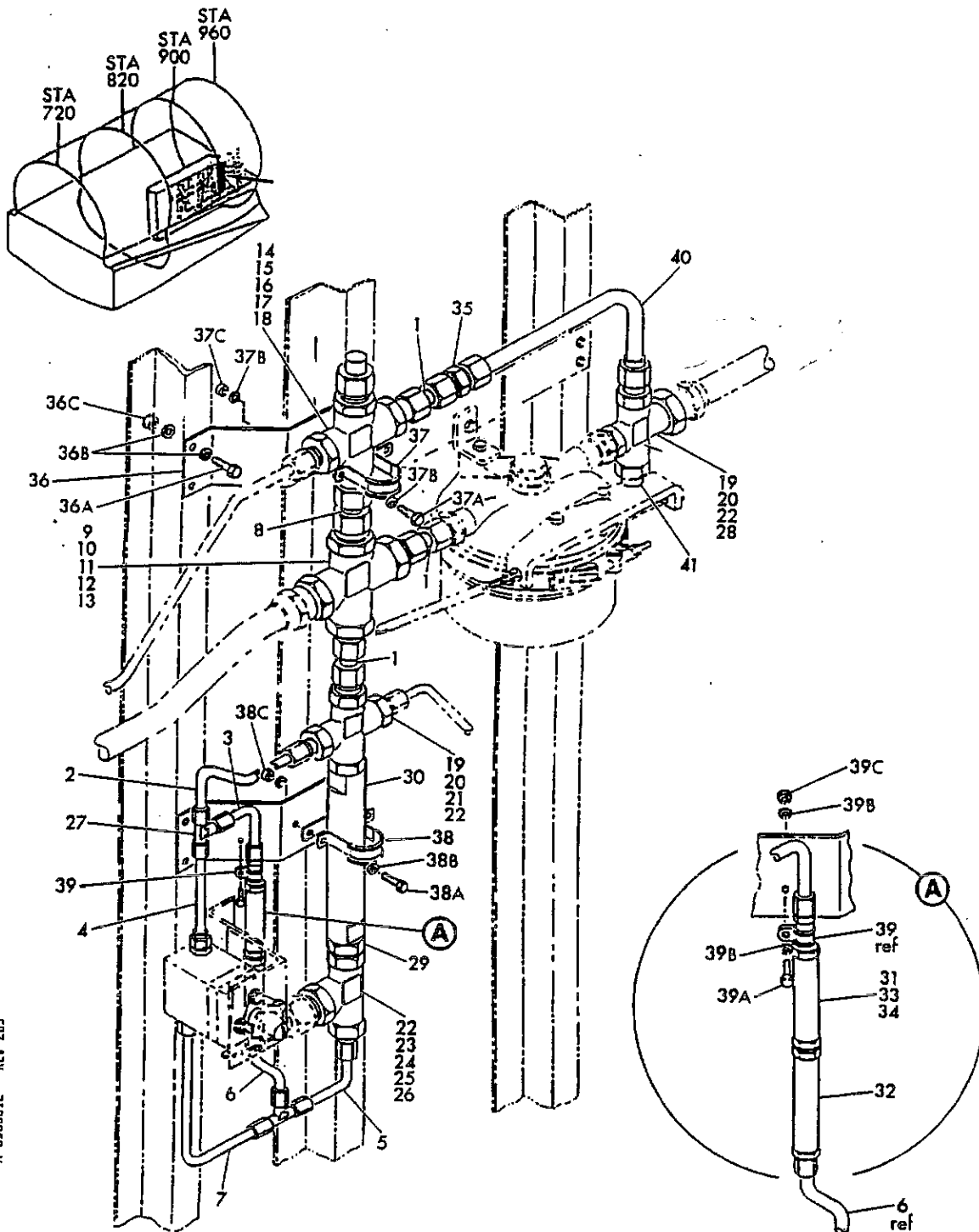
FIGURE 12. MULTIPLE CROSS FITTING INSTL, HYDRAULIC UT II SYSTEM
