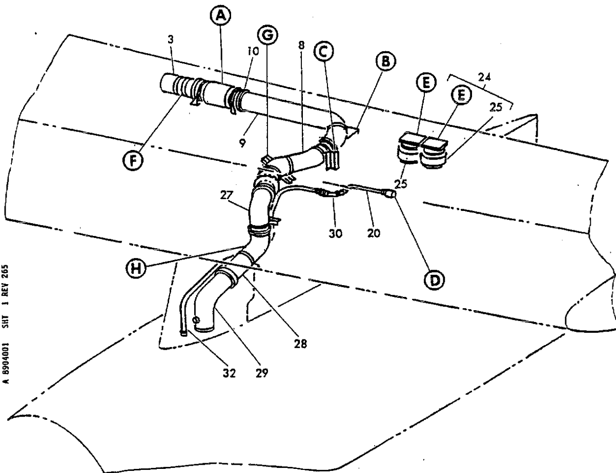
FIGURE 1. ISOLATION VALVE INSTL (SHEET 1)
