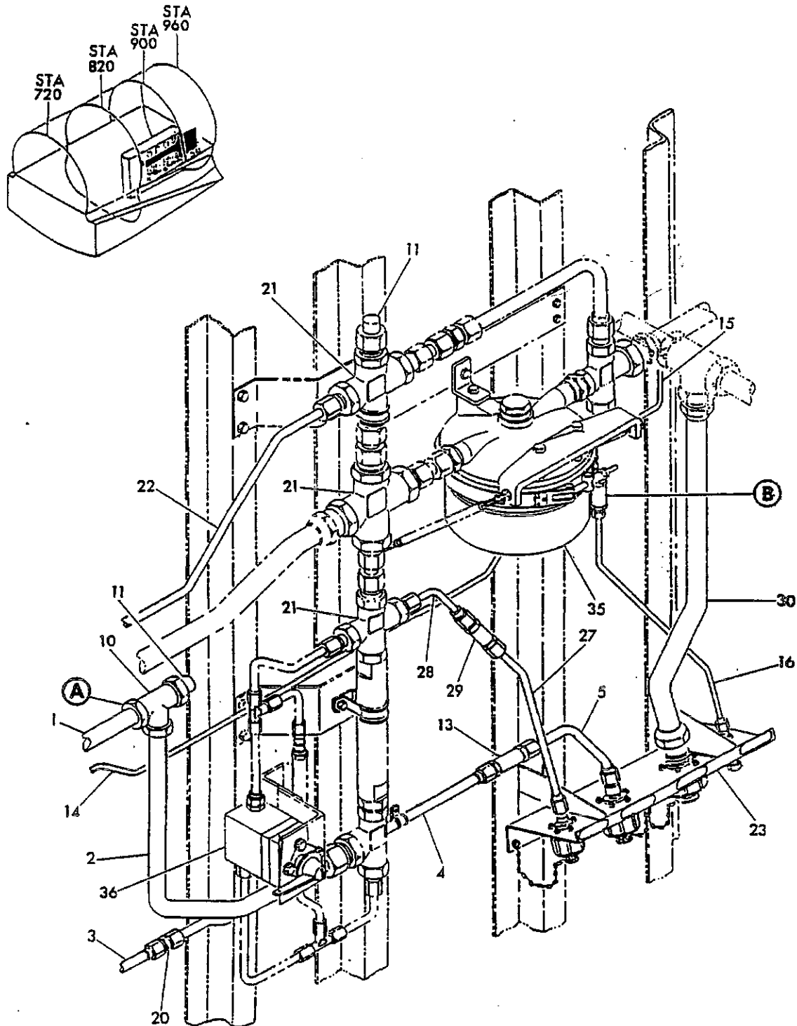
FIGURE 11. WATER TANK AREA HYDRAULIC UT II SYS INSTL. STA 820 TO 960 (SHEET 1)
