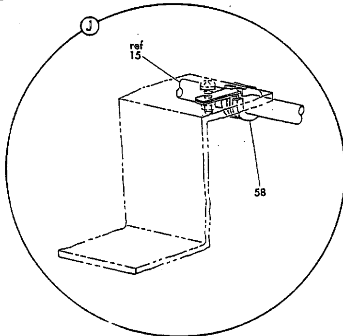
FIGURE 8. DRAIN INSTL. A/R FUEL PUMP SEAL (SHEET 6)
