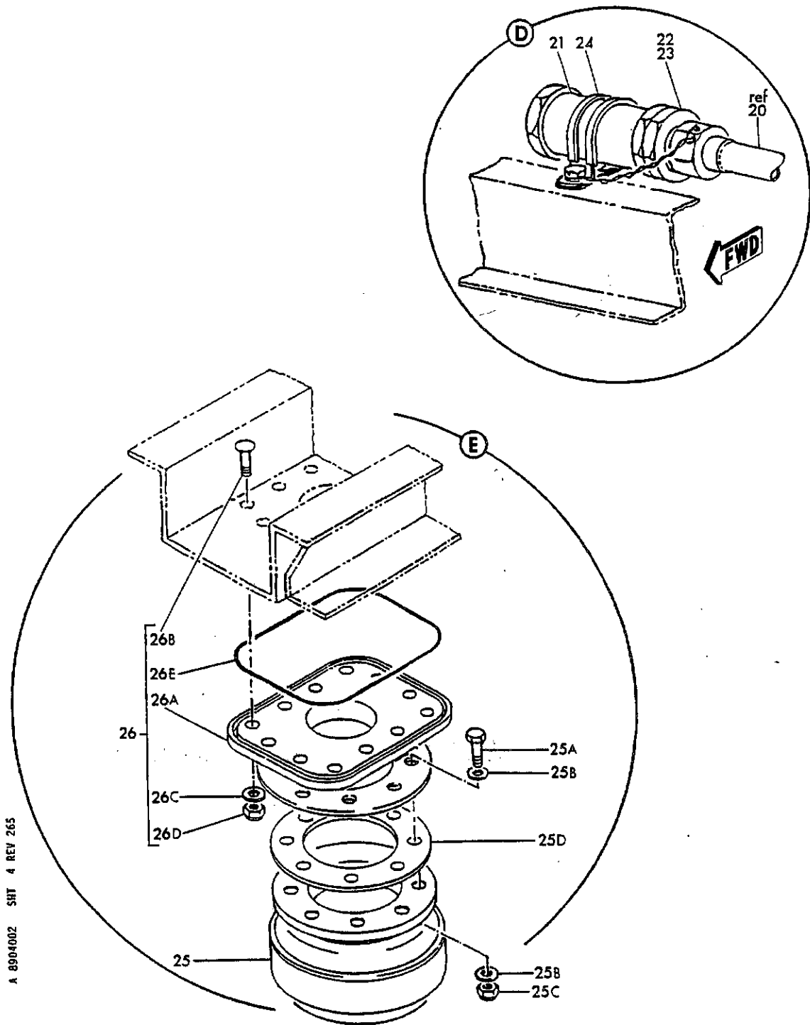
FIGURE 2. FUEL SYSTEM INSTL. WING (R.H.) A/R POD AREA (SHEET 4)
