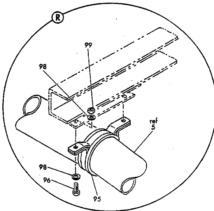
FIGURE 1. FUEL SYSTEM INSTL, SNAKE PIT AREA STA 600K TO 600F (SHEET 9)
