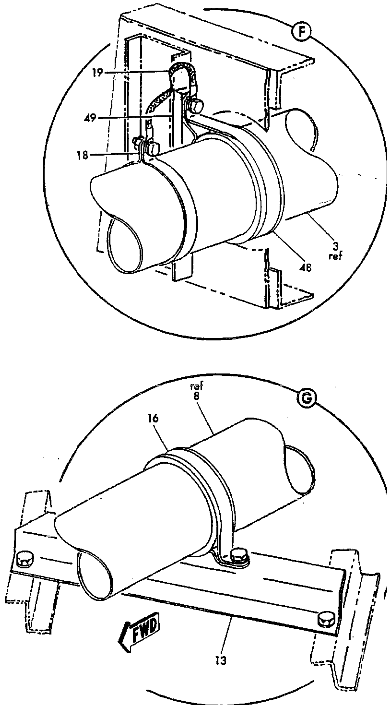
FIGURE 2. FUEL SYSTEM INSTL. WING (R.H.) A/R POD AREA (SHEET 5)
