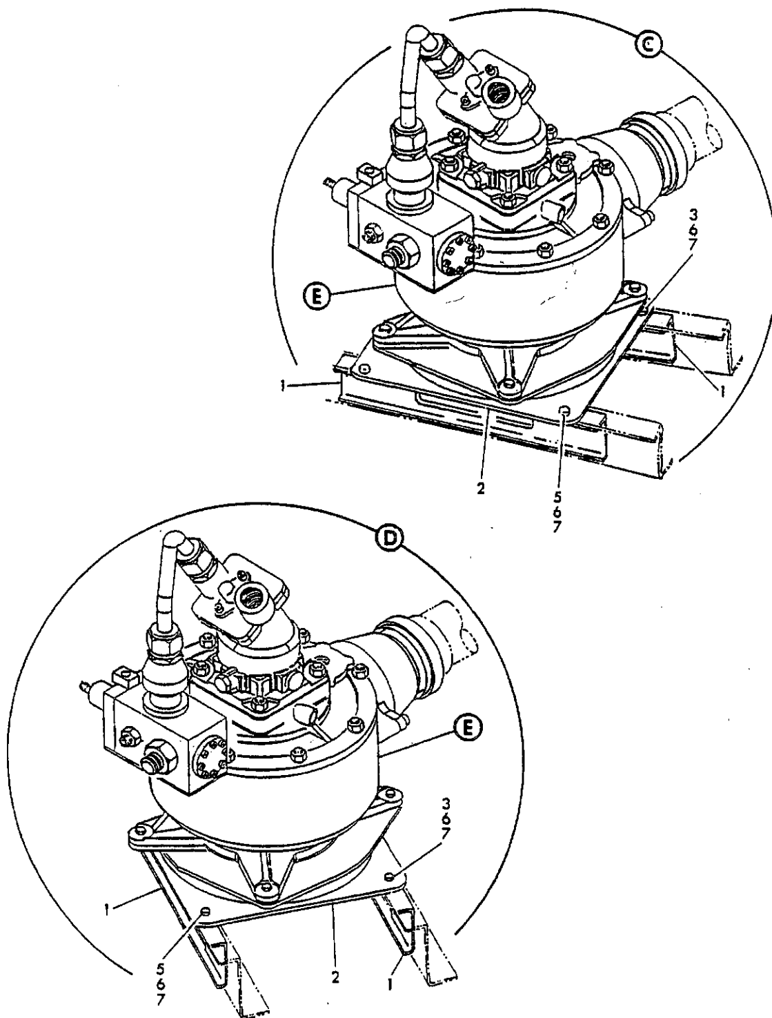
FIGURE 2. A/R FUEL PUMP INSTL. FWD (SHEET 2)
