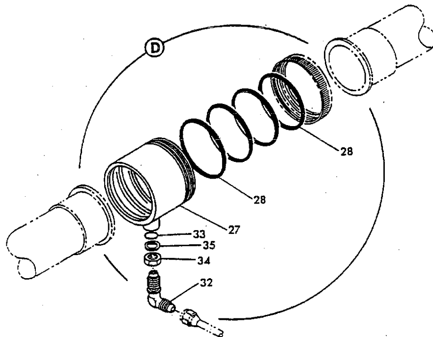
FIGURE 1. FUEL SYSTEM INSTL. SNAKE PIT AREA STA 600K TO 600F (SHEET 3)
