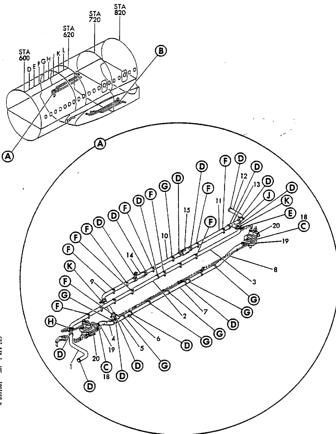
FIGURE 1. FUEL SYSTEM INSTL, WING CENTER SECTION (A/R PUMP PRESSURE LINE ONLY) (SHEET 1)
