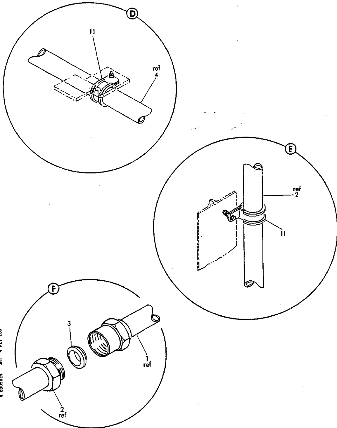
FIGURE 24. TUBE ASSY, HYDRAULIC UT II SUPPLY 1-1/4 IN. (SHEET 4)
