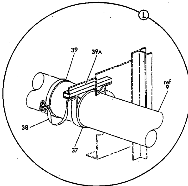
FIGURE 1. WING FUEL SYSTEM INSTL. (SHEET 7)
