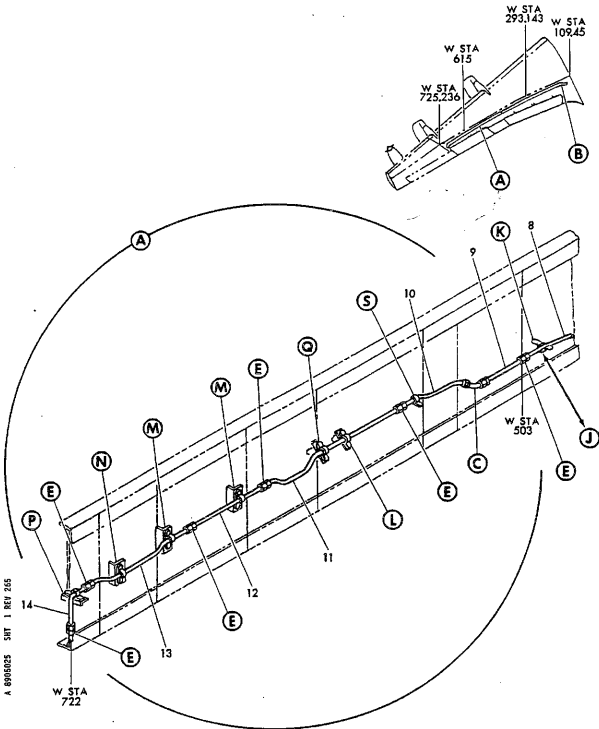
FIGURE 25. HYDRAULIC SYSTEM INSTL WING REAR SPAR (SHEET 1)
