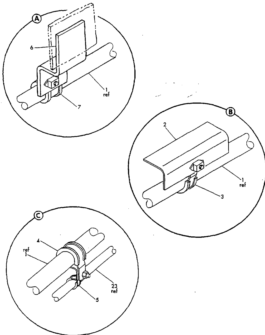
FIGURE 26. HYDRAULIC UT II INSTL, SECT 43(STA 815 TO 840 LH)(HYDRAULIC POWER ONLY)(SHEET 2)
