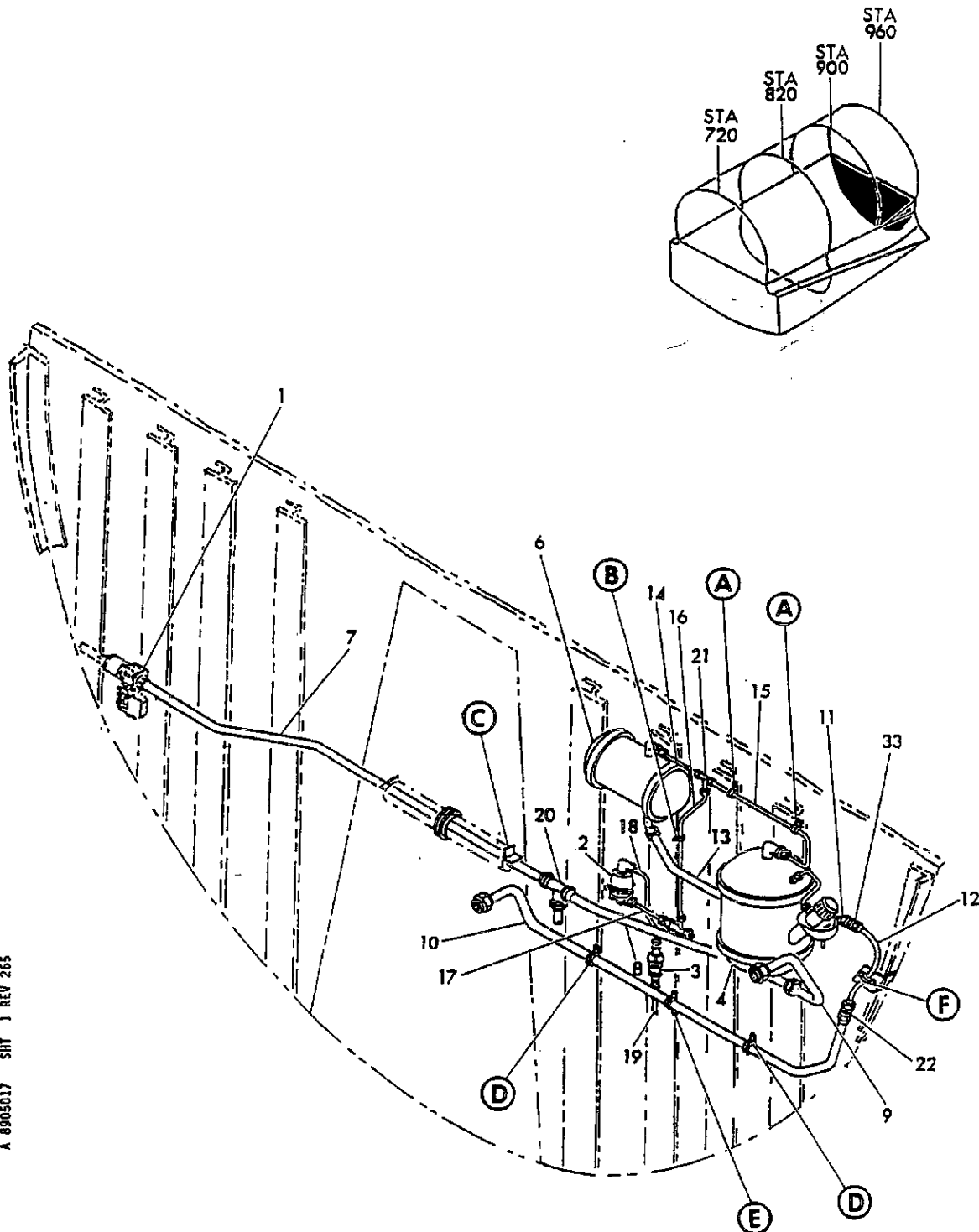
FIGURE 17. SHUT OFF VALVE 1-1/4 IN. INSTL (SHEET 1)
