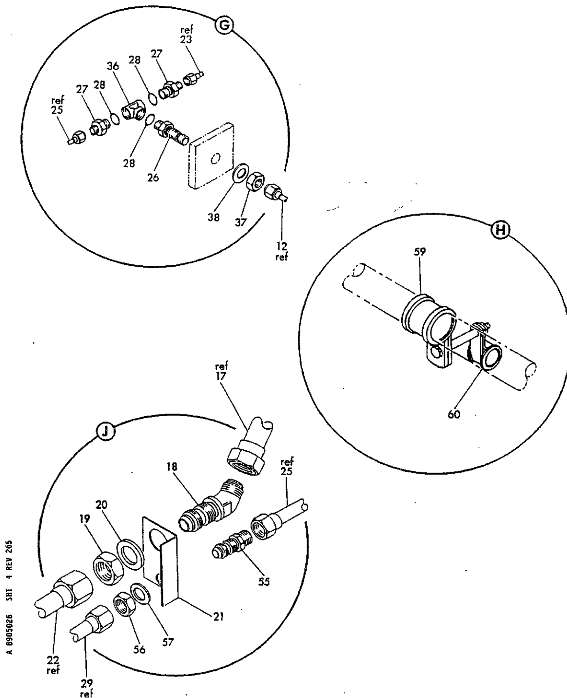
FIGURE 26. HYDRAULIC UT II INSTL. SECT 43(STA 815 TO 840 LH)(HYDRAULIC POWER ONLY)(SHEET 4)
