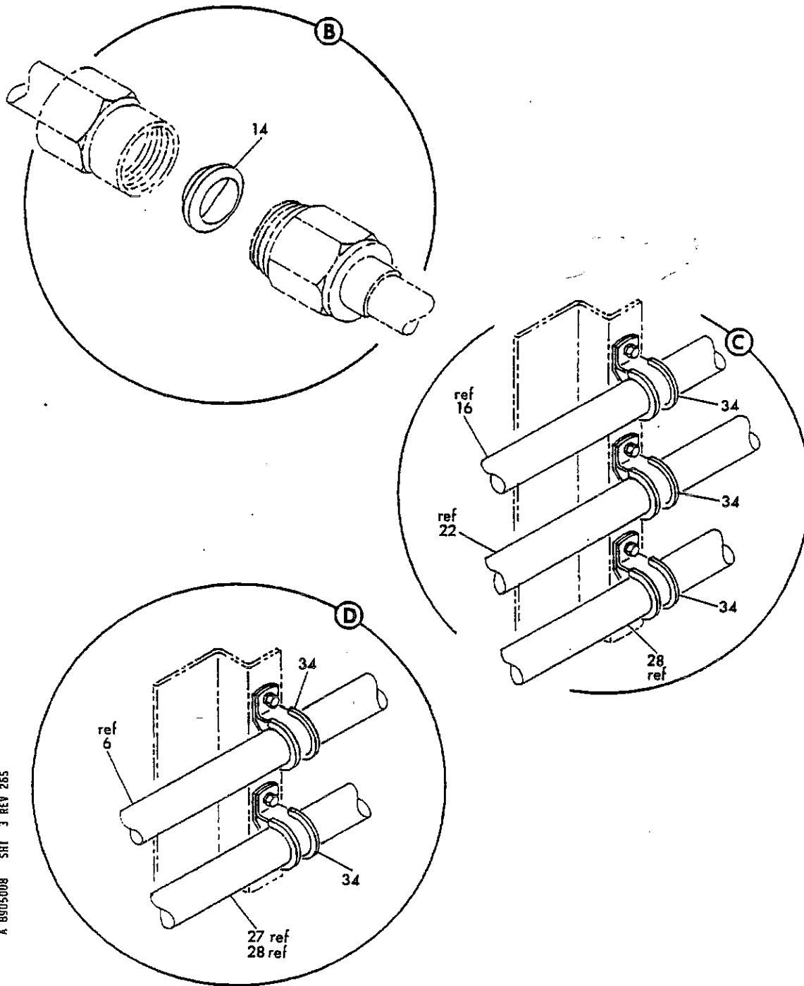
FIGURE 8. HYDRAULIC UT II SYSTEM INSTL. SNAKE PIT ONLY (SHEET 3)
