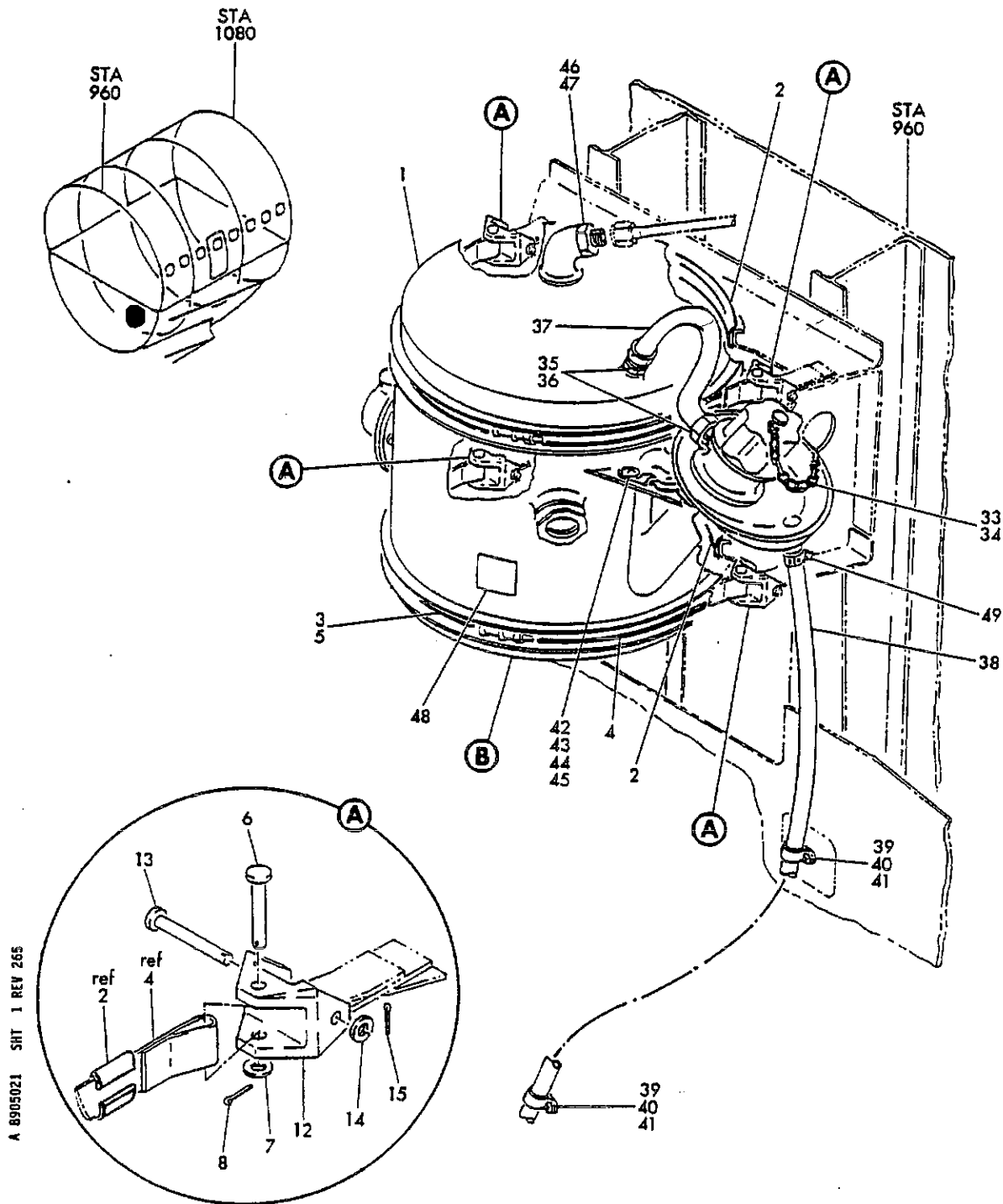
FIGURE 21. HYDRAULIC RESERVOIR INSTL (SHEET 1)
