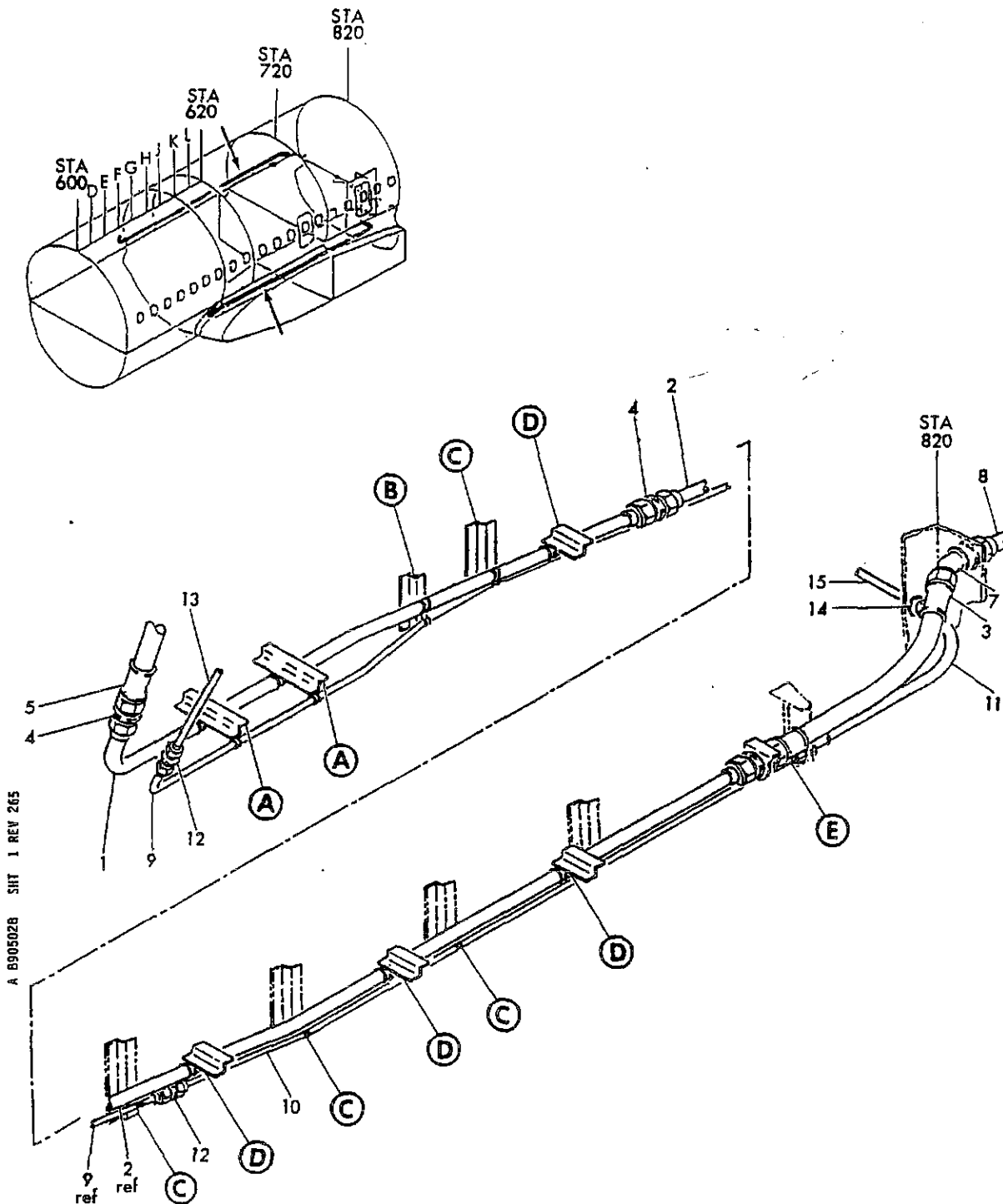
FIGURE 28. HYDRAULIC UT II INSTL. (STA 600K TO B20 L.H. AND R.H.) (HYDRAULIC POWER ONLY) (SHEET 1)
