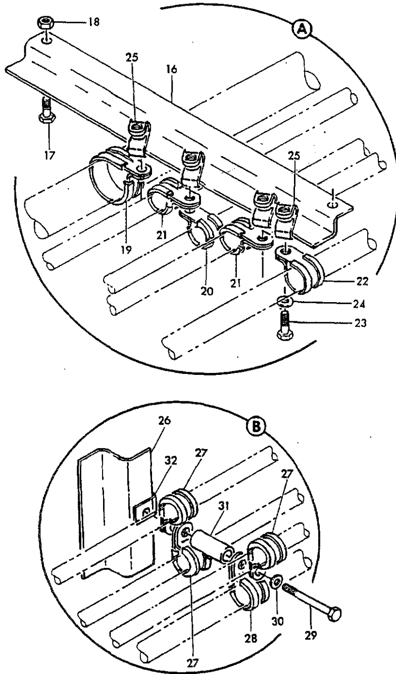
FIGURE 28. HYDRAULIC UT II INSTL. (STA 600K TO 820 L.H. AND R.H.)(HYDRAULIC POWER ONLY)(SHEET 2)
