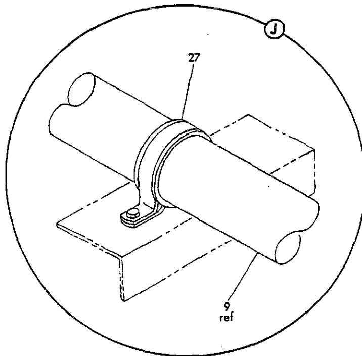
FIGURE 1. FUEL SYSTEM INSTL. WING CENTER SECTION (A/R PUMP PRESSURE LINE ONLY) (SHEET 5)
