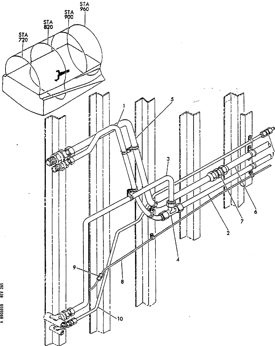
FIGURE 10. WATER TANK WALL AREA HYDRAULIC SYSTEM INSTL, F.S. 820 TO F.S. 870
