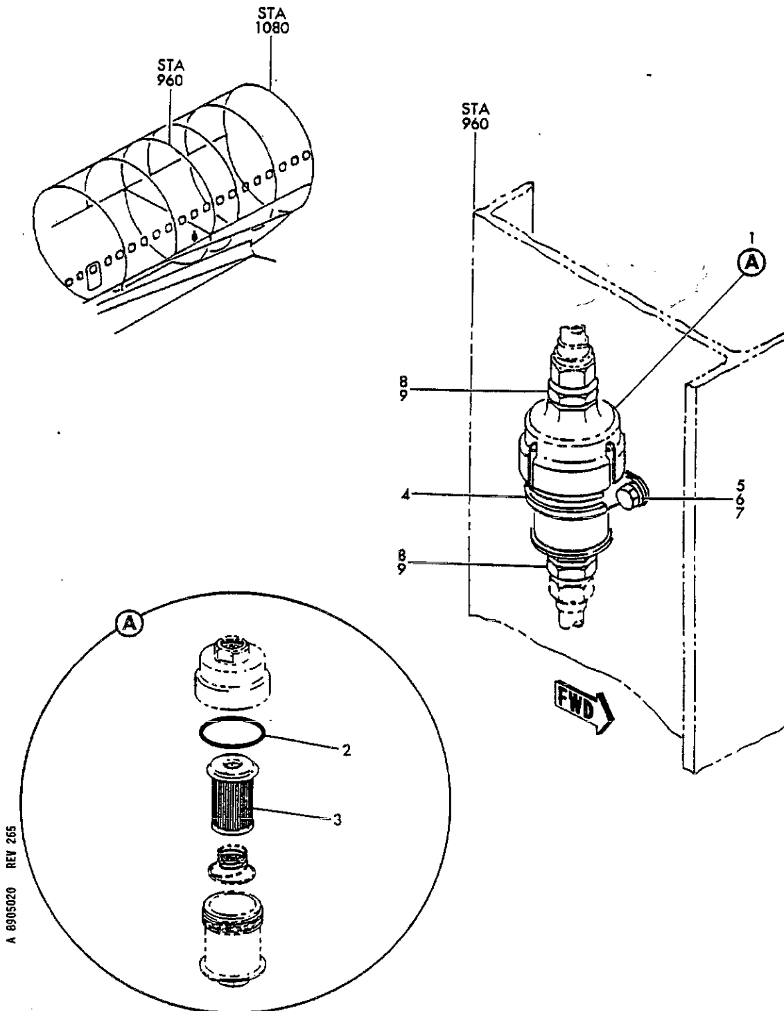
FIGURE 20. AIR FILTER INSTL
