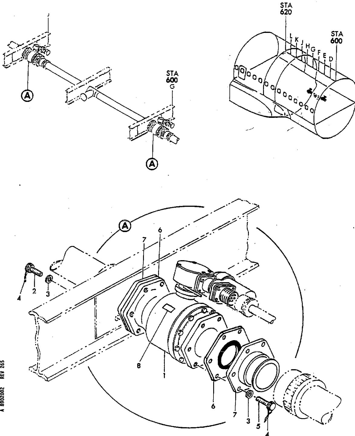
FIGURE 2. VALVE INSTL, FUEL INTERCONNECT
