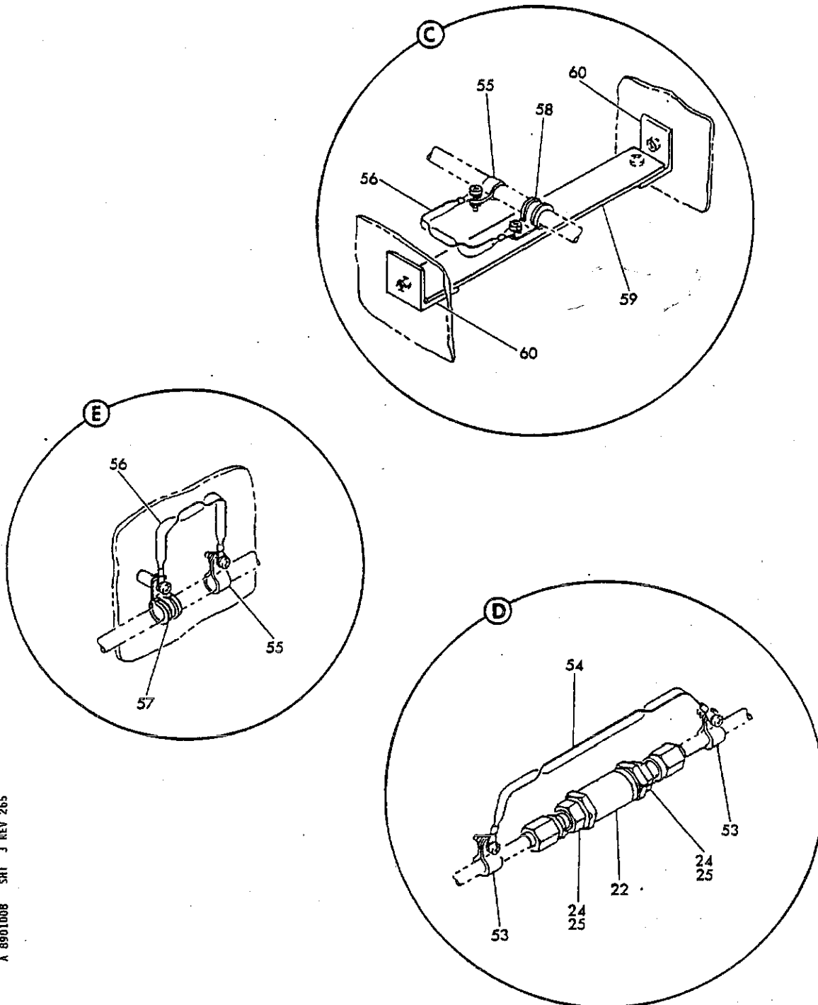
FIGURE 8. DRAIN INSTL. A/R FUEL PUMP SEAL (SHEET 3)
