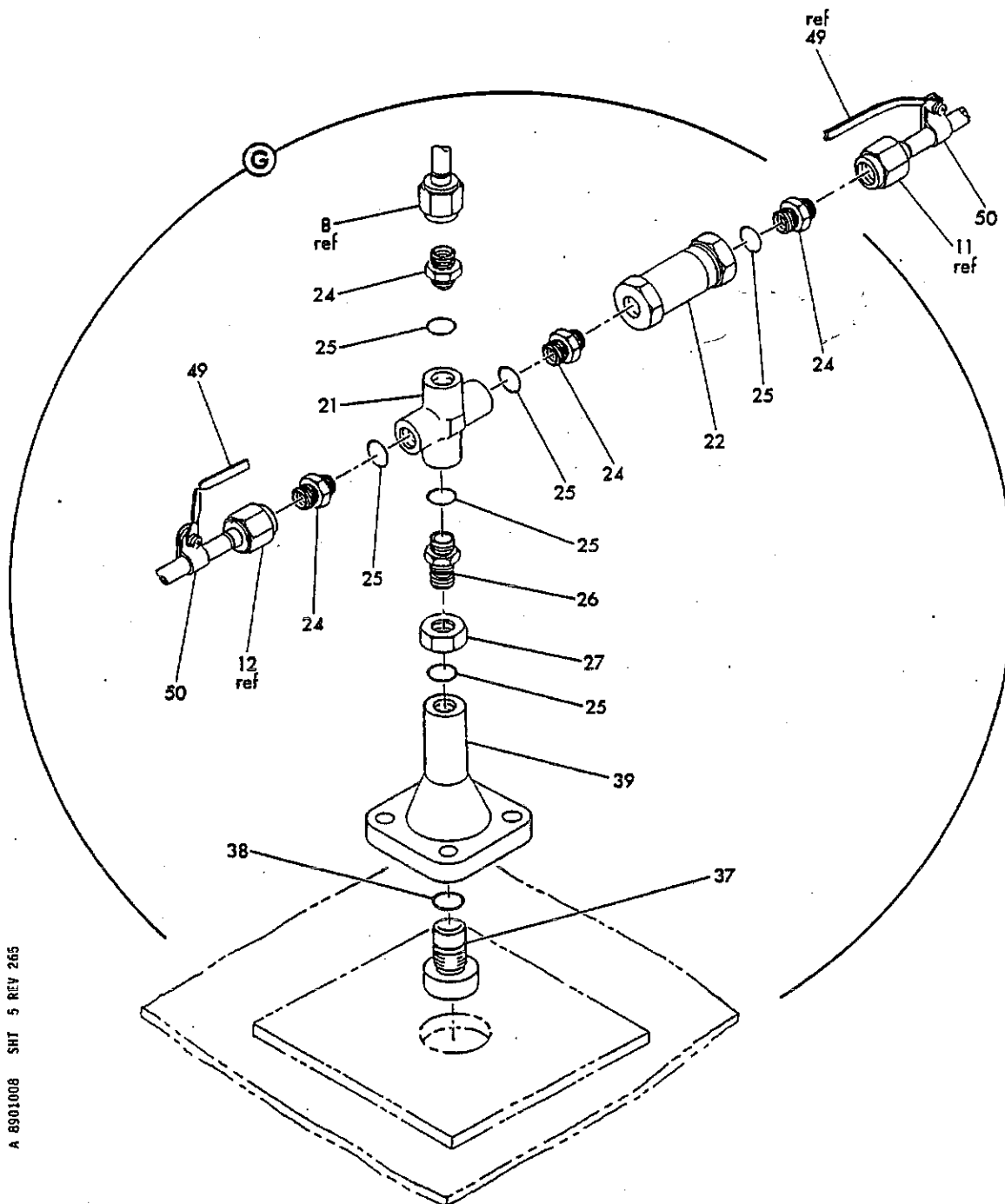
FIGURE 8. DRAIN INSTL, A/R FUEL PUMP SEAL (SHEET 5)
