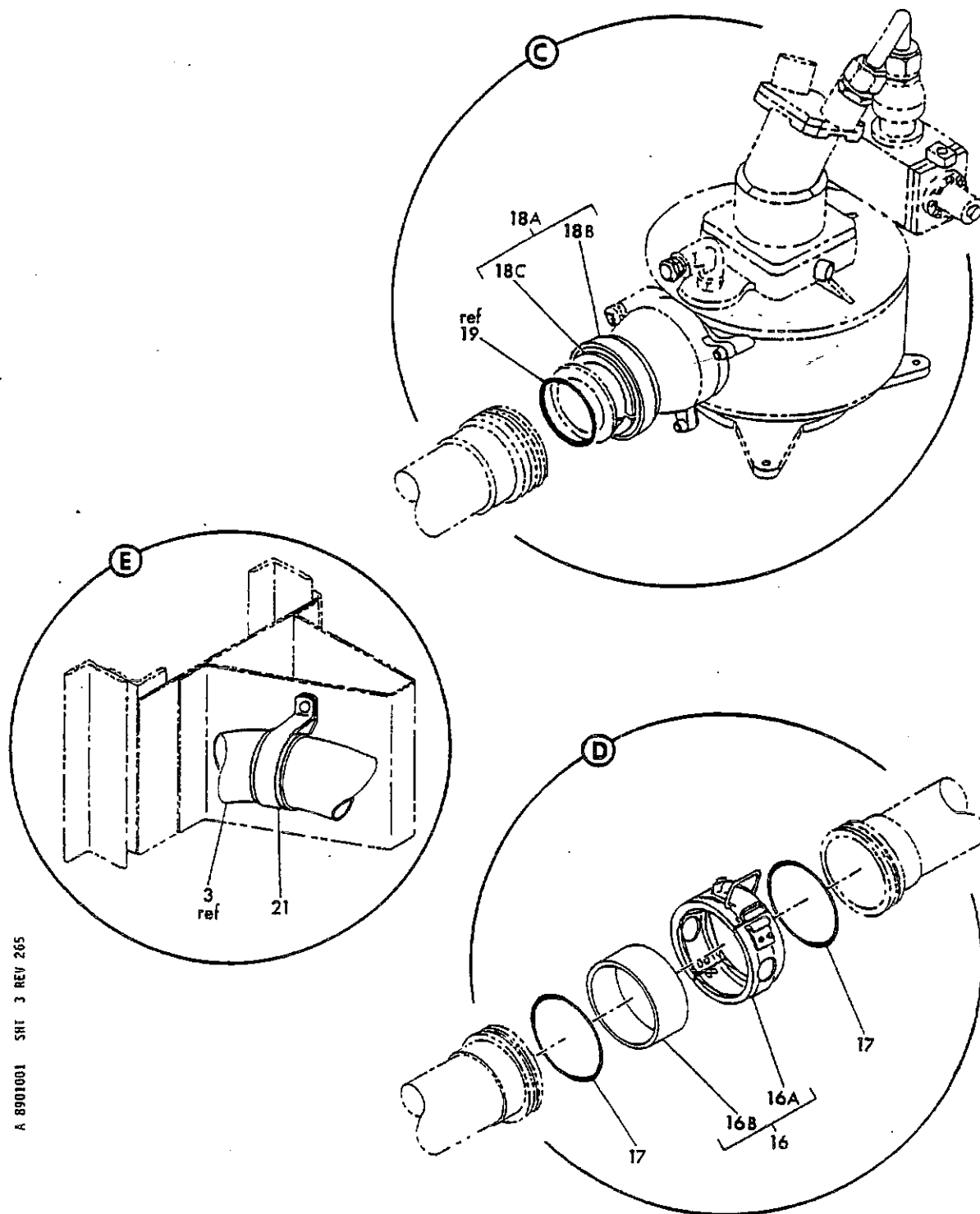
FIGURE 1. FUEL SYSTEM INSTL, WING CENTER SECTION (A/R PUMP PRESSURE LINE ONLY) (SHEET 3)
