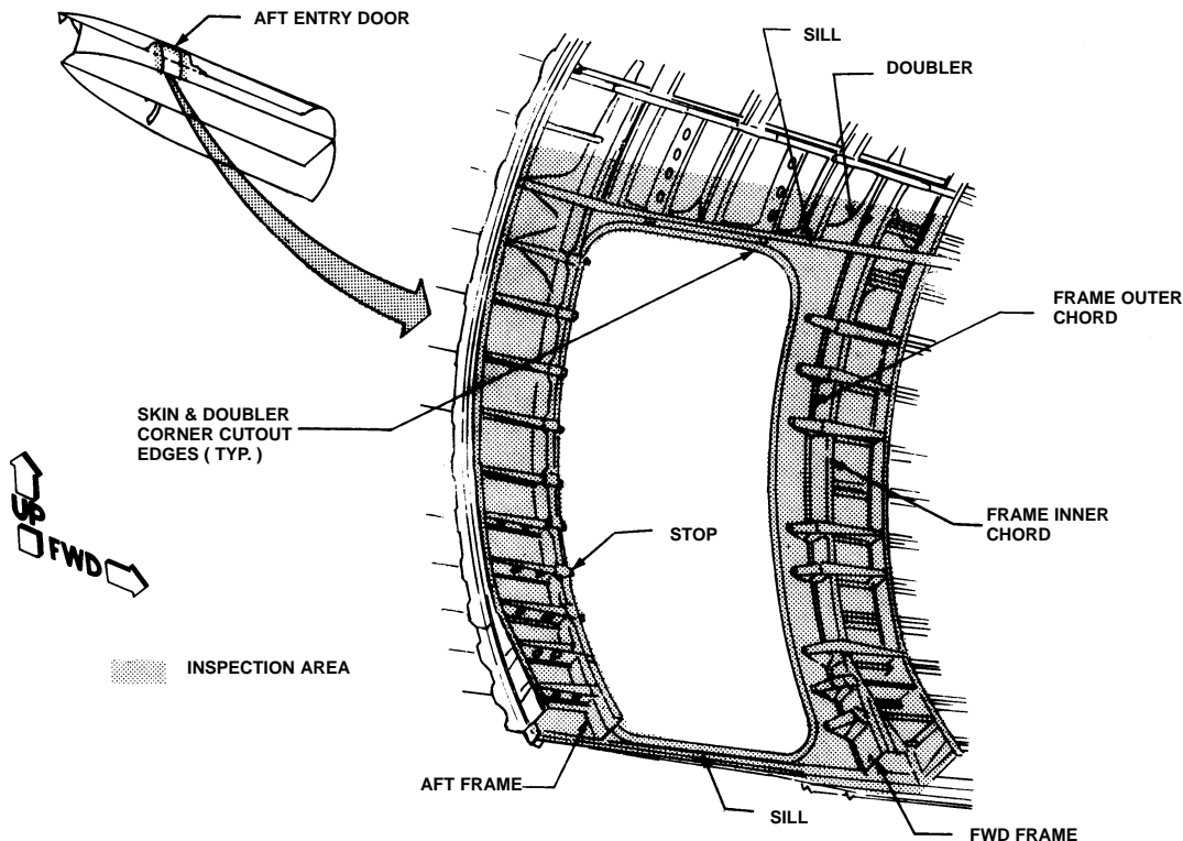
FUSELAGE AFT ENTRY DOOR CUTOUT INSPECTION
