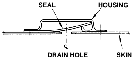
ORIGINAL DRAIN VALVE
