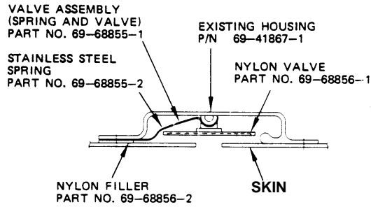
IMPROVED DRAIN VALVE
