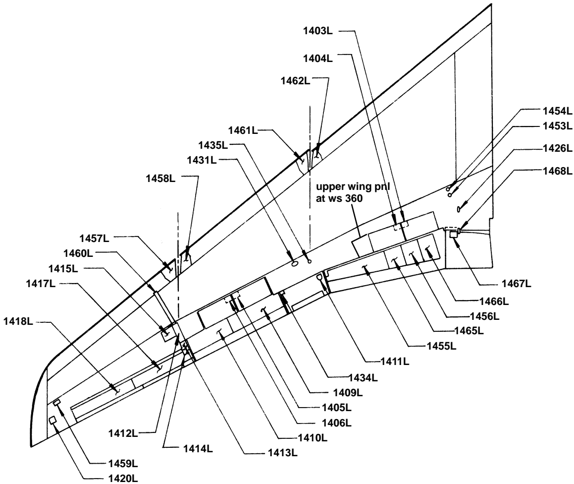
LH UPPER WING SURFACE
