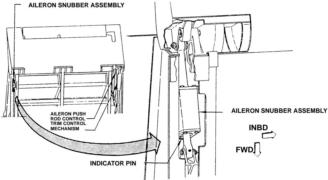
AILERON SNUBBER ASSEMBLY INSTALLATION
