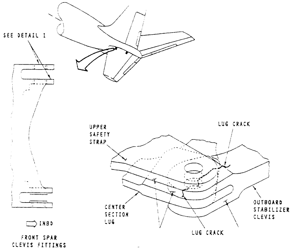
FIGURE 3. UPPER CLEVIS UPPER LUG INSPECTION
