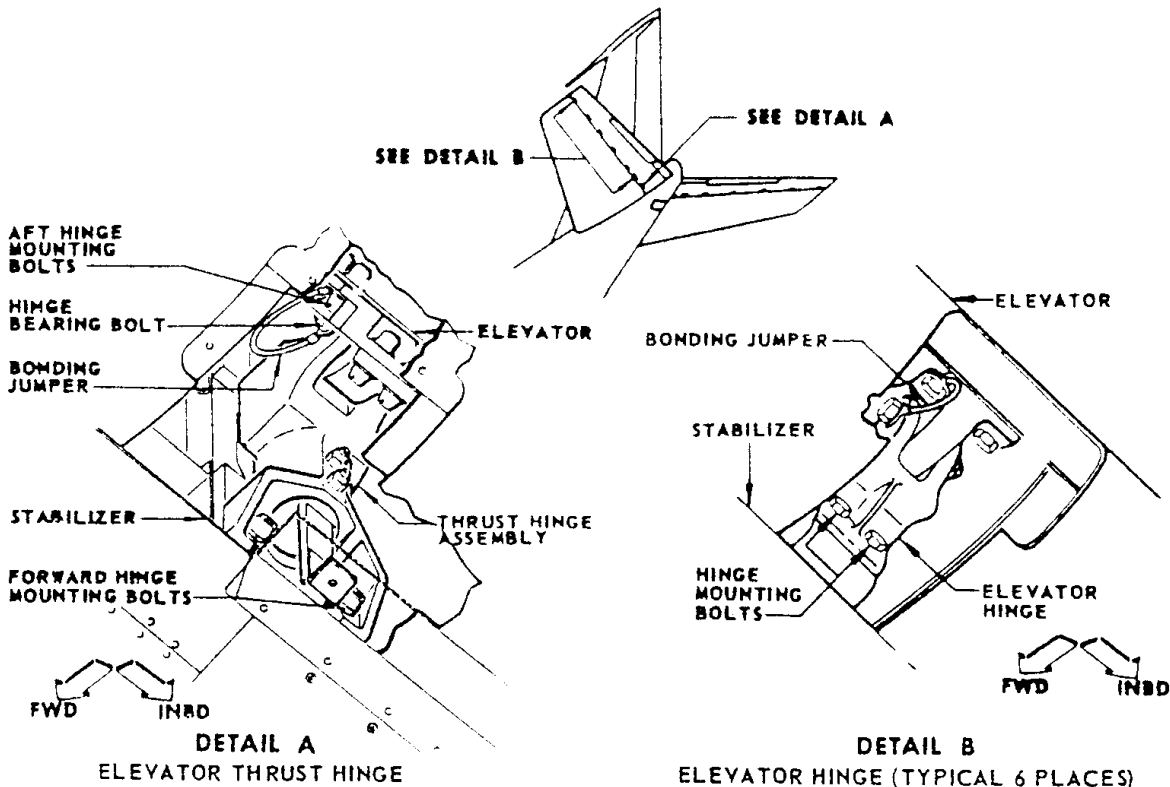
Elevator Hinge Attachment
