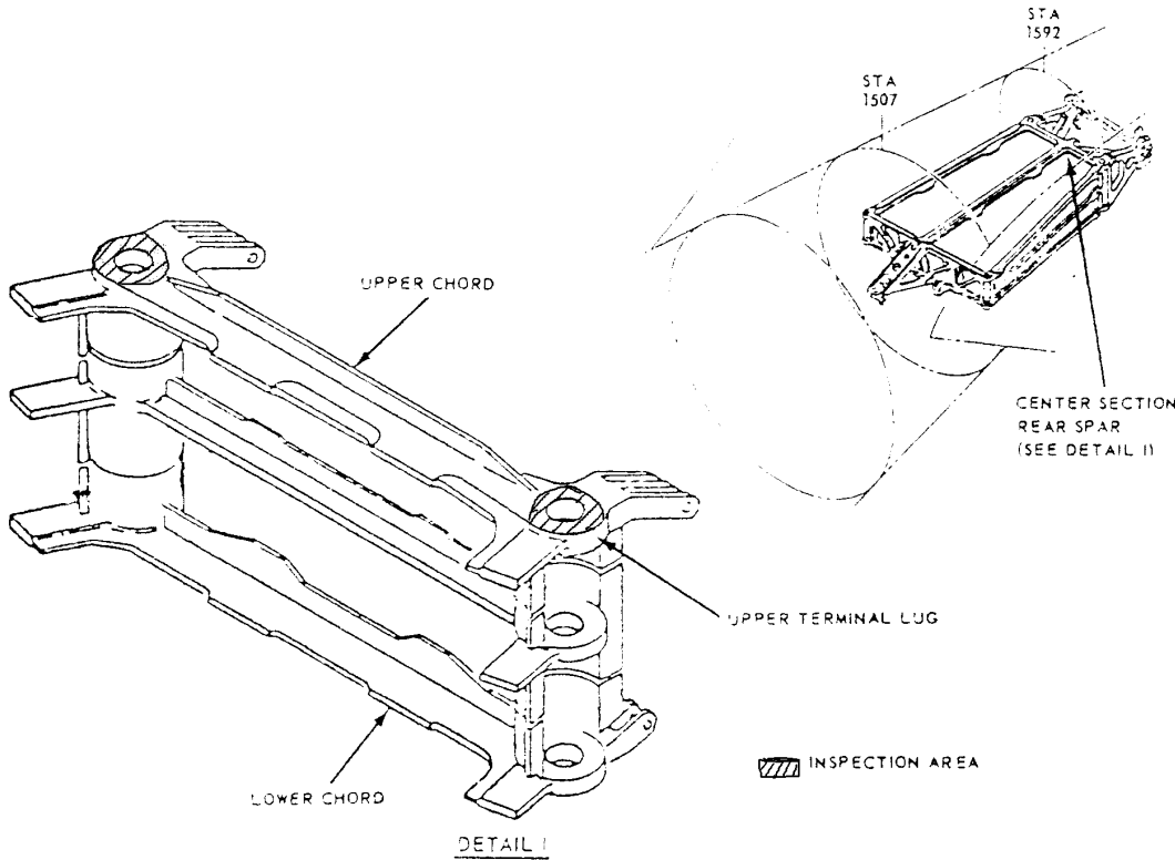
HORIZONTAL STABILIZER CENTER SECTION REAR SPAR LUG INSPECTION
