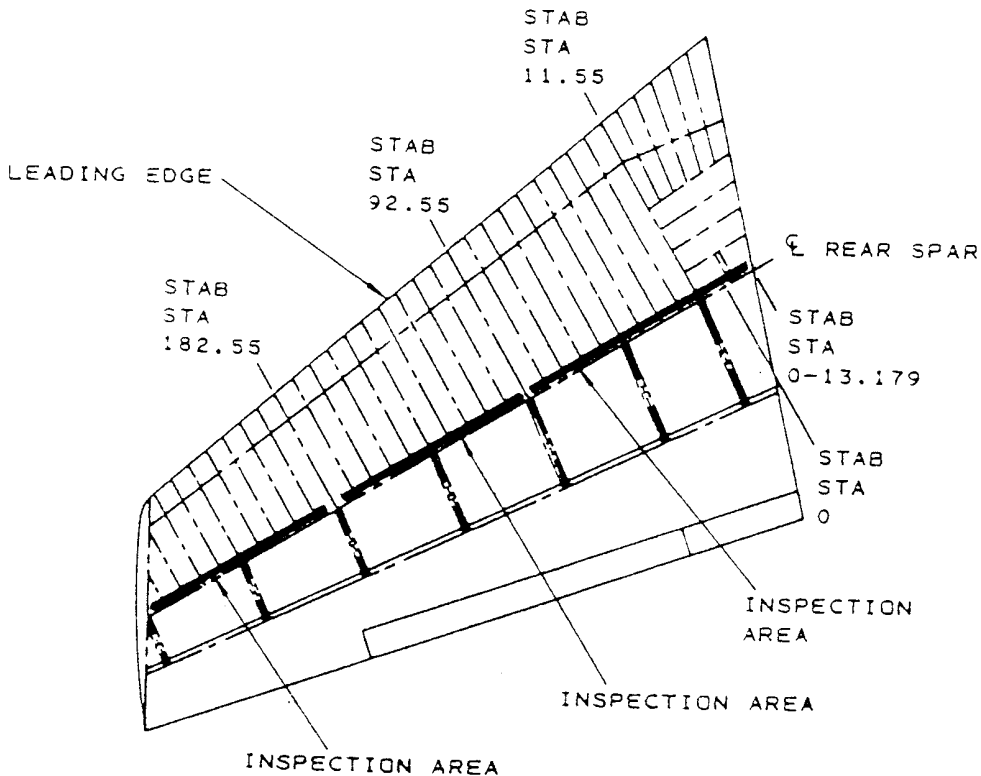
PLAN VIEW HORIZONTAL STABILIZER
