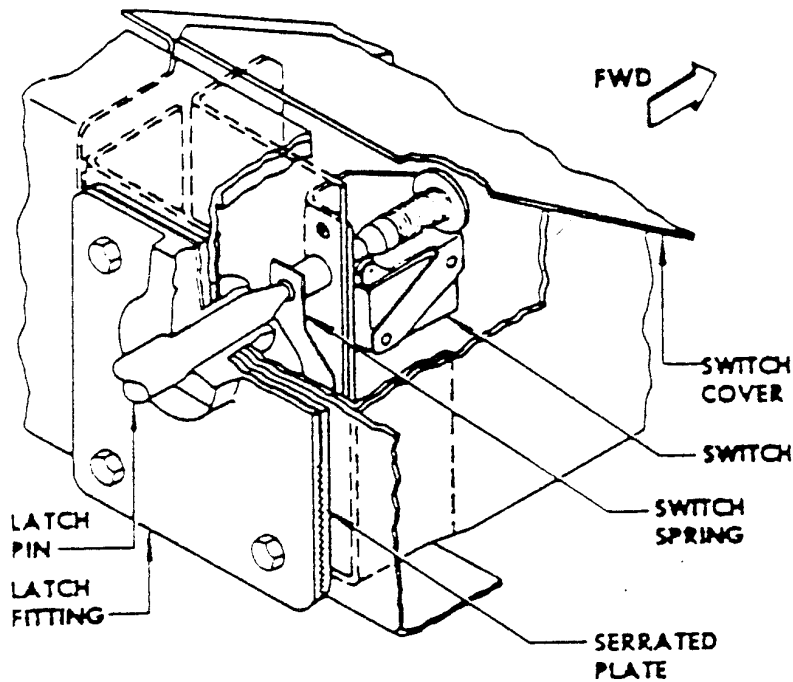
ELECTRONIC COMPARTMENT EXTERNAL DOOR SWITCH INSTALLATION
