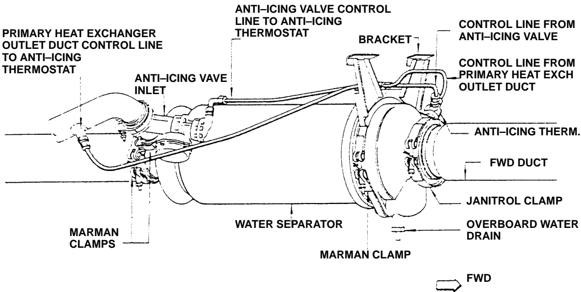
WATER SEPARATOR INSTALLATION
