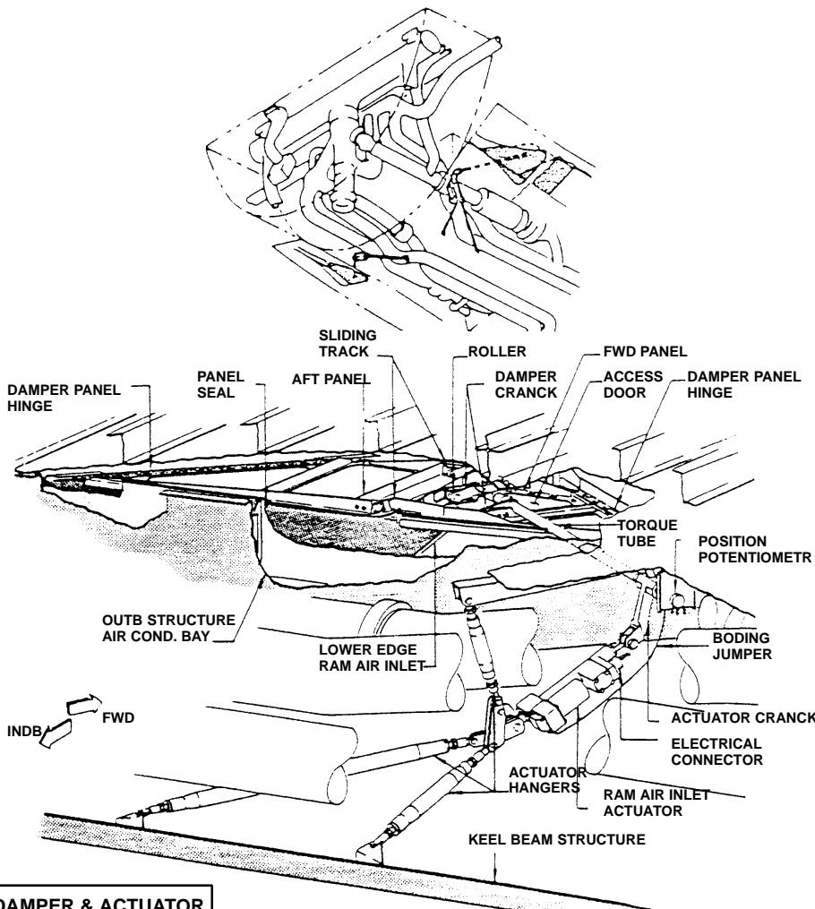
RAM AIR INLET DAMPER & ACTUATOR
