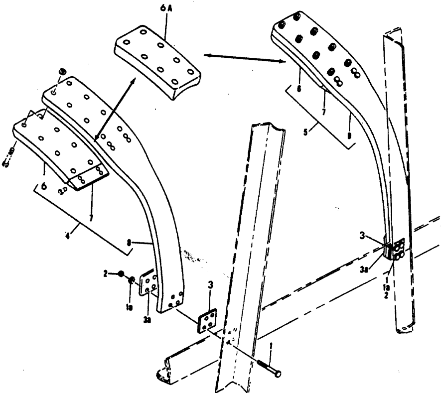
SEE NOTE ON PARTS LIST PAGES FIGURE 19. BRAKE INSTL, NOSE GEAR WHEEL SNUBBER
