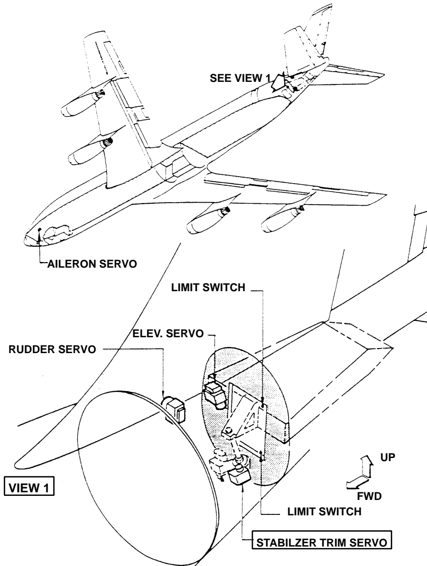
AUTOPILOT FLIGHT CONTROL COMPONENTS LOCATION
