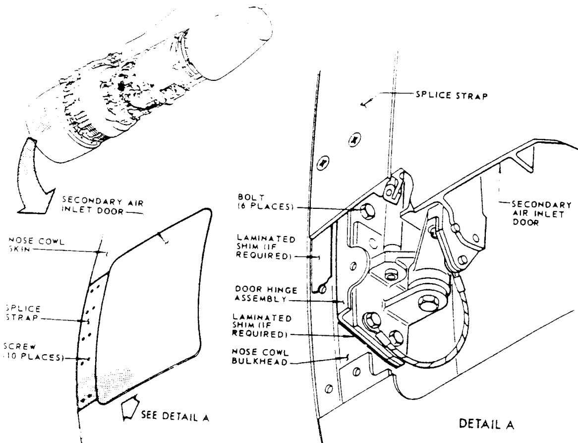
Secondary Air Inlet Door Installation
