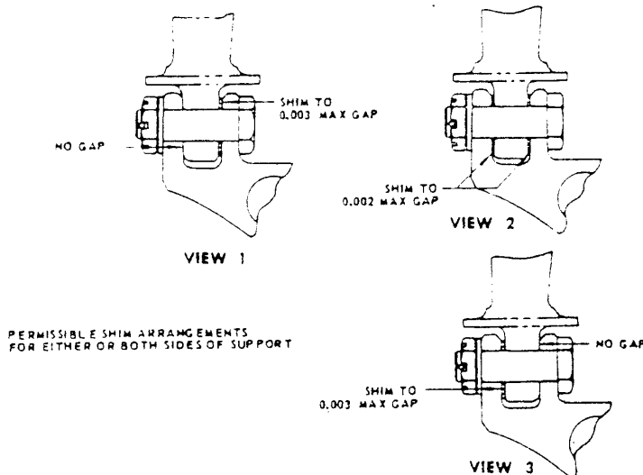
Engine Rear Mount Support
