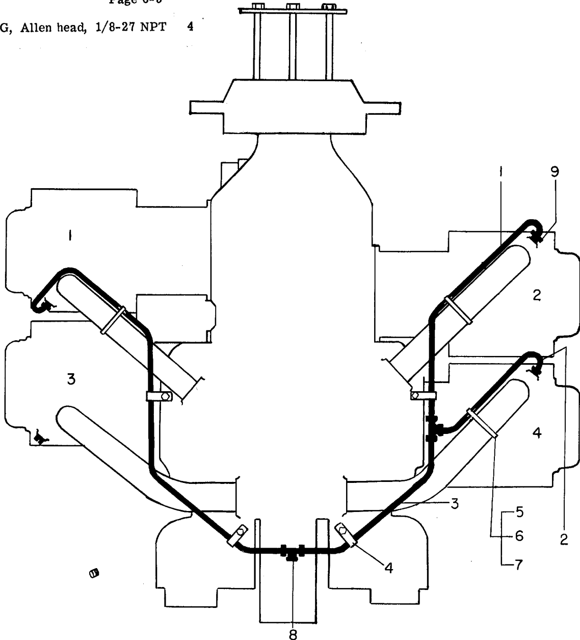
Figure 6-5. Priming System
