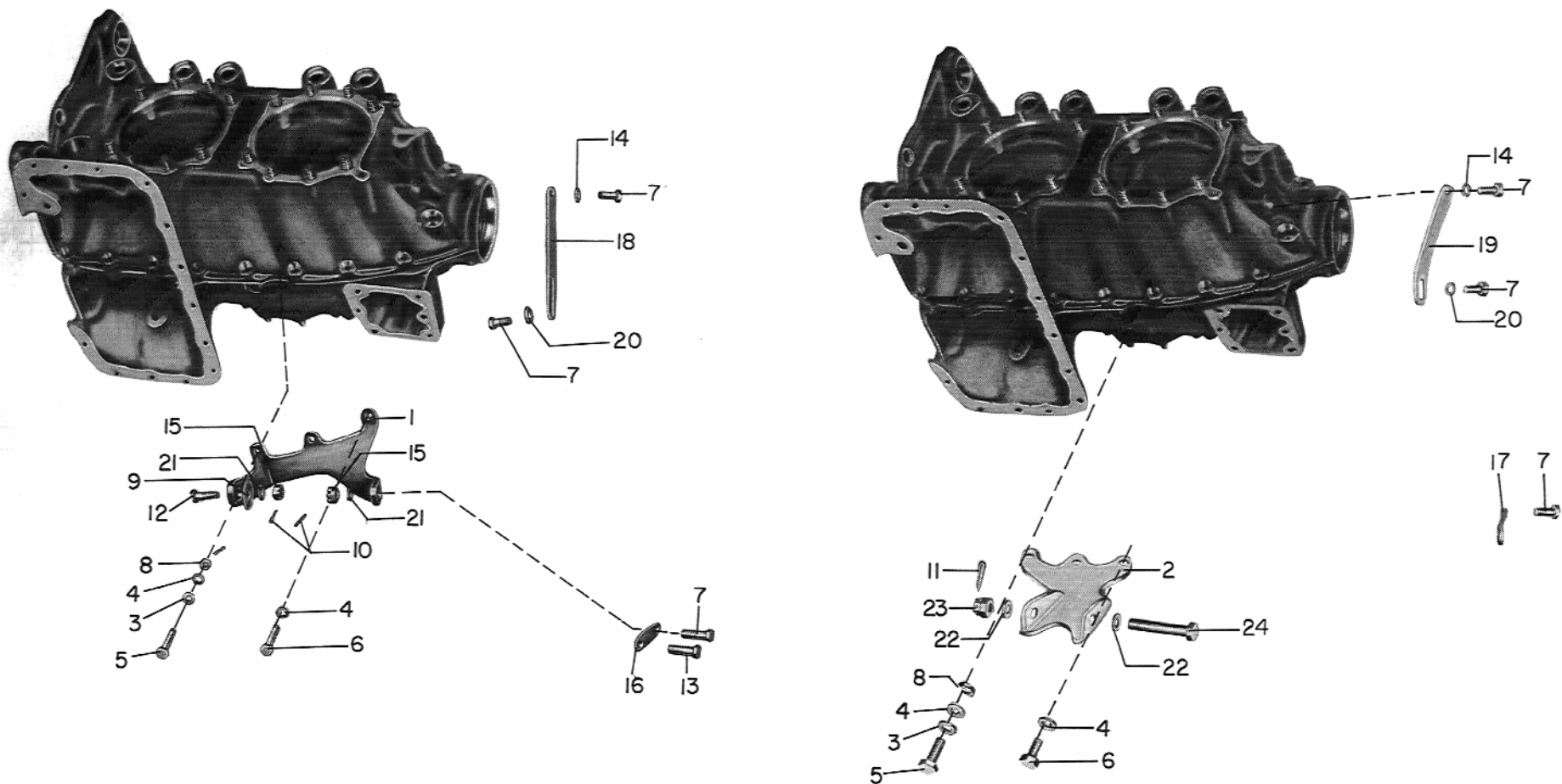
Figure 5-1. Generator/Alternator Bracket - Std. Cylinder Flange Engines
