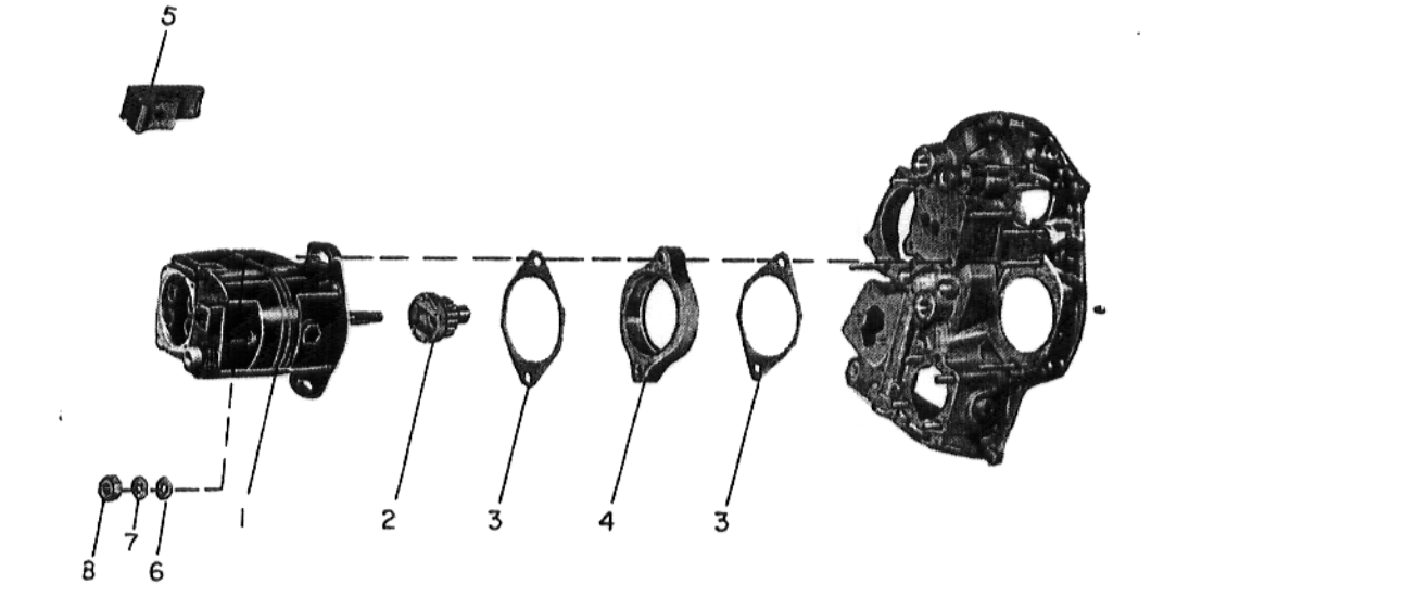
Figure 4-1. Magnetos
