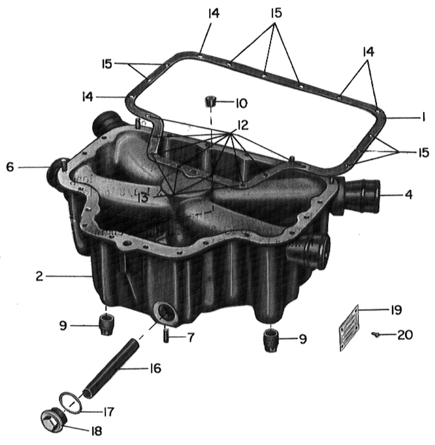
Figure 2-9. Sump Assembly
