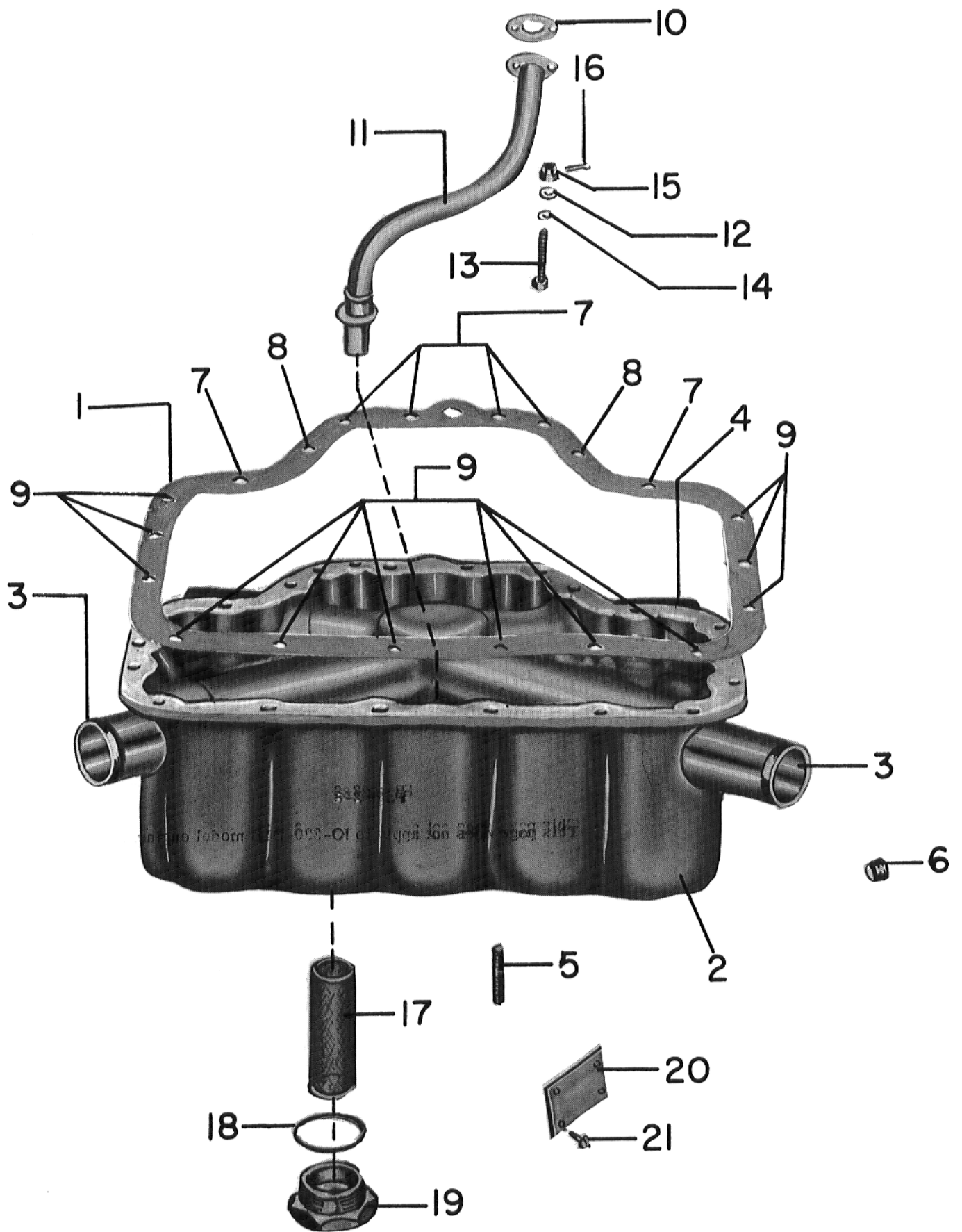
Figure 2-8. Sump Assembly
